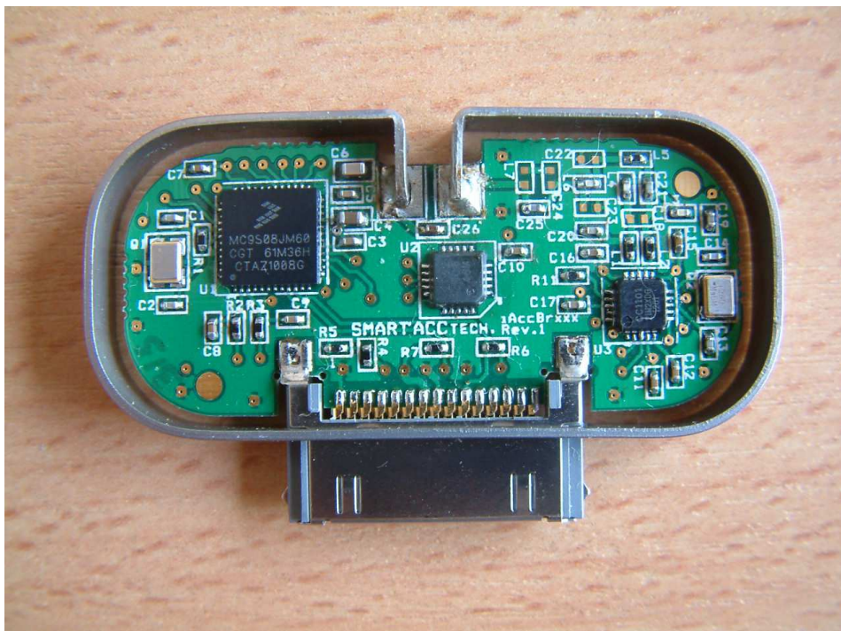
PCB view, with integral antenna
