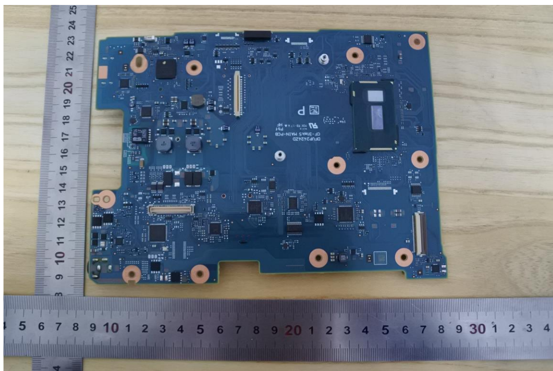
Internal View of EUT-40
