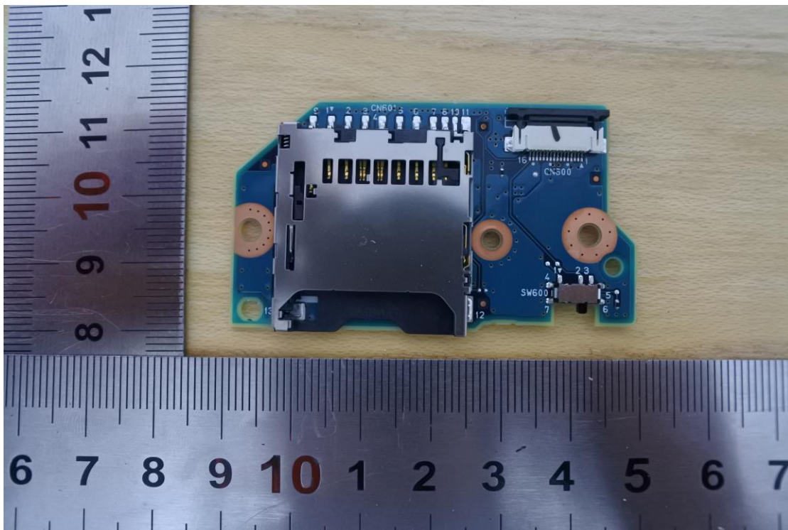
Internal View of EUT-37
