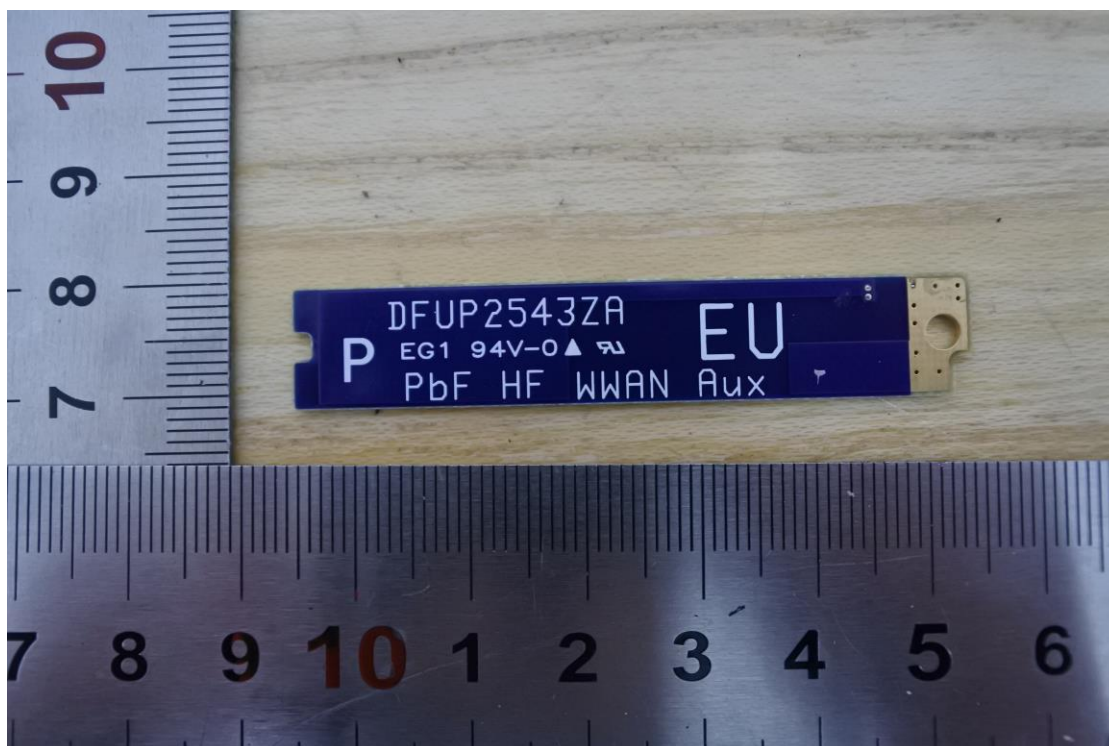
Internal View of EUT-34
