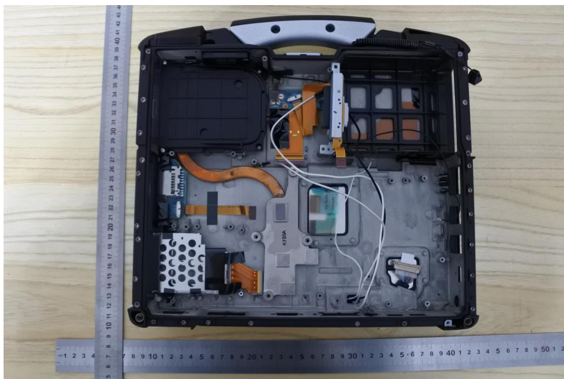
Internal View of EUT-30
