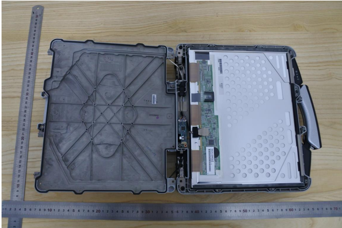
Internal View of EUT-43
