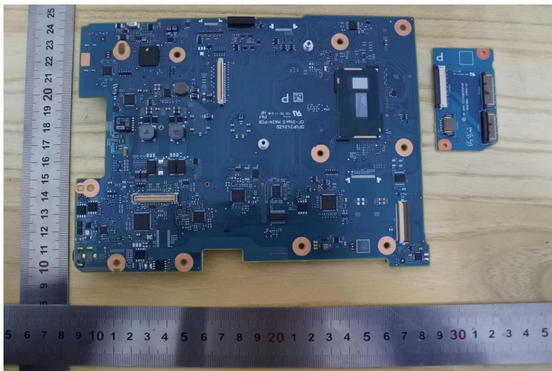
Internal View of EUT-39
