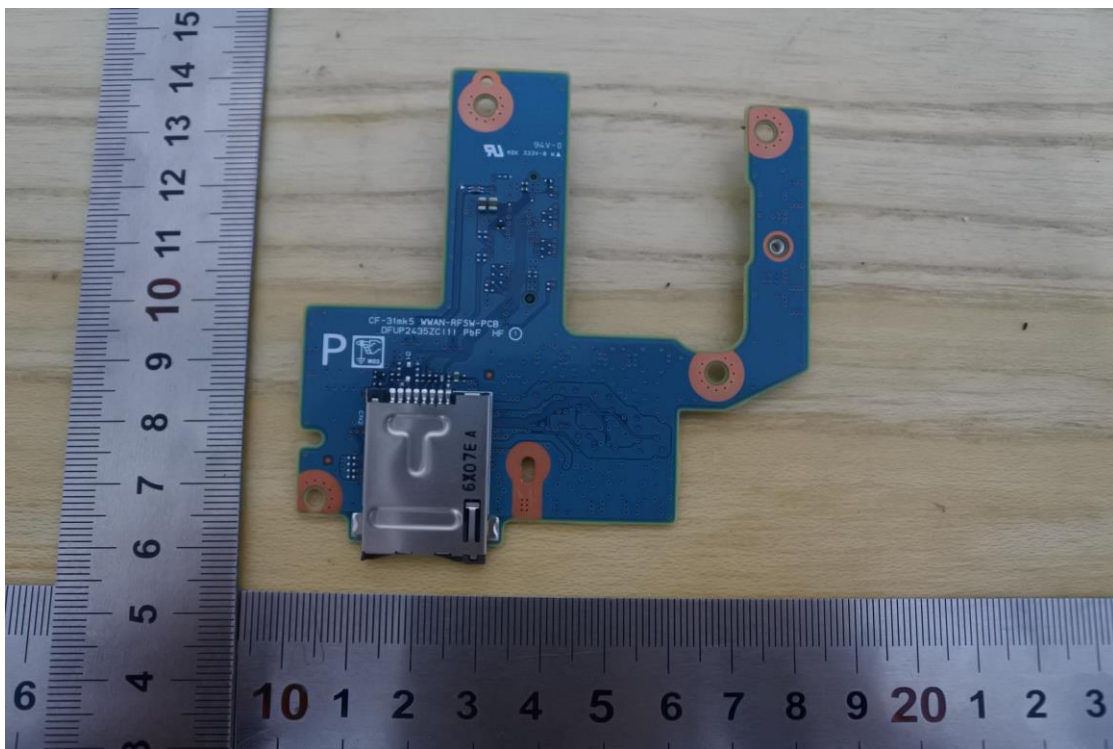
Internal View of EUT-50
