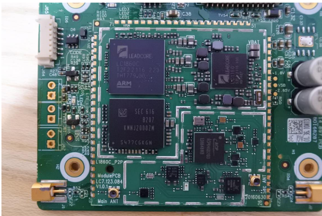
Internal View of EUT-15
