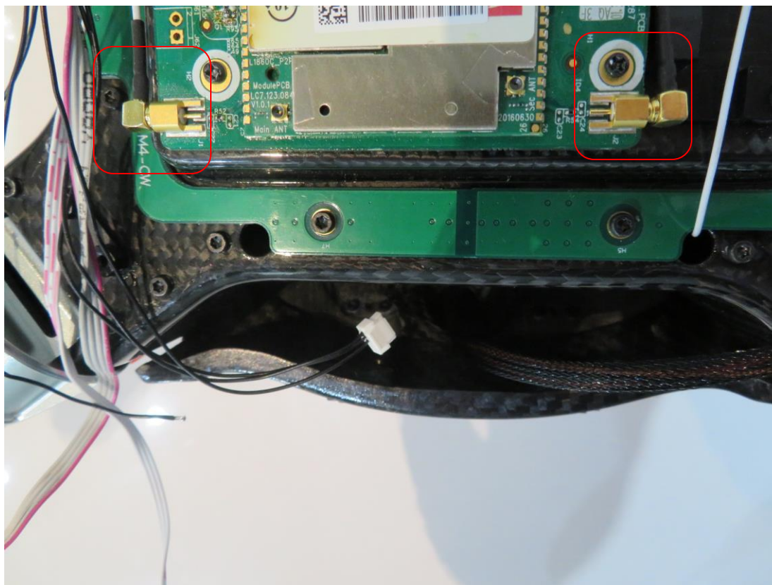
Internal View of RF Connector-1
