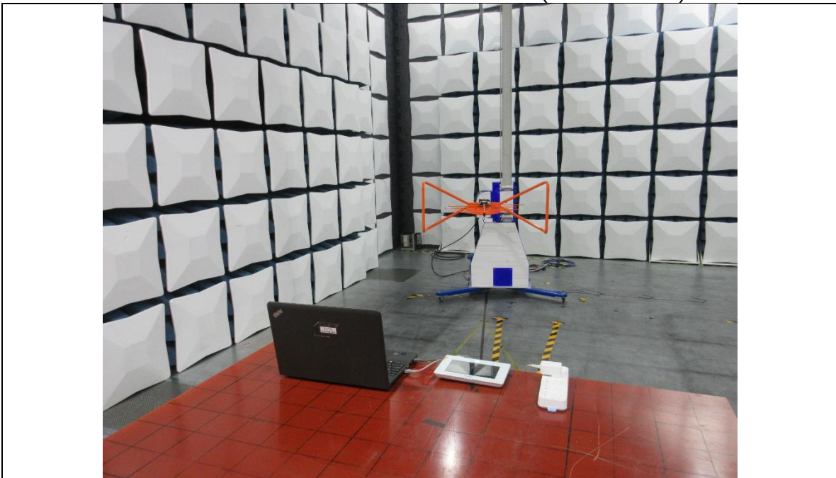
RADIATED RF MEASUREMENT SETUP (30MHz~1GHz)
