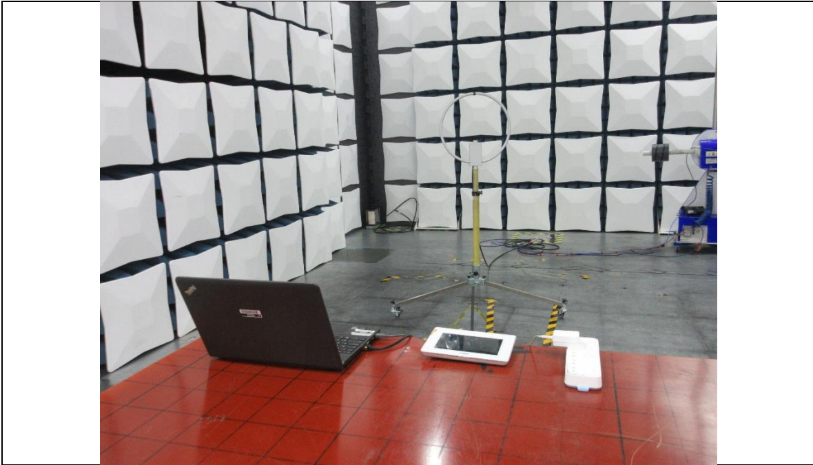
RADIATED RF MEASUREMENT SETUP (Below 30MHz)
