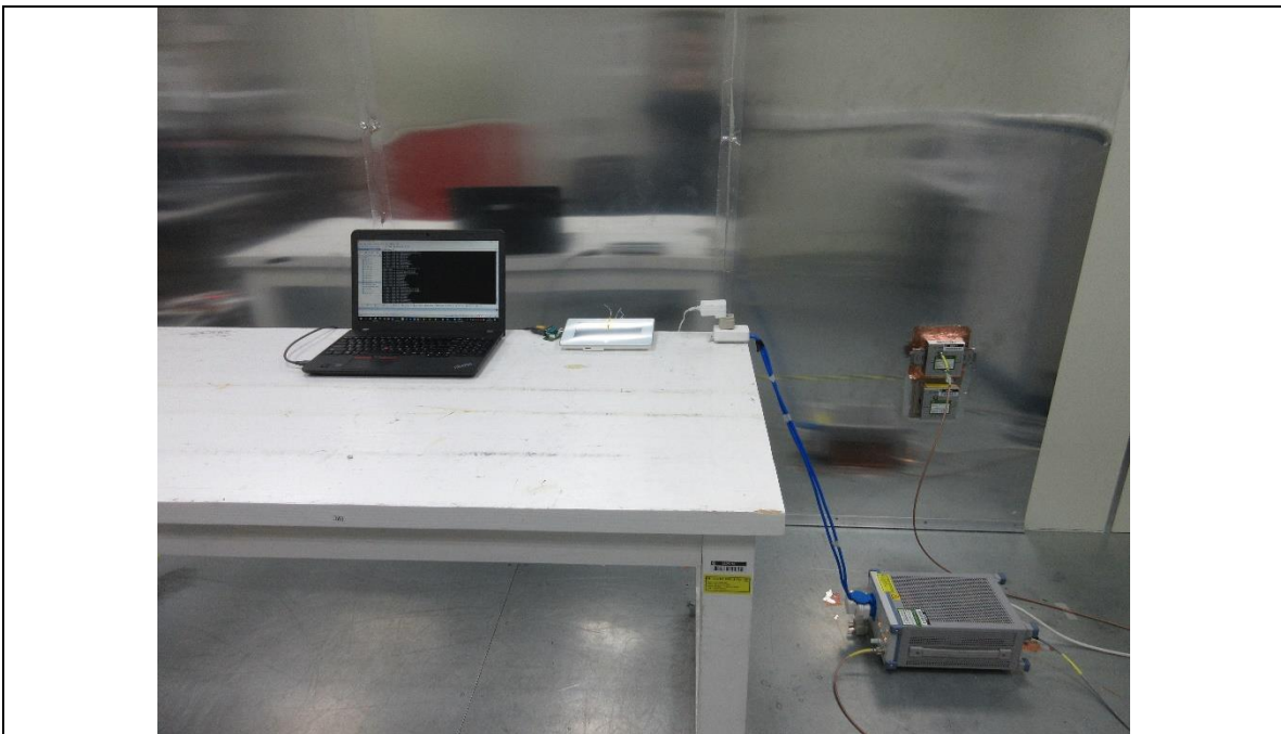
POWERLINE CONDUCTED EMISSIONS MEASUREMENT SETUP
