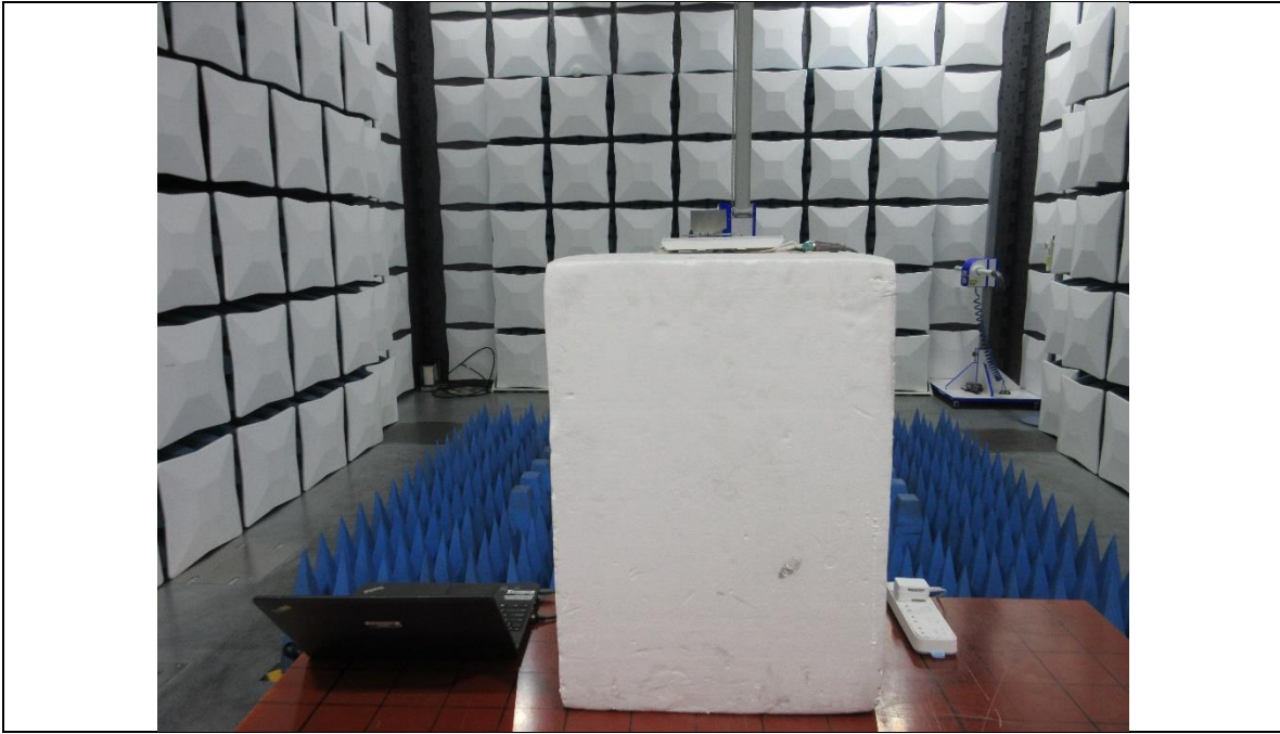
RADIATED RF MEASUREMENT SETUP (ABOVE 1 GHz- X axis)
