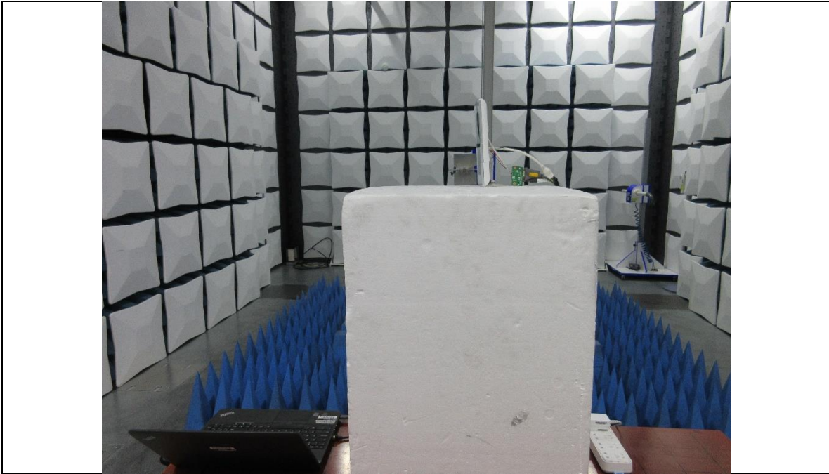
RADIATED RF MEASUREMENT SETUP (ABOVE 1 GHz- Z axis)
