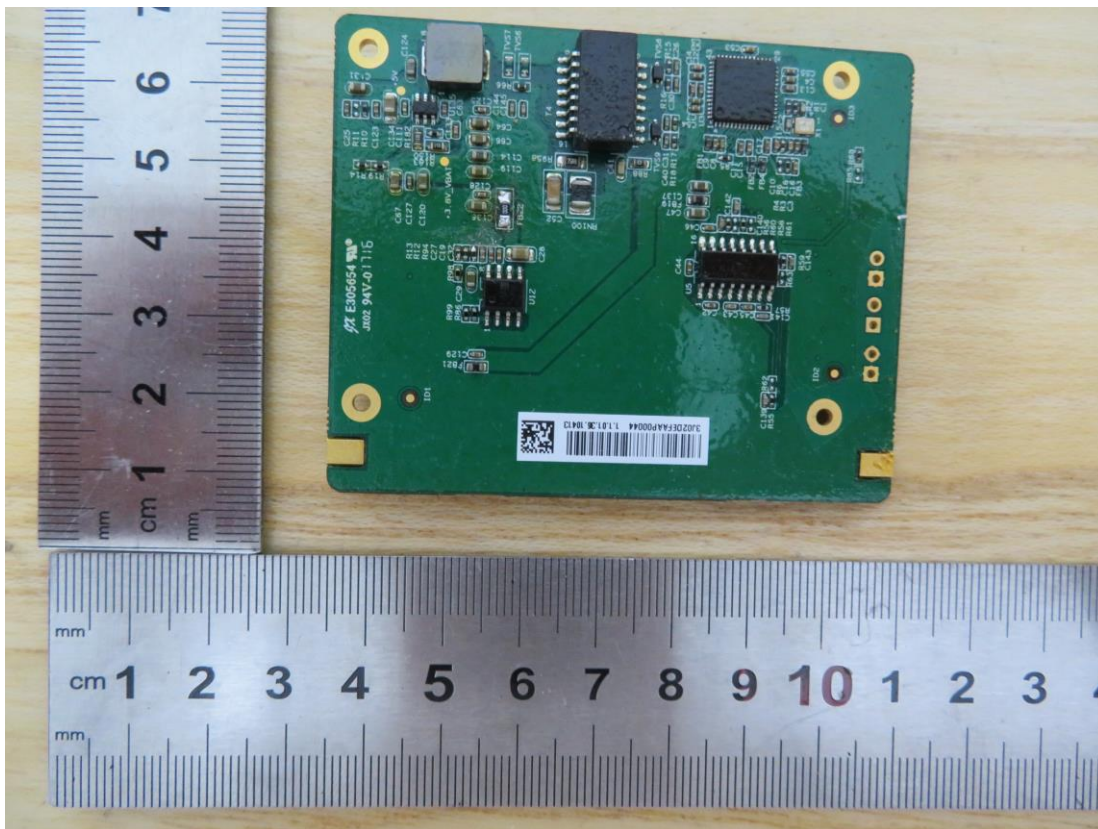
Internal View of EUT-32
