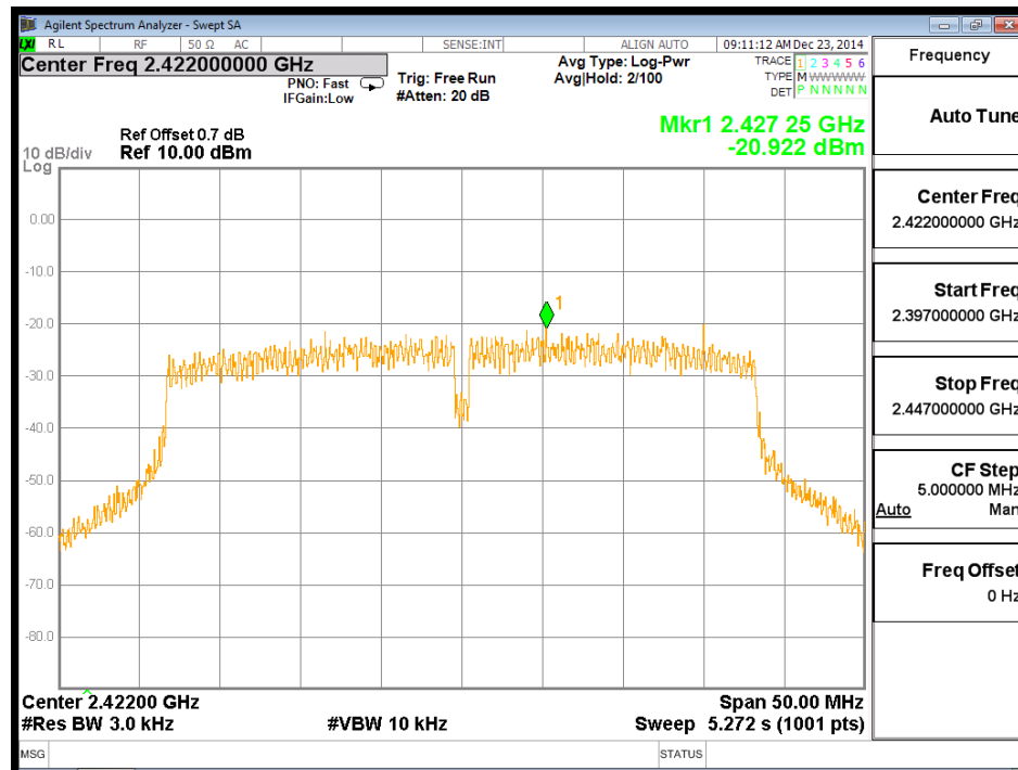
Channel 03 (2422MHz)
