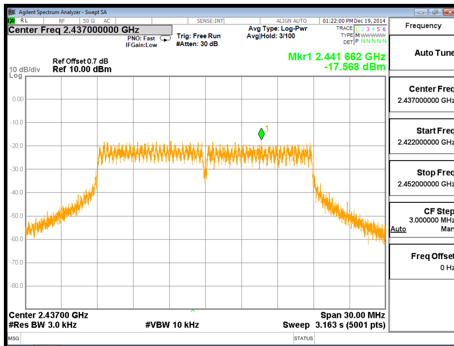
Channel 06 (2437MHz)
