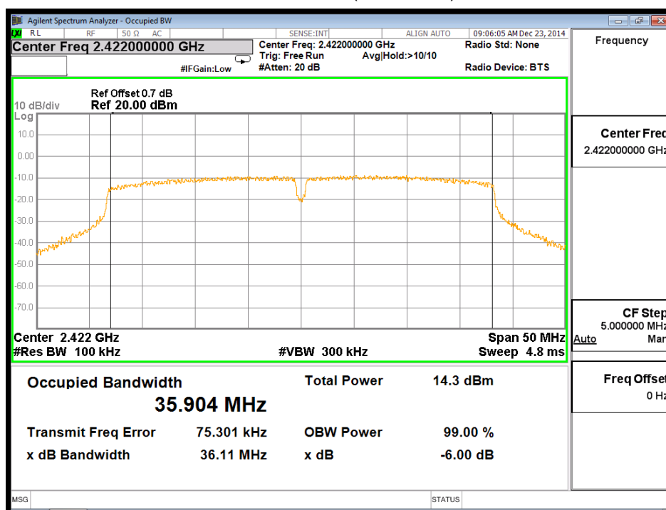
Channel 03 (2422MHz)
