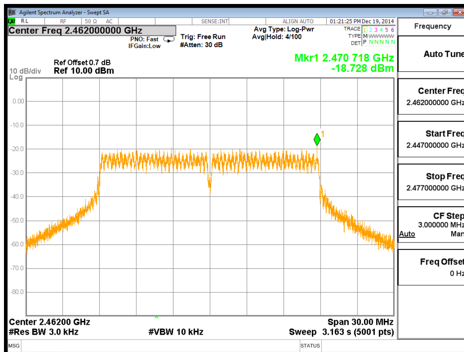
Channel 11 (2462MHz)
