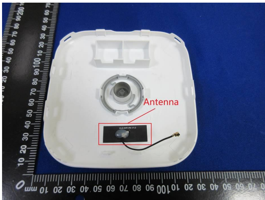
Antenna and RF Model location
