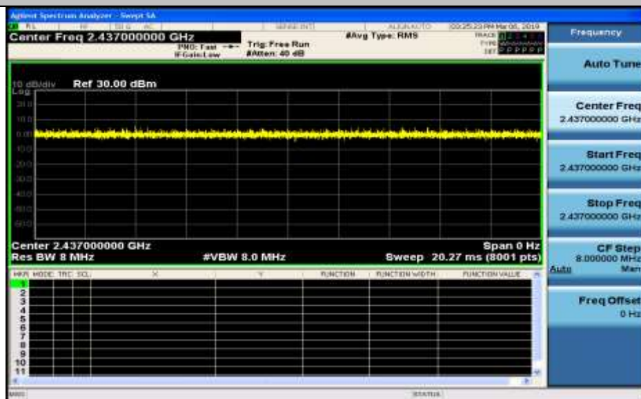
Duty Cycle_11N40SISO_2437_Ant2
