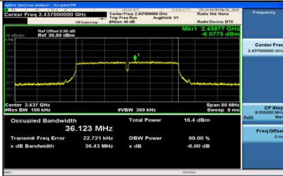
6dB Bandwidth_11N40SISO_2437_Ant2
