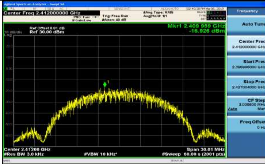
Maximum(average) power spectral density_11B_2412_Ant2
