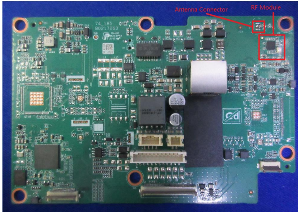
Internal View of EUT-5
