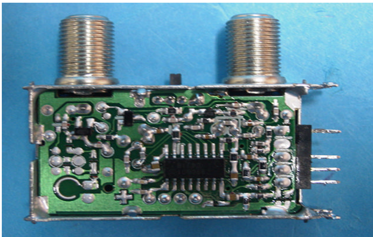
Inner Rear View
