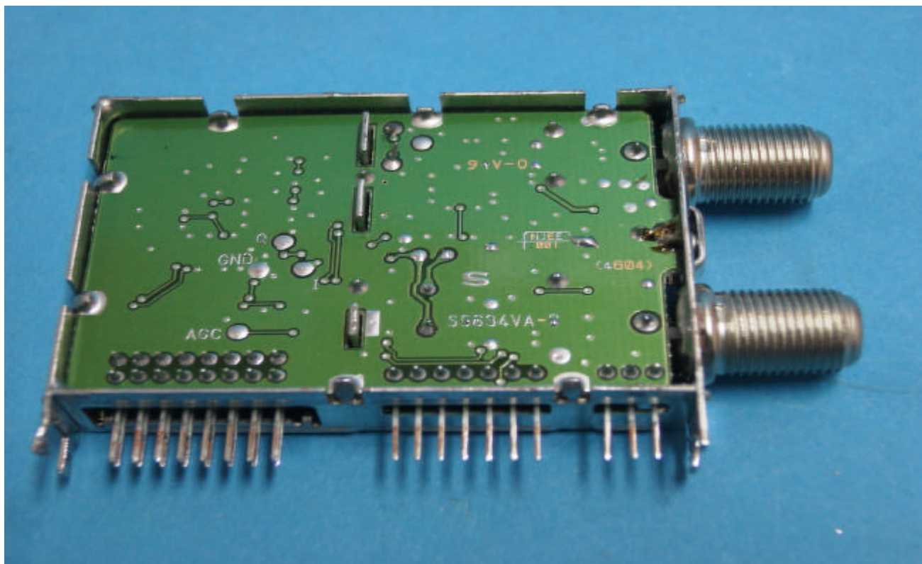
Inner Rear View
