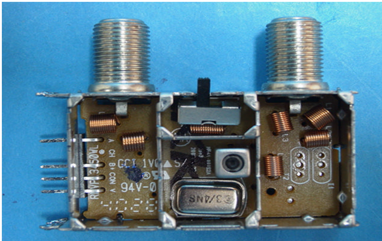
Inner Front View
