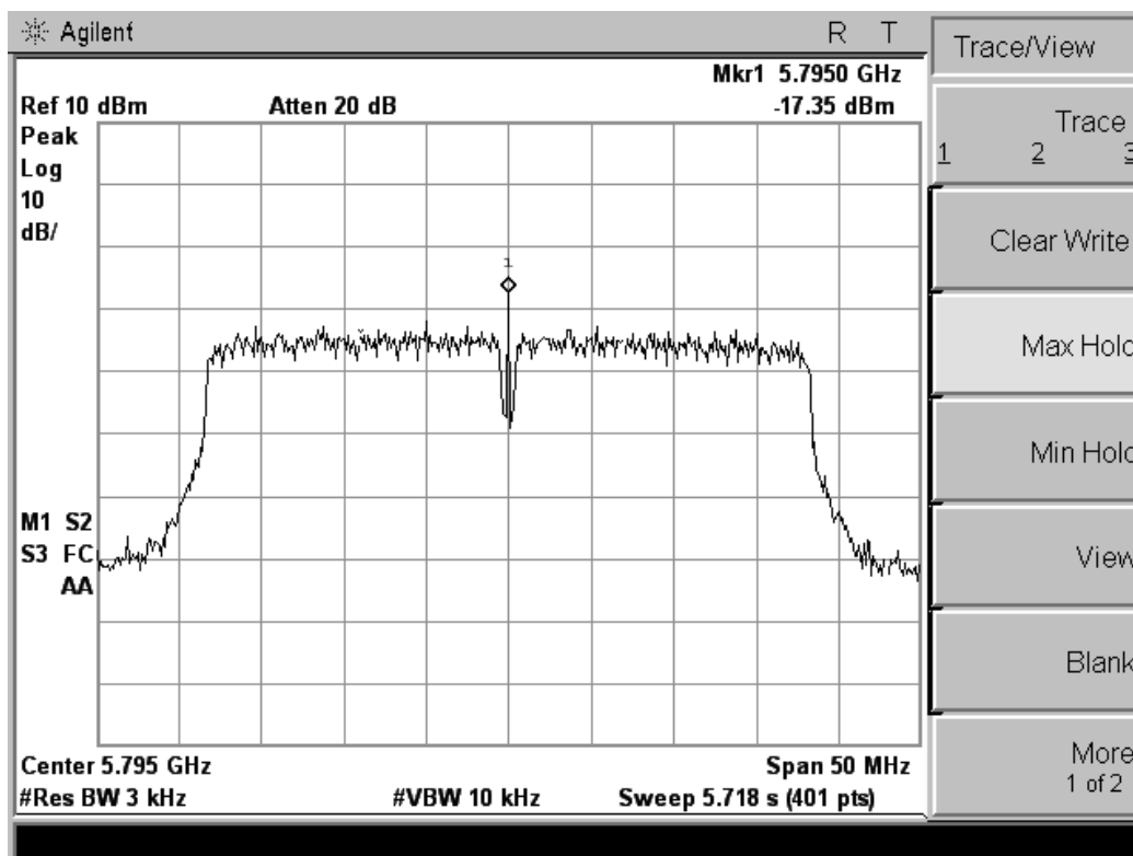
802.11a power density, Port B
