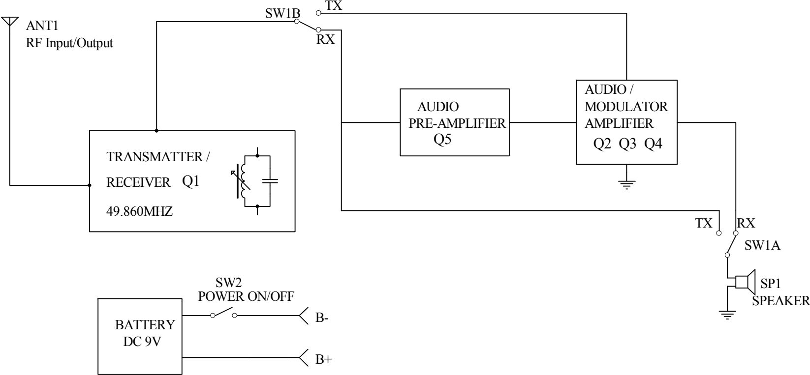
WT-380 block diagram
