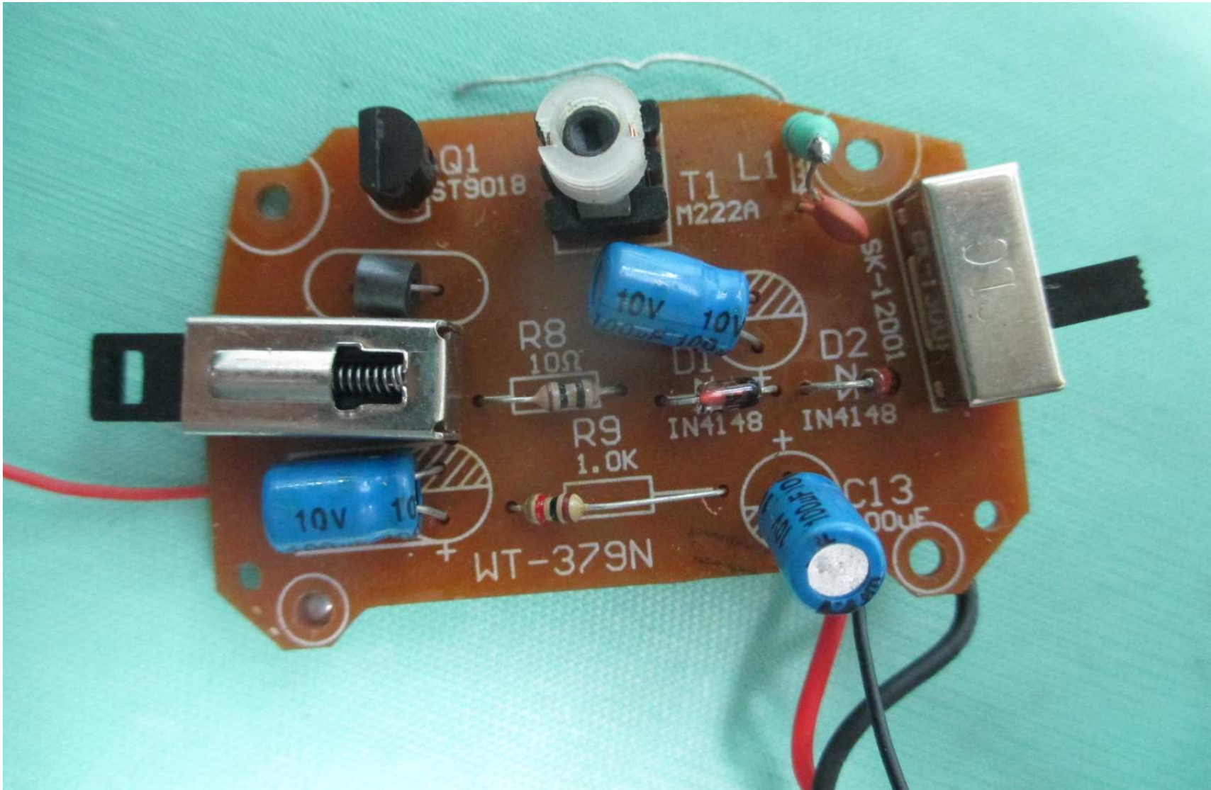
PHOTOGRAPH OF THE PRODUCT INNER CIRCUIT TOP VIEW
