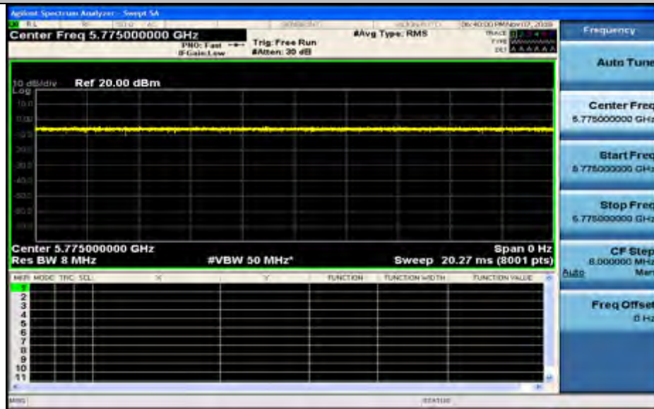
Duty Cycle_11AC80_5775_Ant1
