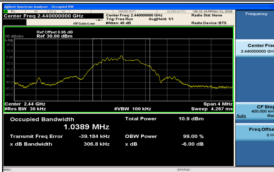
Occupied Bandwidth_BLE_2440
