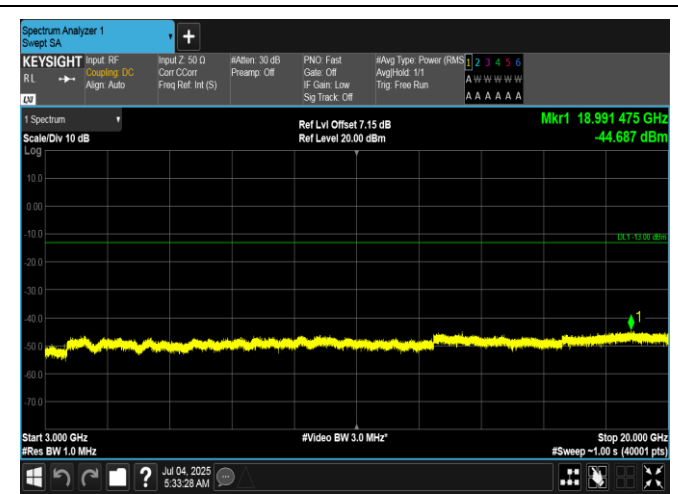
Band66-20MHz-16QAM-132572-1RB#0-3000-20000-PASS
