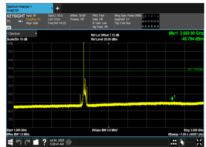
Band66-20MHz-16QAM-132322-1RB#0-1000~3000-PASS
