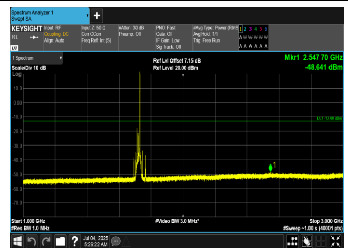
Band66-20MHz-16QAM-132072-1RB#99-1000-3000-PASS
