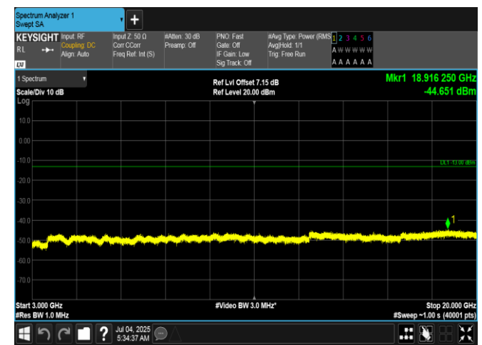
Band66-20MHz-QPSK-132572-1RB#99-3000~20000-PASS
