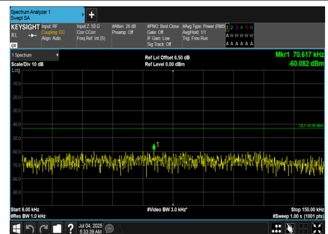
Band66-20MHz-QPSK-132572-1RB#99-0.009~0.15-PASS
