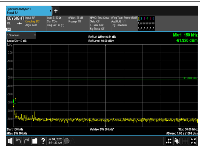
Band66-20MHz-QPSK-132572-1RB#0-0.15~30-PASS
