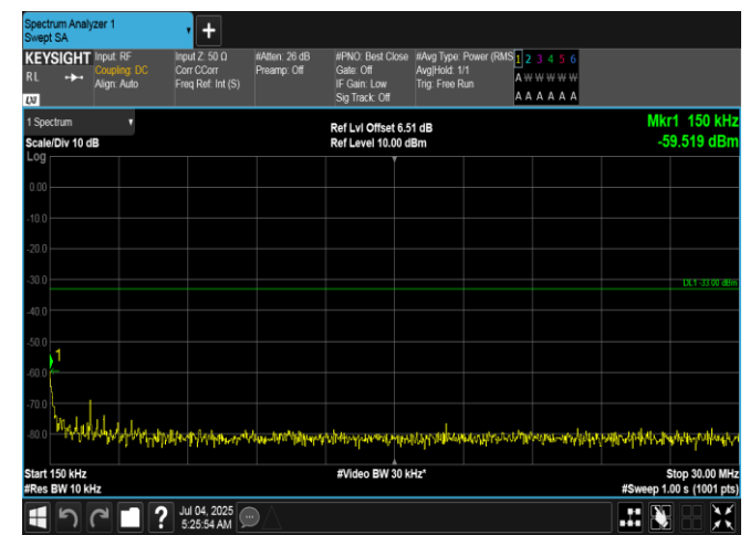
Band66-20MHz-16QAM-132072-1RB#99-0.15-30-PASS
