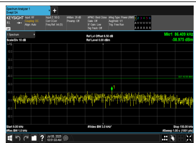
Band66-20MHz-16QAM-132072-100RB#0-0.009~0.15-PASS
