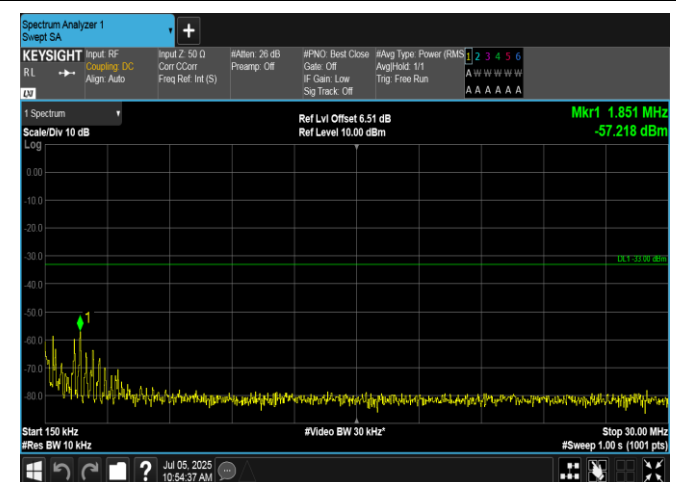
Band66-20MHz-QPSK-132572-100RB#0-0.15~30-PASS
