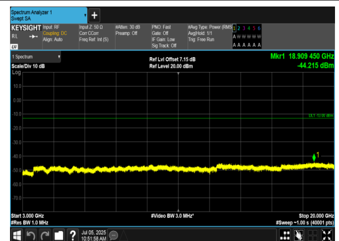
Band66-20MHz-16QAM-132072-100RB#0-3000~20000-PASS
