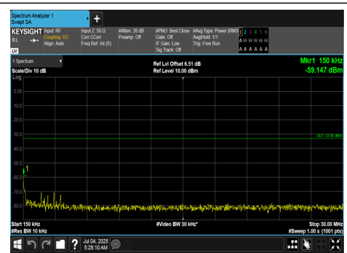
Band66-20MHz-16QAM-132322-1RB#0-0.15~30-PASS
