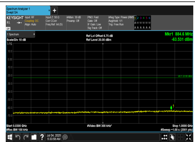
Band66-20MHz-QPSK-132572-1RB#99-30~1000-PASS
