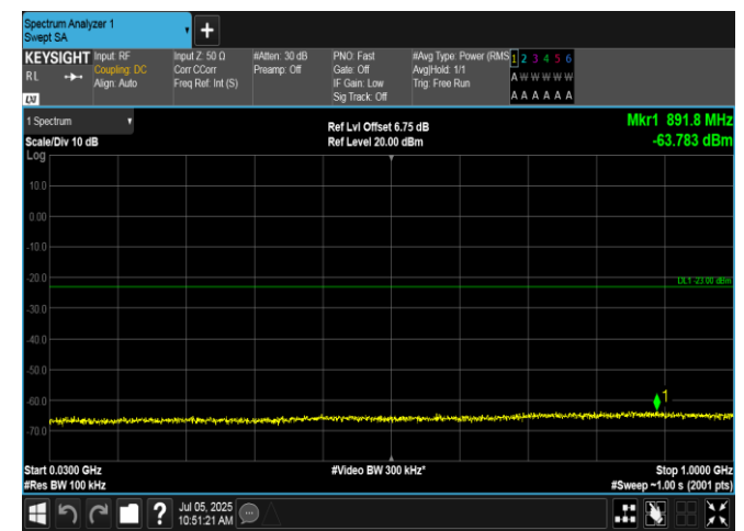
Band66-20MHz-16QAM-132072-100RB#0-30~1000-PASS
