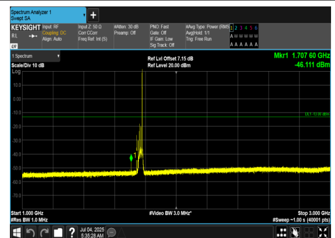
Band66-20MHz-16QAM-132572-1RB#99-1000-3000-PASS
