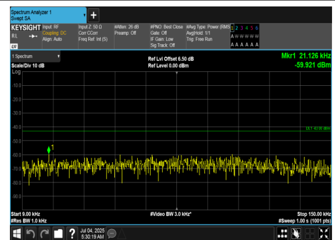
Band66-20MHz-16QAM-132322-1RB#99-0.009~0.15-PASS
