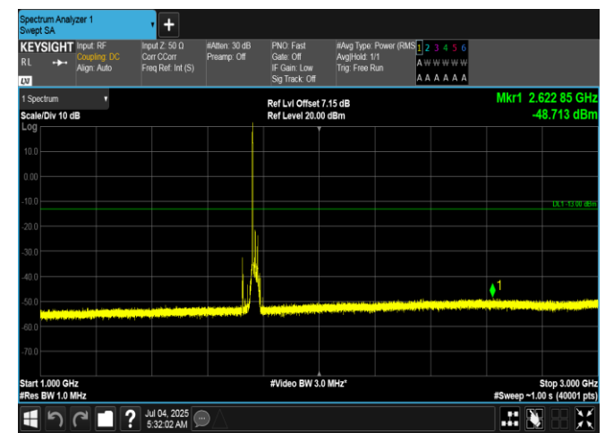
Band66-20MHz-QPSK-132572-1RB#0-1000~3000-PASS
