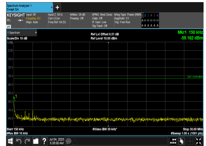
Band66-20MHz-16QAM-132572-1RB#99-0.15-30-PASS
