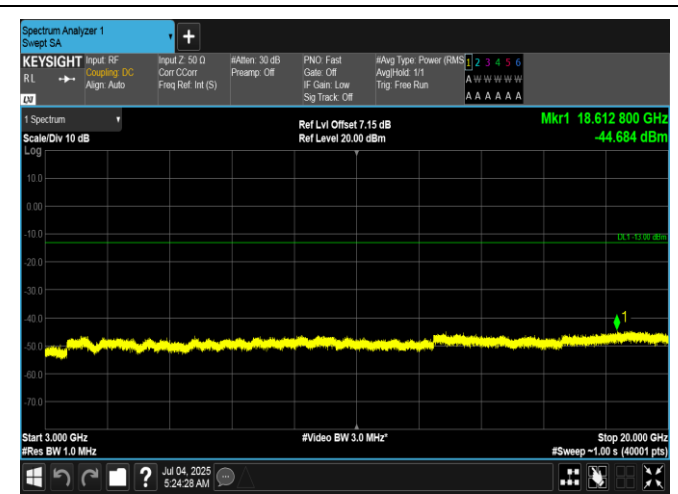
Band66-20MHz-16QAM-132072-1RB#0-3000-20000-PASS
