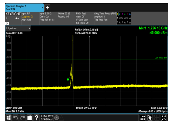
Band66-15MHz-16QAM-132597-1RB#74-1000~3000-PASS
