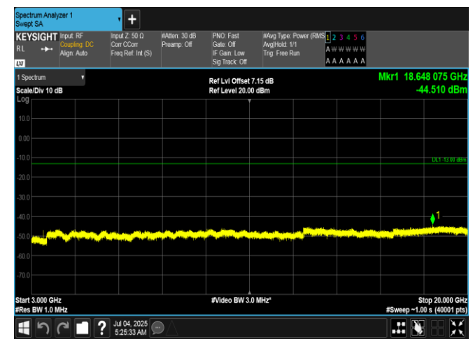
Band66-20MHz-QPSK-132072-1RB#99-3000~20000-PASS
