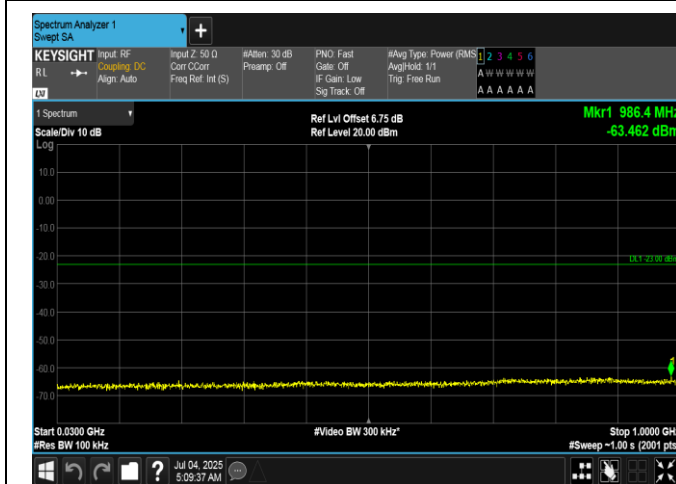
Band66-15MHz-16QAM-132597-1RB#74-30~1000-PASS
