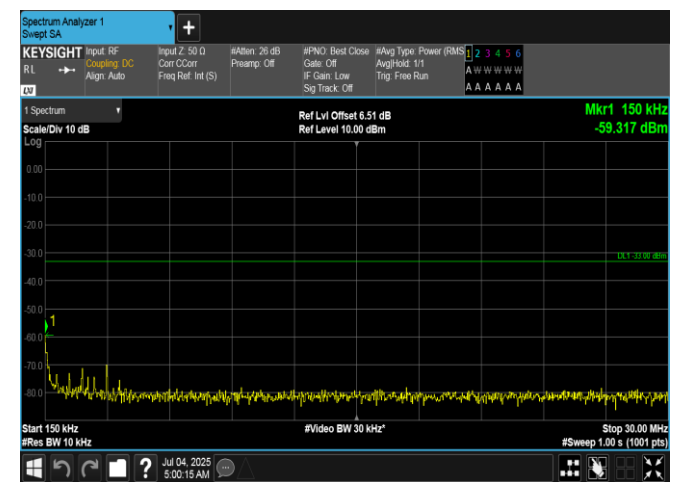
Band66-15MHz-16QAM-132047-1RB#74-0.15~30-PASS
