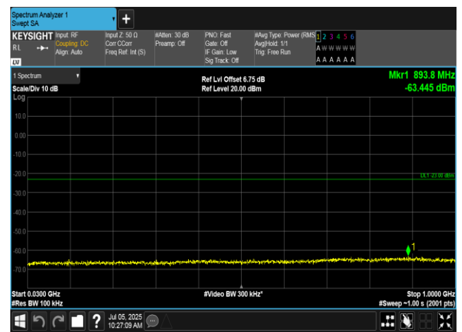
Band66-15MHz-16QAM-132047-75RB#0-30~1000-PASS
