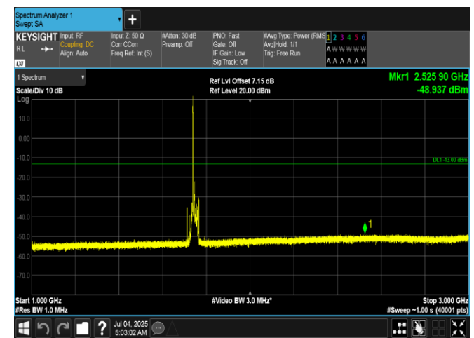
Band66-15MHz-16QAM-132322-1RB#0-1000~3000-PASS
