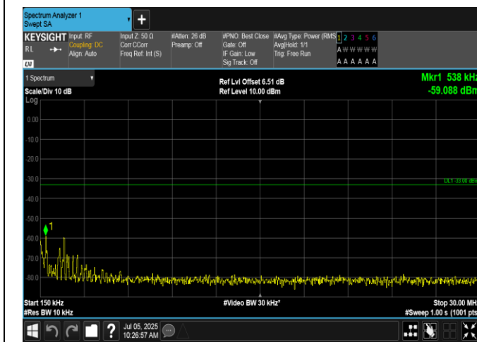
Band66-15MHz-16QAM-132047-75RB#0-0.15~30-PASS
