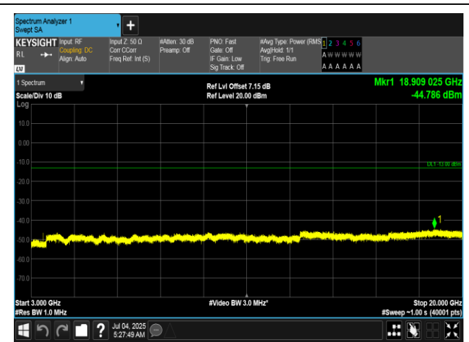
Band66-20MHz-QPSK-132322-1RB#0-3000-20000-PASS
