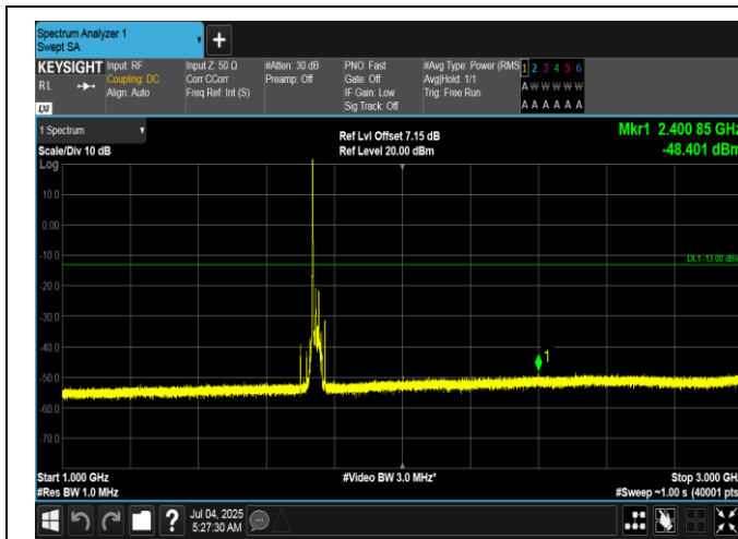
Band66-20MHz-QPSK-132322-1RB#0-1000-3000-PASS
