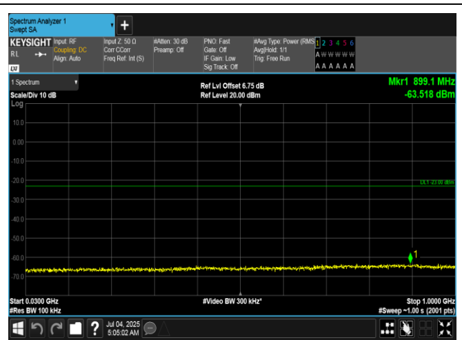
Band66-15MHz-16QAM-132322-1RB#74-30~1000-PASS
