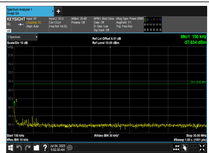
Band66-15MHz-16QAM-132322-1RB#0-0.15~30-PASS
