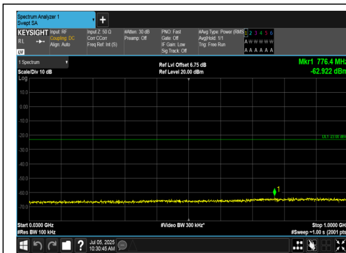
Band66-15MHz-QPSK-132597-75RB#0-30~1000-PASS
