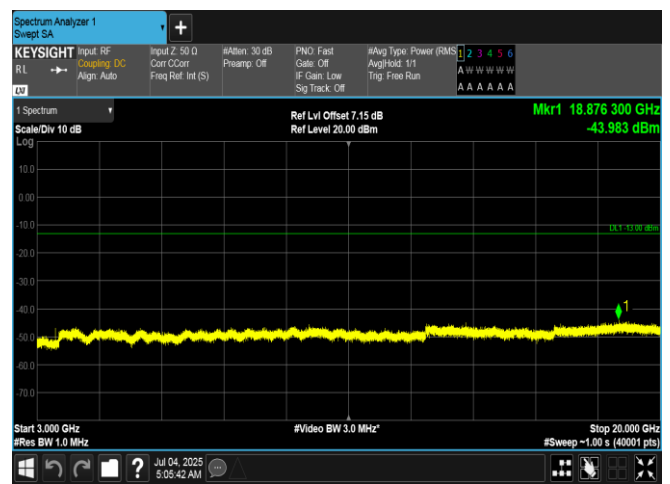
Band66-15MHz-16QAM-132322-1RB#74-3000~20000-PASS
