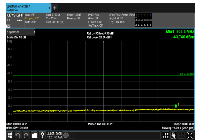
Band66-15MHz-16QAM-132597-75RB#0-30~1000-PASS
