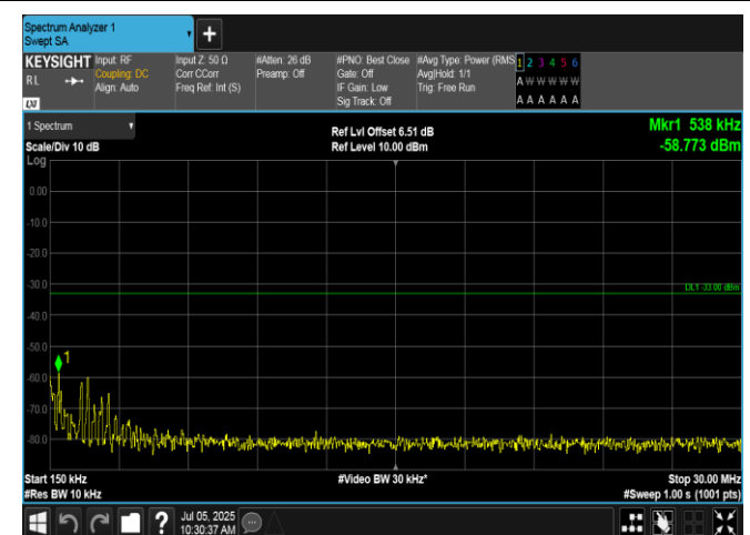
Band66-15MHz-QPSK-132597-75RB#0-0.15~30-PASS
