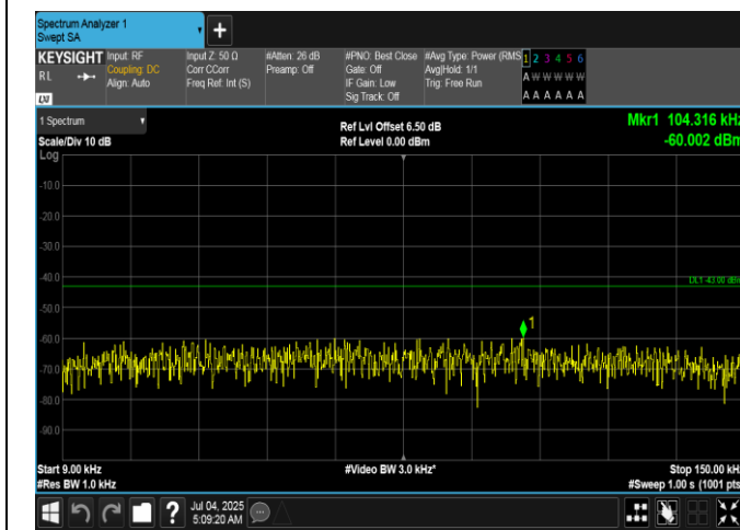
Band66-15MHz-16QAM-132597-1RB#74-0.009~0.15-PASS
