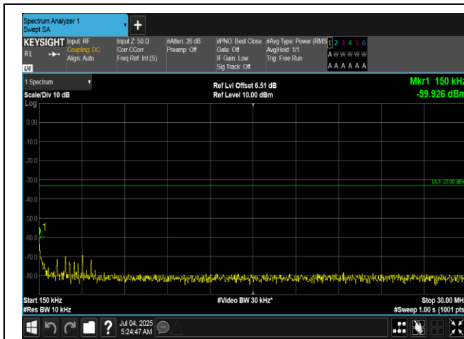
Band66-20MHz-QPSK-132072-1RB#99-0.15~30-PASS
