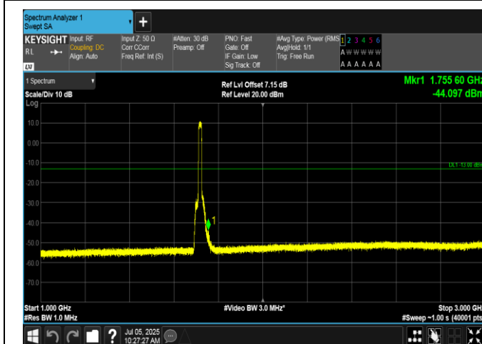
Band66-15MHz-16QAM-132047-75RB#0-1000~3000-PASS
