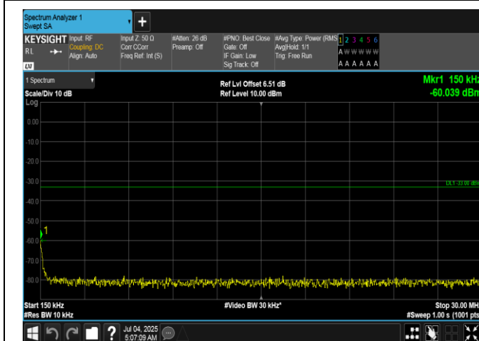
Band66-15MHz-16QAM-132597-1RB#0-0.15~30-PASS
