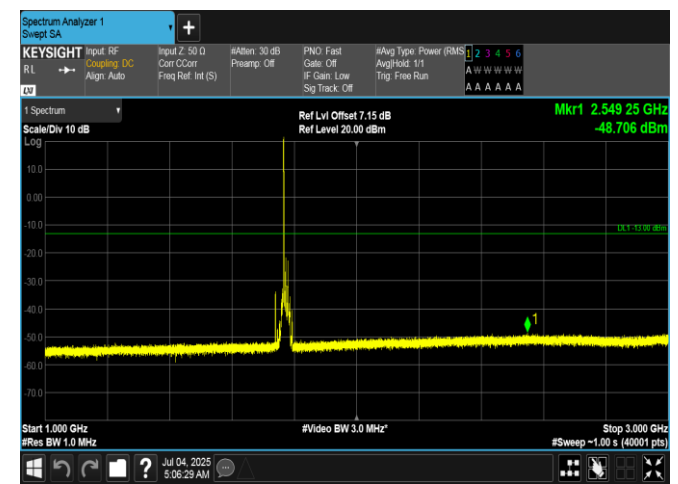
Band66-15MHz-QPSK-132597-1RB#0-1000~3000-PASS
