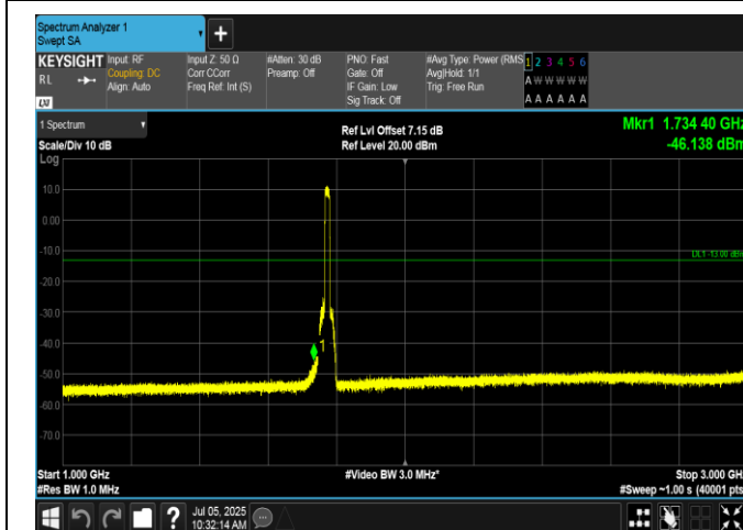
Band66-15MHz-16QAM-132597-75RB#0-1000~3000-PASS
