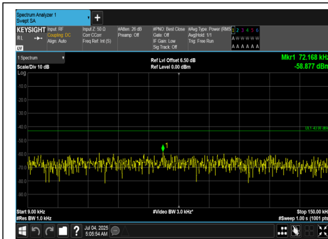
Band66-15MHz-QPSK-132597-1RB#0-0.009~0.15-PASS
