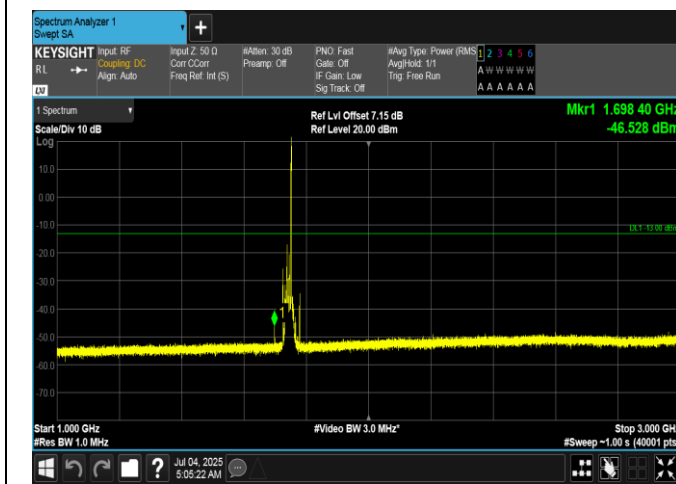
Band66-15MHz-16QAM-132322-1RB#74-1000~3000-PASS
