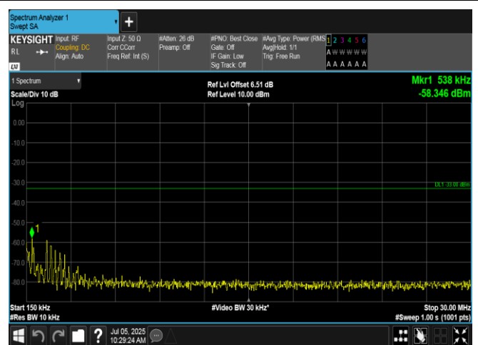
Band66-15MHz-16QAM-132322-75RB#0-0.15~30-PASS
