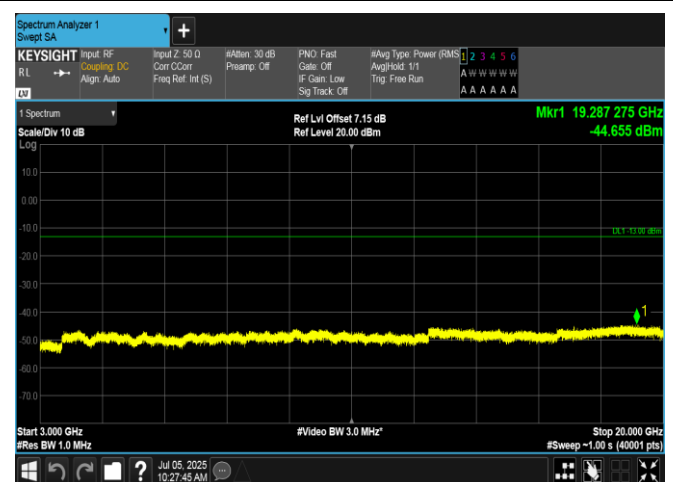
Band66-15MHz-16QAM-132047-75RB#0-3000~20000-PASS
