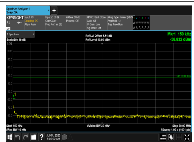
Band66-15MHz-QPSK-132597-1RB#0-0.15~30-PASS
