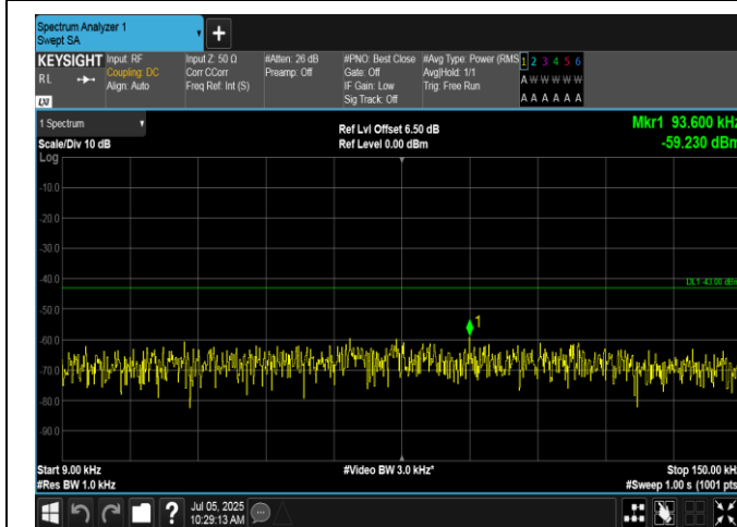
Band66-15MHz-16QAM-132322-75RB#0-0.009~0.15-PASS
