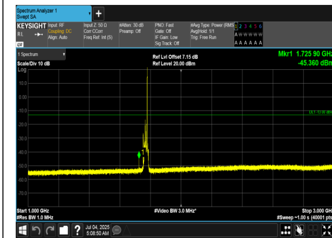
Band66-15MHz-QPSK-132597-1RB#74-1000~3000-PASS
