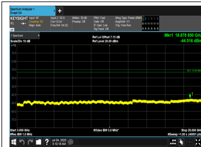
Band66-15MHz-16QAM-132597-1RB#74-3000~20000-PASS
