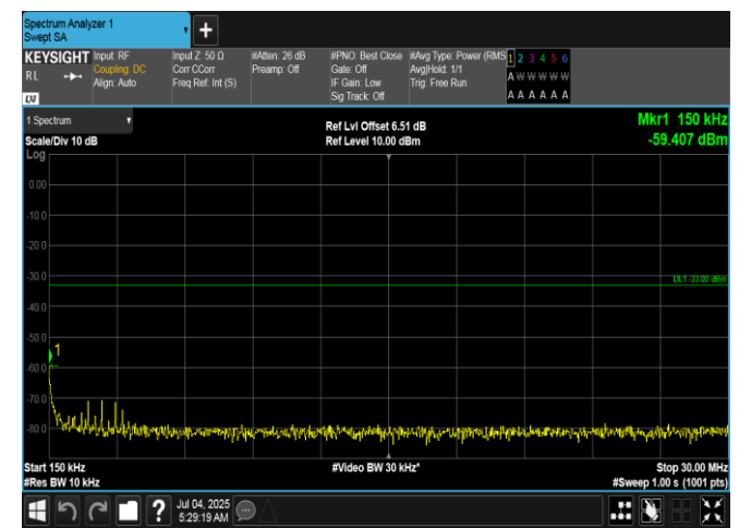
Band66-20MHz-QPSK-132322-1RB#99-0.15-30-PASS
