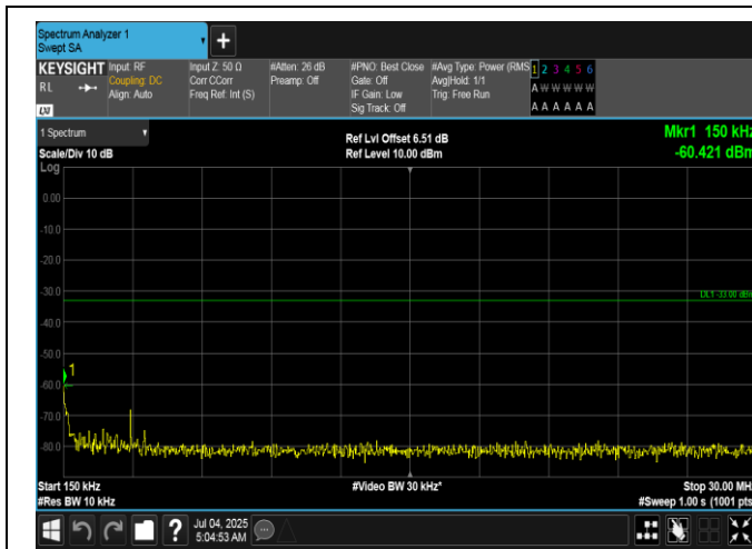
Band66-15MHz-16QAM-132322-1RB#74-0.15~30-PASS
