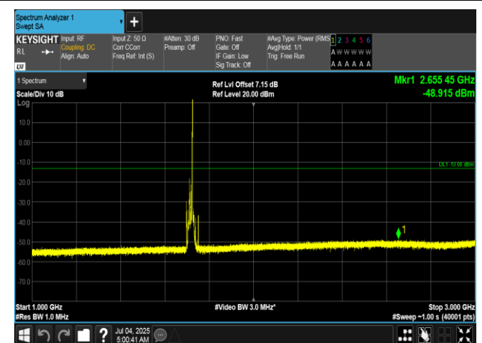
Band66-15MHz-16QAM-132047-1RB#74-1000~3000-PASS
