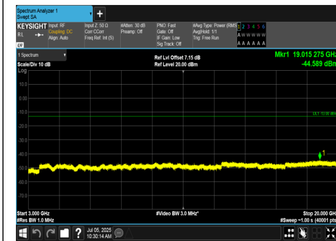
Band66-15MHz-16QAM-132322-75RB#0-3000~20000-PASS
