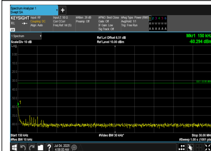
Band66-15MHz-16QAM-132047-1RB#0-0.15~30-PASS
