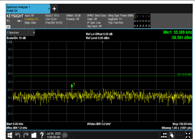
Band66-15MHz-QPSK-132597-1RB#74-0.009~0.15-PASS
