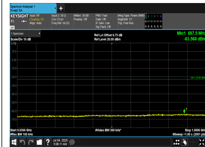
Band66-15MHz-QPSK-132597-1RB#0-30~1000-PASS
