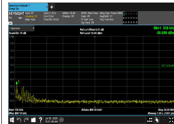
Band66-15MHz-16QAM-132597-75RB#0-0.15~30-PASS
