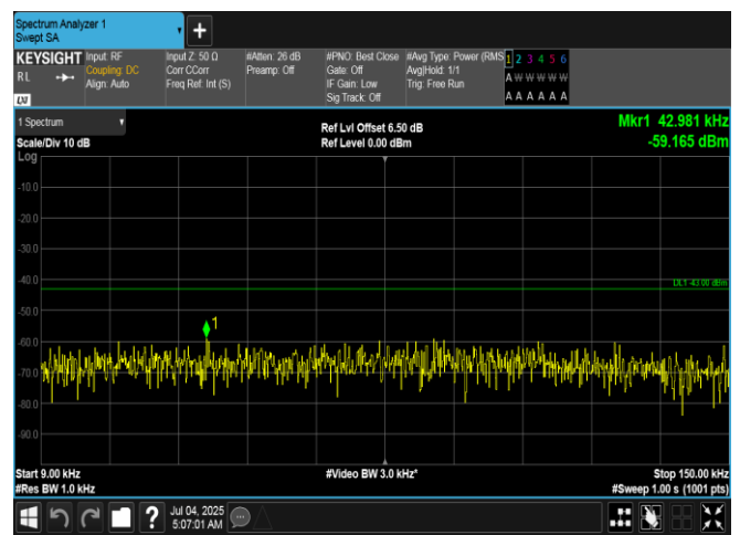
Band66-15MHz-16QAM-132597-1RB#0-0.009~0.15-PASS
