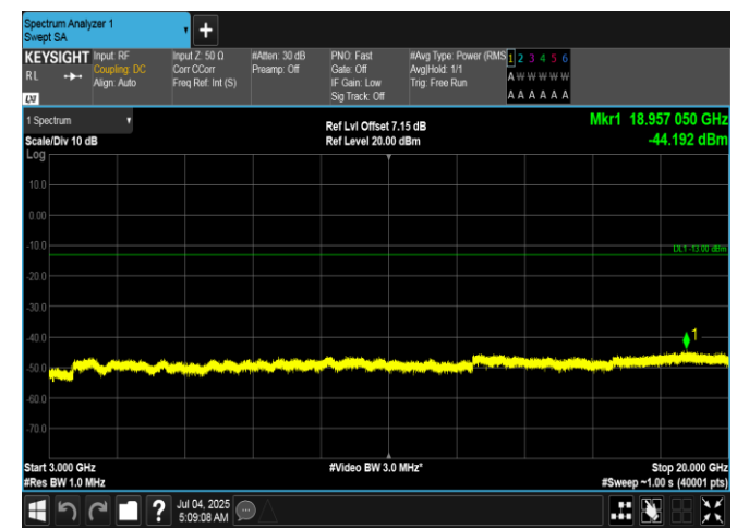
Band66-15MHz-QPSK-132597-1RB#74-3000~20000-PASS
