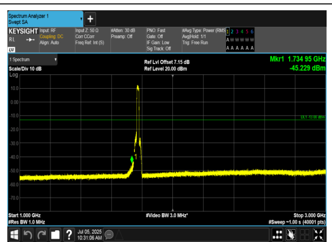
Band66-15MHz-QPSK-132597-75RB#0-1000~3000-PASS
