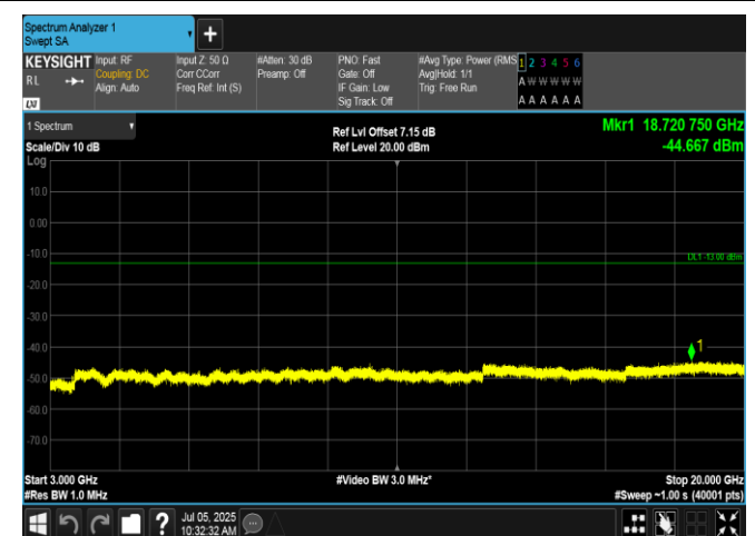
Band66-15MHz-16QAM-132597-75RB#0-3000~20000-PASS
