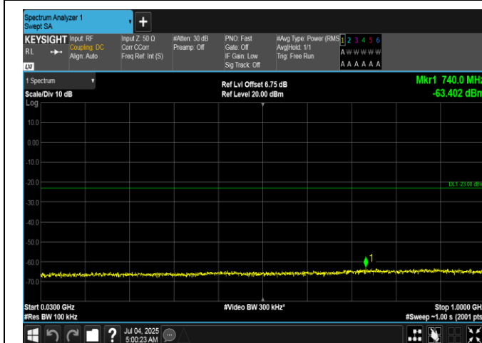
Band66-15MHz-16QAM-132047-1RB#74-30~1000-PASS
