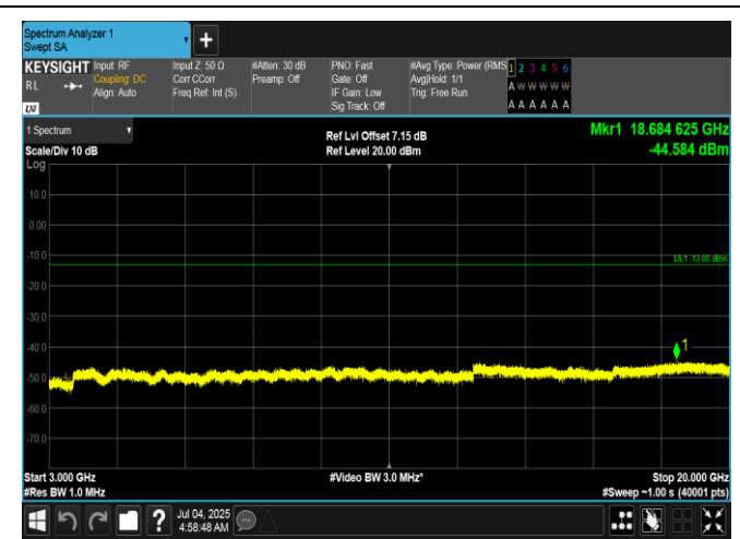
Band66-15MHz-16QAM-132047-1RB#0-3000~20000-PASS
