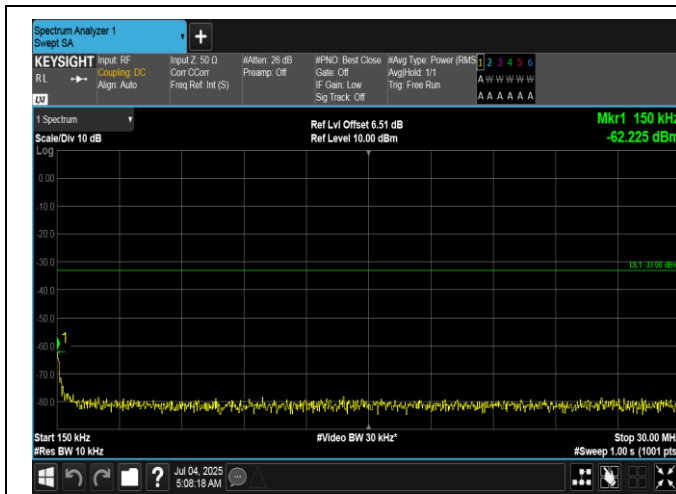
Band66-15MHz-QPSK-132597-1RB#74-0.15~30-PASS
