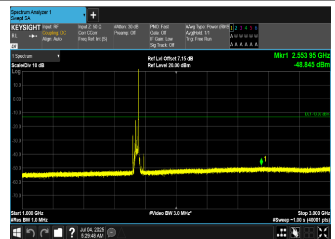
Band66-20MHz-QPSK-132322-1RB#99-1000-3000-PASS
