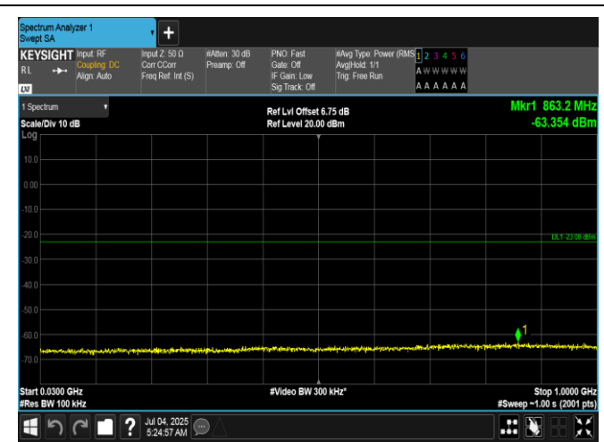
Band66-20MHz-QPSK-132072-1RB#99-30~1000-PASS
