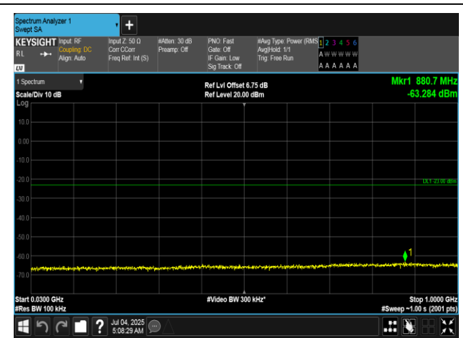
Band66-15MHz-QPSK-132597-1RB#74-30~1000-PASS
