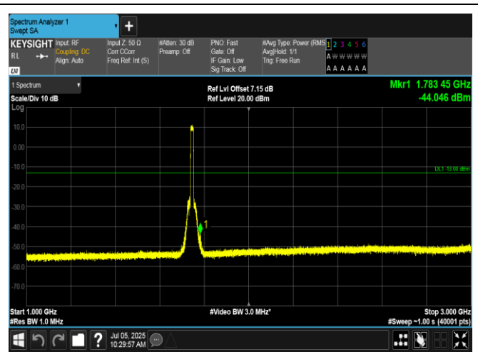
Band66-15MHz-16QAM-132322-75RB#0-1000~3000-PASS
