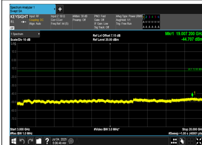
Band66-15MHz-QPSK-132597-1RB#0-3000~20000-PASS
