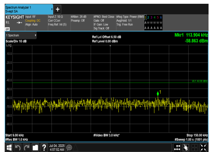
Band66-15MHz-16QAM-132047-1RB#0-0.009~0.15-PASS
