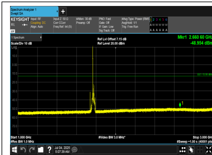
Band66-15MHz-16QAM-132597-1RB#0-1000~3000-PASS
