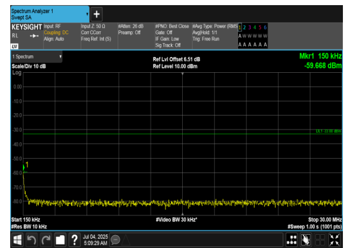
Band66-15MHz-16QAM-132597-1RB#74-0.15~30-PASS
