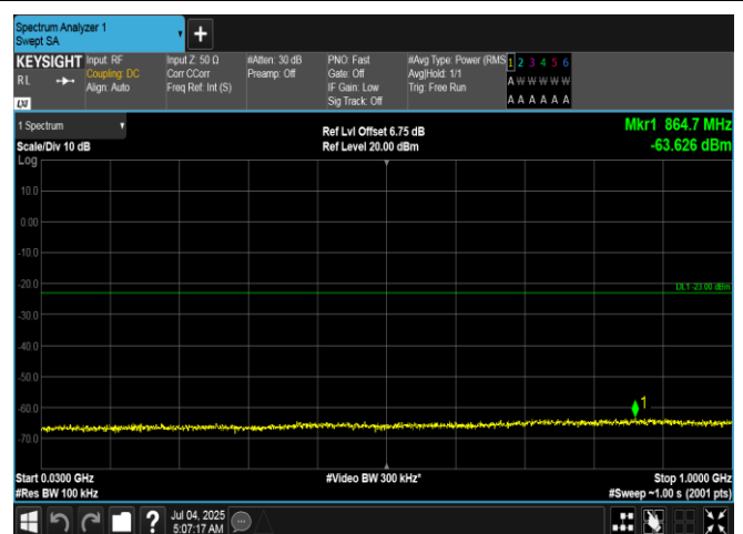
Band66-15MHz-16QAM-132597-1RB#0-30~1000-PASS
