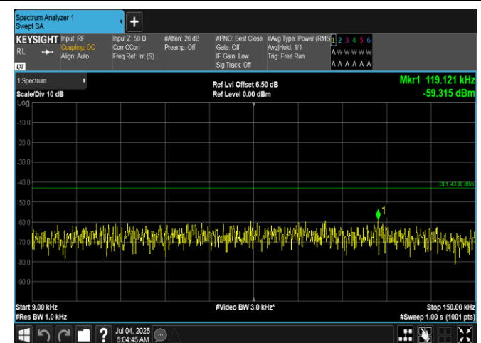
Band66-15MHz-16QAM-132322-1RB#74-0.009~0.15-PASS
