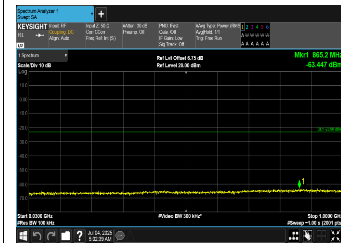
Band66-15MHz-16QAM-132322-1RB#0-30~1000-PASS
