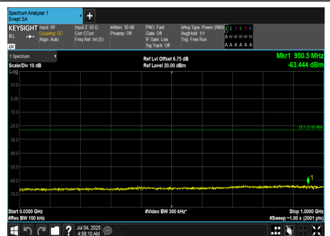
Band66-15MHz-16QAM-132047-1RB#0-30~1000-PASS
