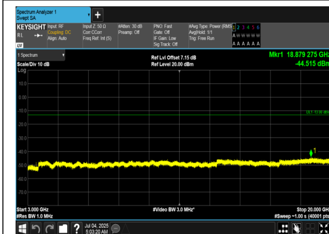
Band66-15MHz-16QAM-132322-1RB#0-3000~20000-PASS
