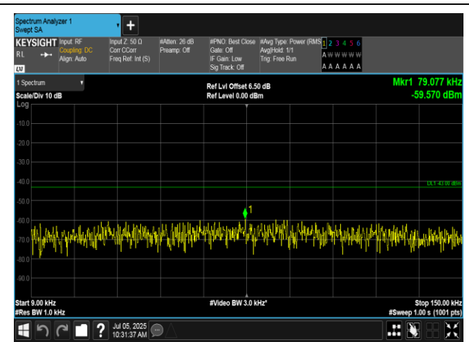
Band66-15MHz-16QAM-132597-75RB#0-0.009~0.15-PASS
