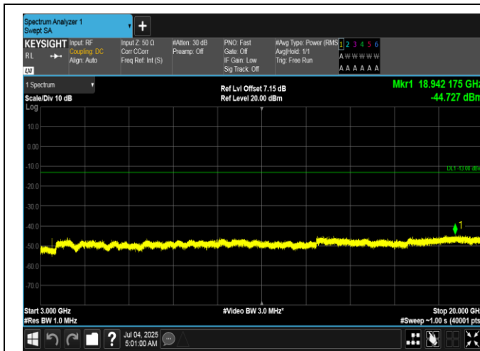
Band66-15MHz-16QAM-132047-1RB#74-3000~20000-PASS
