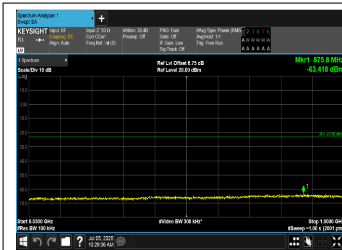
Band66-15MHz-16QAM-132322-75RB#0-30~1000-PASS
