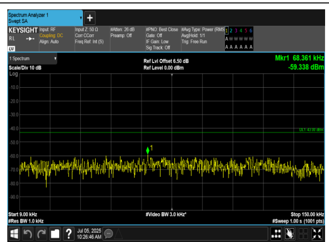
Band66-15MHz-16QAM-132047-75RB#0-0.009~0.15-PASS
