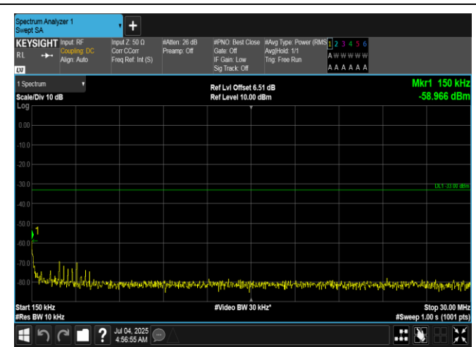
Band66-15MHz-QPSK-132047-1RB#0-0.15~30-PASS
