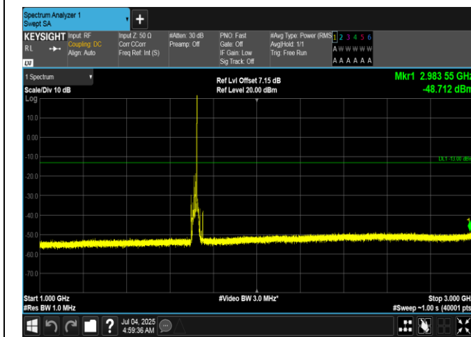
Band66-15MHz-QPSK-132047-1RB#74-1000~3000-PASS
