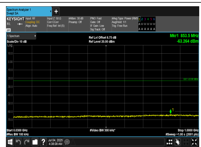
Band66-10MHz-QPSK-132622-1RB#49-30~1000-PASS
