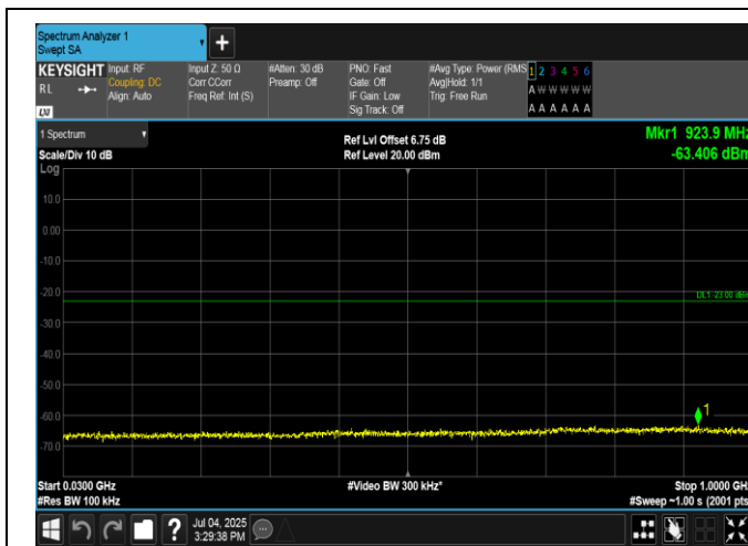
Band66-10MHz-QPSK-132622-50RB#0-30~1000-PASS
