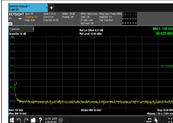
Band66-10MHz-16QAM-132622-1RB#0-0.15~30-PASS
