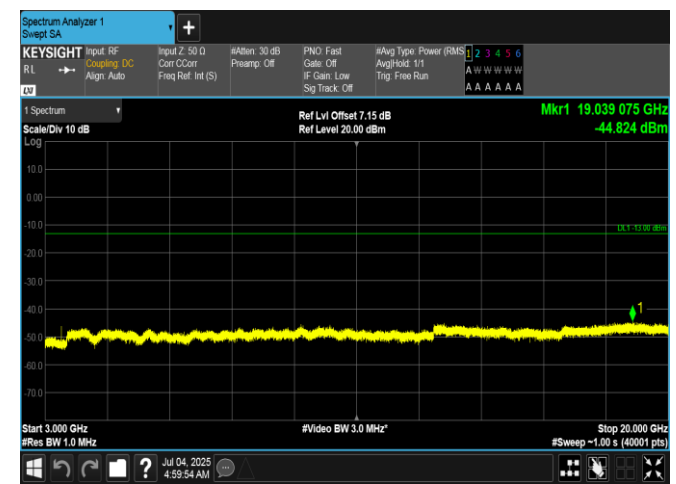
Band66-15MHz-QPSK-132047-1RB#74-3000~20000-PASS
