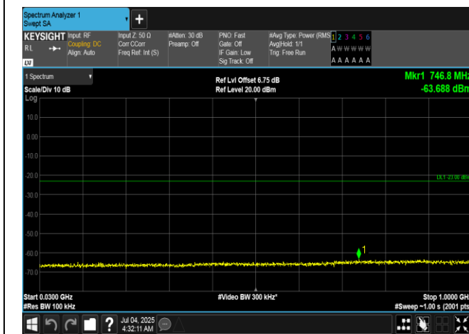
Band66-10MHz-16QAM-132322-1RB#0-30~1000-PASS
