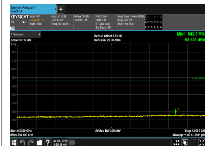
Band66-10MHz-16QAM-132622-1RB#49-30~1000-PASS
