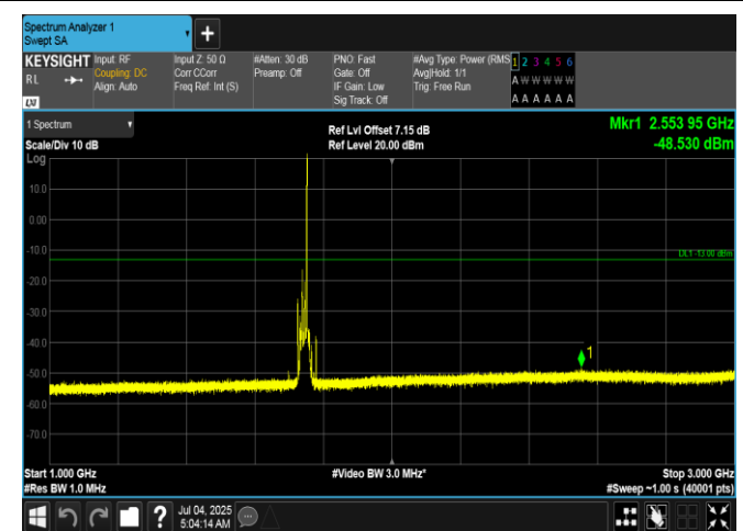
Band66-15MHz-QPSK-132322-1RB#74-1000~3000-PASS
