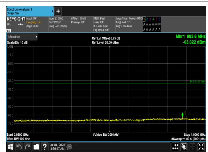
Band66-15MHz-QPSK-132047-1RB#74-30~1000-PASS
