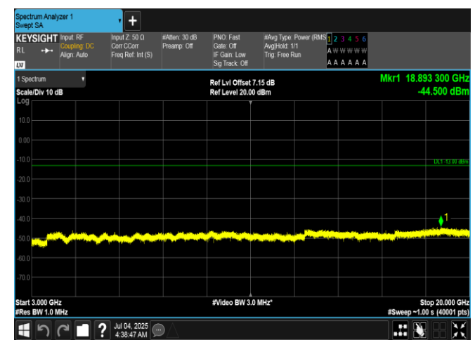
Band66-10MHz-QPSK-132622-1RB#49-3000~20000-PASS
