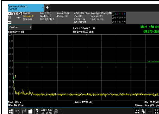
Band66-10MHz-16QAM-132022-1RB#0-0.15~30-PASS
