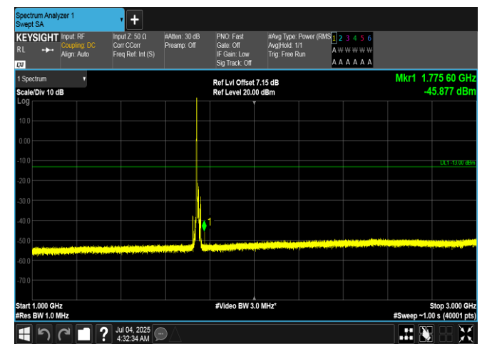
Band66-10MHz-16QAM-132322-1RB#0-1000~3000-PASS
