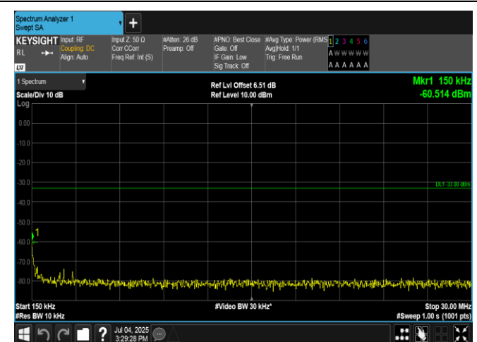
Band66-10MHz-QPSK-132622-50RB#0-0.15~30-PASS
