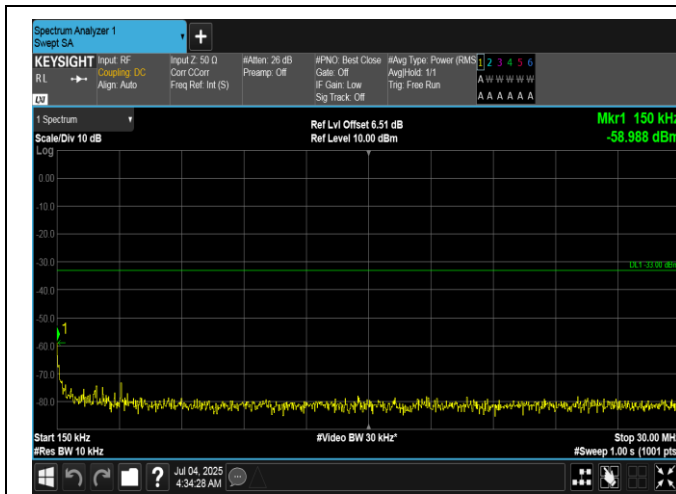
Band66-10MHz-16QAM-132322-1RB#49-0.15~30-PASS
