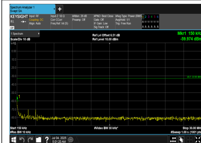
Band66-15MHz-QPSK-132322-1RB#0-0.15~30-PASS
