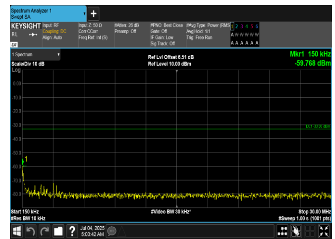
Band66-15MHz-QPSK-132322-1RB#74-0.15~30-PASS
