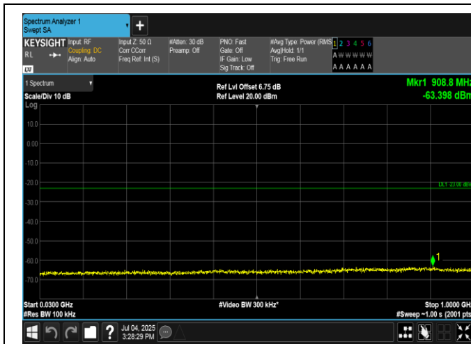
Band66-10MHz-16QAM-132322-50RB#0-30~1000-PASS
