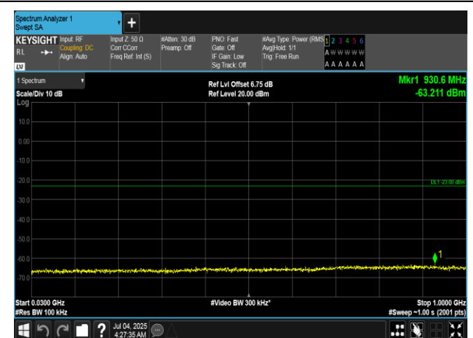
Band66-10MHz-16QAM-132022-1RB#0-30~1000-PASS
