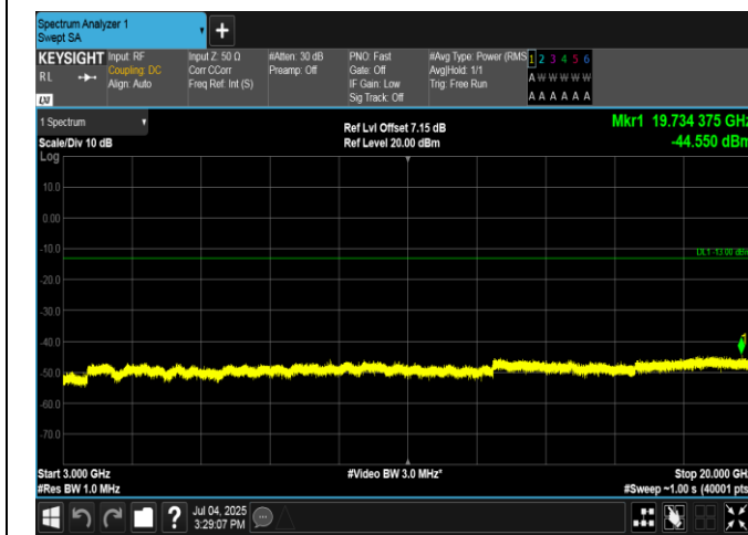
Band66-10MHz-16QAM-132322-50RB#0-3000~20000-PASS
