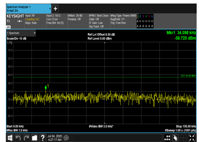
Band66-10MHz-16QAM-132022-1RB#0-0.009~0.15-PASS
