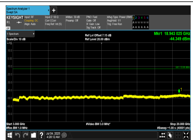
Band66-10MHz-16QAM-132022-1RB#0-3000~20000-PASS
