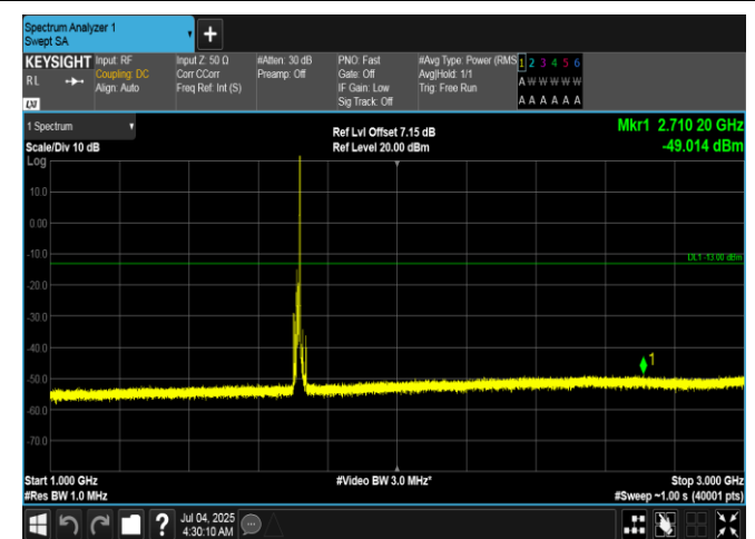
Band66-10MHz-16QAM-132022-1RB#49-1000~3000-PASS
