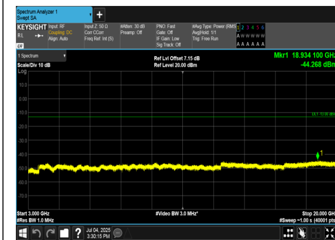
Band66-10MHz-QPSK-132622-50RB#0-3000~20000-PASS
