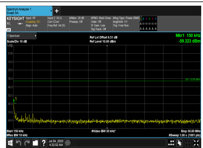
Band66-10MHz-16QAM-132322-1RB#0-0.15~30-PASS
