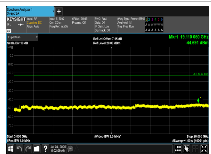
Band66-15MHz-QPSK-132322-1RB#0-3000~20000-PASS
