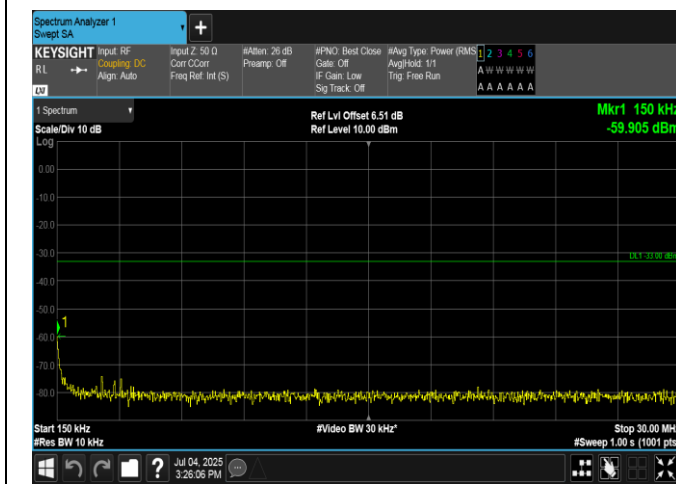
Band66-10MHz-16QAM-132022-50RB#0-0.15~30-PASS
