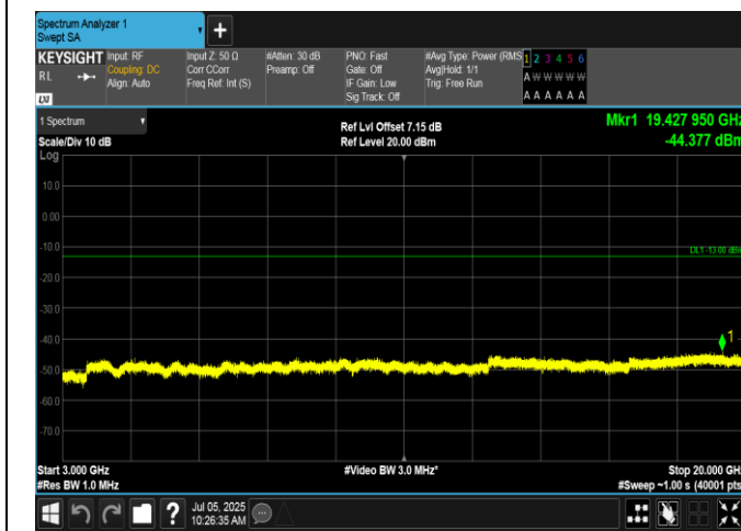
Band66-15MHz-QPSK-132047-75RB#0-3000~20000-PASS
