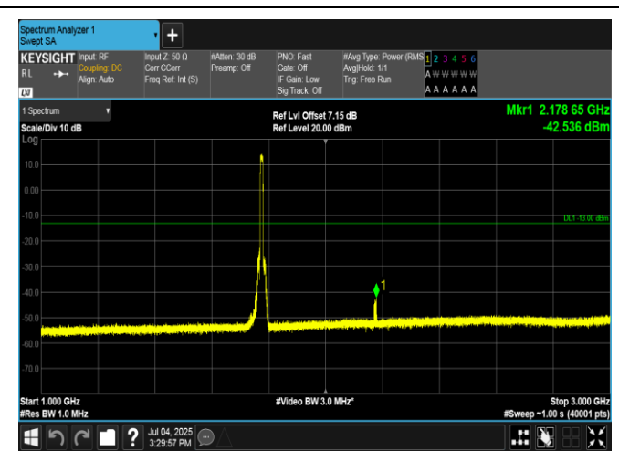
Band66-10MHz-QPSK-132622-50RB#0-1000~3000-PASS
