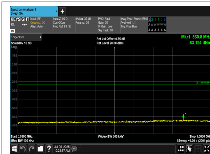
Band66-15MHz-QPSK-132047-75RB#0-30~1000-PASS
