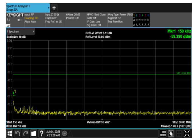
Band66-10MHz-16QAM-132022-1RB#49-0.15~30-PASS
