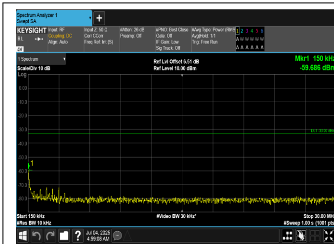
Band66-15MHz-QPSK-132047-1RB#74-0.15~30-PASS
