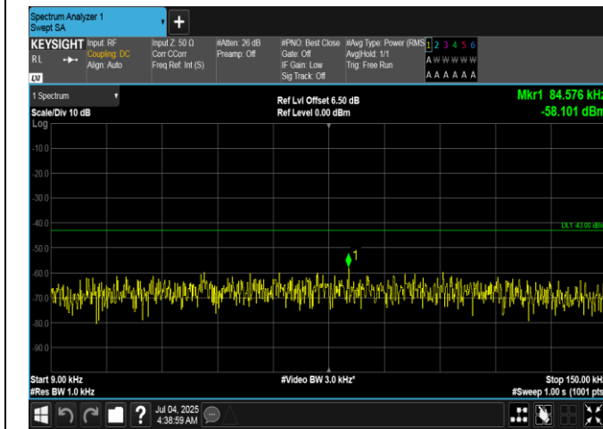
Band66-10MHz-16QAM-132622-1RB#49-0.009~0.15-PASS
