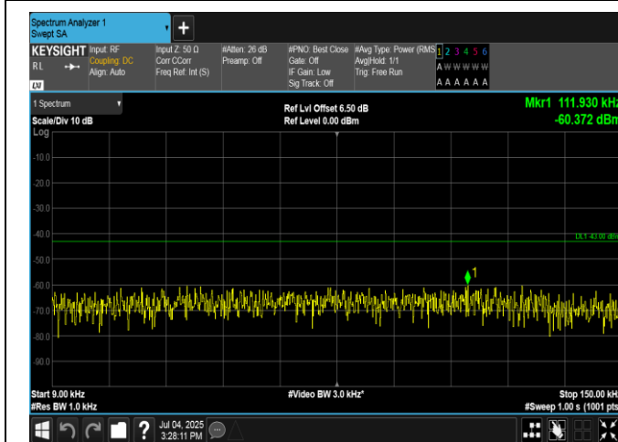
Band66-10MHz-16QAM-132322-50RB#0-0.009~0.15-PASS
