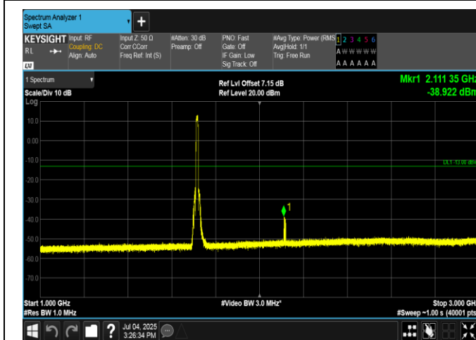
Band66-10MHz-16QAM-132022-50RB#0-1000~3000-PASS
