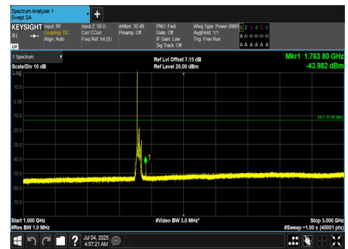
Band66-15MHz-QPSK-132047-1RB#0-1000~3000-PASS
