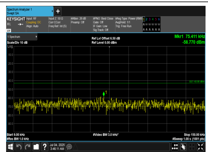
Band66-5MHz-16QAM-131997-25RB#0-0.009~0.15-PASS
