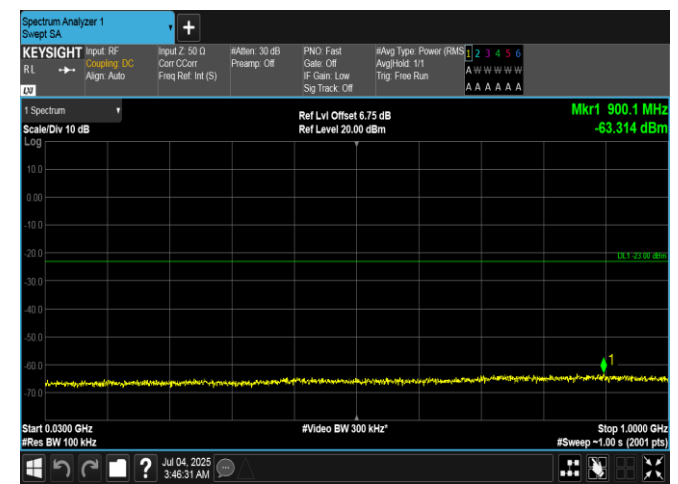
Band66-5MHz-16QAM-131997-25RB#0-30~1000-PASS
