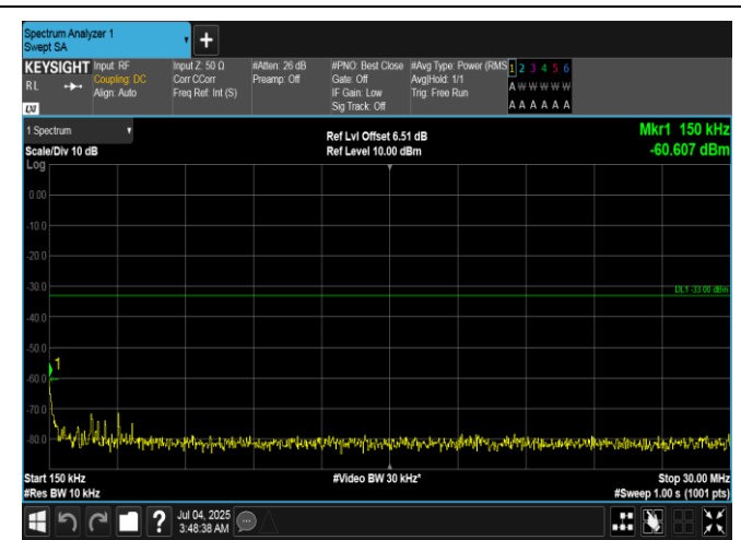
Band66-5MHz-16QAM-132322-1RB#0-0.15~30-PASS
