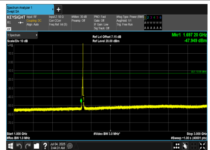
Band66-5MHz-16QAM-131997-1RB#24-1000~3000-PASS
