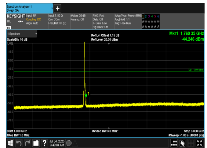
Band66-5MHz-16QAM-132322-1RB#0-1000~3000-PASS
