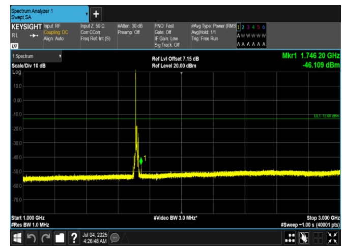
Band66-10MHz-QPSK-132022-1RB#0-1000~3000-PASS
