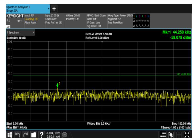
Band66-5MHz-16QAM-132322-1RB#24-0.009~0.15-PASS
