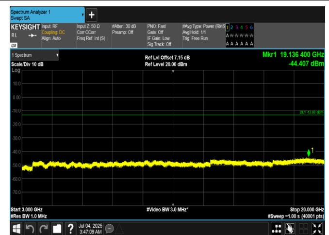
Band66-5MHz-16QAM-131997-25RB#0-3000~20000-PASS
