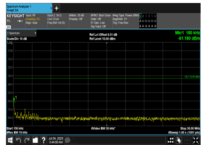
Band66-5MHz-16QAM-131997-1RB#24-0.15~30-PASS
