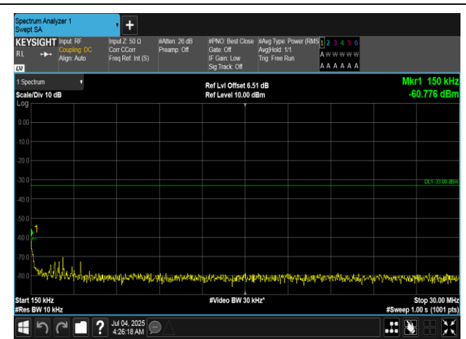
Band66-10MHz-QPSK-132022-1RB#0-0.15~30-PASS
