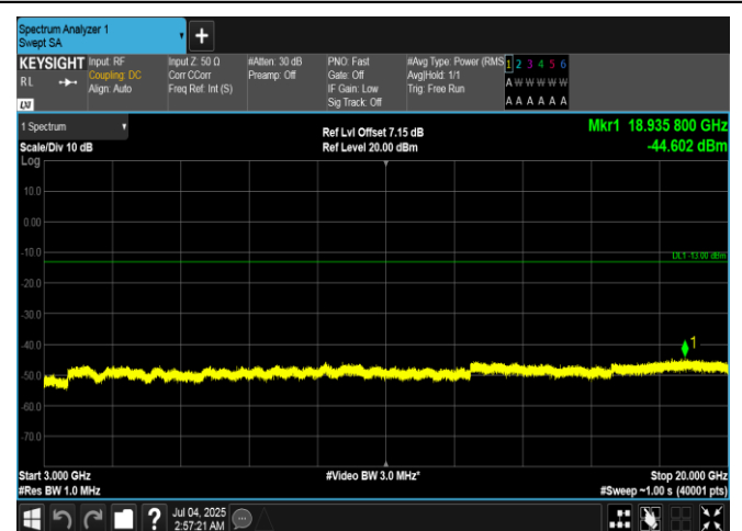
Band66-3MHz-16QAM-131987-15RB#0-3000~20000-PASS
