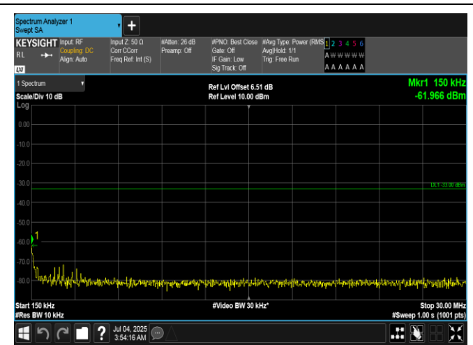
Band66-5MHz-QPSK-132647-1RB#0-0.15-30-PASS
