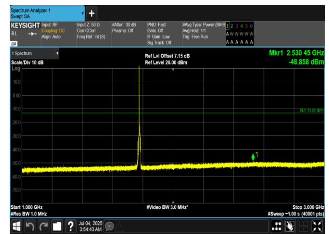
Band66-5MHz-QPSK-132647-1RB#0-1000-3000-PASS
