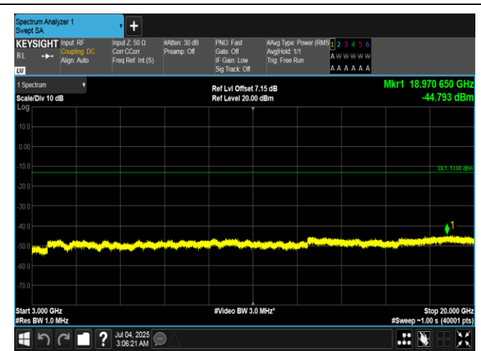
Band66-3MHz-16QAM-132657-1RB#0-3000-20000-PASS
