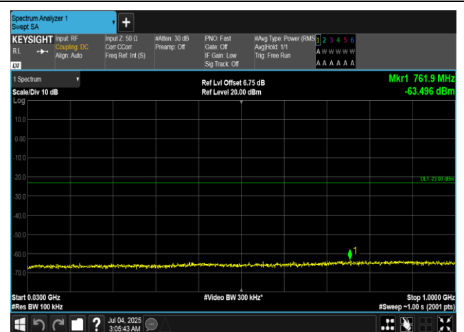
Band66-3MHz-16QAM-132657-1RB#0-30~1000-PASS
