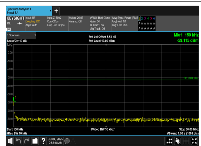
Band66-3MHz-16QAM-132322-1RB#0-0.15~30-PASS
