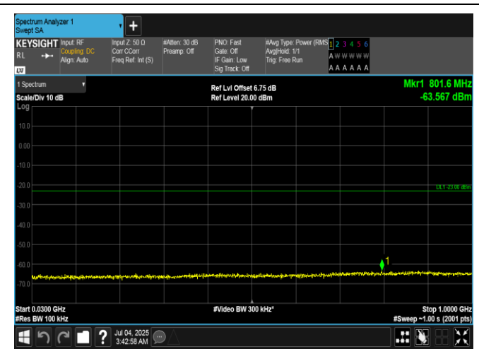
Band66-5MHz-QPSK-131997-1RB#24-30~1000-PASS
