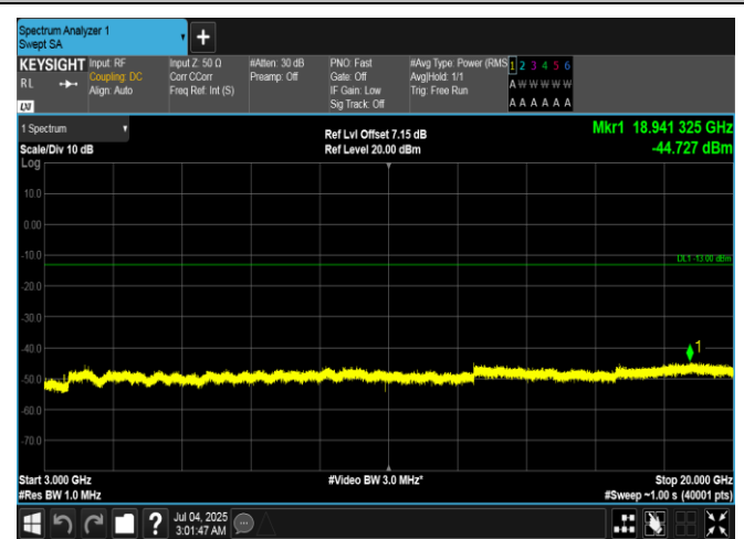
Band66-3MHz-16QAM-132322-1RB#14-3000~20000-PASS
