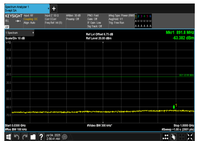
Band66-3MHz-16QAM-131987-15RB#0-30~1000-PASS
