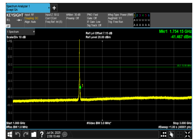
Band66-3MHz-16QAM-132322-1RB#0-1000~3000-PASS
