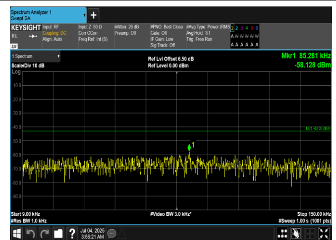
Band66-5MHz-QPSK-132647-1RB#24-0.009-0.15-PASS
