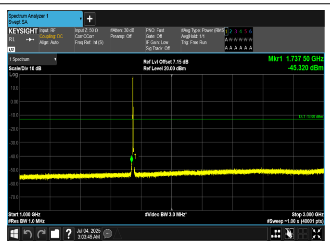
Band66-3MHz-16QAM-132322-15RB#0-1000~3000-PASS
