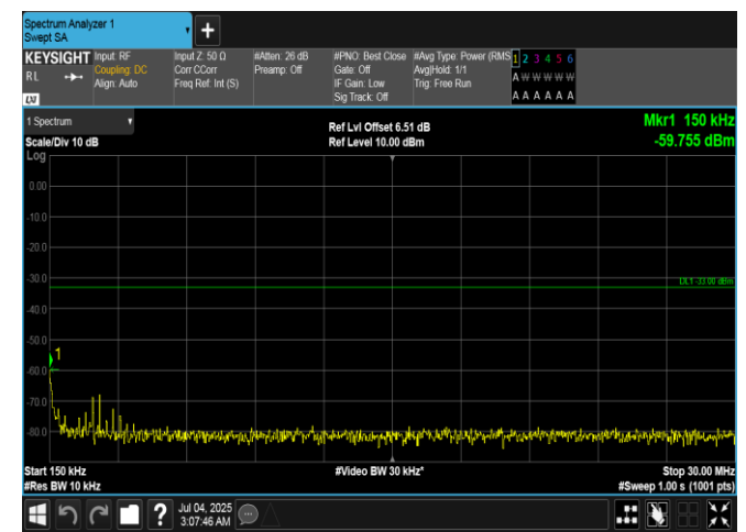
Band66-3MHz-16QAM-132657-1RB#14-0.15-30-PASS
