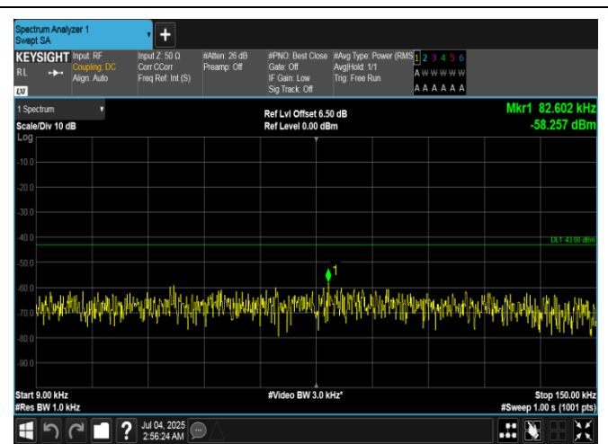
Band66-3MHz-16QAM-131987-15RB#0-0.009~0.15-PASS
