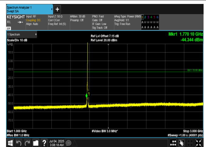
Band66-3MHz-16QAM-132657-1RB#14-1000-3000-PASS
