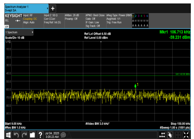
Band66-3MHz-16QAM-132657-1RB#0-0.009~0.15-PASS
