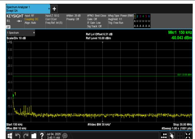
Band66-5MHz-QPSK-131997-25RB#0-0.15~30-PASS
