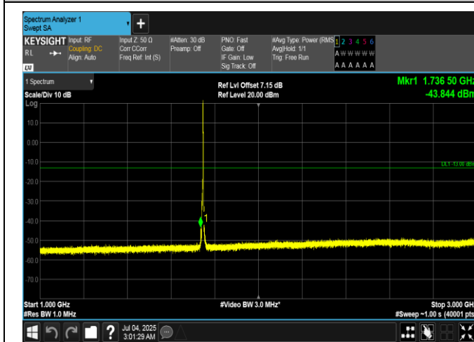
Band66-3MHz-16QAM-132322-1RB#14-1000~3000-PASS
