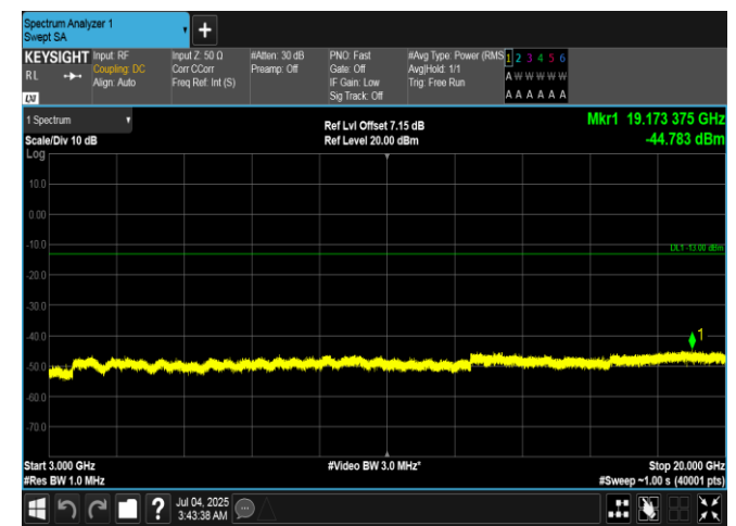
Band66-5MHz-QPSK-131997-1RB#24-3000~20000-PASS
