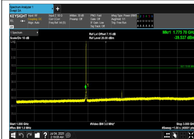
Band66-1.4MHz-16QAM-132665-6RB#0-1000~3000-PASS
