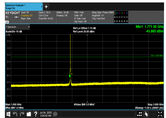
Band66-3MHz-QPSK-132657-1RB#0-1000-3000-PASS
