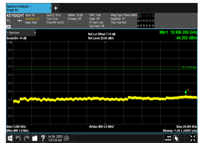
Band66-3MHz-QPSK-132657-1RB#14-3000~20000-PASS
