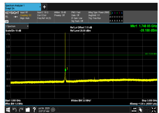
Band66-1.4MHz-16QAM-132322-1RB#0-1000~3000-PASS
