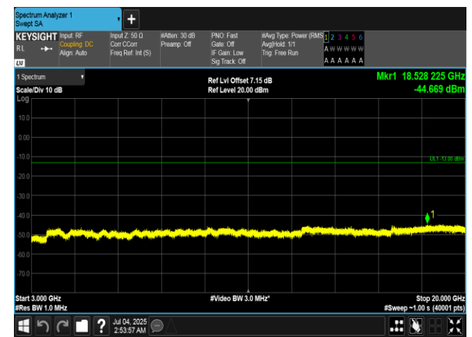
Band66-3MHz-QPSK-131987-1RB#14-3000~20000-PASS
