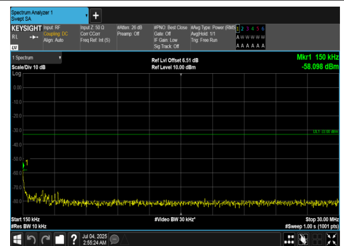
Band66-3MHz-QPSK-131987-15RB#0-0.15~30-PASS
