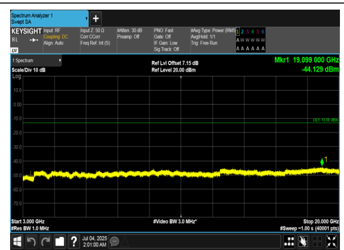
Band66-1.4MHz-16QAM-131979-1RB#0-3000~20000-PASS
