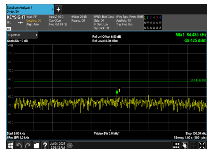
Band66-1.4MHz-16QAM-132322-1RB#5-0.009~0.15-PASS
