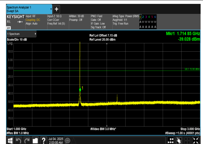
Band66-1.4MHz-16QAM-131979-1RB#5-1000~3000-PASS
