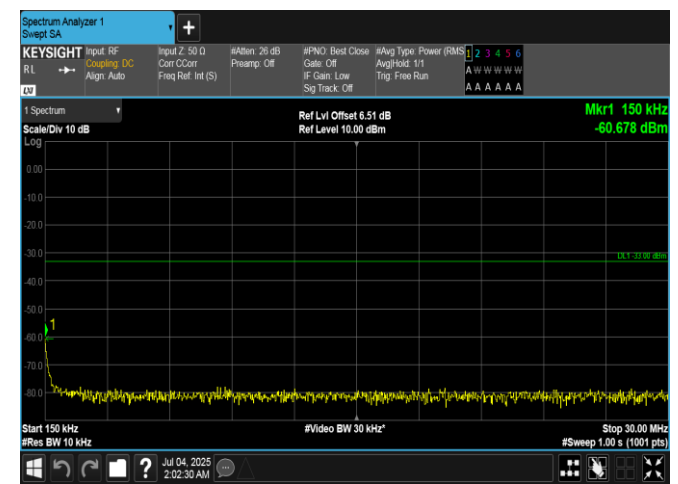
Band66-1.4MHz-16QAM-131979-1RB#5-0.15~30-PASS
