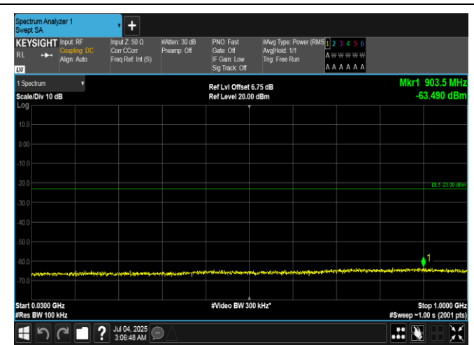
Band66-3MHz-QPSK-132657-1RB#14-30~1000-PASS
