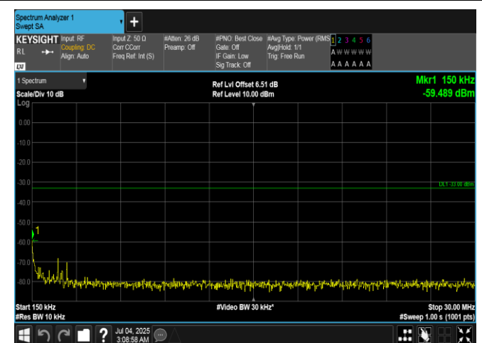
Band66-3MHz-QPSK-132657-15RB#0-0.15~30-PASS
