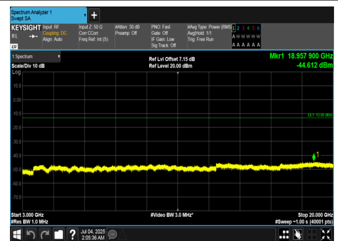
Band66-1.4MHz-16QAM-131979-6RB#0-3000~20000-PASS
