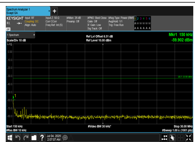
Band66-1.4MHz-16QAM-132322-1RB#0-0.15~30-PASS
