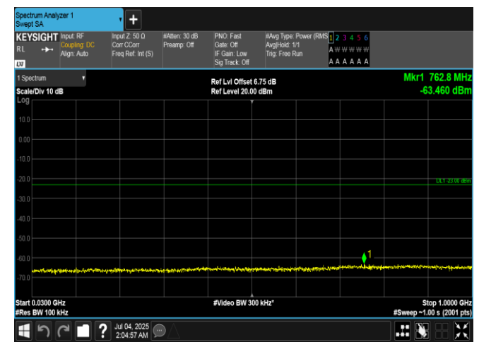
Band66-1.4MHz-16QAM-131979-6RB#0-30~1000-PASS
