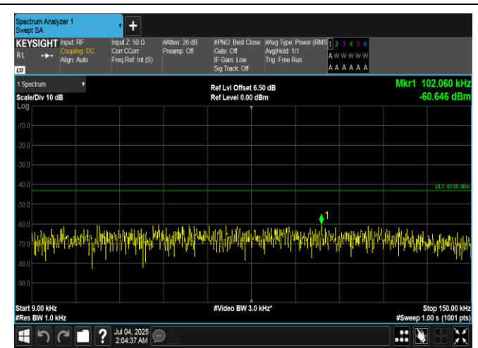
Band66-1.4MHz-16QAM-131979-6RB#0-0.009~0.15-PASS
