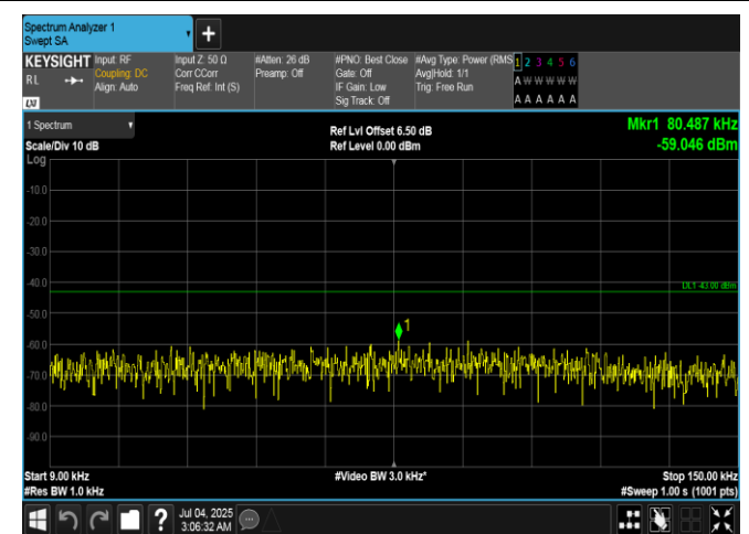
Band66-3MHz-QPSK-132657-1RB#14-0.009-0.15-PASS
