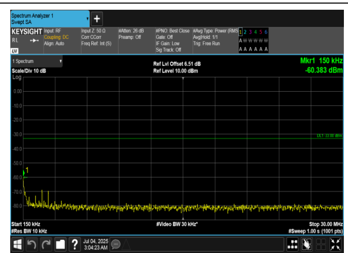
Band66-3MHz-QPSK-132657-1RB#0-0.15-30-PASS
