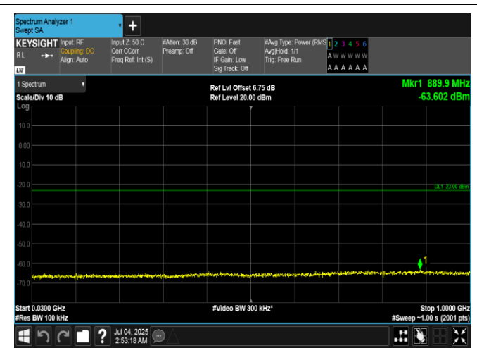
Band66-3MHz-QPSK-131987-1RB#14-30~1000-PASS
