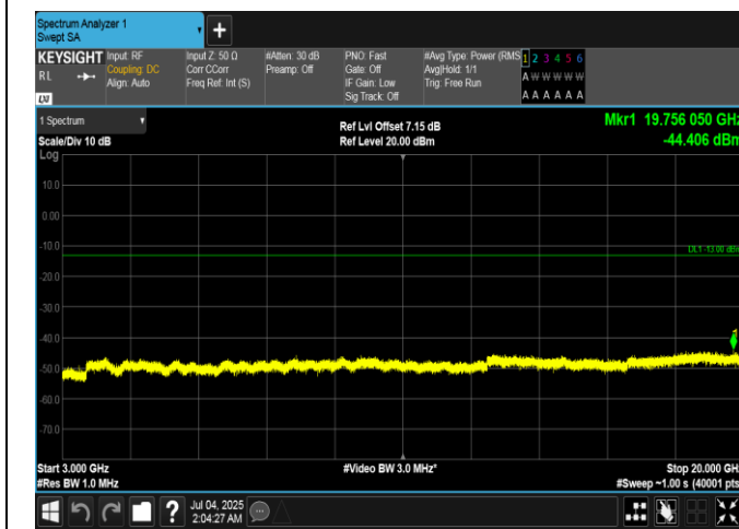
Band66-1.4MHz-QPSK-131979-6RB#0-3000~20000-PASS
