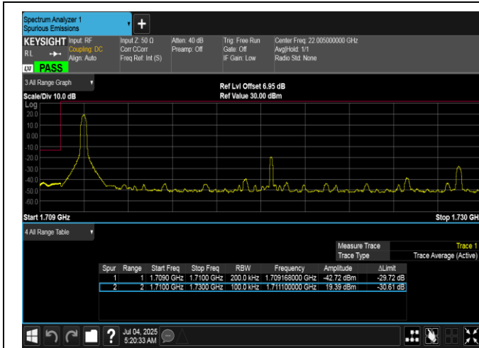
Band66-20MHz-16QAM-132072-1RB#0-PASS
