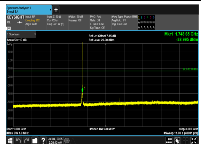
Band66-1.4MHz-QPSK-132322-1RB#5-1000-3000-PASS
