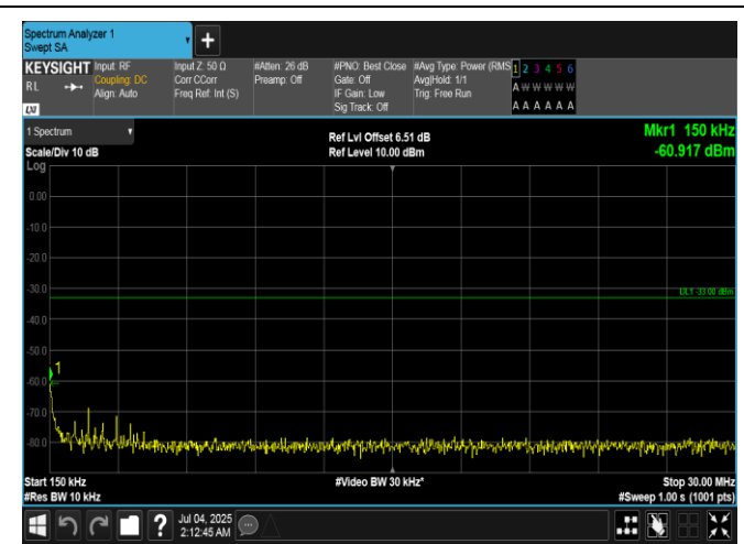
Band66-1.4MHz-QPSK-132665-1RB#0-0.15~30-PASS
