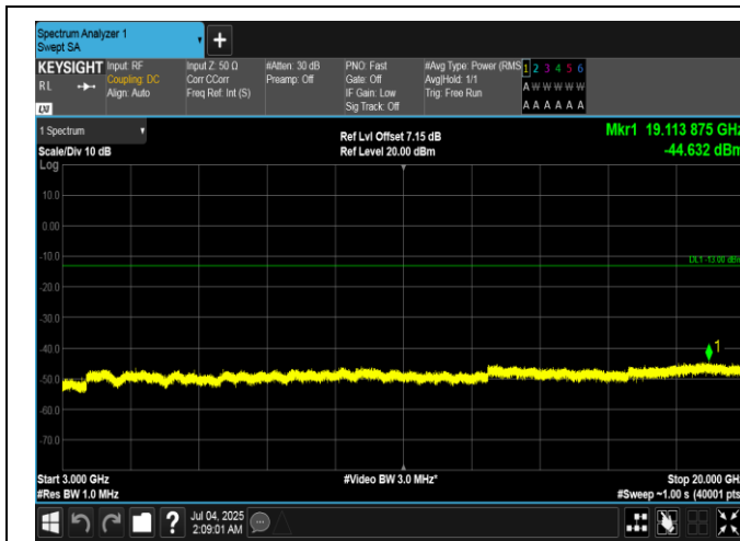
Band66-1.4MHz-QPSK-132322-1RB#5-3000~20000-PASS
