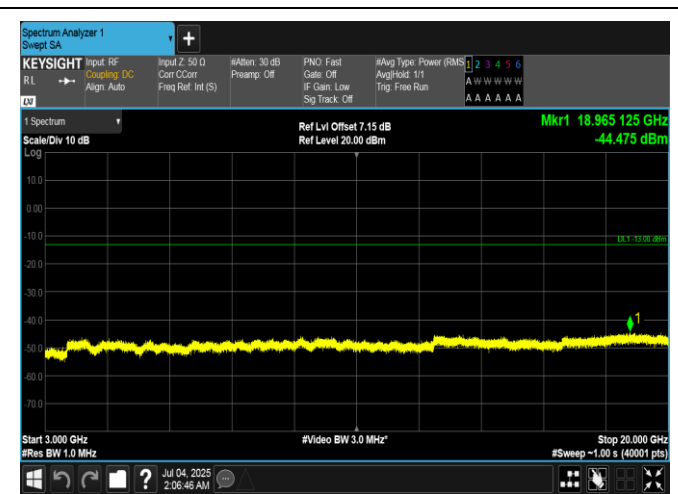
Band66-1.4MHz-QPSK-132322-1RB#0-3000-20000-PASS
