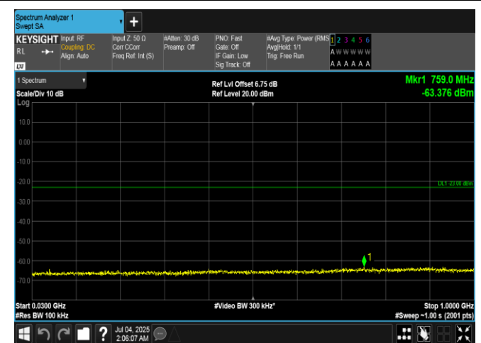
Band66-1.4MHz-QPSK-132322-1RB#0-30~1000-PASS
