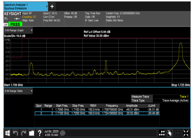
Band66-15MHz-QPSK-132047-1RB#74-PASS
