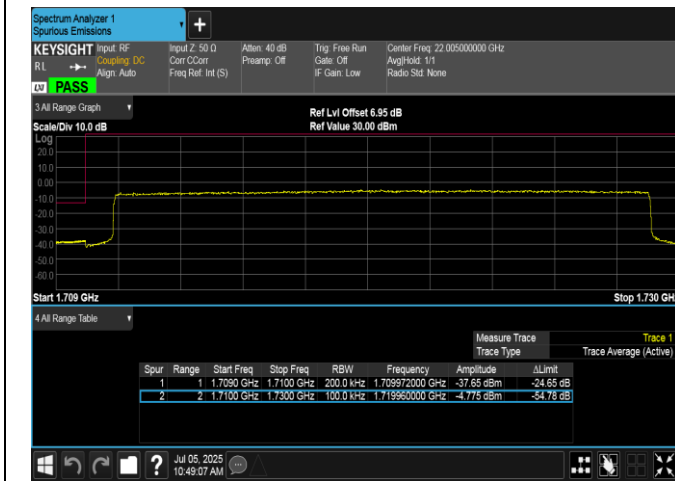
Band66-20MHz-16QAM-132072-100RB#0-PASS
