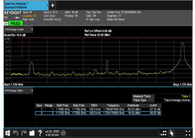
Band66-15MHz-16QAM-132047-1RB#74-PASS
