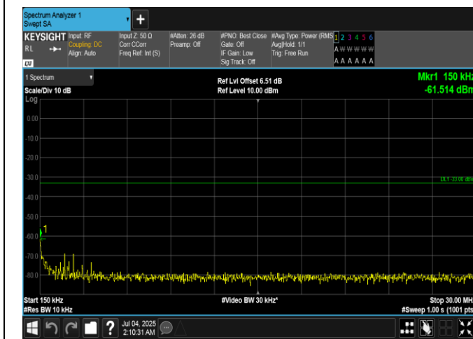
Band66-1.4MHz-QPSK-132322-6RB#0-0.15~30-PASS
