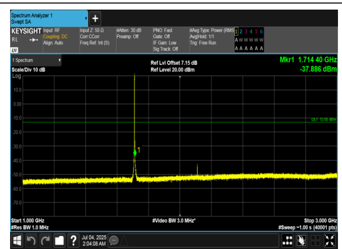
Band66-1.4MHz-QPSK-131979-6RB#0-1000~3000-PASS
