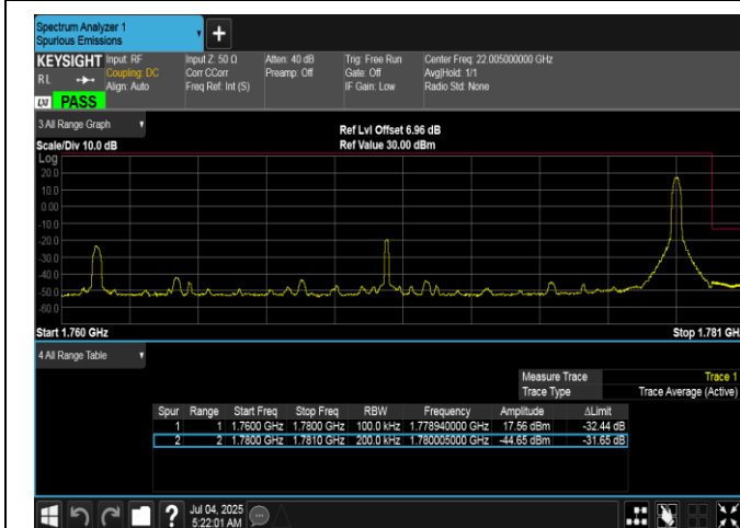
Band66-20MHz-16QAM-132572-1RB#99-PASS
