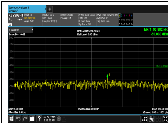
Band66-1.4MHz-QPSK-132665-1RB#0-0.009~0.15-PASS
