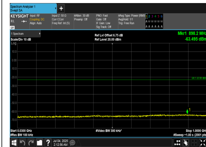
Band66-1.4MHz-QPSK-132665-1RB#0-30~1000-PASS
