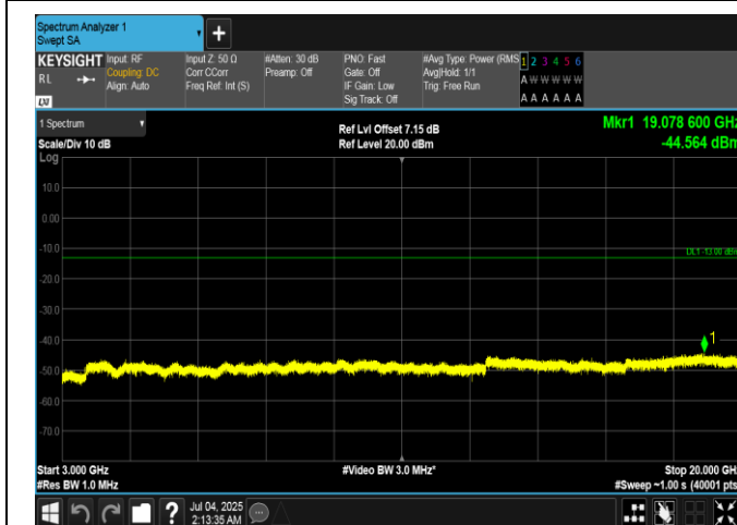
Band66-1.4MHz-QPSK-132665-1RB#0-3000~20000-PASS
