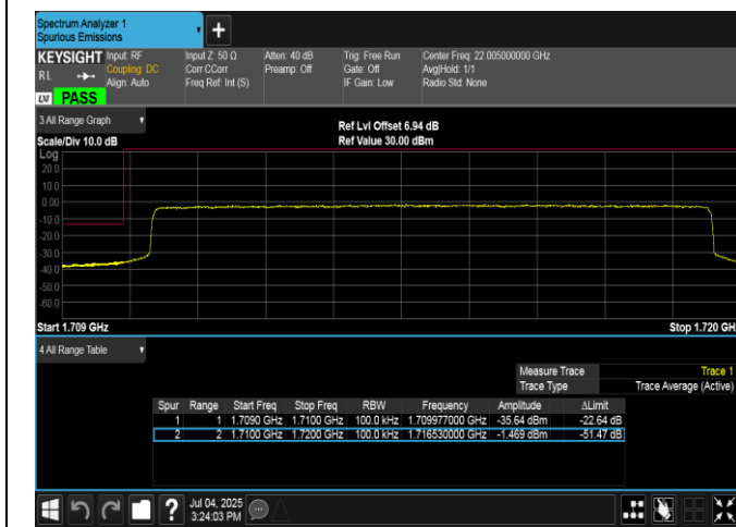
Band66-10MHz-16QAM-132022-50RB#0-PASS
