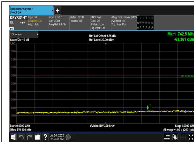
Band66-1.4MHz-QPSK-131979-6RB#0-30~1000-PASS
