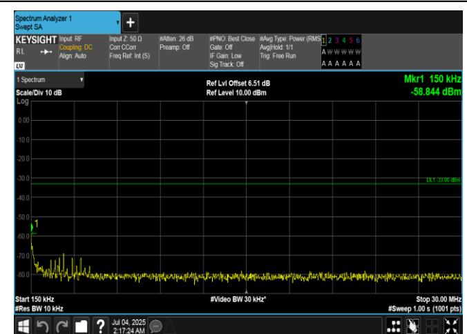
Band66-1.4MHz-QPSK-132665-6RB#0-0.15~30-PASS
