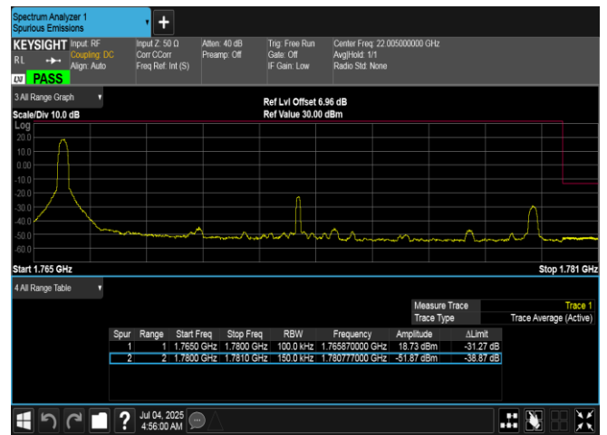
Band66-15MHz-16QAM-132597-1RB#0-PASS
