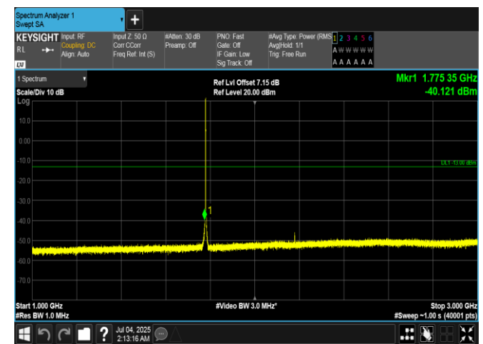
Band66-1.4MHz-QPSK-132665-1RB#0-1000~3000-PASS
