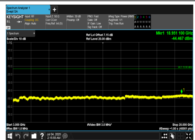
Band66-1.4MHz-QPSK-132665-1RB#5-3000~20000-PASS
