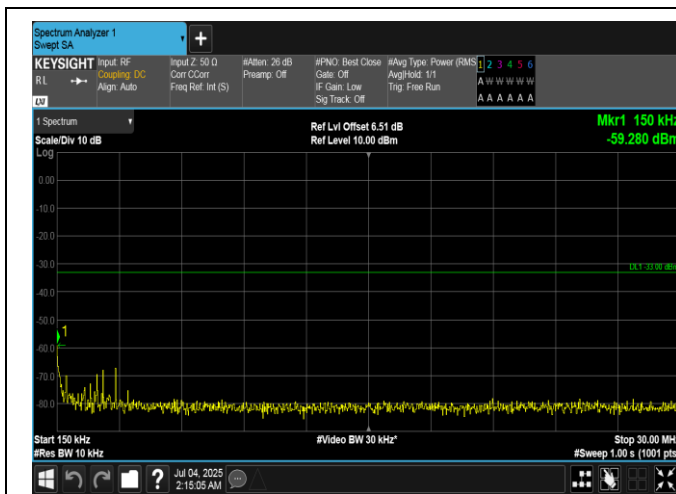
Band66-1.4MHz-QPSK-132665-1RB#5-0.15~30-PASS
