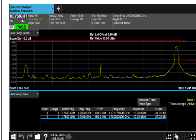
Band66-15MHz-QPSK-132597-1RB#74-PASS
