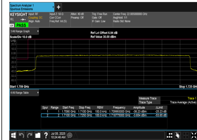
Band66-15MHz-16QAM-132047-75RB#0-PASS
