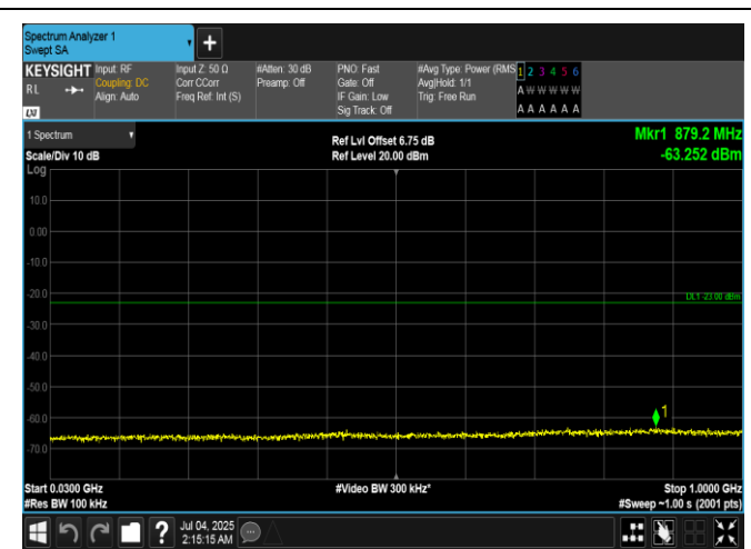
Band66-1.4MHz-QPSK-132665-1RB#5-30~1000-PASS
