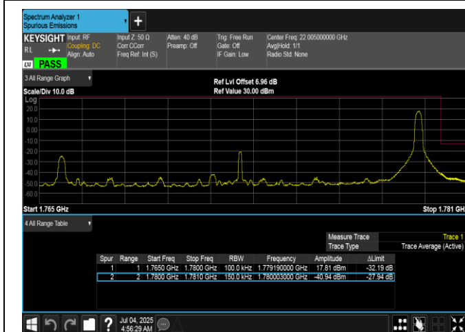
Band66-15MHz-16QAM-132597-1RB#74-PASS
