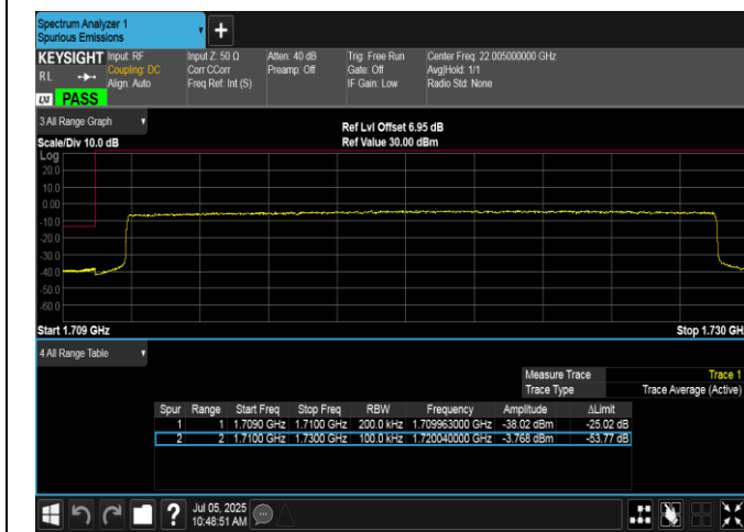
Band66-20MHz-QPSK-132072-100RB#0-PASS
