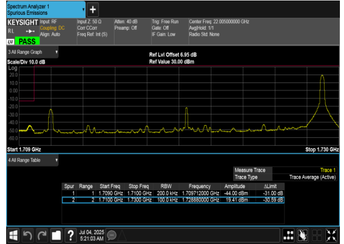
Band66-20MHz-16QAM-132072-1RB#99-PASS
