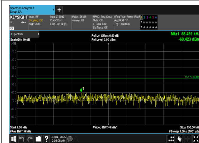
Band66-1.4MHz-QPSK-132322-1RB#5-0.009-0.15-PASS
