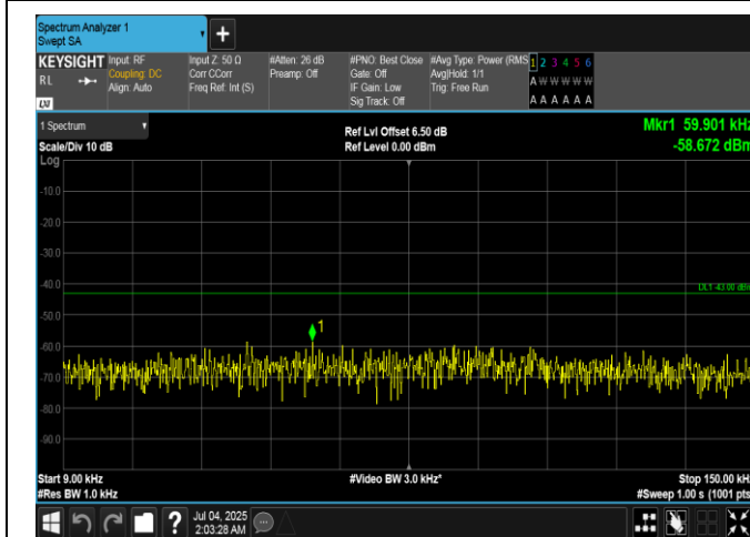
Band66-1.4MHz-QPSK-131979-6RB#0-0.009~0.15-PASS
