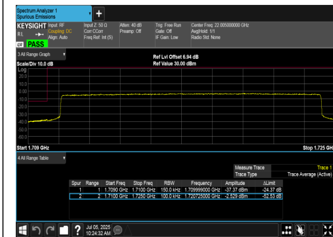
Band66-15MHz-QPSK-132047-75RB#0-PASS
