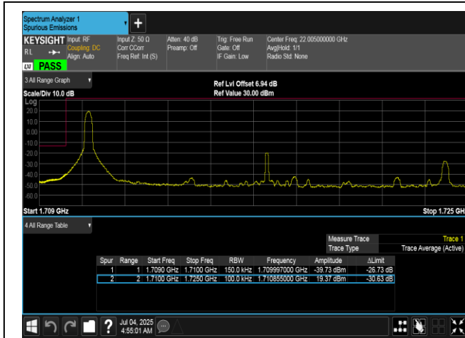
Band66-15MHz-16QAM-132047-1RB#0-PASS
