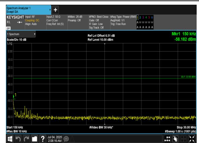
Band66-1.4MHz-QPSK-132322-1RB#5-0.15-30-PASS
