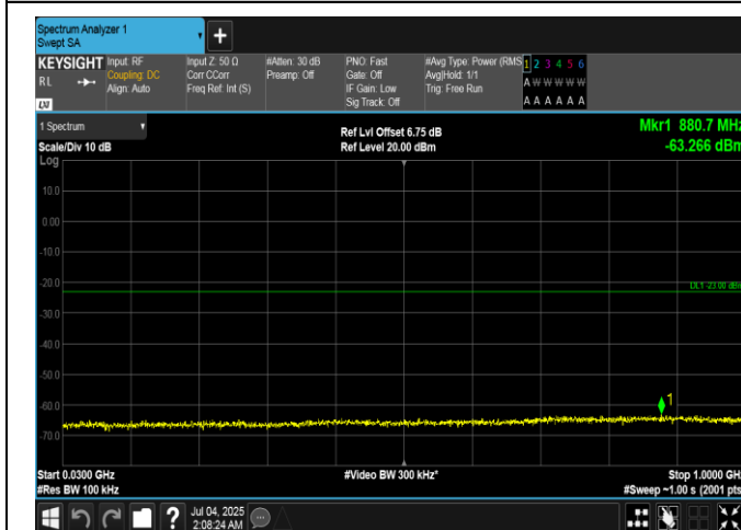
Band66-1.4MHz-QPSK-132322-1RB#5-30-1000-PASS
