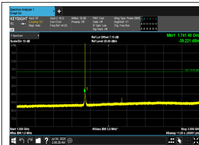
Band66-1.4MHz-QPSK-132322-1RB#0-1000-3000-PASS
