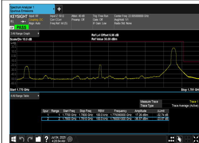
Band66-10MHz-16QAM-132622-1RB#49-PASS
