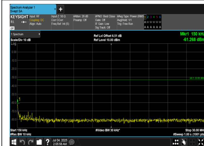
Band66-1.4MHz-QPSK-132322-1RB#0-0.15~30-PASS
