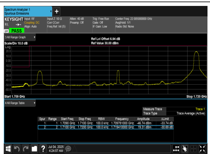
Band66-10MHz-16QAM-132022-1RB#49-PASS
