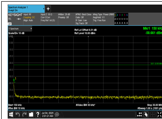
Band66-1.4MHz-QPSK-131979-1RB#5-0.15~30-PASS
