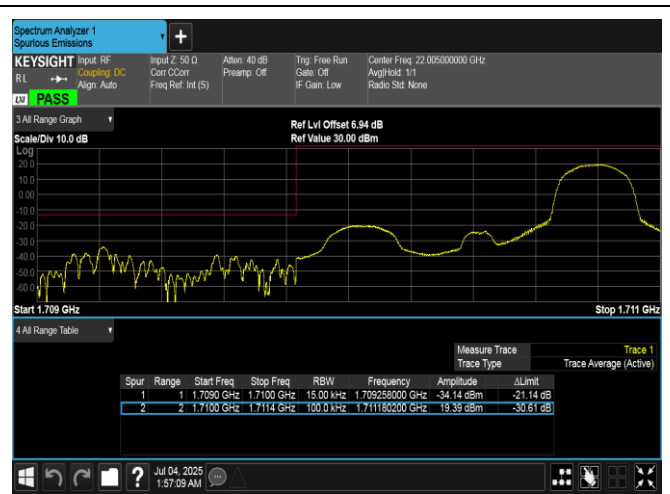
Band66-1.4MHz-16QAM-131979-1RB#5-PASS
