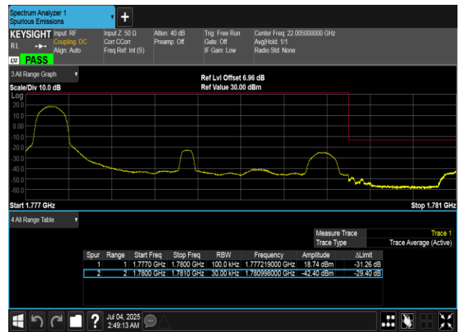
Band66-3MHz-QPSK-132657-1RB#0-PASS
