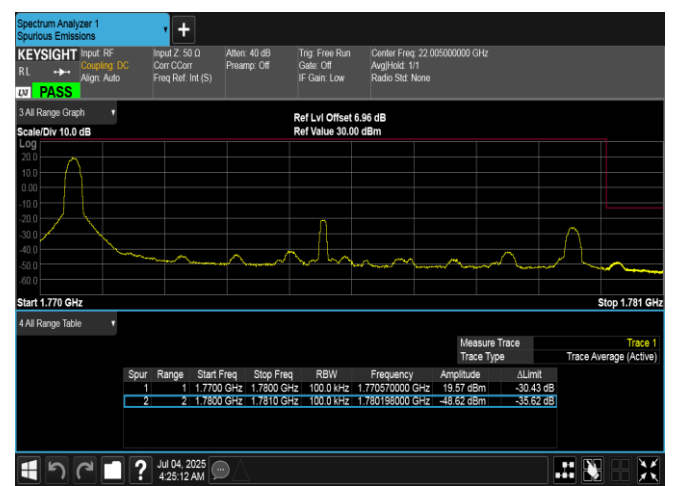
Band66-10MHz-QPSK-132622-1RB#0-PASS
