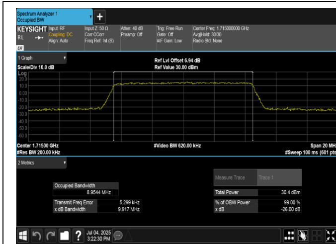
Band66-10MHz-QPSK-132022-50RB#0-PASS
