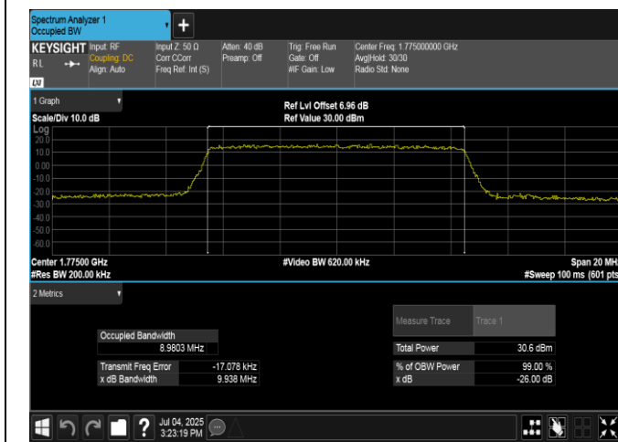
Band66-10MHz-QPSK-132622-50RB#0-PASS
