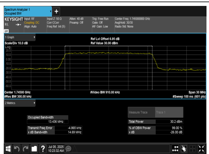
Band66-15MHz-QPSK-132322-75RB#0-PASS
