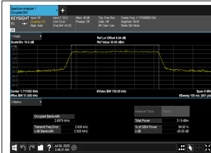
Band66-3MHz-QPSK-131987-15RB#0-PASS
