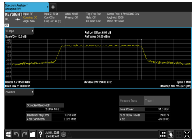
Band66-3MHz-16QAM-131987-15RB#0-PASS
