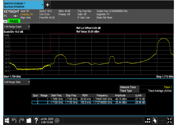
Band66-3MHz-QPSK-131987-1RB#14-PASS
