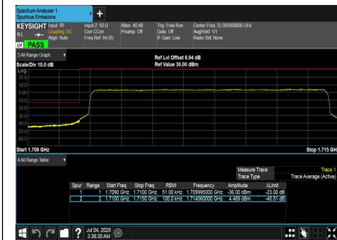
Band66-5MHz-QPSK-131997-25RB#0-PASS
