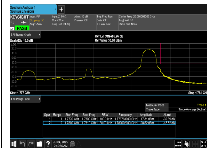
Band66-3MHz-16QAM-132657-1RB#14-PASS
