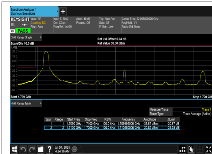
Band66-10MHz-QPSK-132022-1RB#0-PASS
