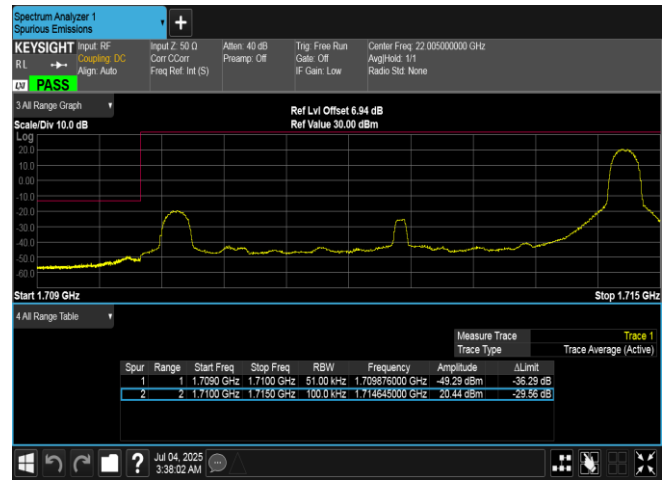
Band66-5MHz-QPSK-131997-1RB#24-PASS
