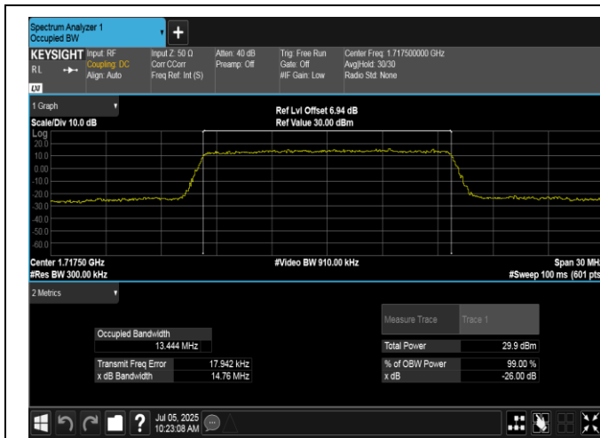
Band66-15MHz-QPSK-132047-75RB#0-PASS
