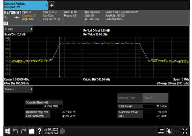
Band66-5MHz-QPSK-132322-25RB#0-PASS
