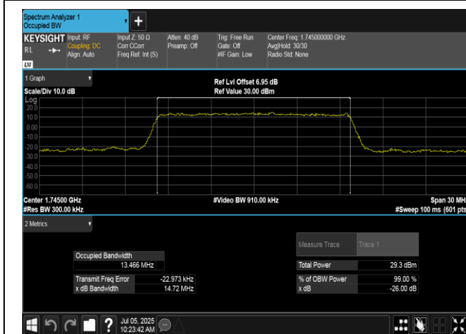
Band66-15MHz-16QAM-132322-75RB#0-PASS
