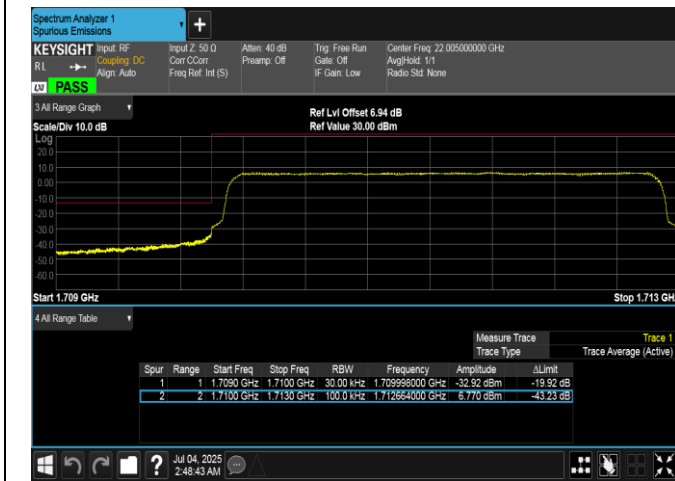
Band66-3MHz-QPSK-131987-15RB#0-PASS
