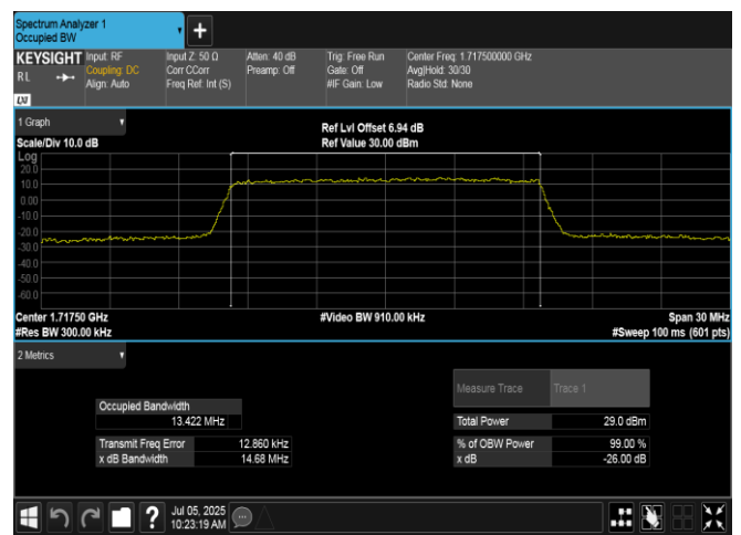
Band66-15MHz-16QAM-132047-75RB#0-PASS
