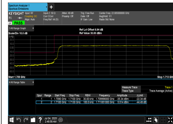
Band66-3MHz-16QAM-131987-15RB#0-PASS
