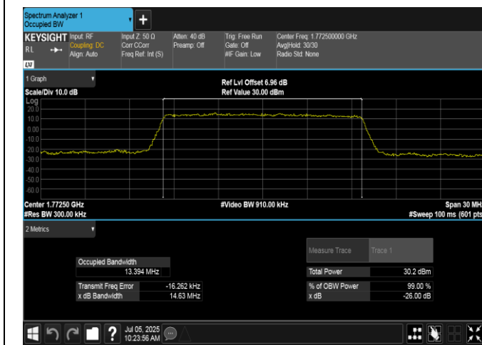
Band66-15MHz-QPSK-132597-75RB#0-PASS
