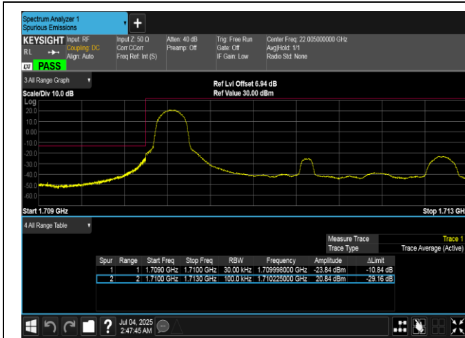
Band66-3MHz-QPSK-131987-1RB#0-PASS
