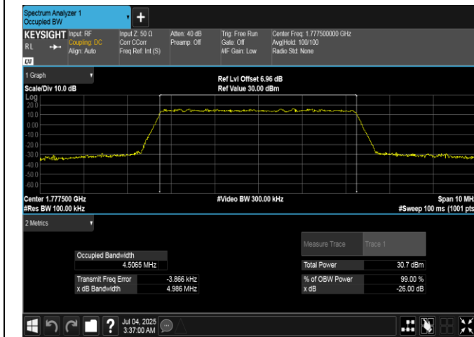
Band66-5MHz-QPSK-132647-25RB#0-PASS
