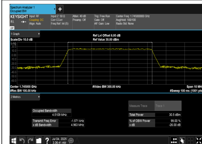
Band66-5MHz-16QAM-132322-25RB#0-PASS
