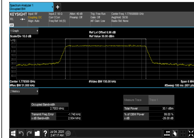
Band66-3MHz-QPSK-132657-15RB#0-PASS
