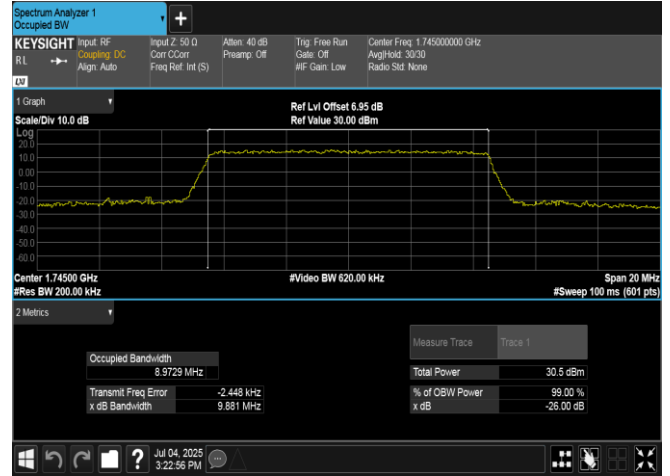
Band66-10MHz-QPSK-132322-50RB#0-PASS
