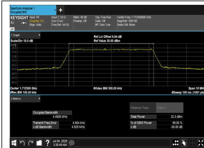
Band66-5MHz-QPSK-131997-25RB#0-PASS
