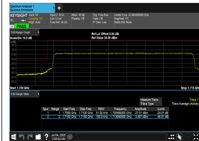
Band66-5MHz-16QAM-131997-25RB#0-PASS
