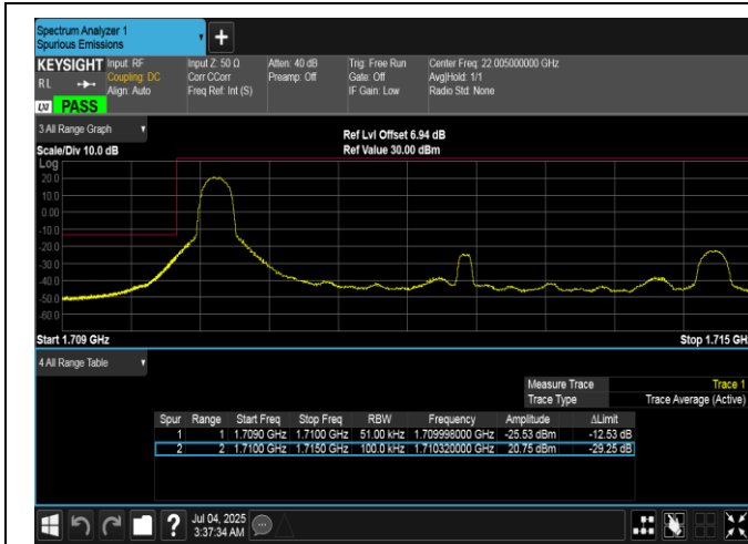
Band66-5MHz-QPSK-131997-1RB#0-PASS
