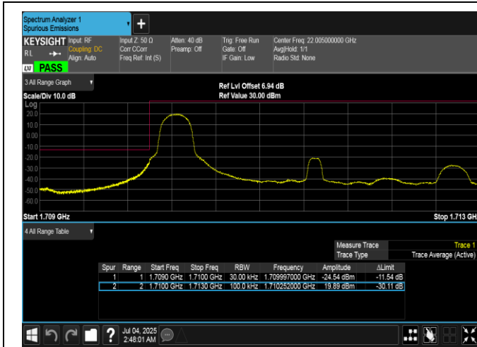
Band66-3MHz-16QAM-131987-1RB#0-PASS
