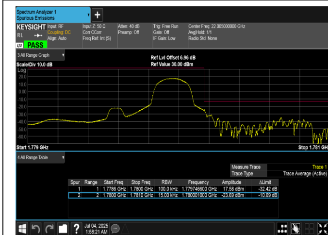
Band66-1.4MHz-16QAM-132665-1RB#5-PASS
