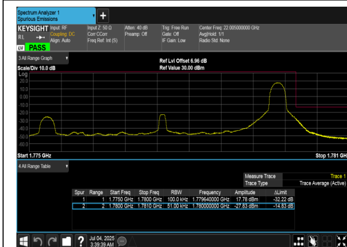
Band66-5MHz-16QAM-132647-1RB#24-PASS
