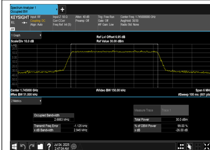
Band66-3MHz-16QAM-132322-15RB#0-PASS
