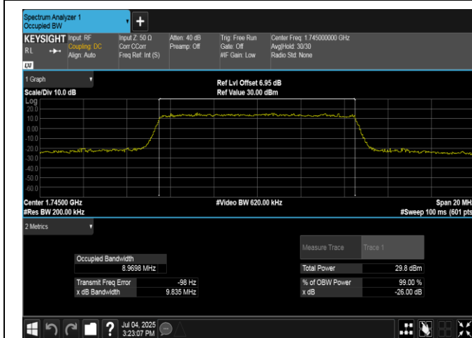
Band66-10MHz-16QAM-132322-50RB#0-PASS
