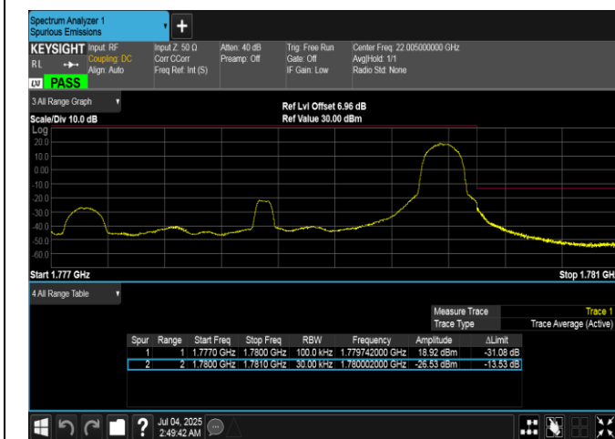
Band66-3MHz-QPSK-132657-1RB#14-PASS
