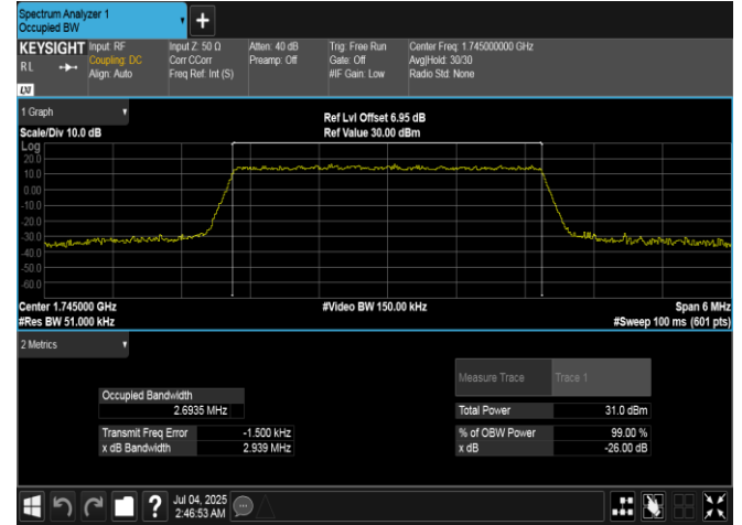
Band66-3MHz-QPSK-132322-15RB#0-PASS
