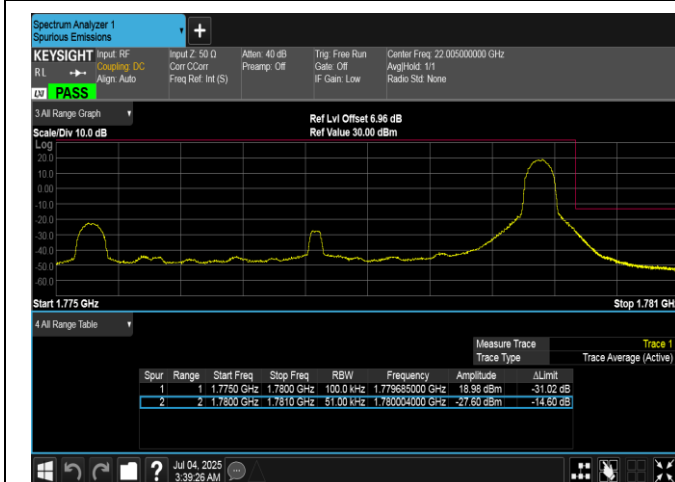
Band66-5MHz-QPSK-132647-1RB#24-PASS
