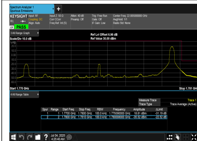
Band66-10MHz-QPSK-132622-1RB#49-PASS
