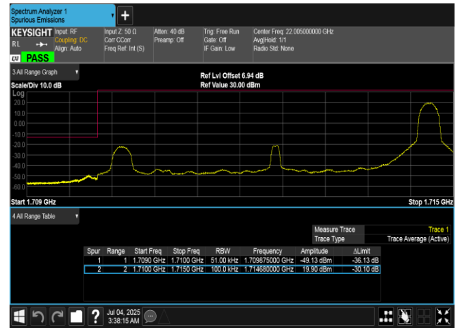
Band66-5MHz-16QAM-131997-1RB#24-PASS
