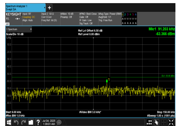
Band7-20MHz-QPSK-21350-1RB#99-0.009~0.15-PASS
