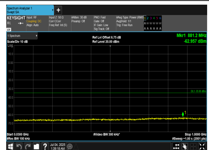
Band7-20MHz-QPSK-21350-1RB#99-30~1000-PASS
