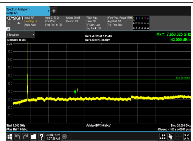
Band7-20MHz-QPSK-21350-1RB#0-1000~20000-PASS
