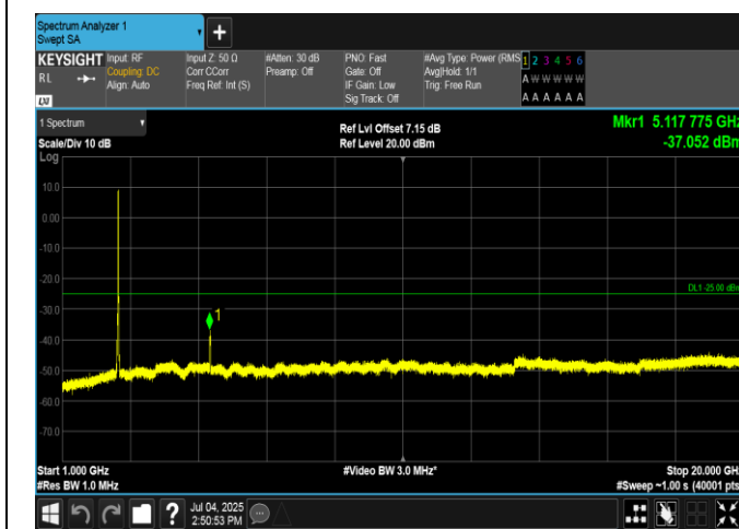
Band7-20MHz-16QAM-21350-100RB#0-1000~20000-PASS
