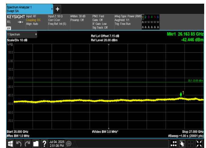
Band7-20MHz-16QAM-21350-100RB#0-20000~27000-PASS
