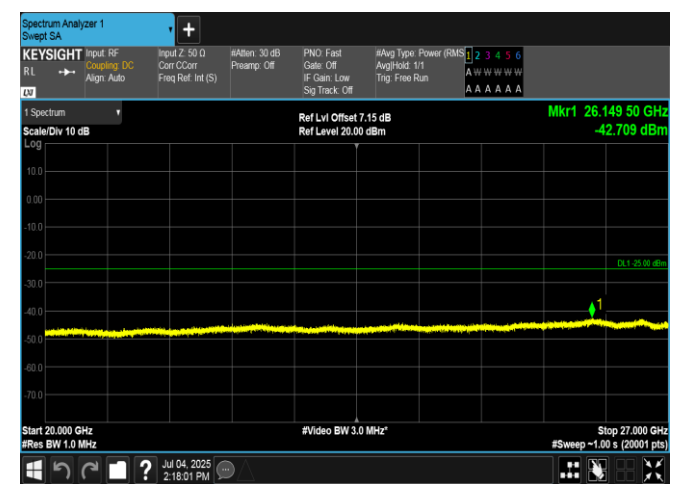
Band7-15MHz-16QAM-20825-75RB#0-20000~27000-PASS
