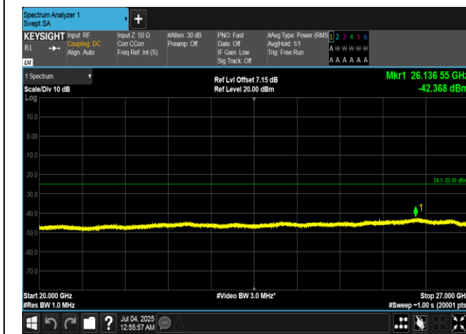
Band7-15MHz-16QAM-21100-1RB#0-20000~27000-PASS
