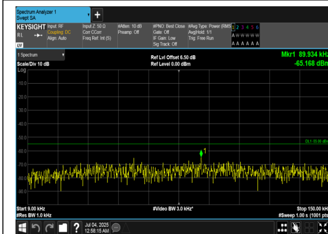
Band7-15MHz-QPSK-21375-1RB#0-0.009~0.15-PASS
