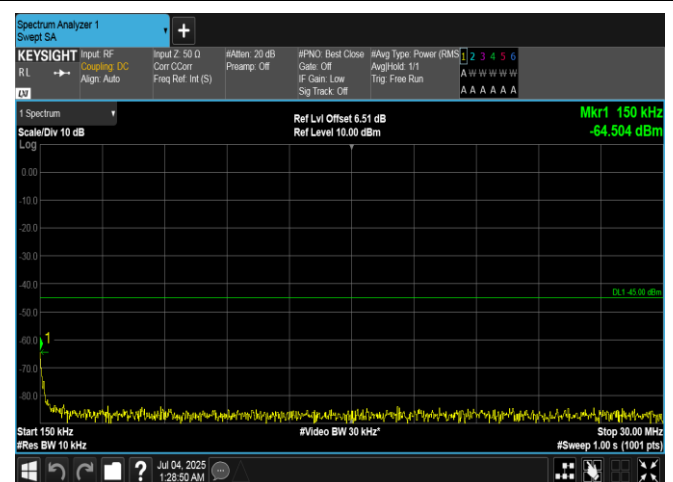
Band7-20MHz-QPSK-20850-1RB#0-0.15~30-PASS
