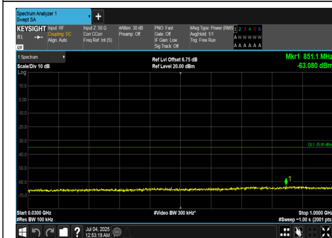
Band7-15MHz-16QAM-20825-1RB#74-30~1000-PASS
