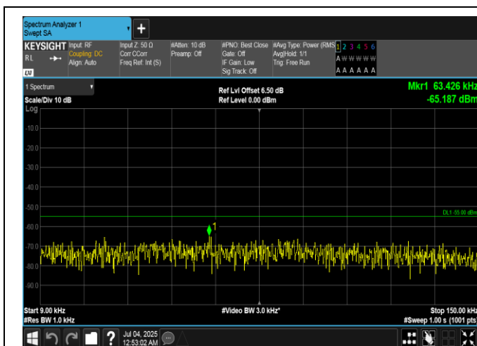
Band7-15MHz-16OAM-20825-1RB#74-0.009~0.15-PASS
