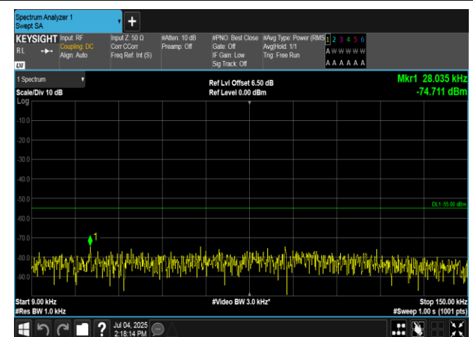
Band7-15MHz-QPSK-21100-75RB#0-0.009~0.15-PASS
