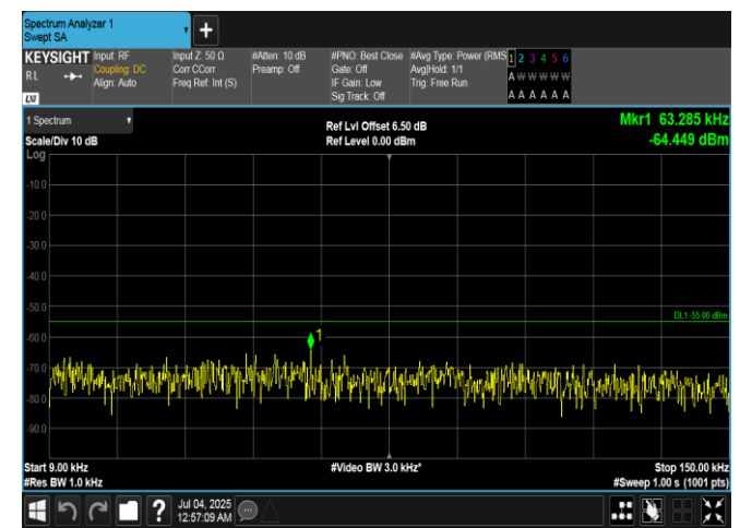
Band7-15MHz-16QAM-21100-1RB#74-0.009~0.15-PASS
