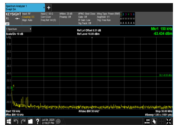
Band7-15MHz-16QAM-21100-75RB#0-0.15~30-PASS
