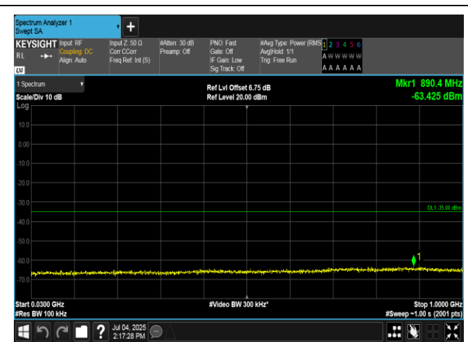
Band7-15MHz-16QAM-20825-75RB#0-30~1000-PASS
