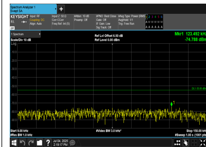
Band7-15MHz-16QAM-21100-75RB#0-0.009~0.15-PASS
