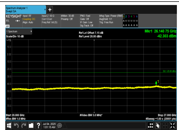
Band7-15MHz-QPSK-21375-1RB#74-20000~27000-PASS
