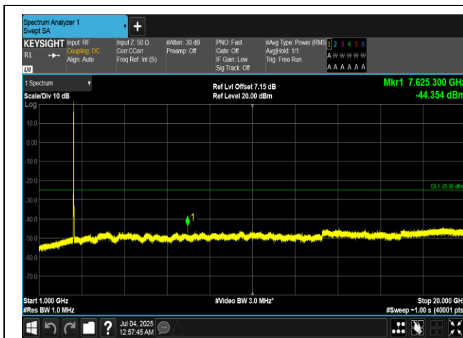
Band7-15MHz-16QAM-21100-1RB#74-1000~20000-PASS
