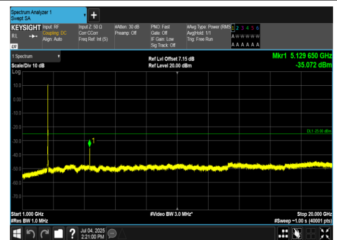
Band7-15MHz-QPSK-21375-75RB#0-1000~20000-PASS
