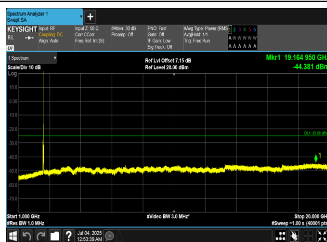
Band7-15MHz-16QAM-20825-1RB#74-1000~20000-PASS
