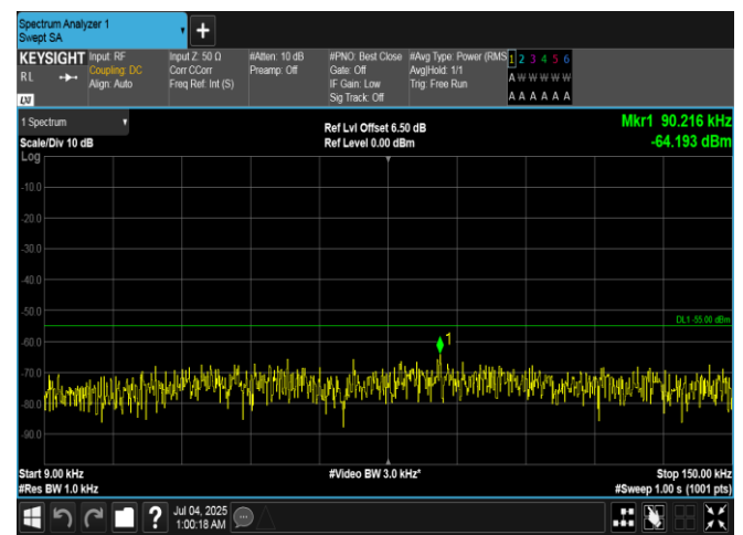
Band7-15MHz-QPSK-21375-1RB#74-0.009~0.15-PASS
