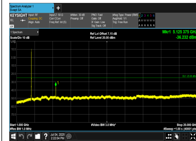
Band7-15MHz-16QAM-21375-75RB#0-1000~20000-PASS
