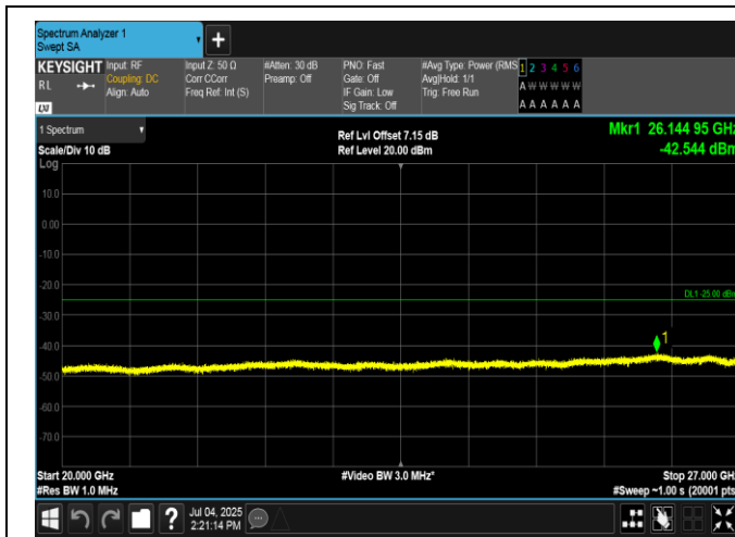
Band7-15MHz-QPSK-21375-75RB#0-20000~27000-PASS
