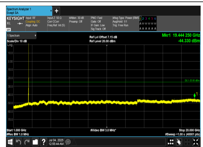
Band7-15MHz-16QAM-21100-1RB#0-1000~20000-PASS
