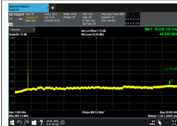
Band7-15MHz-16QAM-20825-1RB#0-1000~20000-PASS
