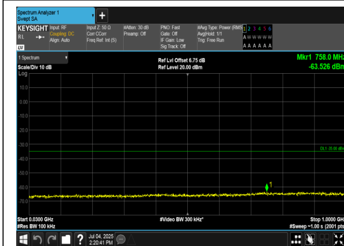
Band7-15MHz-QPSK-21375-75RB#0-30~1000-PASS
