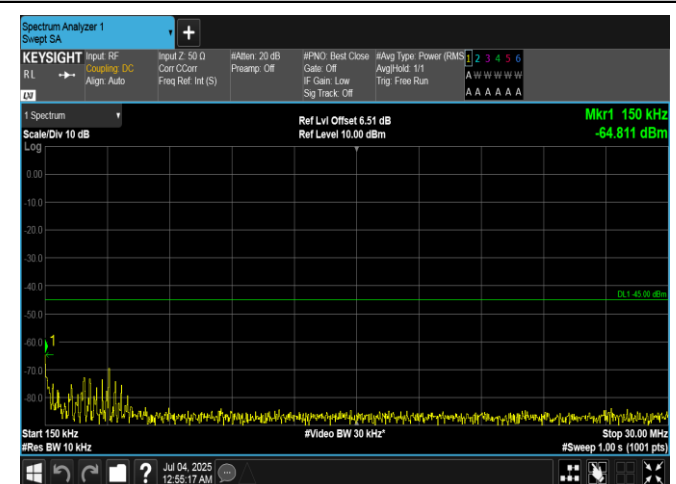
Band7-15MHz-16QAM-21100-1RB#0-0.15~30-PASS
