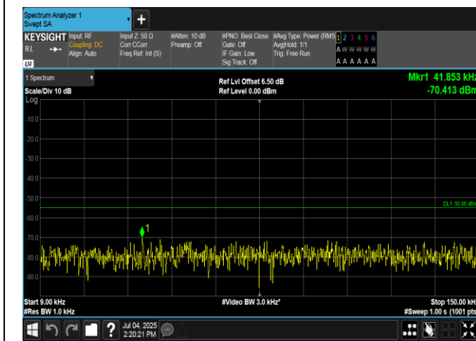
Band7-15MHz-QPSK-21375-75RB#0-0.009~0.15-PASS
