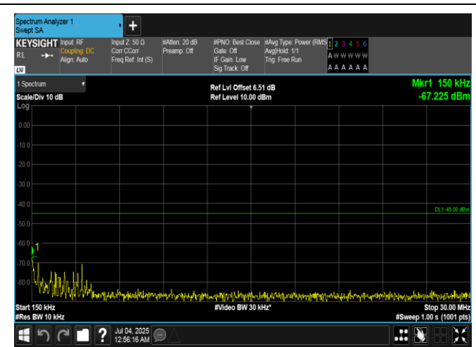
Band7-15MHz-QPSK-21100-1RB#74-0.15~30-PASS
