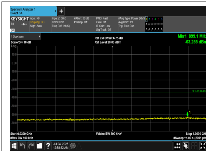
Band7-15MHz-QPSK-21375-1RB#0-30~1000-PASS
