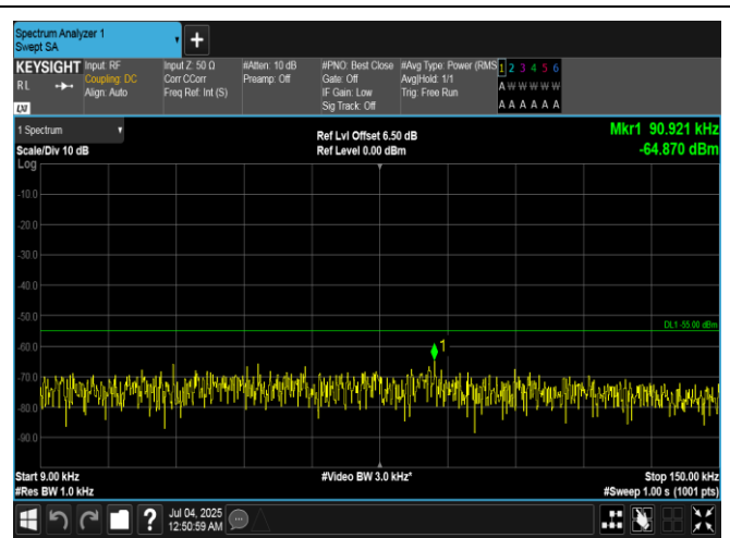
Band7-15MHz-16QAM-20825-1RB#0-0.009~0.15-PASS
