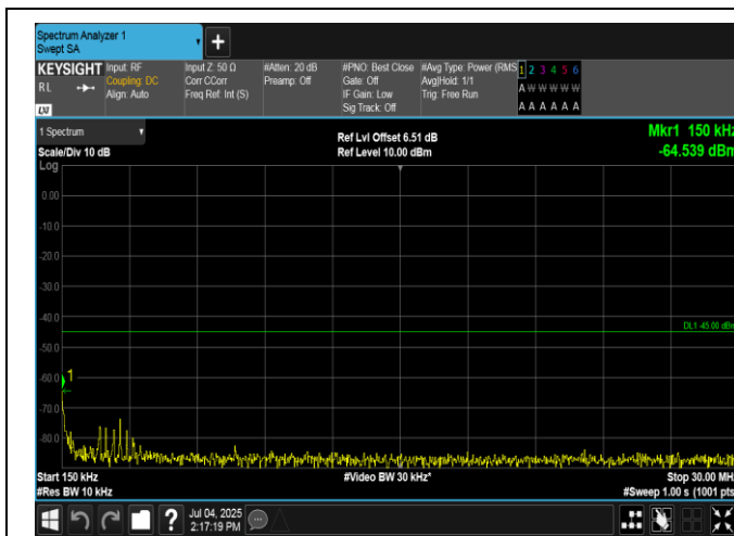
Band7-15MHz-16QAM-20825-75RB#0-0.15~30-PASS
