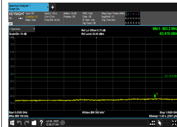
Band7-15MHz-QPSK-21100-1RB#74-30~1000-PASS
