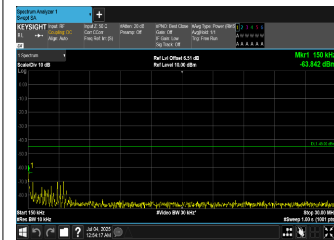
Band7-15MHz-QPSK-21100-1RB#0-0.15~30-PASS
