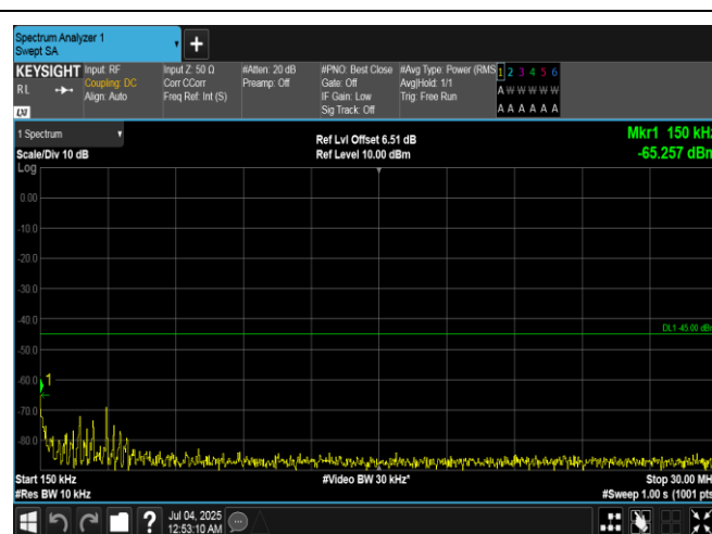
Band7-15MHz-16OAM-20825-1RB#74-0.15~30-PASS
