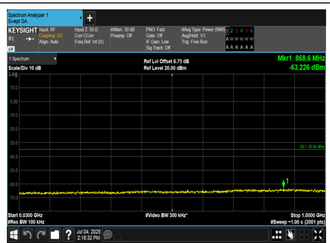
Band7-15MHz-QPSK-21100-75RB#0-30~1000-PASS
