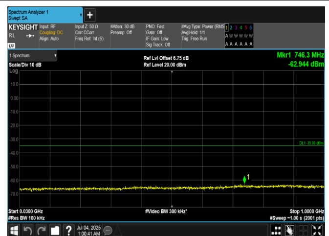
Band7-15MHz-QPSK-21375-1RB#74-30~1000-PASS
