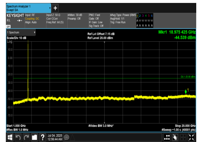
Band7-15MHz-QPSK-21100-1RB#74-1000~20000-PASS
