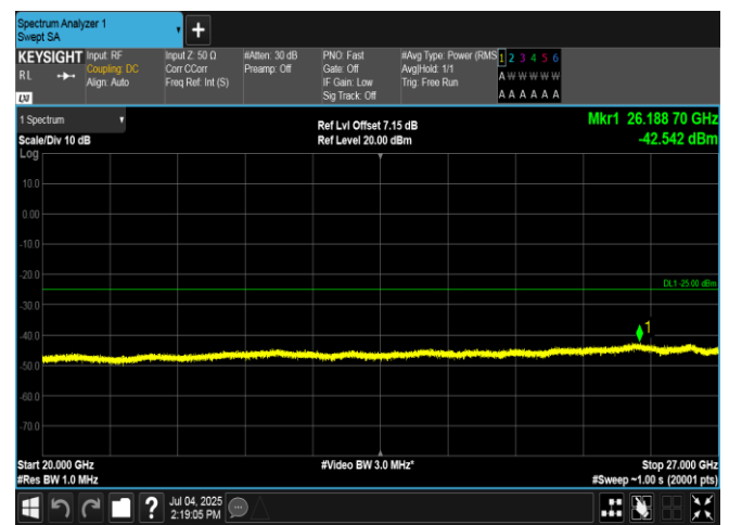
Band7-15MHz-QPSK-21100-75RB#0-20000~27000-PASS
