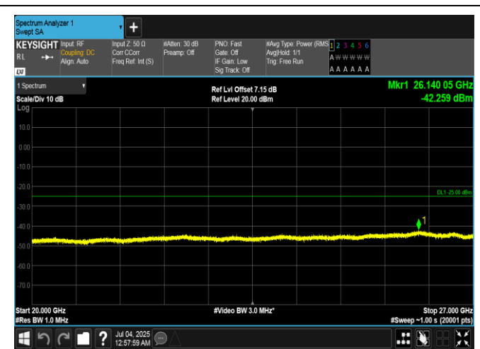
Band7-15MHz-16QAM-21100-1RB#74-20000~27000-PASS
