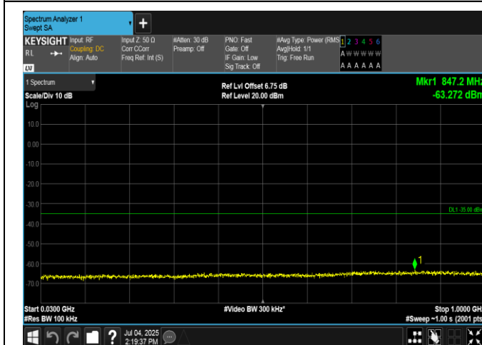
Band7-15MHz-16QAM-21100-75RB#0-30~1000-PASS
