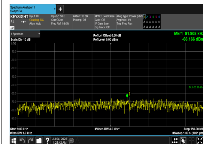
Band7-20MHz-QPSK-20850-1RB#0-0.009~0.15-PASS
