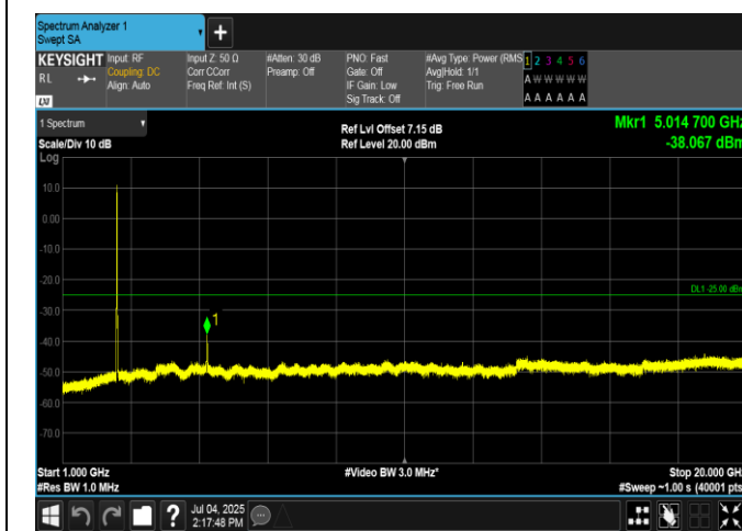
Band7-15MHz-16QAM-20825-75RB#0-1000~20000-PASS
