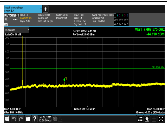
Band7-15MHz-QPSK-21375-1RB#0-1000~20000-PASS
