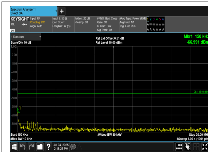
Band7-15MHz-QPSK-21100-75RB#0-0.15~30-PASS
