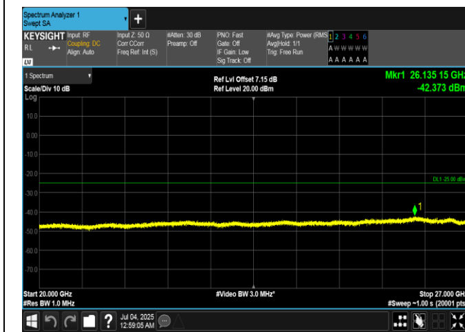
Band7-15MHz-QPSK-21375-1RB#0-20000~27000-PASS
