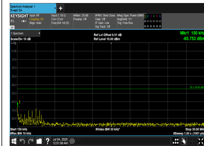
Band7-15MHz-16QAM-20825-1RB#0-0.15~30-PASS
