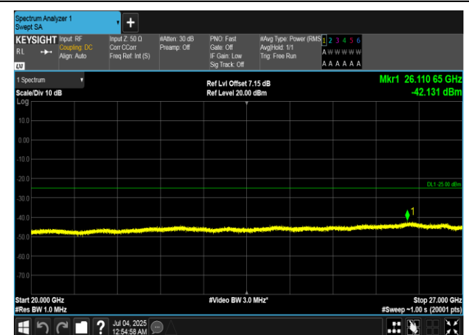
Band7-15MHz-QPSK-21100-1RB#0-20000~27000-PASS
