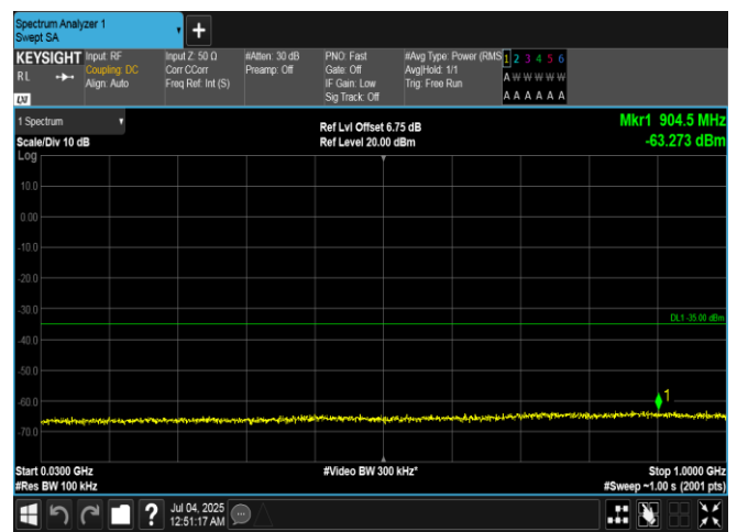
Band7-15MHz-16QAM-20825-1RB#0-30~1000-PASS
