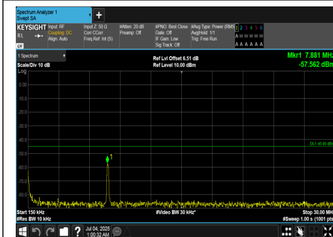
Band7-15MHz-QPSK-21375-1RB#74-0.15~30-PASS
