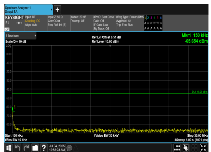
Band7-15MHz-QPSK-21375-1RB#0-0.15~30-PASS
