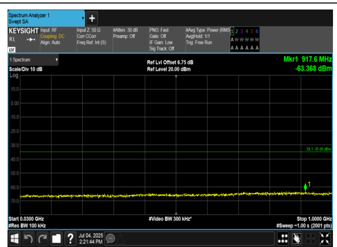
Band7-15MHz-16QAM-21375-75RB#0-30~1000-PASS
