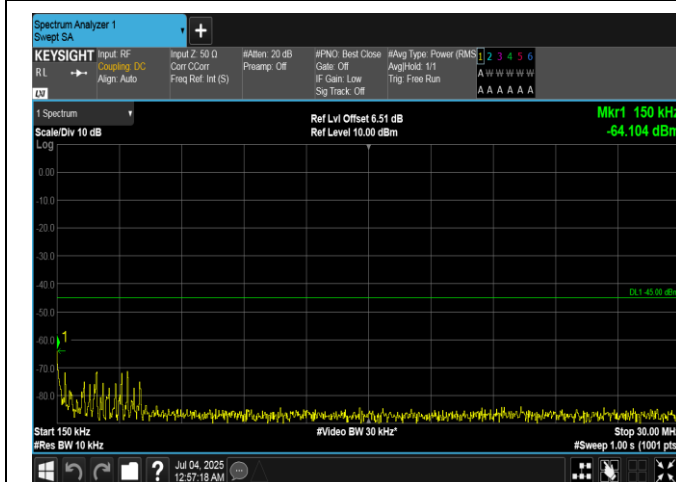
Band7-15MHz-16QAM-21100-1RB#74-0.15~30-PASS
