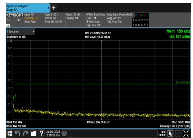
Band7-15MHz-QPSK-21375-75RB#0-0.15~30-PASS
