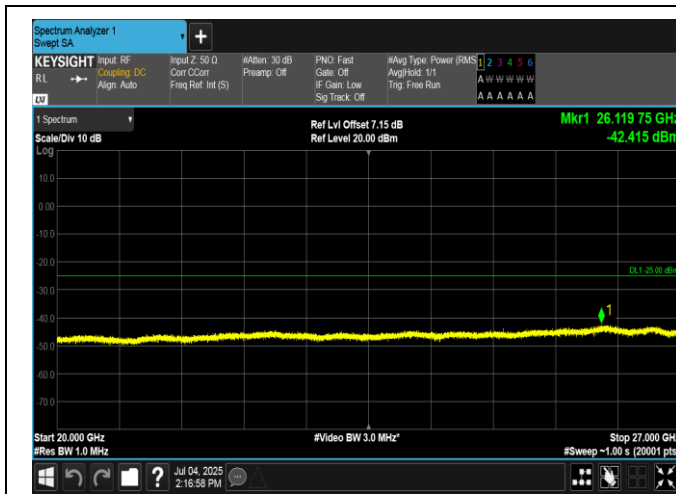
Band7-15MHz-QPSK-20825-75RB#0-20000~27000-PASS
