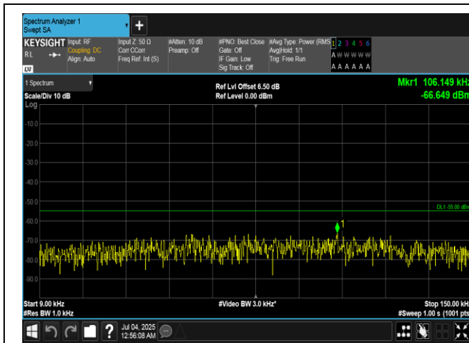
Band7-15MHz-QPSK-21100-1RB#74-0.009~0.15-PASS
