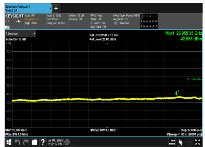
Band7-15MHz-16QAM-21375-75RB#0-20000~27000-PASS
