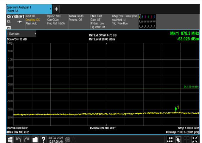
Band7-15MHz-16QAM-21100-1RB#74-30~1000-PASS
