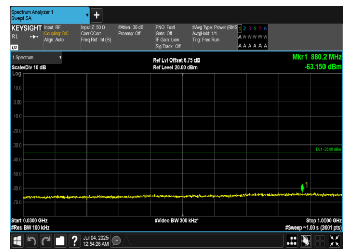
Band7-15MHz-QPSK-21100-1RB#0-30~1000-PASS
