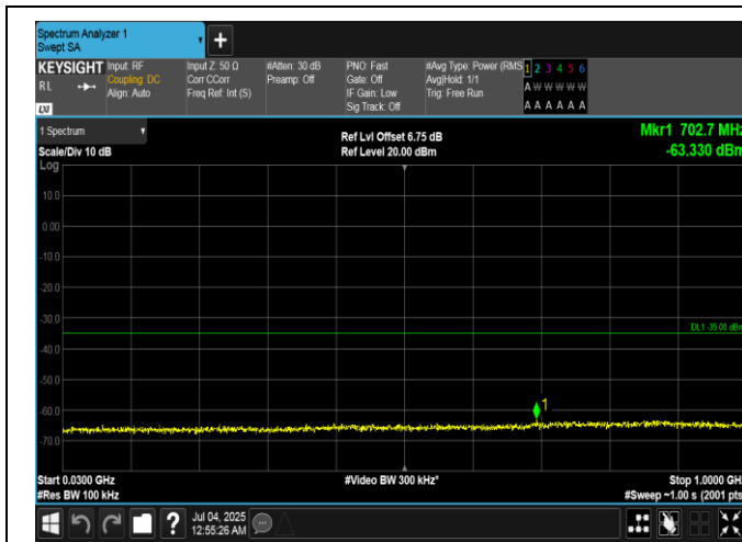
Band7-15MHz-16QAM-21100-1RB#0-30~1000-PASS
