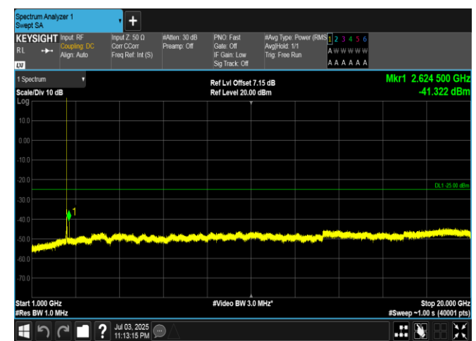
Band7-5MHz-16QAM-20775-1RB#24-1000~20000-PASS
