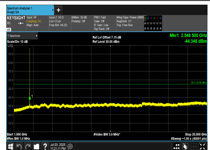
Band7-5MHz-16QAM-21100-25RB#0-1000~20000-PASS
