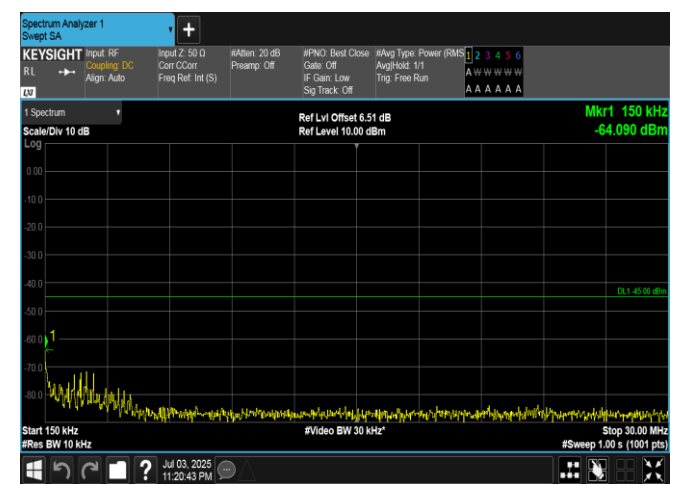
Band7-5MHz-16QAM-21100-25RB#0-0.15~30-PASS
