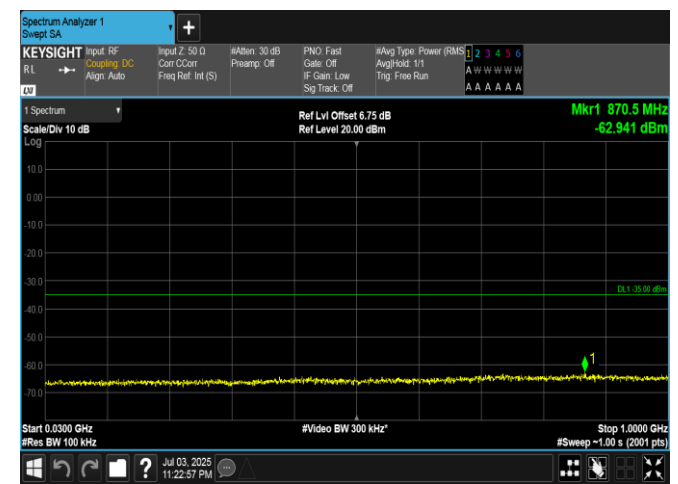
Band7-5MHz-16QAM-21425-1RB#0-30~1000-PASS
