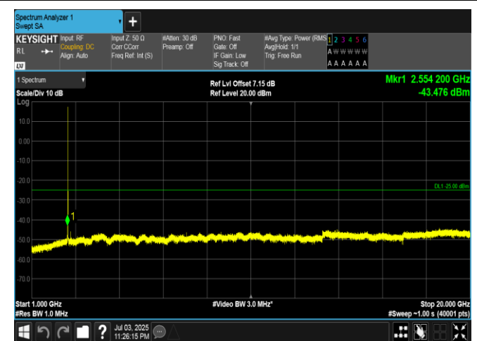
Band7-5MHz-QPSK-21425-25RB#0-1000~20000-PASS
