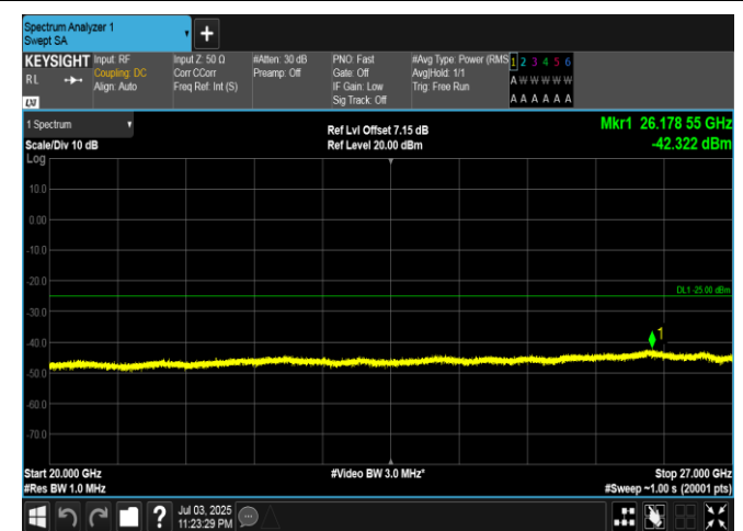
Band7-5MHz-16QAM-21425-1RB#0-20000~27000-PASS
