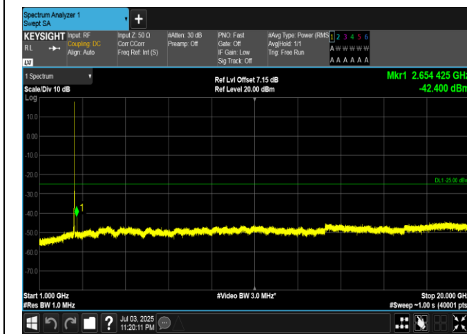
Band7-5MHz-QPSK-21100-25RB#0-1000~20000-PASS
