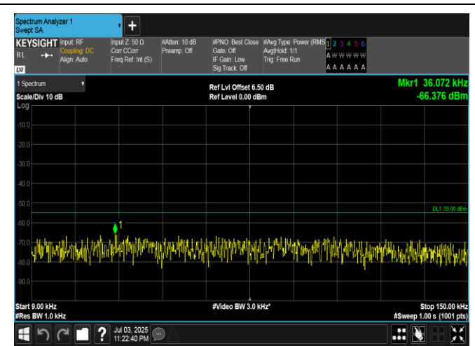
Band7-5MHz-16QAM-21425-1RB#0-0.009~0.15-PASS
