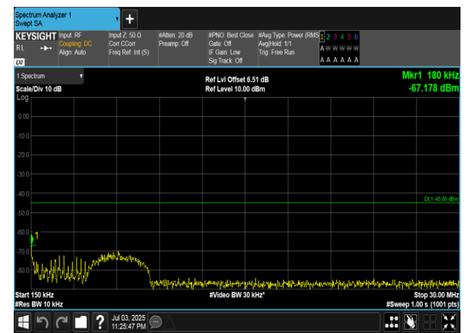
Band7-5MHz-QPSK-21425-25RB#0-0.15~30-PASS
