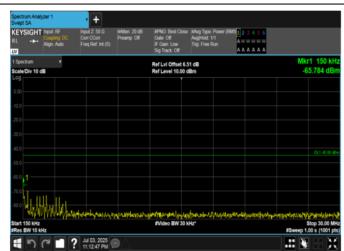
Band7-5MHz-16QAM-20775-1RB#24-0.15~30-PASS
