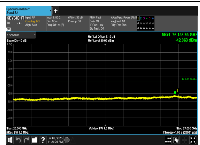
Band7-5MHz-QPSK-21425-1RB#24-20000~27000-PASS
