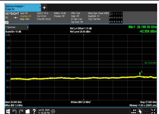
Band7-5MHz-QPSK-21100-1RB#0-20000~27000-PASS
