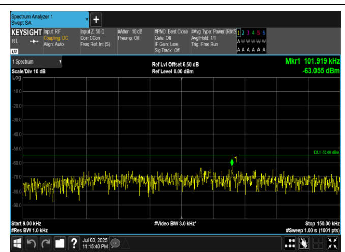
Band7-5MHz-QPSK-21100-1RB#0-0.009~0.15-PASS
