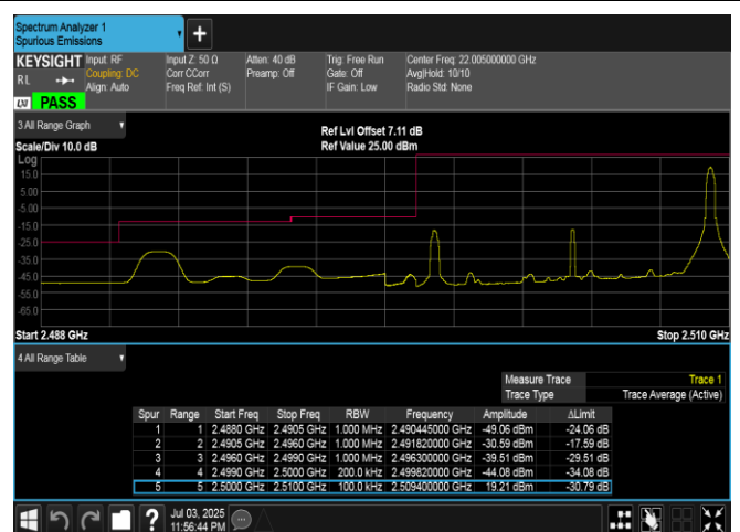
Band7-10MHz-QPSK-20800-1RB#49-PASS
