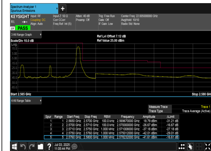
Band7-5MHz-16QAM-21425-1RB#24-PASS
