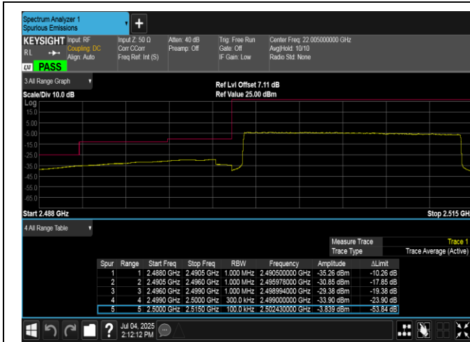
Band7-15MHz-16QAM-20825-75RB#0-PASS
