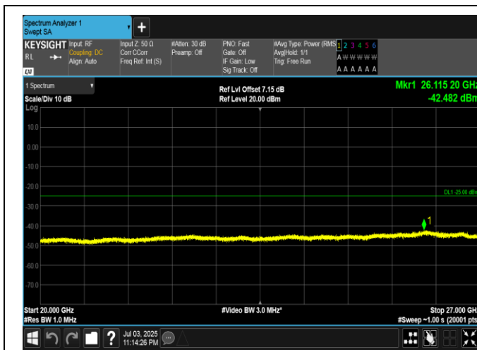
Band7-5MHz-QPSK-20775-25RB#0-20000~27000-PASS
