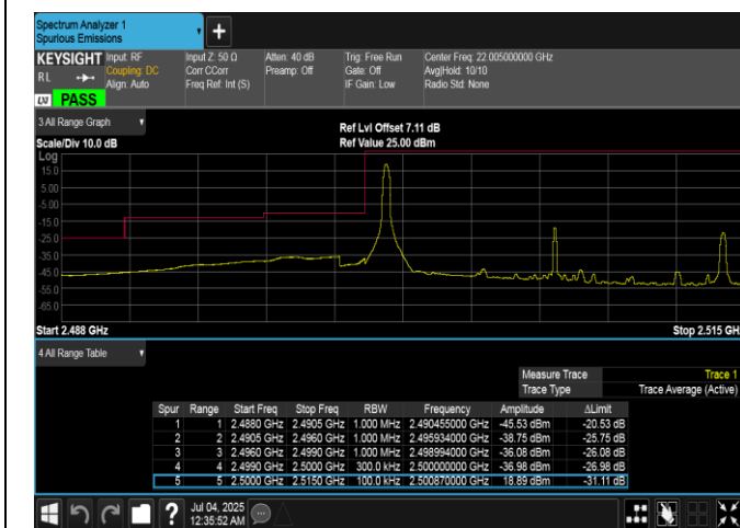
Band7-15MHz-QPSK-20825-1RB#0-PASS
