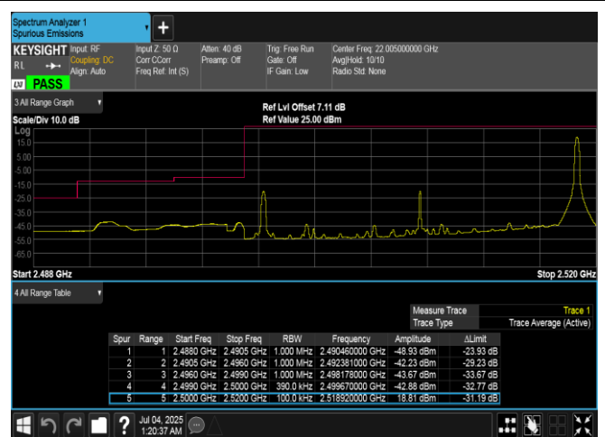
Band7-20MHz-16QAM-20850-1RB#99-PASS
