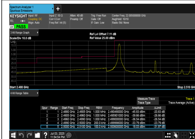
Band7-10MHz-16QAM-20800-1RB#0-PASS
