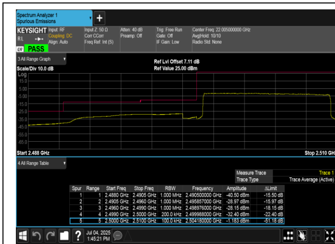
Band7-10MHz-QPSK-20800-50RB#0-PASS
