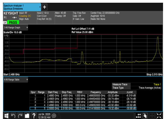
Band7-15MHz-QPSK-20825-1RB#74-PASS
