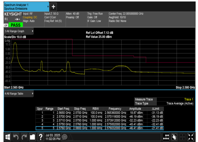
Band7-5MHz-16QAM-21425-1RB#0-PASS
