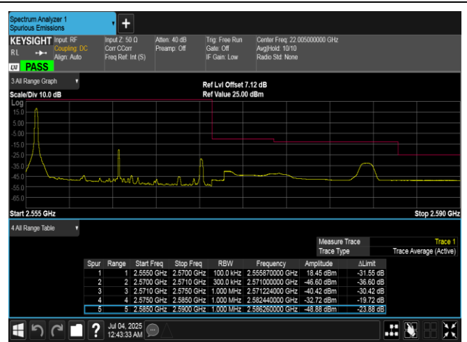
Band7-15MHz-QPSK-21375-1RB#0-PASS
