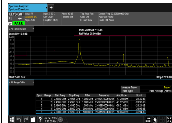
Band7-20MHz-16QAM-20850-1RB#0-PASS
