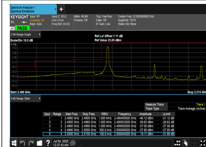
Band7-15MHz-16QAM-20825-1RB#0-PASS
