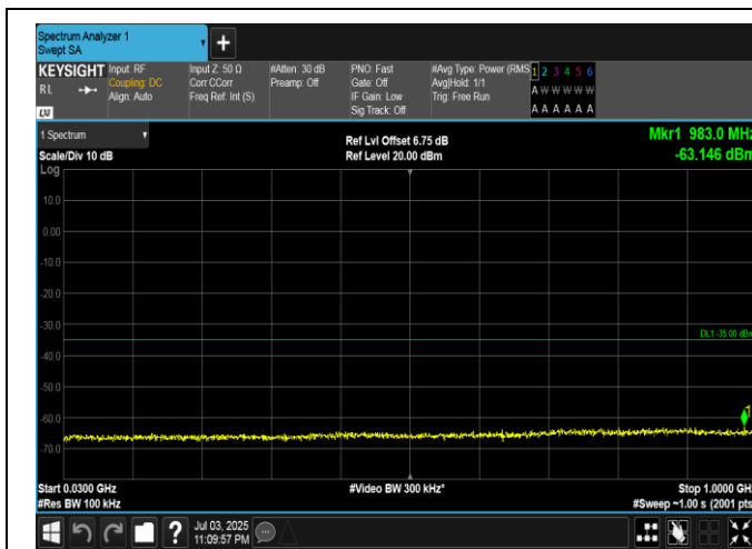
Band7-5MHz-QPSK-20775-1RB#0-30~1000-PASS
