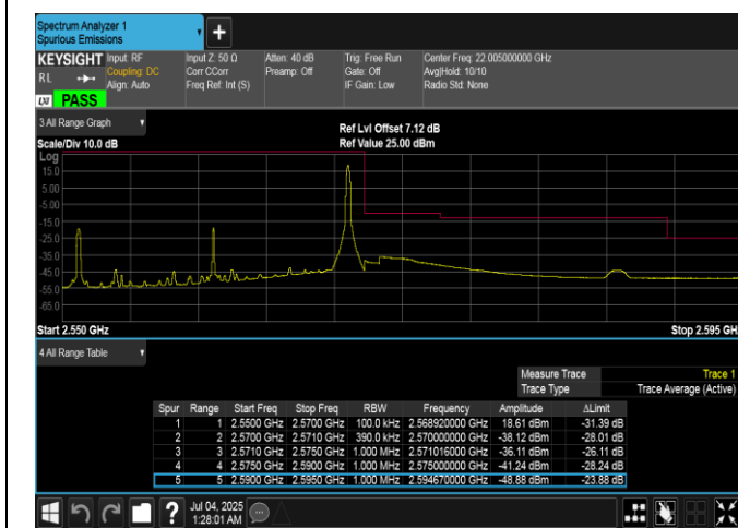
Band7-20MHz-16QAM-21350-1RB#99-PASS
