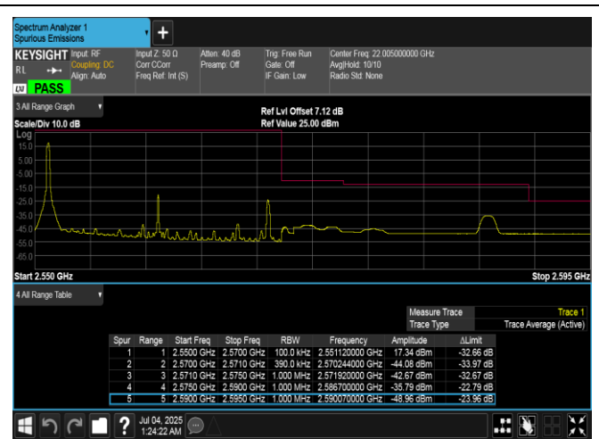
Band7-20MHz-16QAM-21350-1RB#0-PASS
