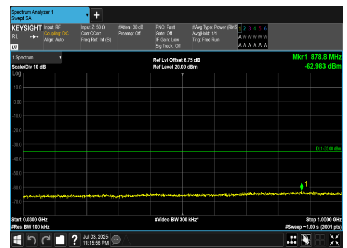
Band7-5MHz-QPSK-21100-1RB#0-30~1000-PASS
