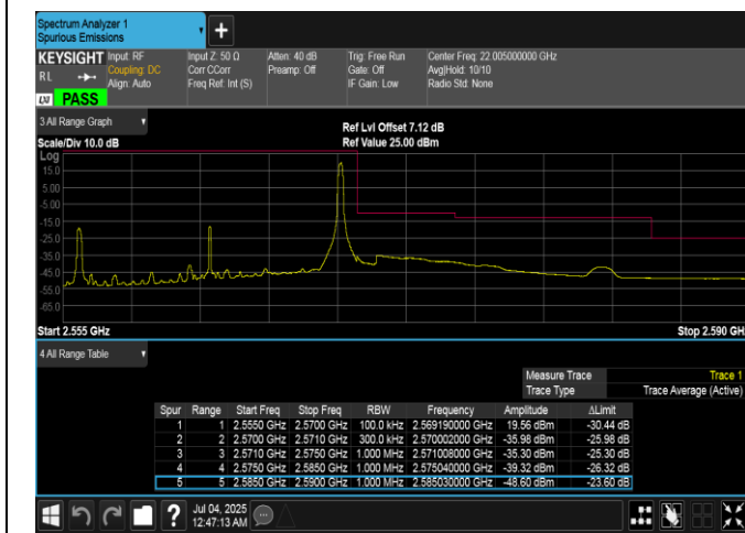
Band7-15MHz-QPSK-21375-1RB#74-PASS
