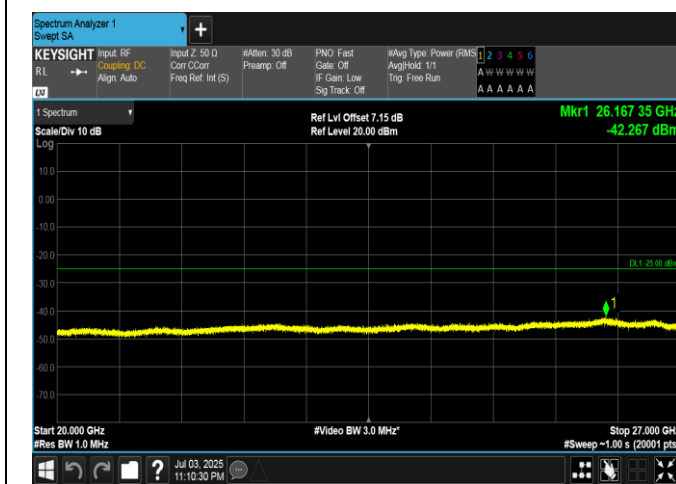
Band7-5MHz-QPSK-20775-1RB#0-20000~27000-PASS
