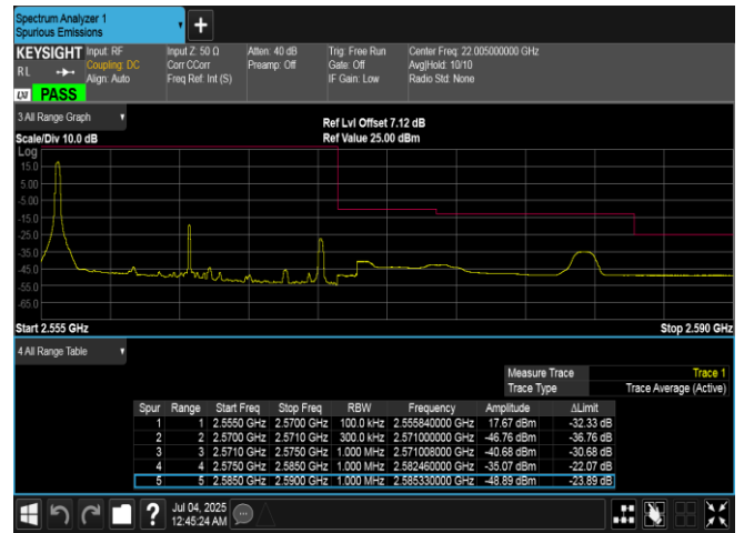
Band7-15MHz-16QAM-21375-1RB#0-PASS
