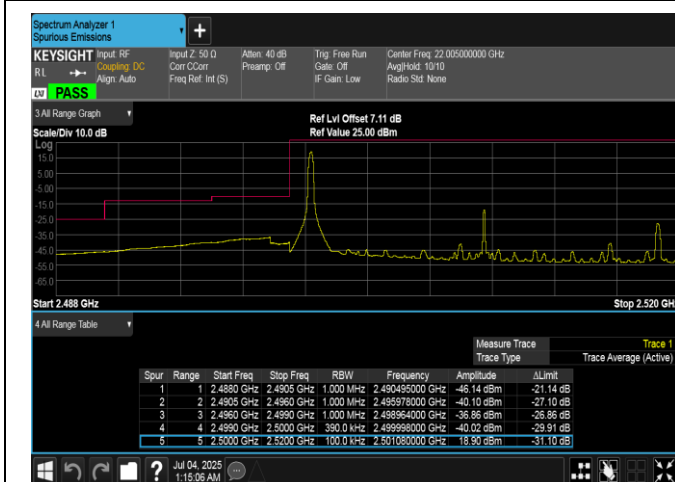
Band7-20MHz-QPSK-20850-1RB#0-PASS
