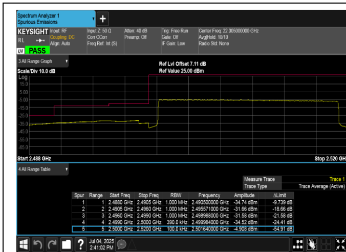
Band7-20MHz-16QAM-20850-100RB#0-PASS
