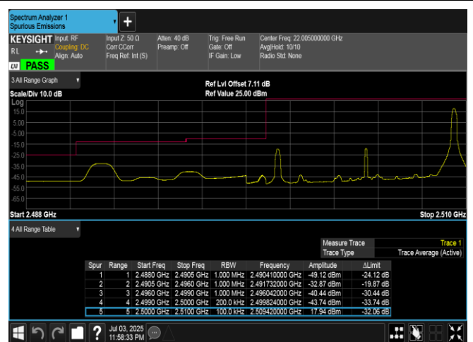
Band7-10MHz-16QAM-20800-1RB#49-PASS
