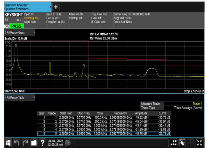
Band7-10MHz-QPSK-21400-1RB#0-PASS
