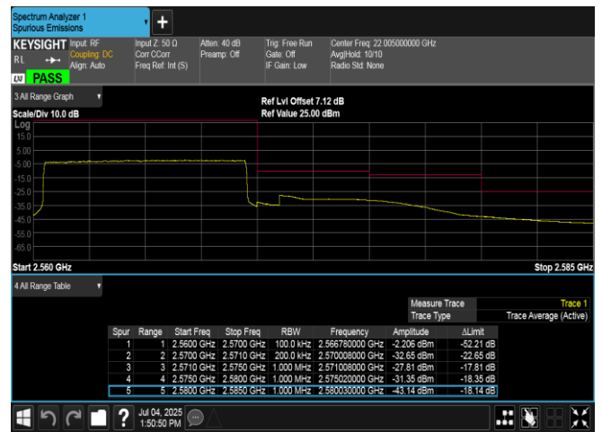
Band7-10MHz-16QAM-21400-50RB#0-PASS
