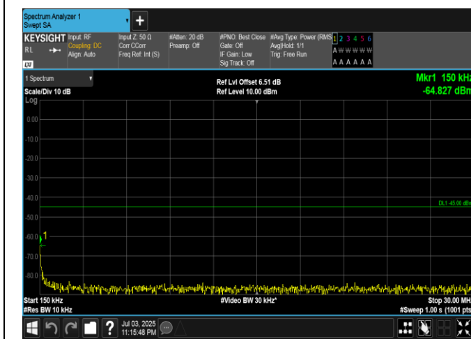
Band7-5MHz-QPSK-21100-1RB#0-0.15~30-PASS
