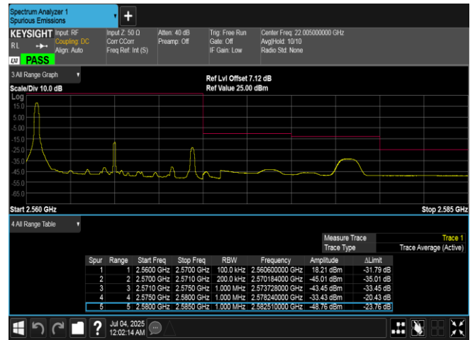
Band7-10MHz-16QAM-21400-1RB#0-PASS
