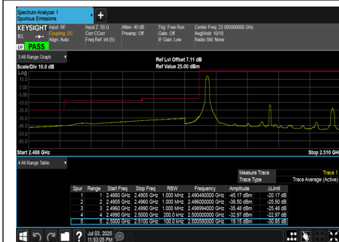
Band7-10MHz-QPSK-20800-1RB#0-PASS
