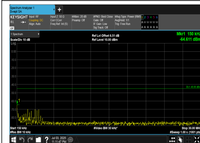
Band7-5MHz-QPSK-20775-1RB#24-0.15~30-PASS
