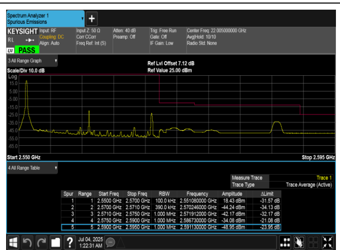
Band7-20MHz-QPSK-21350-1RB#0-PASS
