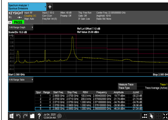
Band7-10MHz-QPSK-21400-1RB#49-PASS
