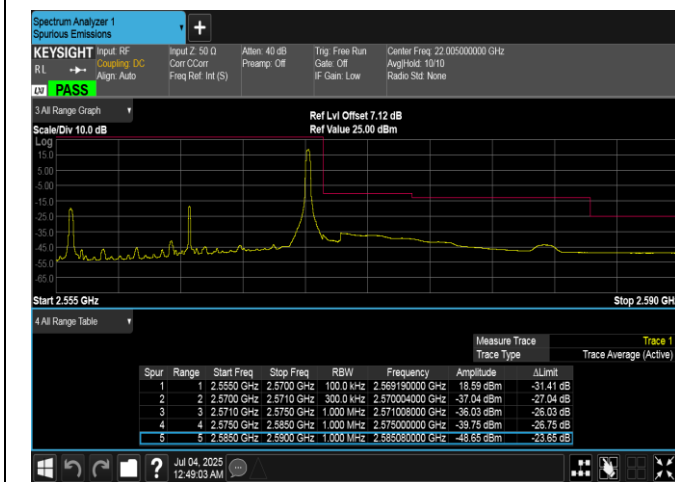
Band7-15MHz-16QAM-21375-1RB#74-PASS
