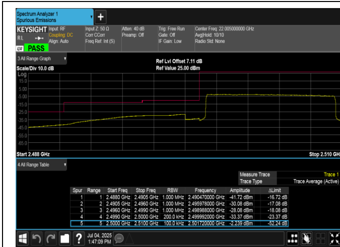
Band7-10MHz-16QAM-20800-50RB#0-PASS
