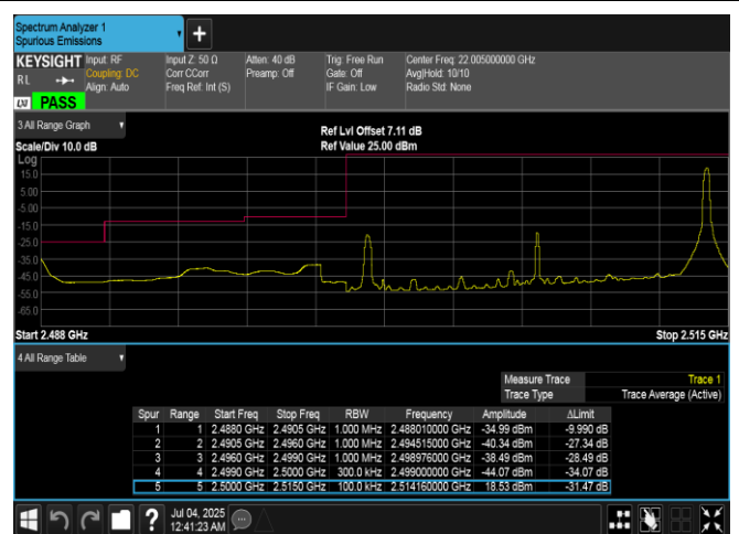
Band7-15MHz-16QAM-20825-1RB#74-PASS
