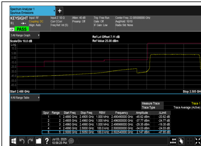
Band7-5MHz-16QAM-20775-25RB#0-PASS
