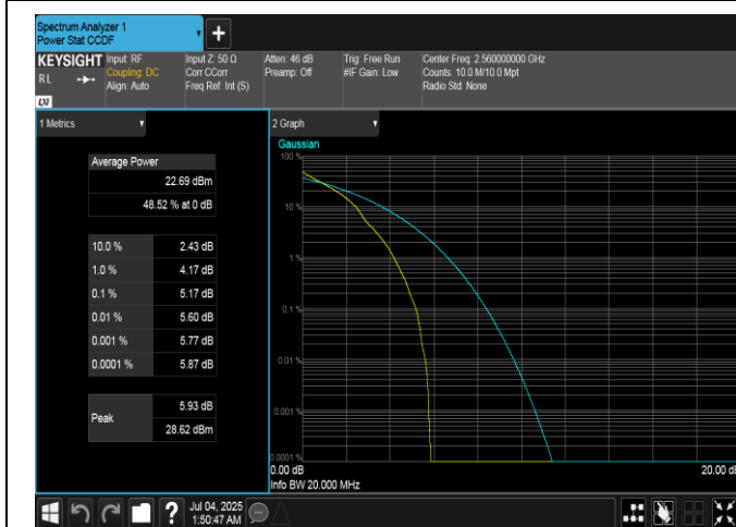
Band7-20MHz-QPSK-21350-1RB#0-PASS
