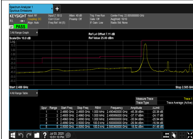
Band7-5MHz-16QAM-20775-1RB#0-PASS
