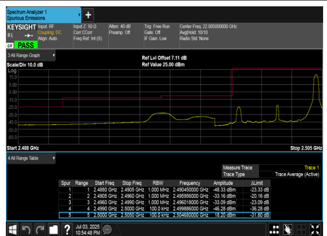
Band7-5MHz-16QAM-20775-1RB#24-PASS
