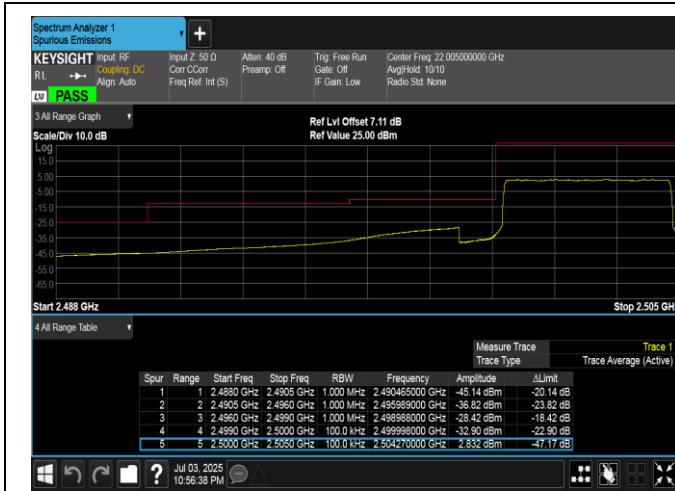
Band7-5MHz-QPSK-20775-25RB#0-PASS
