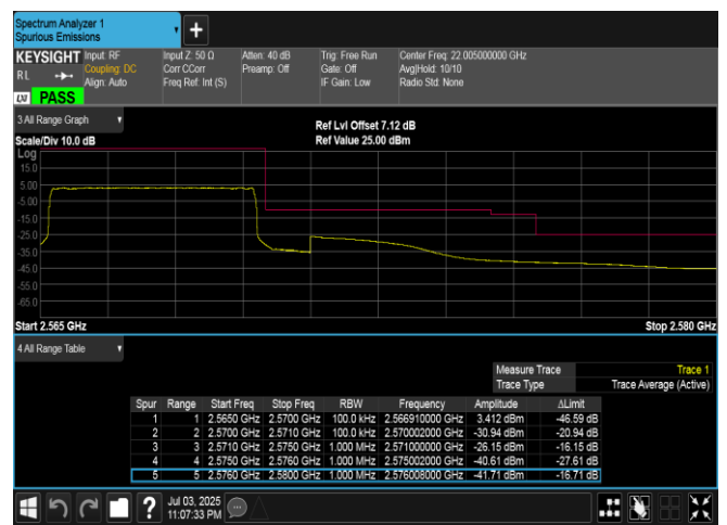
Band7-5MHz-QPSK-21425-25RB#0-PASS
