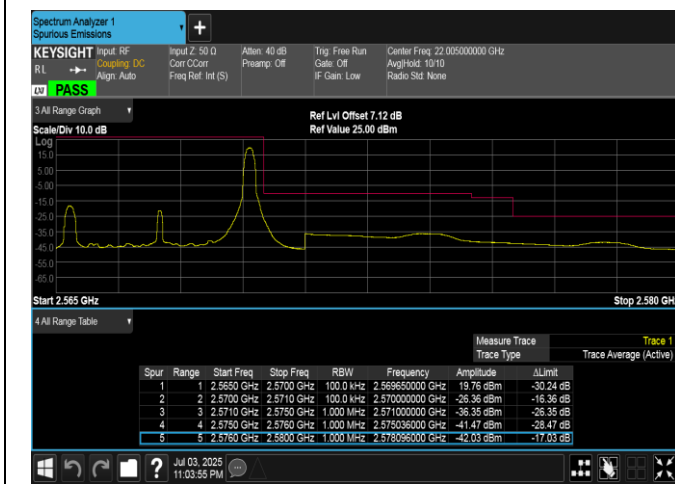
Band7-5MHz-QPSK-21425-1RB#24-PASS
