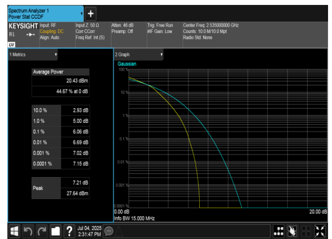
Band7-15MHz-16QAM-21100-75RB#0-PASS
