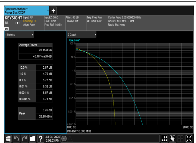
Band7-10MHz-16QAM-20800-50RB#0-PASS
