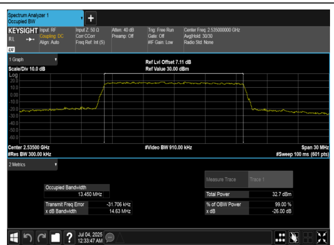
Band7-15MHz-QPSK-21100-75RB#0-PASS
