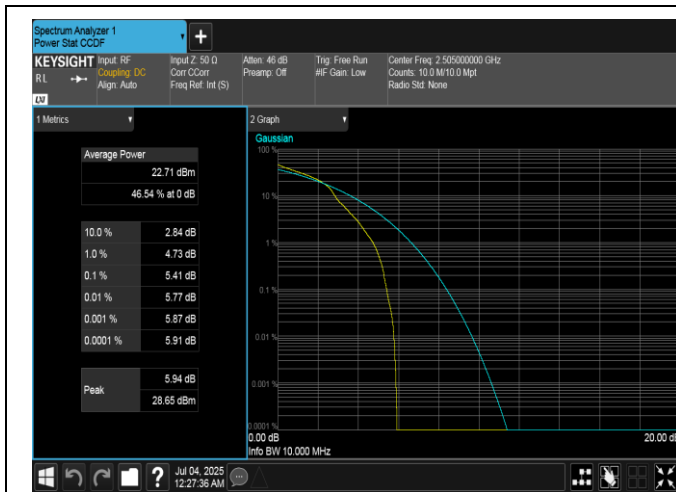
Band7-10MHz-16QAM-20800-1RB#0-PASS
