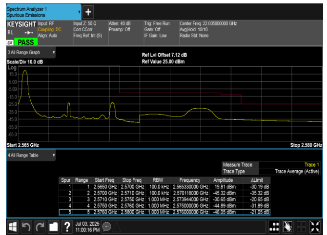
Band7-5MHz-QPSK-21425-1RB#0-PASS
