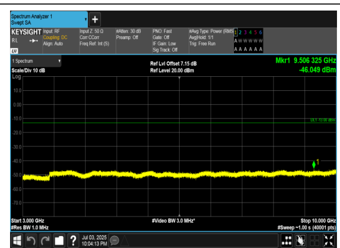
Band5-5MHz-16QAM-20525-1RB#24-3000~10000-PASS
