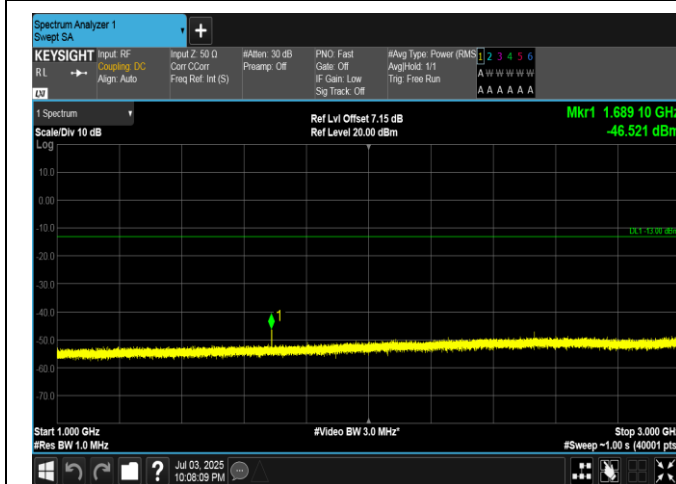
Band5-5MHz-16QAM-20625-1RB#0-1000~3000-PASS
