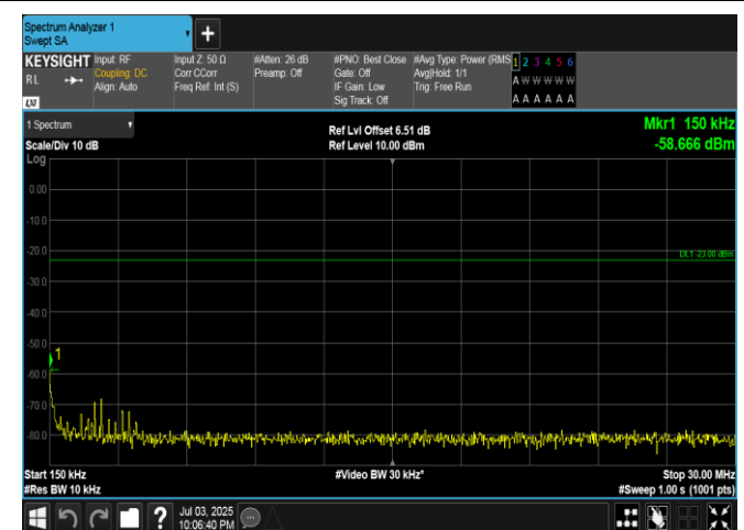
Band5-5MHz-QPSK-20625-1RB#0-0.15~30-PASS
