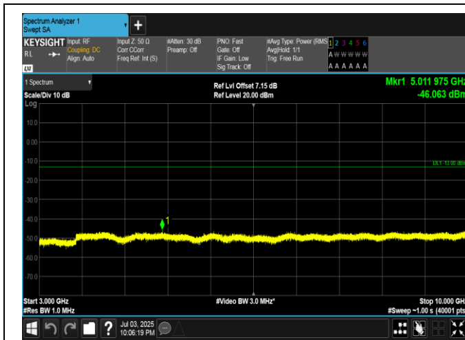
Band5-5MHz-16QAM-20525-25RB#0-3000~10000-PASS
