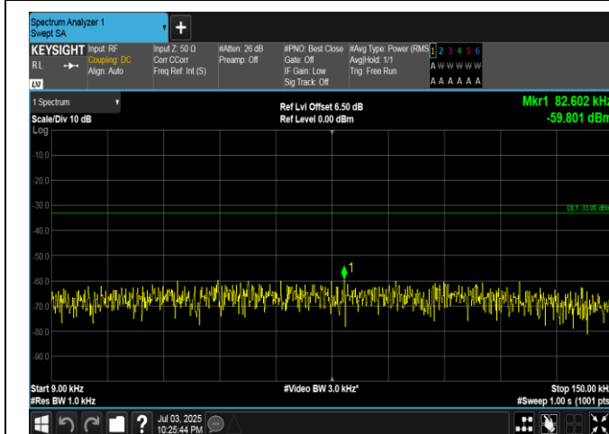
Band5-10MHz-QPSK-20450-1RB#0-0.009~0.15-PASS
