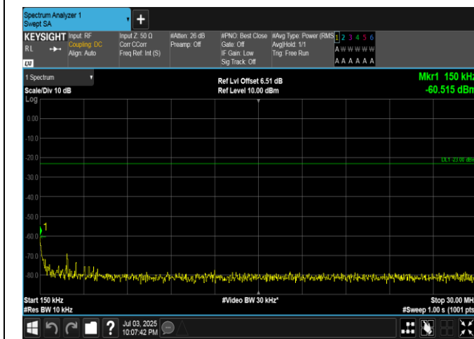
Band5-5MHz-16QAM-20625-1RB#0-0.15~30-PASS
