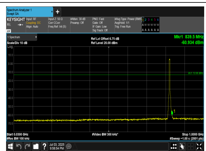
Band5-5MHz-16QAM-20425-25RB#0-30~1000-PASS
