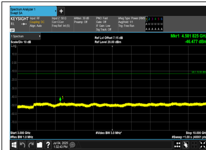
Band5-10MHz-QPSK-20450-50RB#0-3000~10000-PASS
