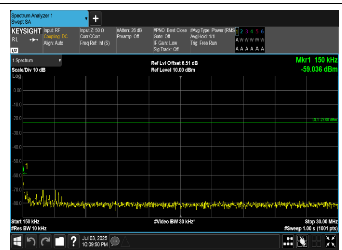
Band5-5MHz-16QAM-20625-1RB#24-0.15~30-PASS
