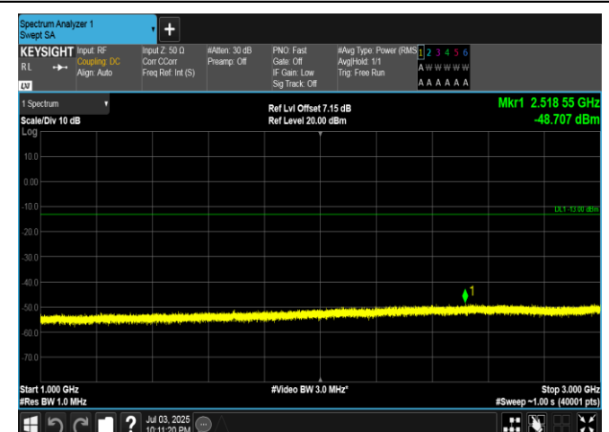
Band5-5MHz-QPSK-20625-25RB#0-1000~3000-PASS
