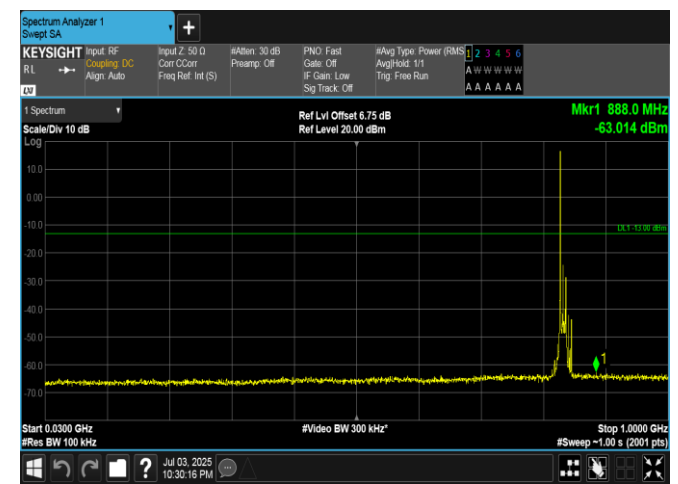
Band5-10MHz-QPSK-20525-1RB#0-30~1000-PASS
