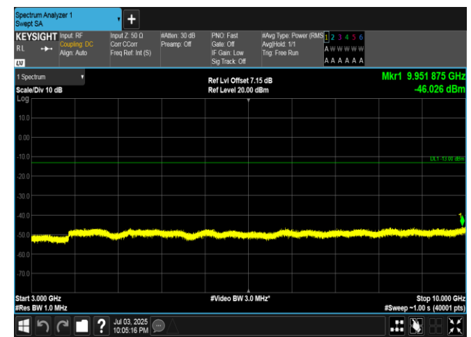
Band5-5MHz-QPSK-20525-25RB#0-3000~10000-PASS
