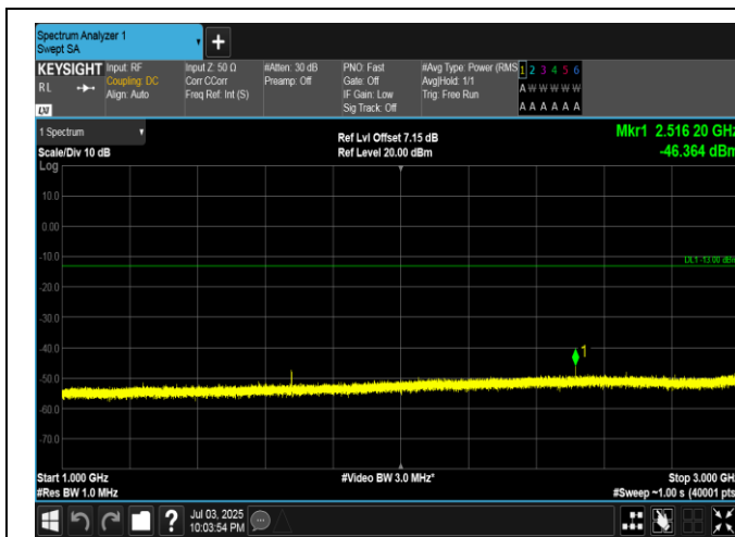
Band5-5MHz-16QAM-20525-1RB#24-1000~3000-PASS
