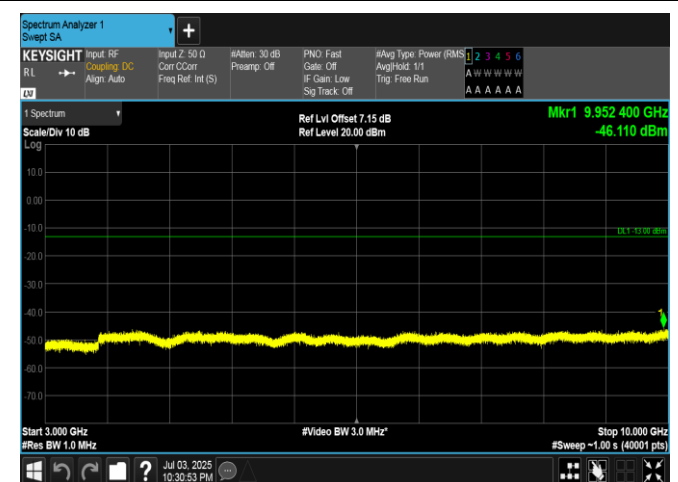
Band5-10MHz-QPSK-20525-1RB#0-3000~10000-PASS
