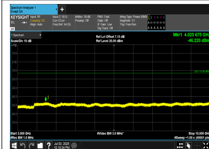
Band5-5MHz-16QAM-20625-1RB#24-3000~10000-PASS
