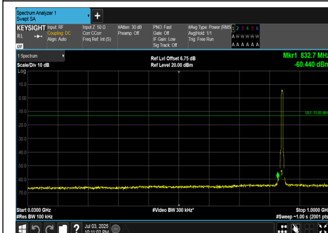
Band5-5MHz-QPSK-20625-25RB#0-30~1000-PASS
