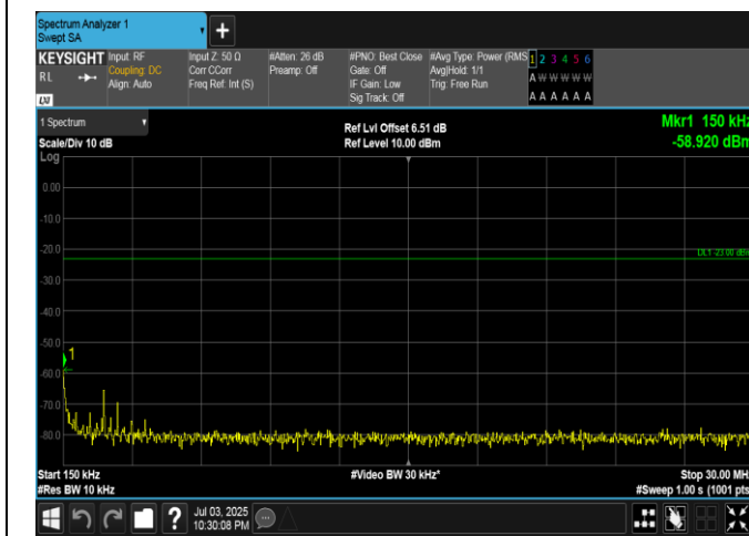
Band5-10MHz-QPSK-20525-1RB#0-0.15~30-PASS
