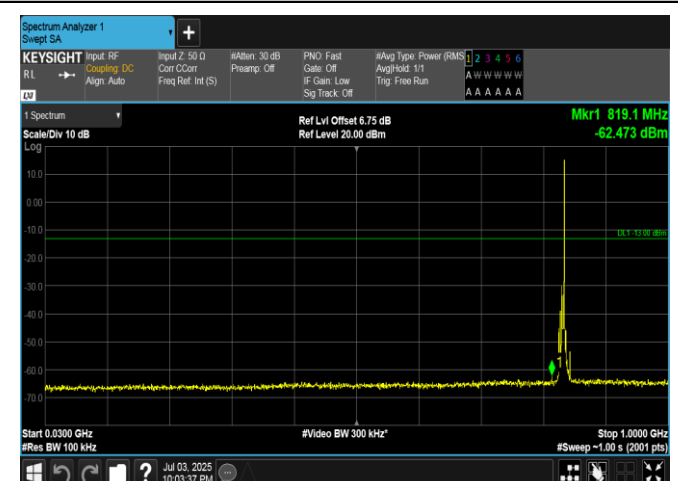
Band5-5MHz-16QAM-20525-1RB#24-30~1000-PASS
