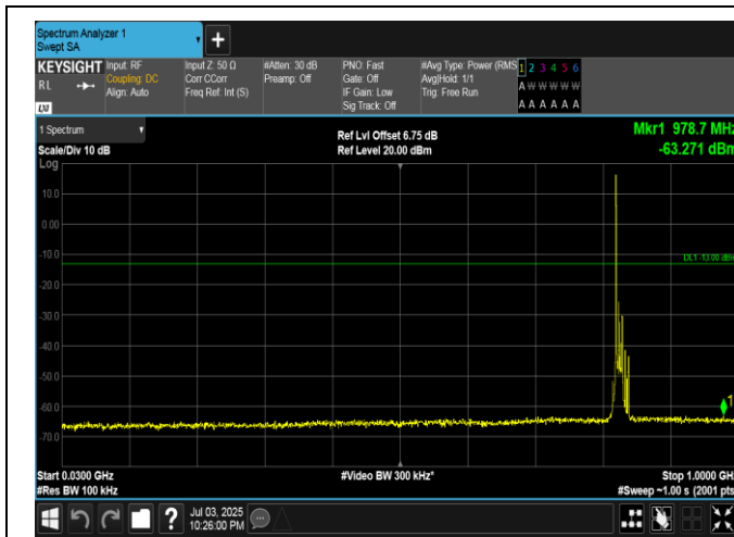
Band5-10MHz-QPSK-20450-1RB#0-30~1000-PASS
