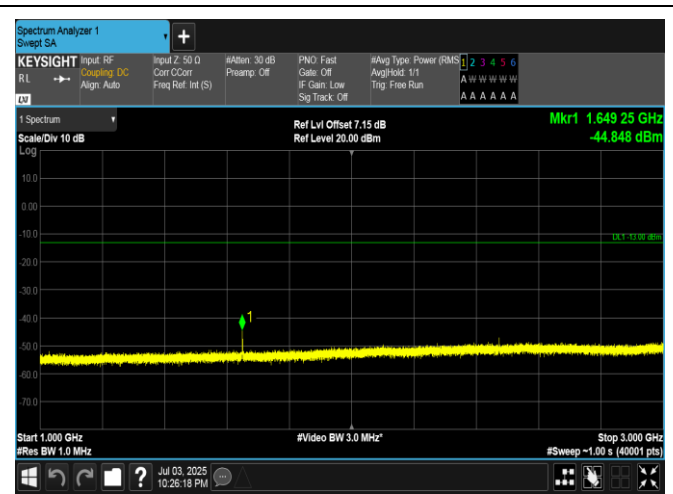
Band5-10MHz-QPSK-20450-1RB#0-1000~3000-PASS
