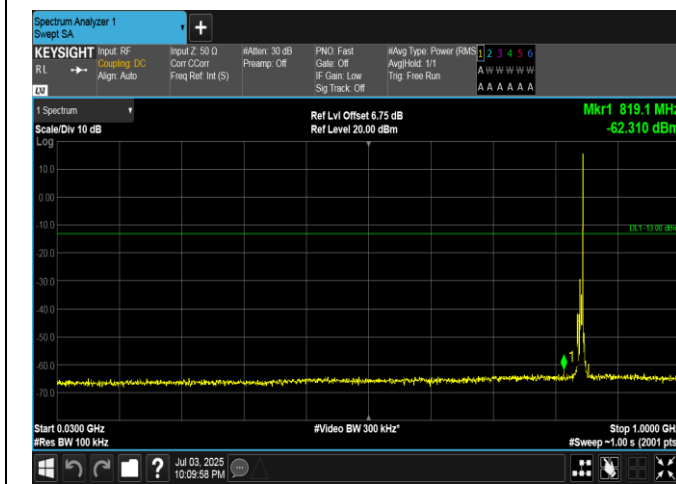
Band5-5MHz-16QAM-20625-1RB#24-30~1000-PASS
