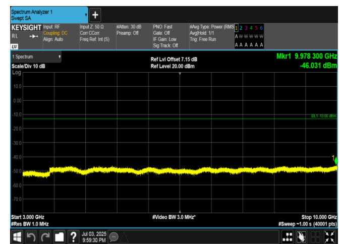
Band5-5MHz-16QAM-20425-25RB#0-3000~10000-PASS
