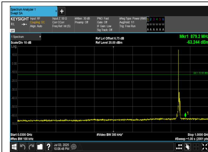
Band5-5MHz-QPSK-20625-1RB#0-30~1000-PASS
