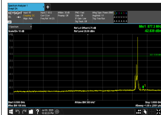
Band5-10MHz-QPSK-20525-1RB#49-30~1000-PASS
