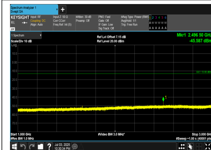
Band5-10MHz-QPSK-20525-1RB#0-1000~3000-PASS
