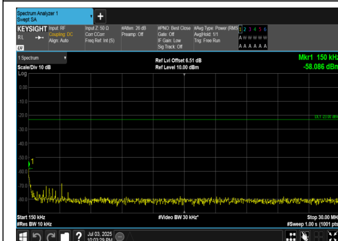
Band5-5MHz-16QAM-20525-1RB#24-0.15~30-PASS
