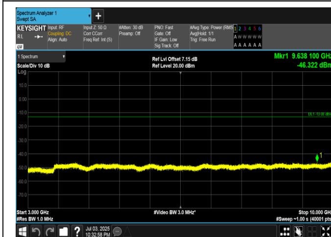
Band5-10MHz-QPSK-20525-1RB#49-3000~10000-PASS
