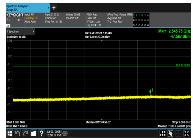
Band5-5MHz-16QAM-20625-1RB#24-1000~3000-PASS
