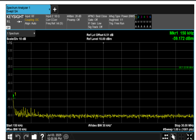
Band5-5MHz-16QAM-20525-1RB#0-0.15~30-PASS
