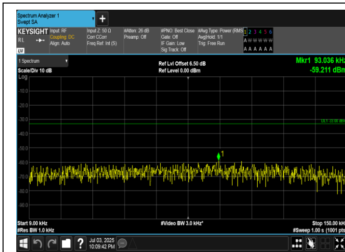
Band5-5MHz-16QAM-20625-1RB#24-0.009~0.15-PASS
