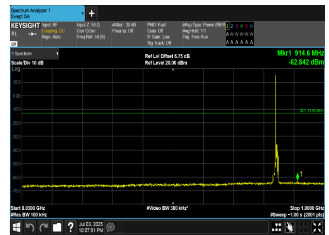
Band5-5MHz-16QAM-20625-1RB#0-30~1000-PASS
