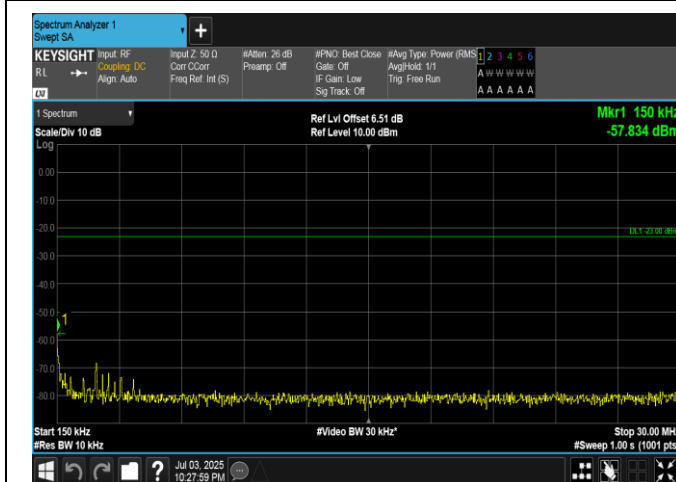
Band5-10MHz-QPSK-20450-1RB#49-0.15~30-PASS
