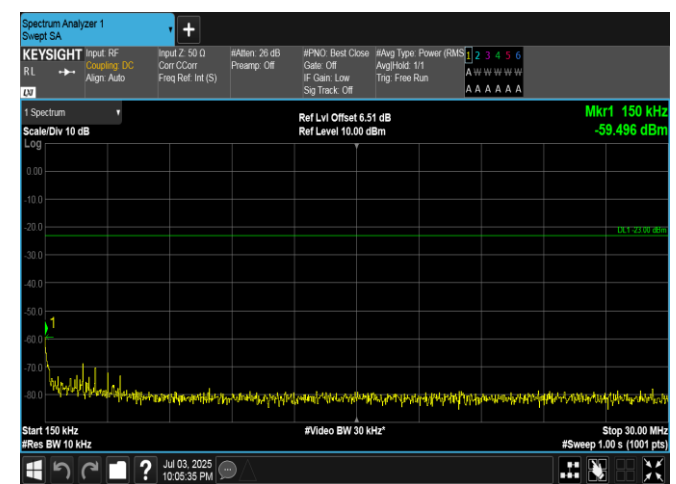
Band5-5MHz-16QAM-20525-25RB#0-0.15~30-PASS
