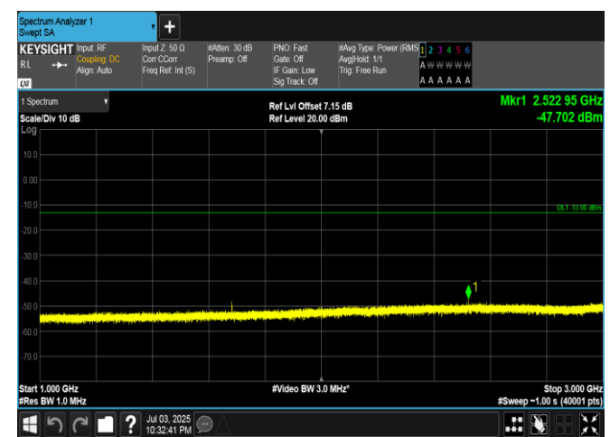
Band5-10MHz-QPSK-20525-1RB#49-1000~3000-PASS
