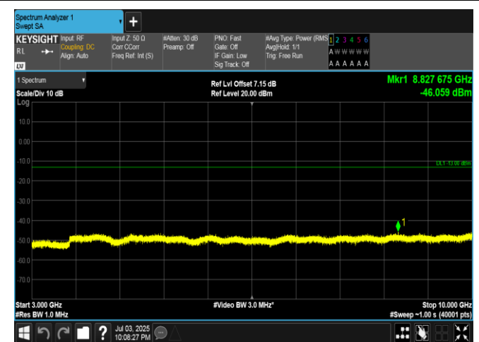
Band5-5MHz-16QAM-20625-1RB#0-3000~10000-PASS
