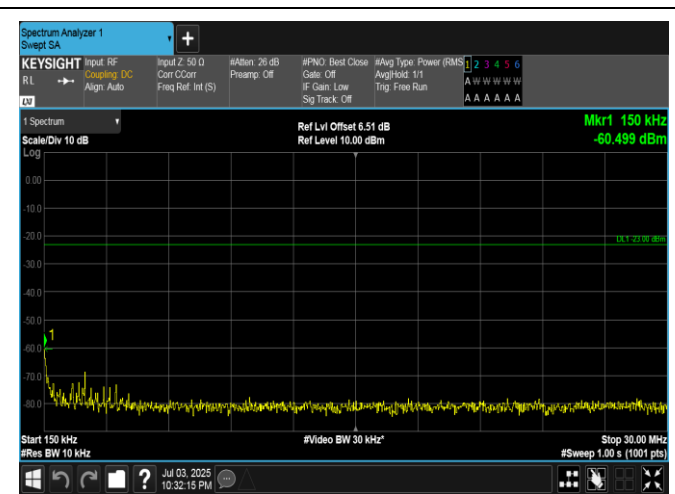
Band5-10MHz-QPSK-20525-1RB#49-0.15~30-PASS
