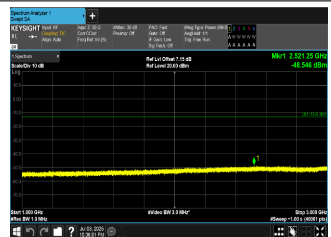
Band5-5MHz-16QAM-20525-25RB#0-1000~3000-PASS
