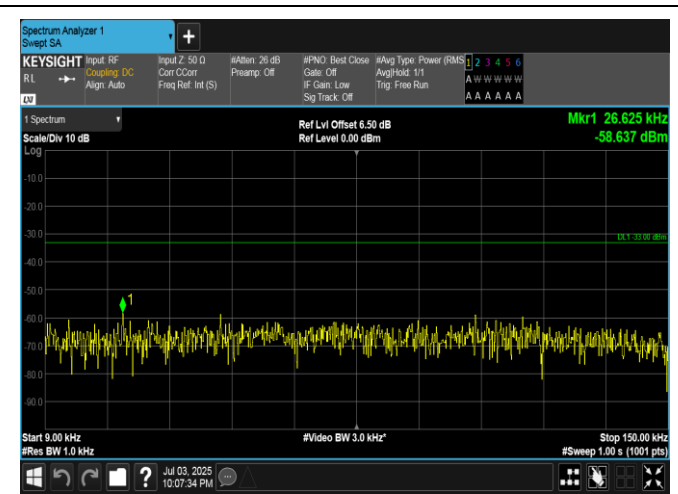
Band5-5MHz-16QAM-20625-1RB#0-0.009~0.15-PASS
