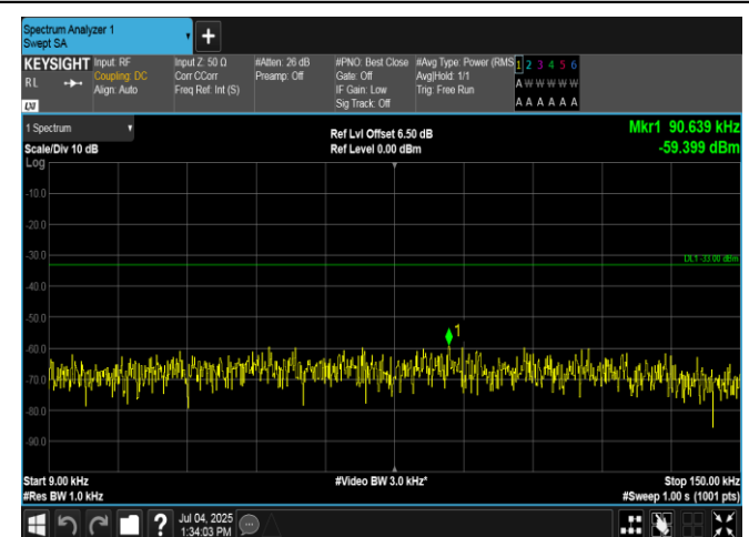
Band5-10MHz-QPSK-20525-50RB#0-0.009~0.15-PASS
