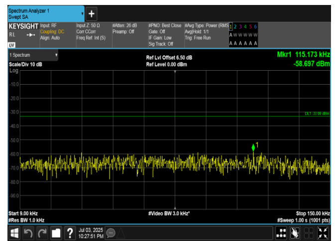
Band5-10MHz-QPSK-20450-1RB#49-0.009~0.15-PASS
