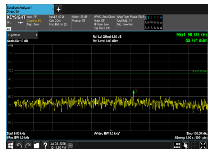
Band5-5MHz-16QAM-20625-25RB#0-0.009~0.15-PASS
