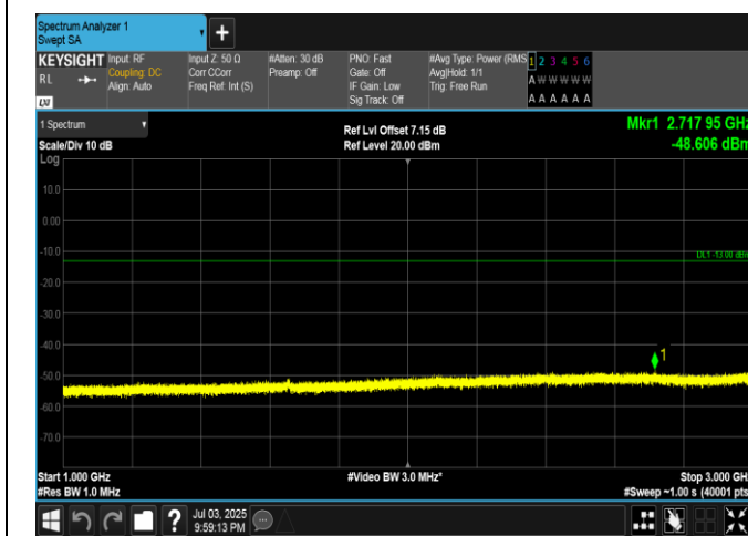
Band5-5MHz-16QAM-20425-25RB#0-1000~3000-PASS
