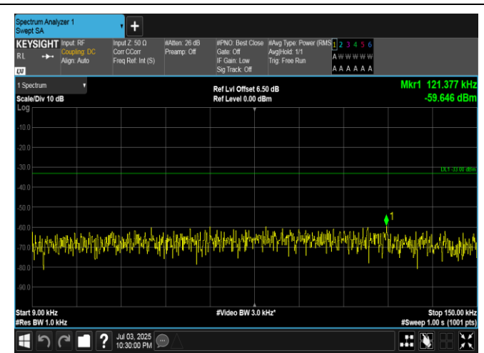
Band5-10MHz-QPSK-20525-1RB#0-0.009~0.15-PASS
