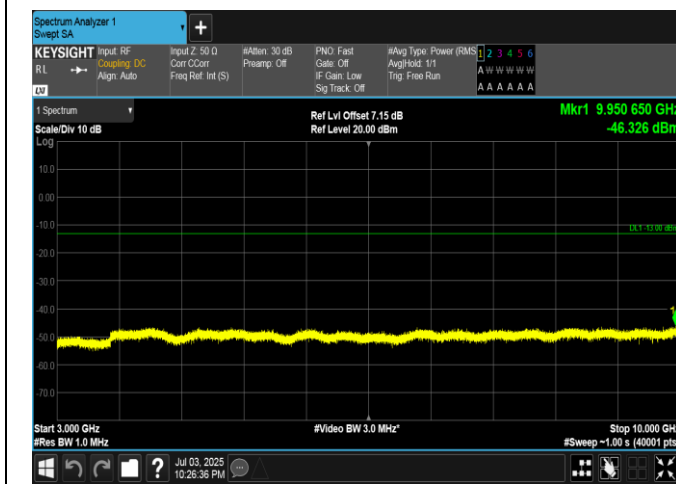
Band5-10MHz-QPSK-20450-1RB#0-3000~10000-PASS
