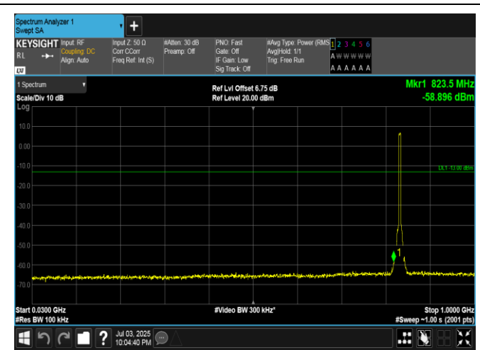
Band5-5MHz-QPSK-20525-25RB#0-30~1000-PASS
