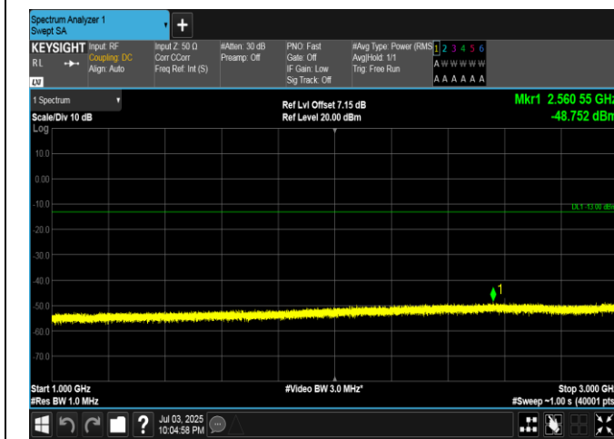
Band5-5MHz-QPSK-20525-25RB#0-1000~3000-PASS
