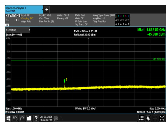
Band5-3MHz-QPSK-20635-1RB#0-1000~3000-PASS
