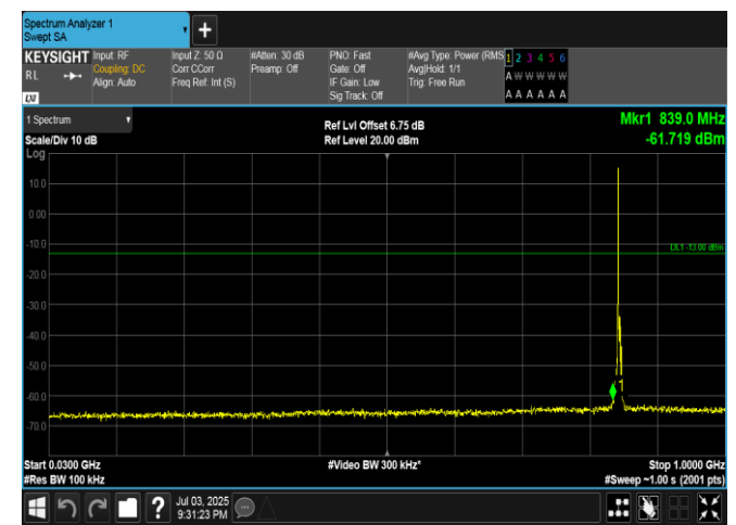
Band5-3MHz-16QAM-20635-1RB#0-30~1000-PASS
