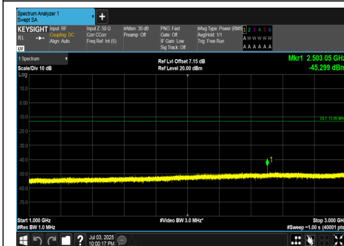
Band5-5MHz-QPSK-20525-1RB#0-1000~3000-PASS
