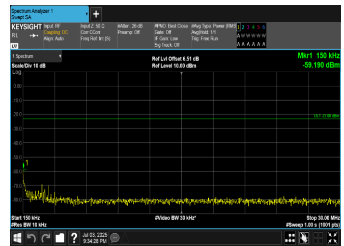
Band5-3MHz-QPSK-20635-15RB#0-0.15~30-PASS
