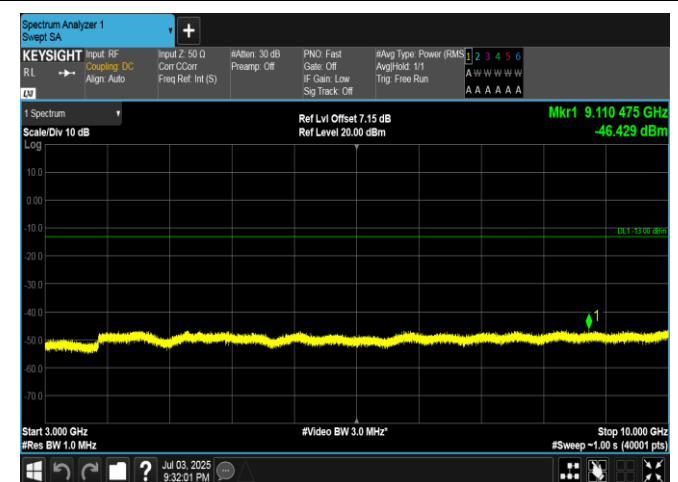
Band5-3MHz-16QAM-20635-1RB#0-3000~10000-PASS
