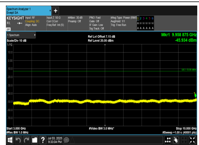
Band5-3MHz-QPSK-20635-1RB#14-3000~10000-PASS
