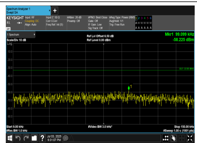
Band5-3MHz-16QAM-20635-1RB#0-0.009~0.15-PASS
