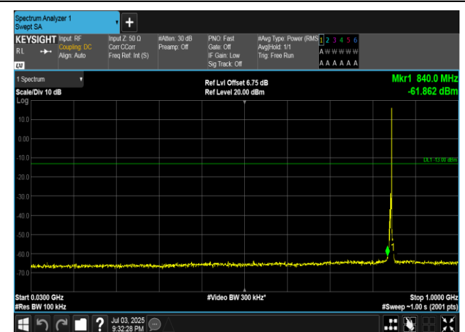
Band5-3MHz-QPSK-20635-1RB#14-30~1000-PASS
