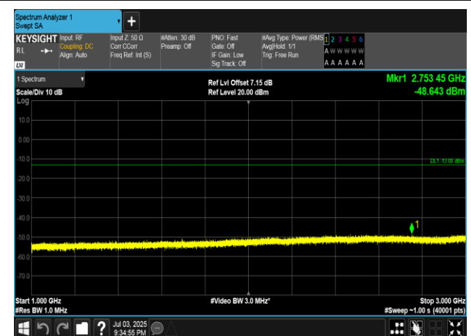
Band5-3MHz-QPSK-20635-15RB#0-1000~3000-PASS
