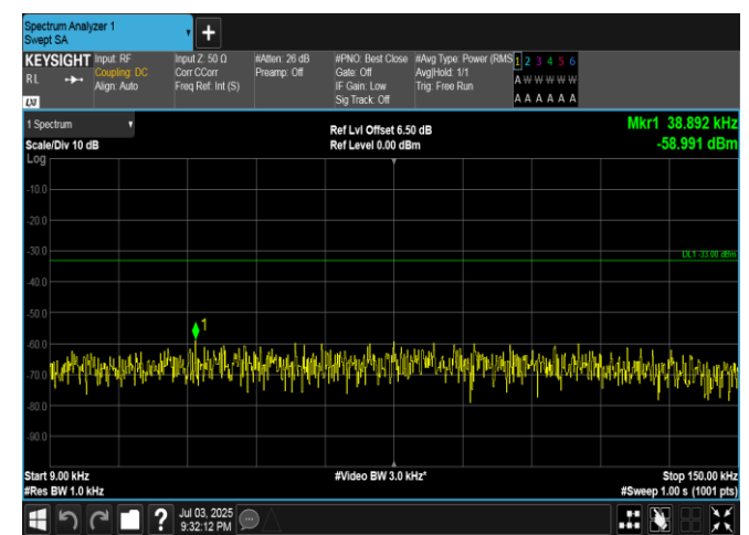
Band5-3MHz-QPSK-20635-1RB#14-0.009~0.15-PASS
