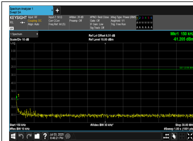
Band5-1.4MHz-16QAM-20407-6RB#0-0.15~30-PASS
