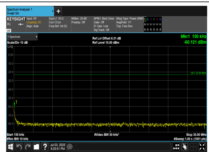
Band5-3MHz-QPSK-20525-1RB#14-0.15~30-PASS
