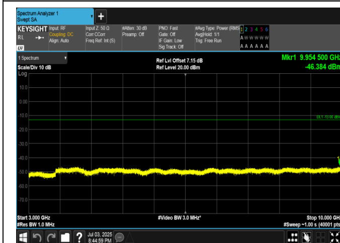
Band5-1.4MHz-16QAM-20407-1RB#5-3000~10000-PASS
