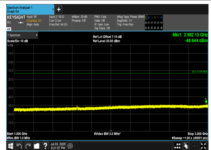
Band5-3MHz-QPSK-20415-15RB#0-1000~3000-PASS
