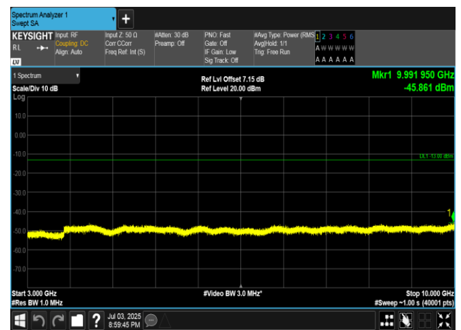
Band5-1.4MHz-16QAM-20643-6RB#0-3000~10000-PASS
