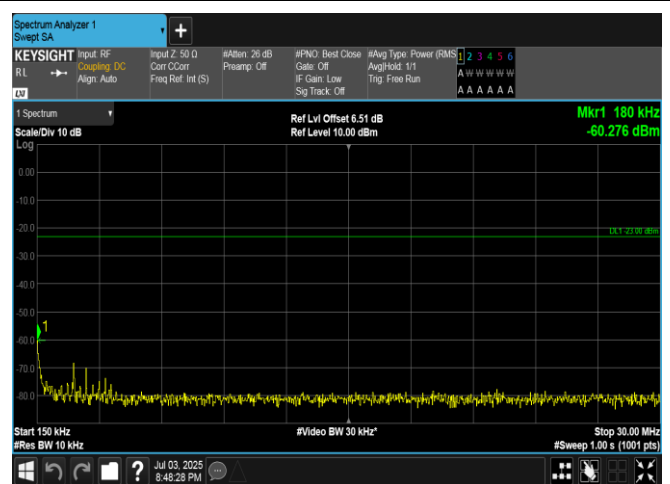
Band5-1.4MHz-16QAM-20525-1RB#0-0.15~30-PASS
