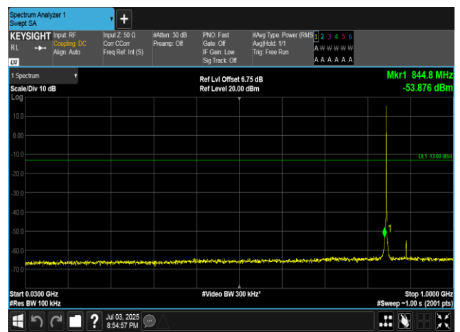
Band5-1.4MHz-16QAM-20643-1RB#0-30~1000-PASS
