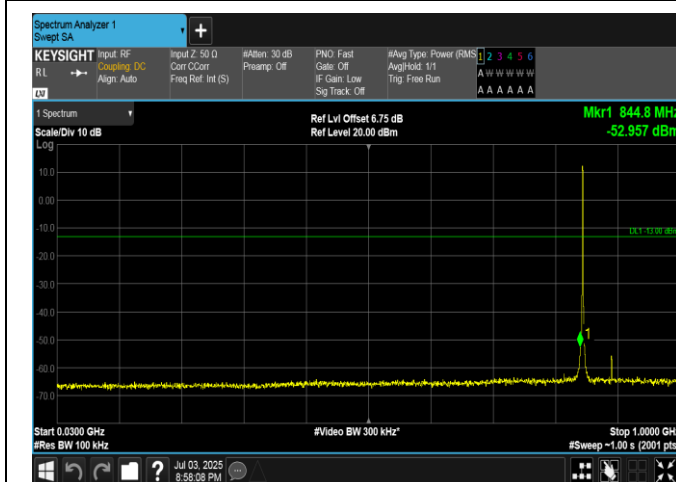
Band5-1.4MHz-QPSK-20643-6RB#0-30~1000-PASS
