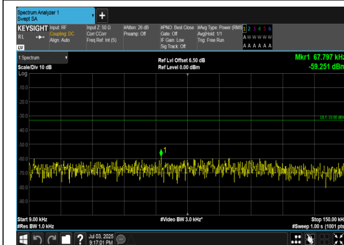
Band5-3MHz-QPSK-20415-1RB#0-0.009~0.15-PASS
