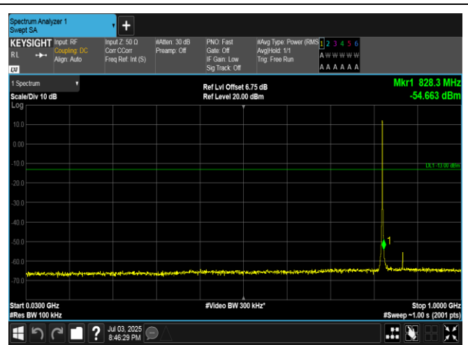
Band5-1.4MHz-16QAM-20407-6RB#0-30~1000-PASS
