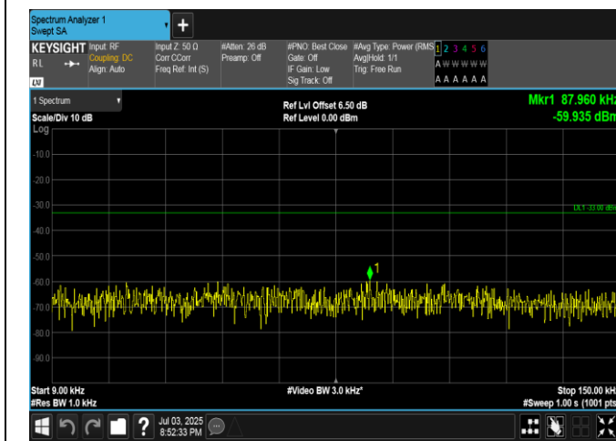
Band5-1.4MHz-16QAM-20525-6RB#0-0.009~0.15-PASS
