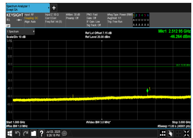
Band5-3MHz-QPSK-20525-1RB#14-1000~3000-PASS
