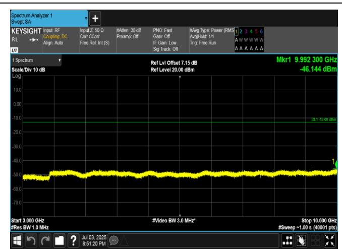
Band5-1.4MHz-16QAM-20525-1RB#5-3000~10000-PASS
