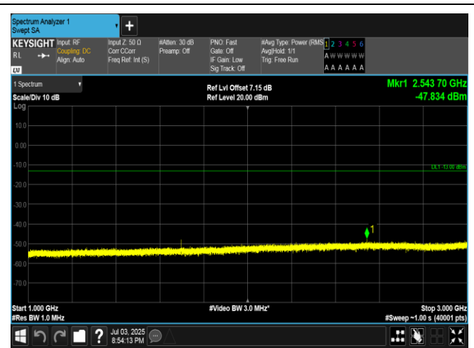
Band5-1.4MHz-QPSK-20643-1RB#0-1000~3000-PASS
