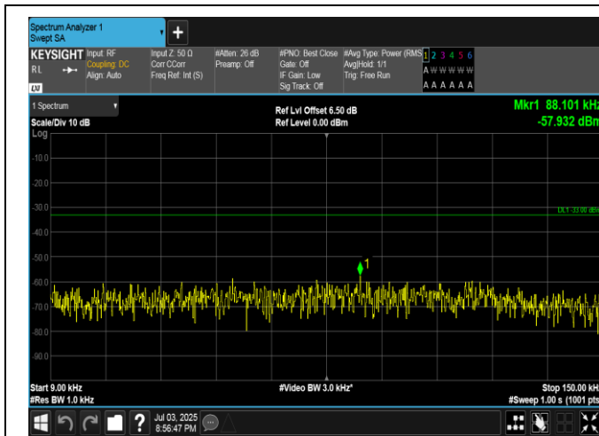
Band5-1.4MHz-16QAM-20643-1RB#5-0.009~0.15-PASS
