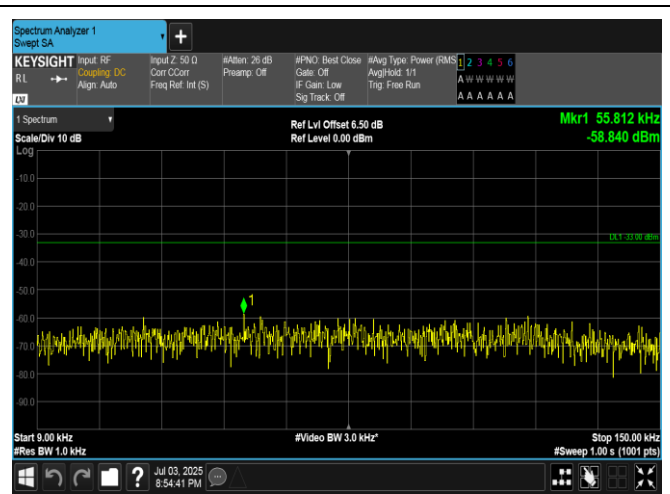
Band5-1.4MHz-16QAM-20643-1RB#0-0.009~0.15-PASS
