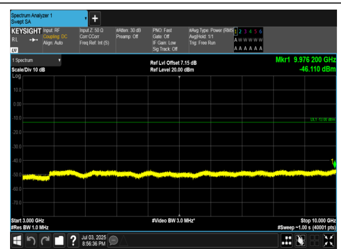
Band5-1.4MHz-QPSK-20643-1RB#5-3000~10000-PASS
