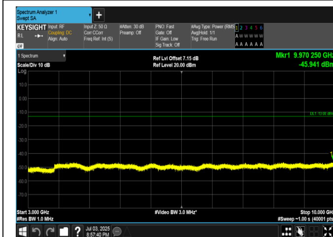
Band5-1.4MHz-16QAM-20643-1RB#5-3000~10000-PASS
