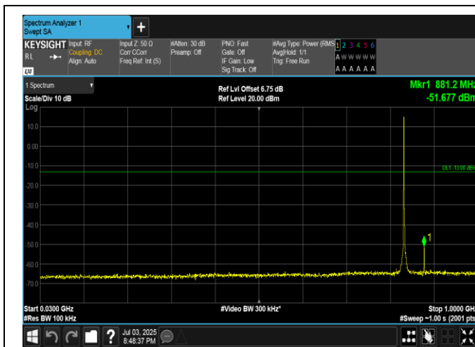
Band5-1.4MHz-16QAM-20525-1RB#0-30~1000-PASS
