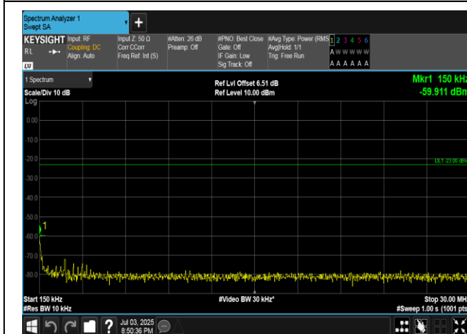
Band5-1.4MHz-16QAM-20525-1RB#5-0.15~30-PASS
