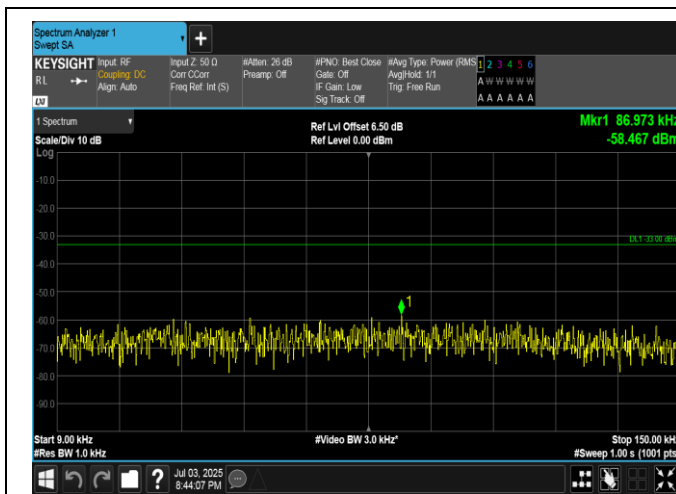
Band5-1.4MHz-16QAM-20407-1RB#5-0.009~0.15-PASS
