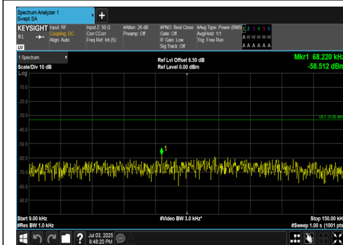
Band5-1.4MHz-16QAM-20525-1RB#0-0.009~0.15-PASS
