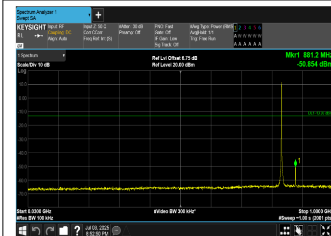
Band5-1.4MHz-16QAM-20525-6RB#0-30~1000-PASS
