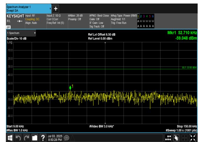
Band5-1.4MHz-16QAM-20525-1RB#5-0.009~0.15-PASS
