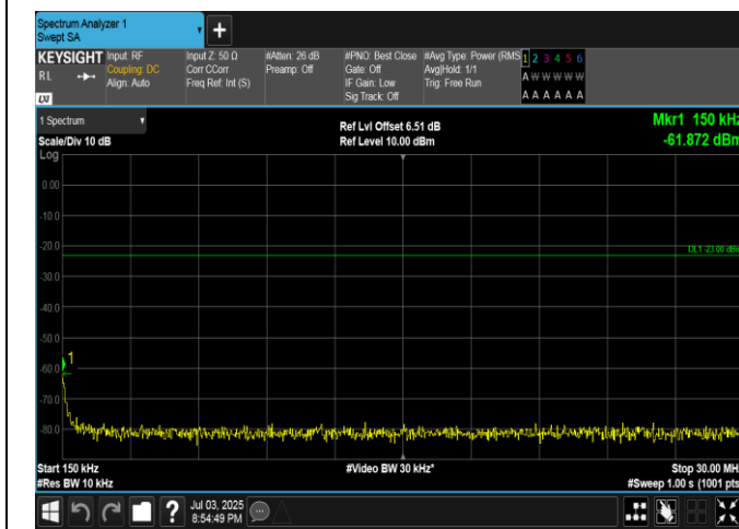
Band5-1.4MHz-16QAM-20643-1RB#0-0.15~30-PASS
