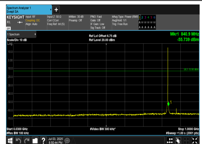
Band5-1.4MHz-16QAM-20525-1RB#5-30~1000-PASS
