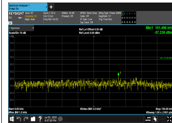
Band5-1.4MHz-QPSK-20643-6RB#0-0.009~0.15-PASS
