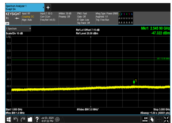
Band5-1.4MHz-16QAM-20643-1RB#5-1000~3000-PASS
