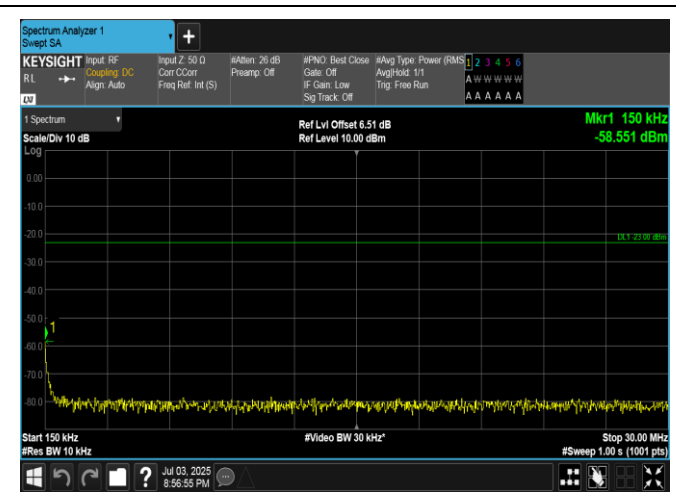
Band5-1.4MHz-16QAM-20643-1RB#5-0.15~30-PASS
