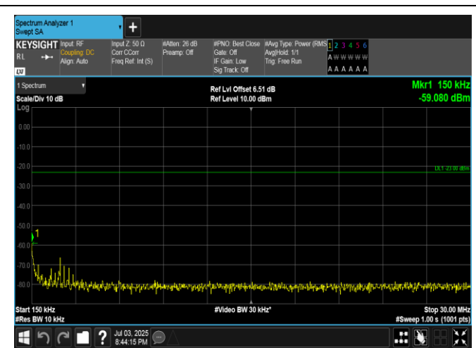
Band5-1.4MHz-16QAM-20407-1RB#5-0.15~30-PASS
