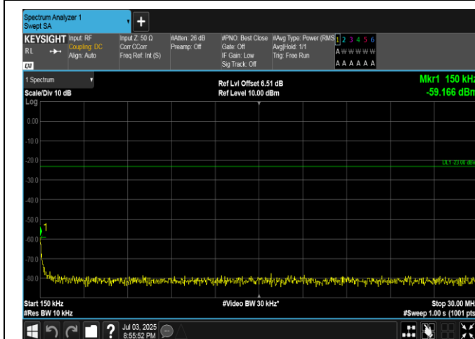
Band5-1.4MHz-QPSK-20643-1RB#5-0.15~30-PASS
