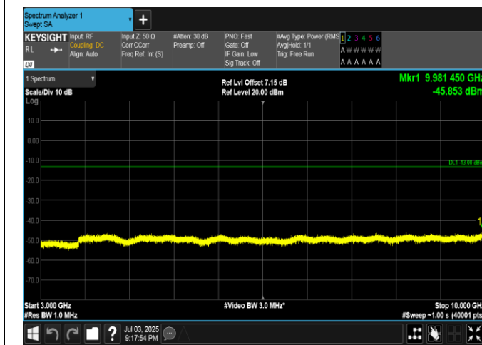
Band5-3MHz-QPSK-20415-1RB#0-3000~10000-PASS
