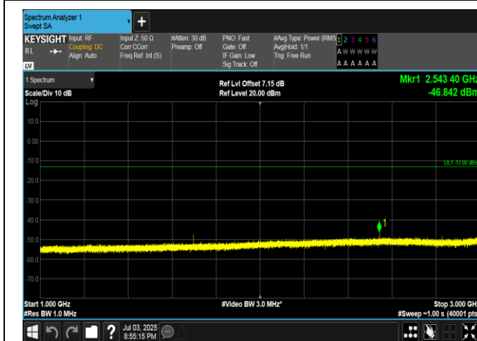
Band5-1.4MHz-16QAM-20643-1RB#0-1000~3000-PASS
