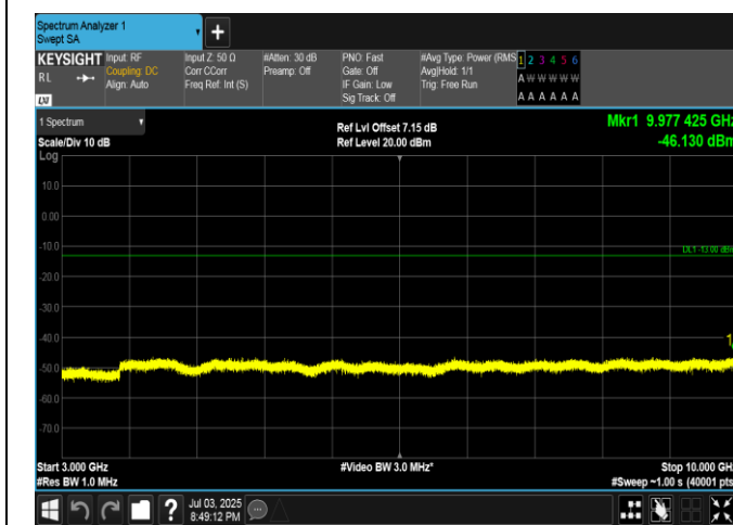
Band5-1.4MHz-16QAM-20525-1RB#0-3000~10000-PASS
