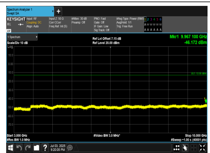
Band5-3MHz-QPSK-20415-1RB#14-3000~10000-PASS
