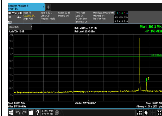
Band5-1.4MHz-16QAM-20643-1RB#5-30~1000-PASS
