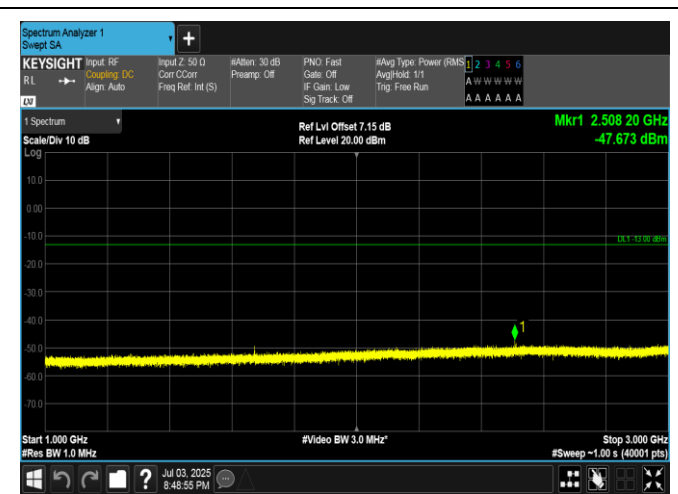
Band5-1.4MHz-16QAM-20525-1RB#0-1000~3000-PASS
