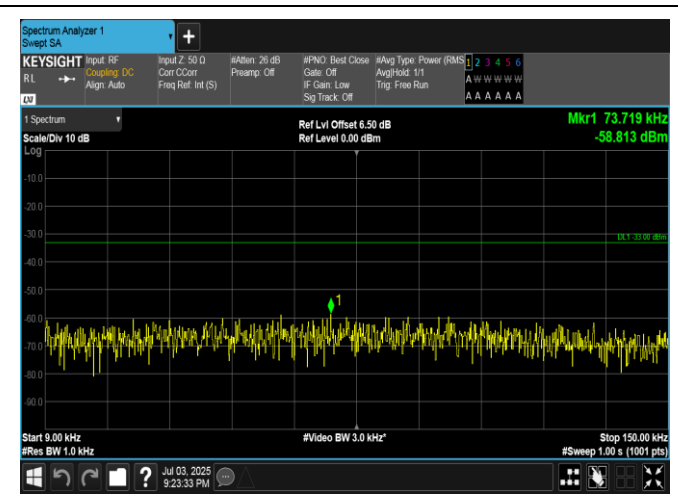
Band5-3MHz-QPSK-20525-1RB#0-0.009~0.15-PASS
