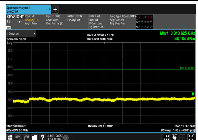
Band5-3MHz-QPSK-20525-1RB#0-3000~10000-PASS
