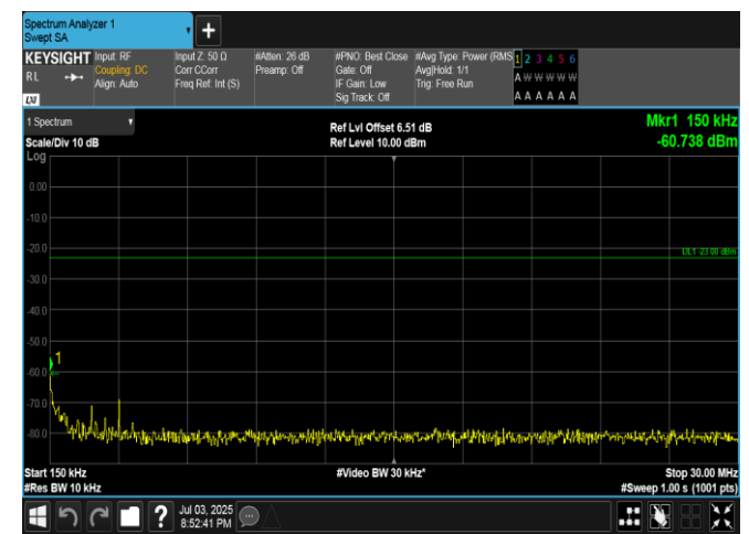
Band5-1.4MHz-16QAM-20525-6RB#0-0.15~30-PASS
