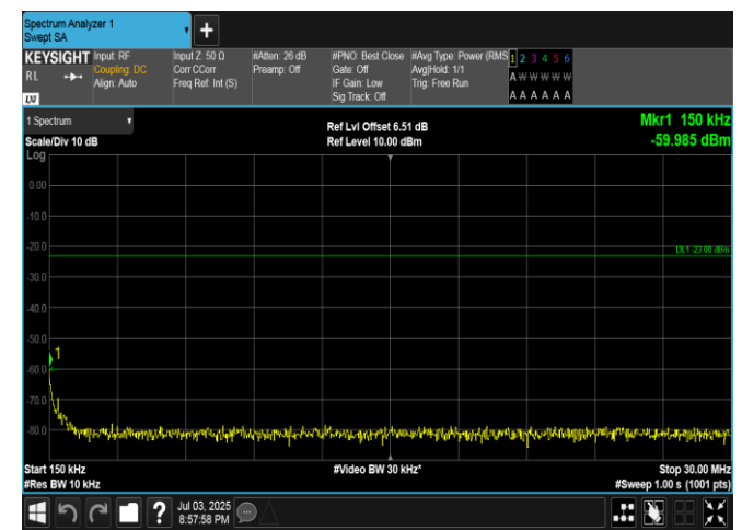
Band5-1.4MHz-QPSK-20643-6RB#0-0.15~30-PASS
