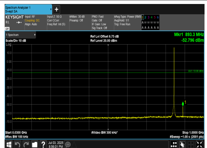
Band5-1.4MHz-QPSK-20643-1RB#5-30~1000-PASS
