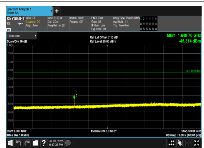
Band5-3MHz-QPSK-20415-1RB#0-1000~3000-PASS
