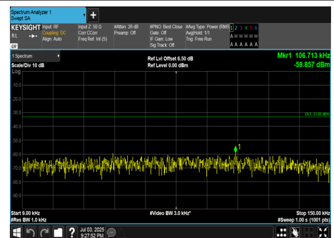
Band5-3MHz-QPSK-20525-15RB#0-0.009~0.15-PASS
