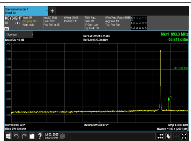
Band5-1.4MHz-16QAM-20643-6RB#0-30~1000-PASS
