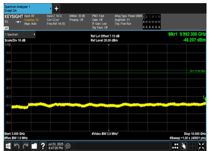
Band5-1.4MHz-16QAM-20407-6RB#0-3000~10000-PASS
