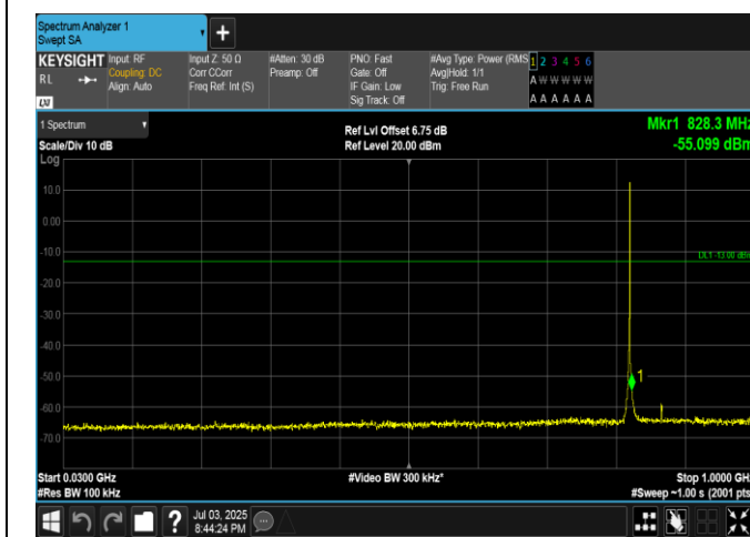
Band5-1.4MHz-16QAM-20407-1RB#5-30~1000-PASS
