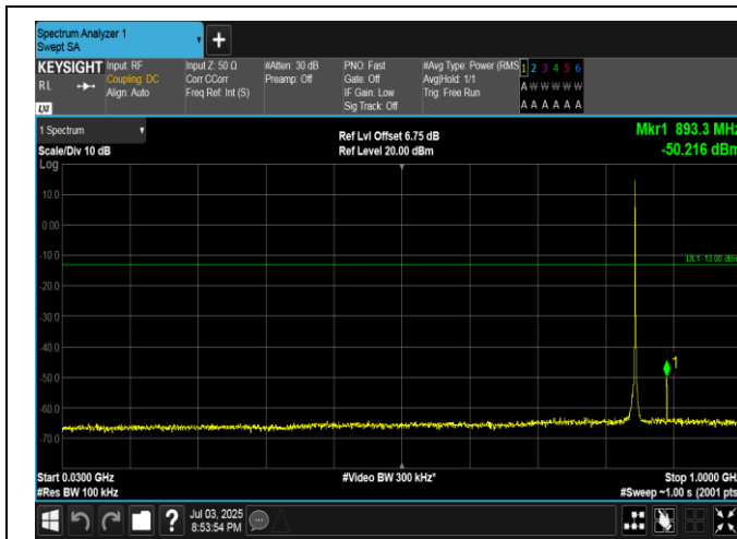
Band5-1.4MHz-QPSK-20643-1RB#0-30~1000-PASS
