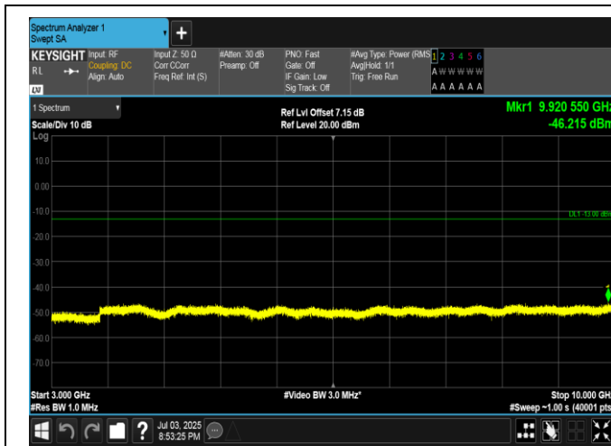
Band5-1.4MHz-16QAM-20525-6RB#0-3000~10000-PASS
