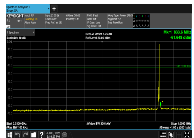
Band5-3MHz-QPSK-20415-1RB#14-30~1000-PASS
