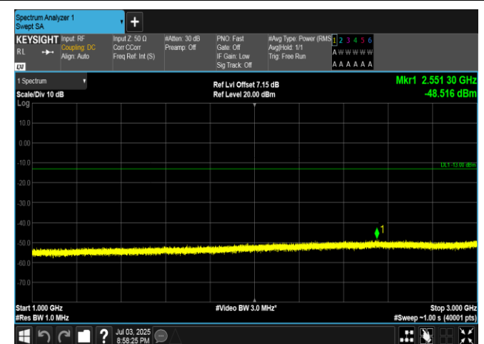
Band5-1.4MHz-QPSK-20643-6RB#0-1000~3000-PASS
