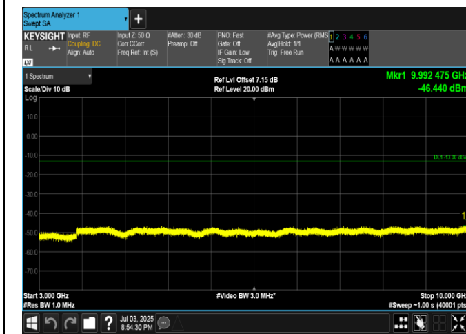
Band5-1.4MHz-QPSK-20643-1RB#0-3000~10000-PASS
