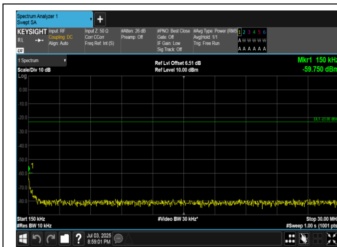
Band5-1.4MHz-16QAM-20643-6RB#0-0.15~30-PASS
