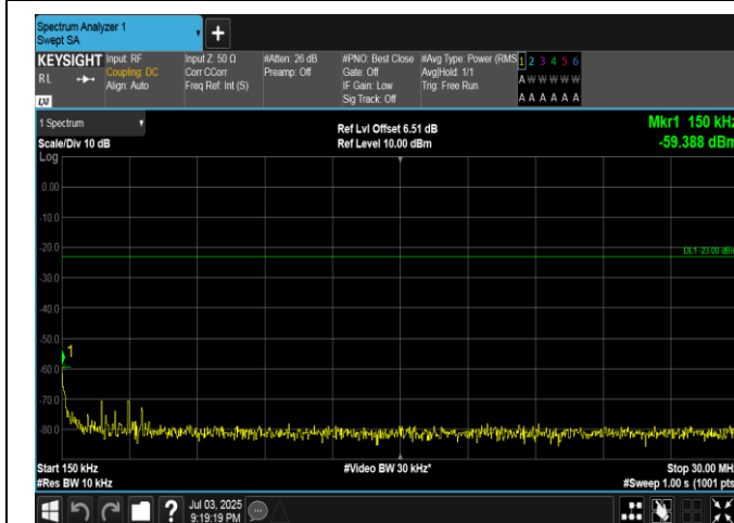
Band5-3MHz-QPSK-20415-1RB#14-0.15~30-PASS
