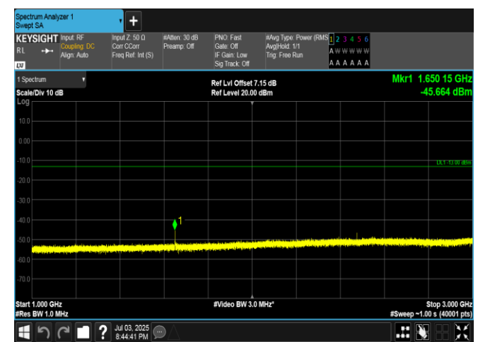
Band5-1.4MHz-16QAM-20407-1RB#5-1000~3000-PASS
