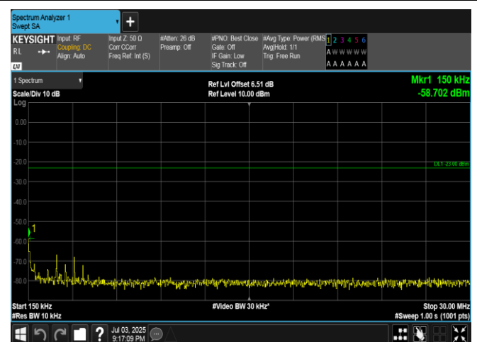
Band5-3MHz-QPSK-20415-1RB#0-0.15~30-PASS
