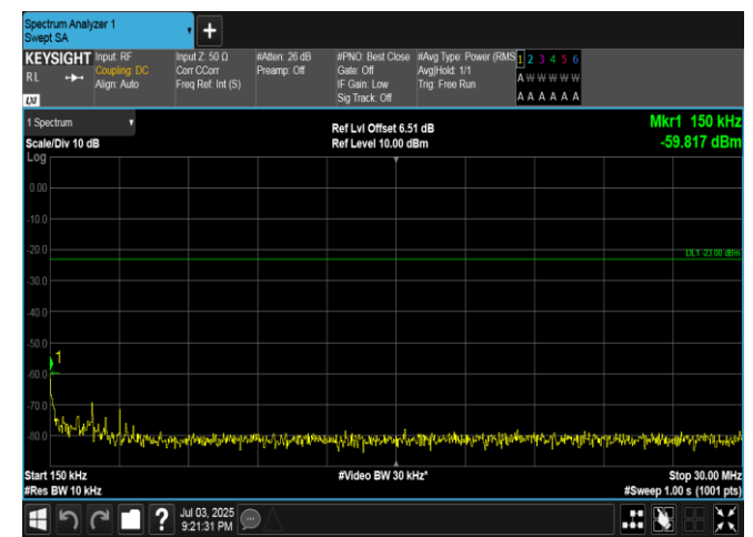
Band5-3MHz-QPSK-20415-15RB#0-0.15~30-PASS
