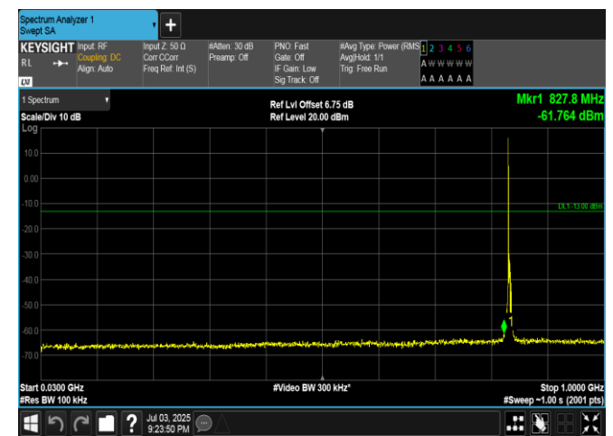
Band5-3MHz-QPSK-20525-1RB#0-30~1000-PASS
