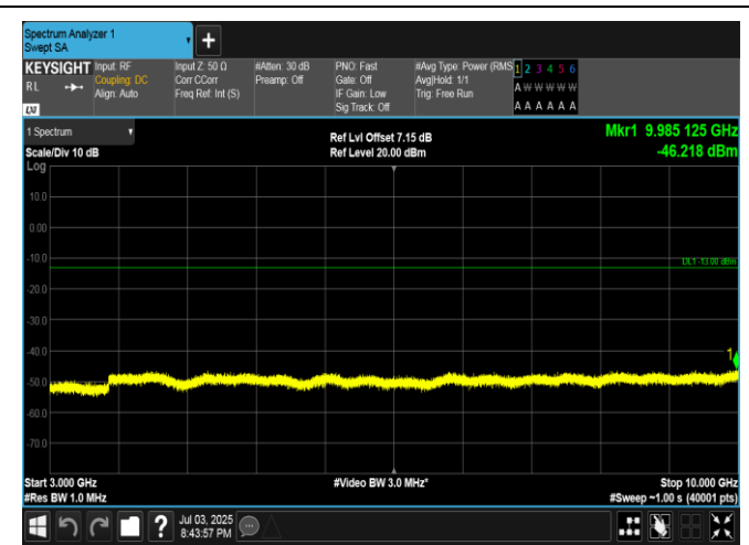
Band5-1.4MHz-QPSK-20407-1RB#5-3000~10000-PASS
