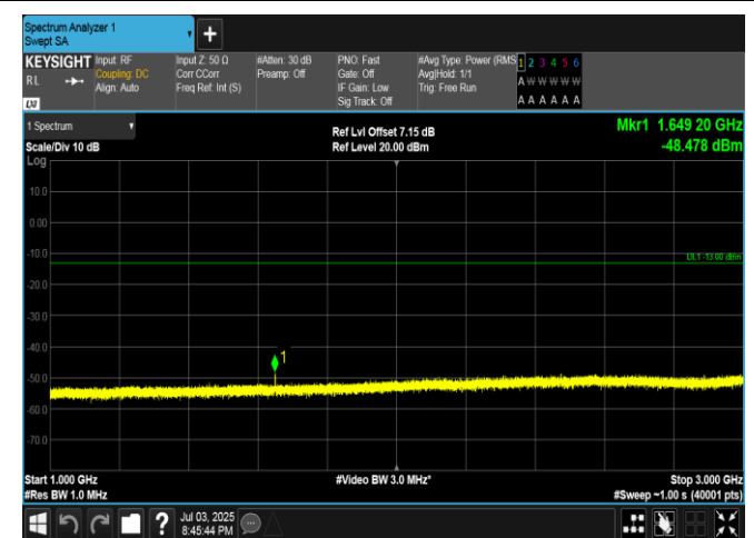
Band5-1.4MHz-QPSK-20407-6RB#0-1000~3000-PASS
