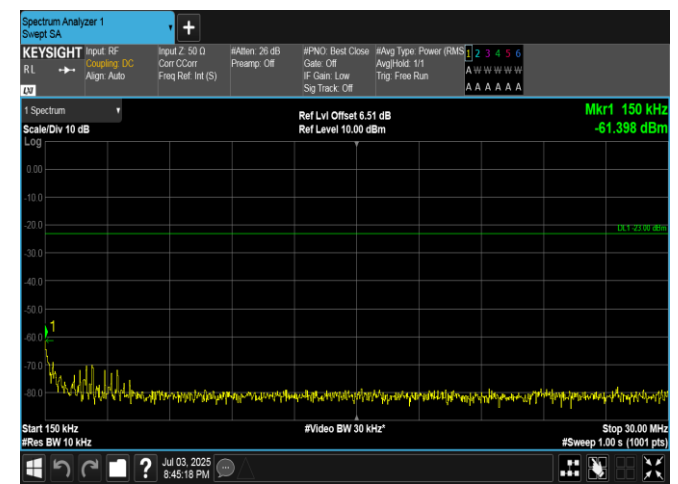
Band5-1.4MHz-QPSK-20407-6RB#0-0.15~30-PASS
