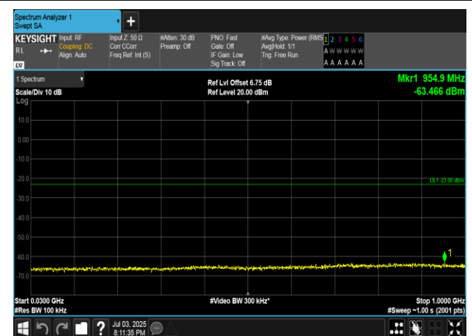
Band4-20MHz-16QAM-20050-1RB#0-30-1000-PASS
