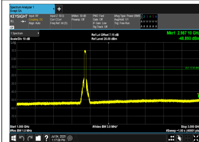
Band4-20MHz-16QAM-20300-100RB#0-1000~3000-PASS
