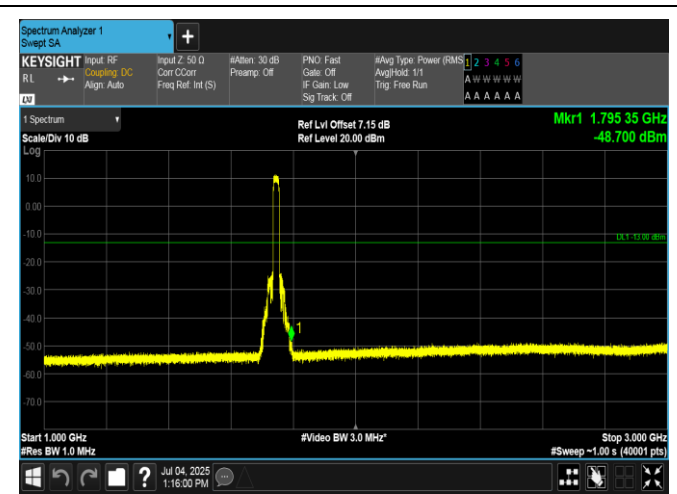
Band4-20MHz-QPSK-20300-100RB#0-1000-3000-PASS
