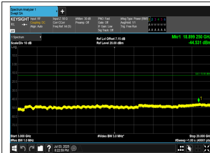
Band4-20MHz-16QAM-20300-1RB#99-3000~20000-PASS
