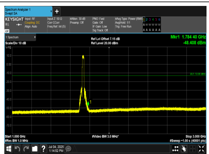
Band4-20MHz-16QAM-20175-100RB#0-1000~3000-PASS
