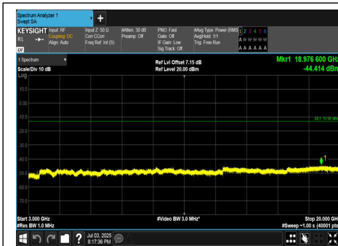
Band4-20MHz-QPSK-20175-1RB#99-3000~20000-PASS
