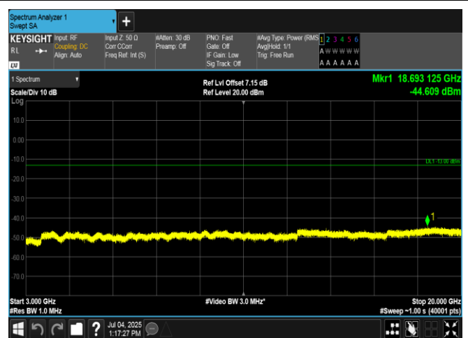
Band4-20MHz-16QAM-20300-100RB#0-3000~20000-PASS
