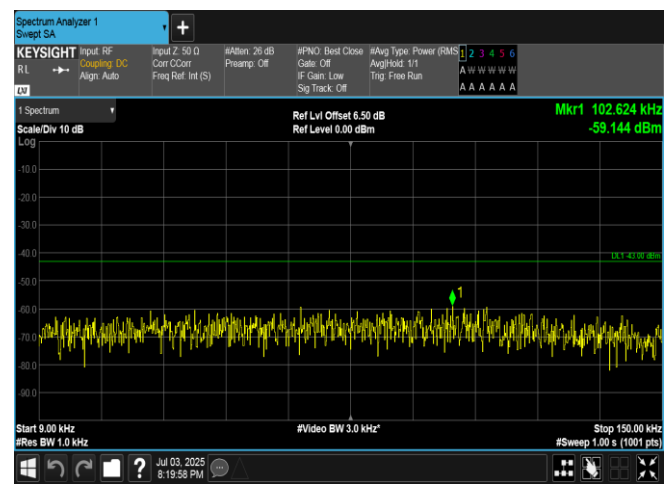
Band4-20MHz-16QAM-20300-1RB#0-0.009~0.15-PASS
