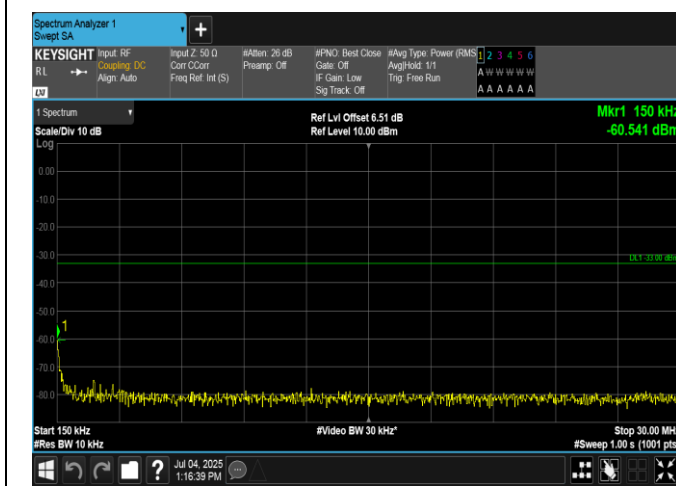
Band4-20MHz-16QAM-20300-100RB#0-0.15~30-PASS
