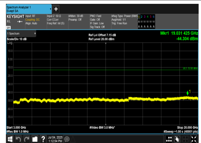
Band4-20MHz-16QAM-20050-100RB#0-3000~20000-PASS
