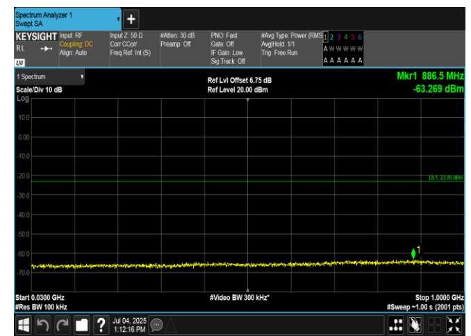
Band4-20MHz-16QAM-20050-100RB#0-30~1000-PASS
