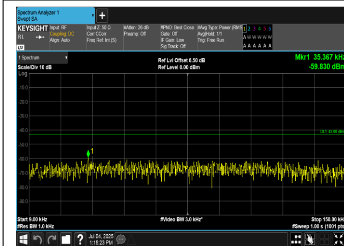
Band4-20MHz-QPSK-20300-100RB#0-0.009~0.15-PASS
