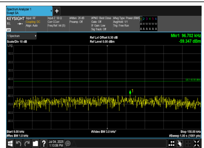
Band4-20MHz-QPSK-20175-100RB#0-0.009~0.15-PASS
