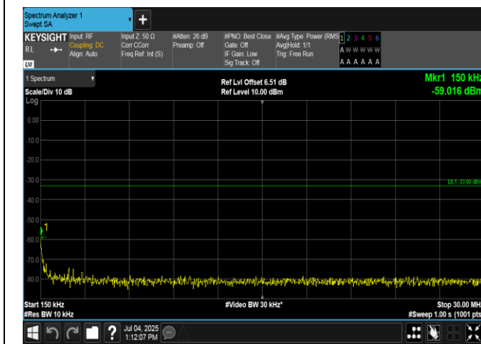
Band4-20MHz-16QAM-20050-100RB#0-0.15~30-PASS
