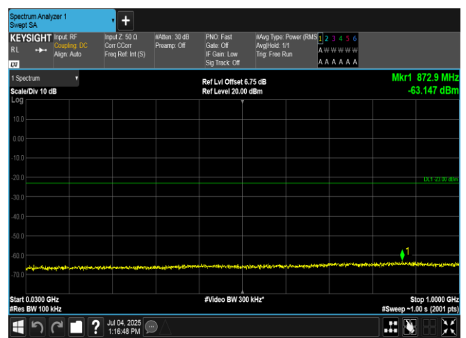
Band4-20MHz-16QAM-20300-100RB#0-30~1000-PASS
