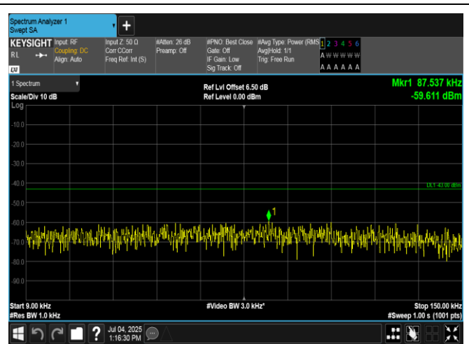
Band4-20MHz-16QAM-20300-100RB#0-0.009~0.15-PASS
