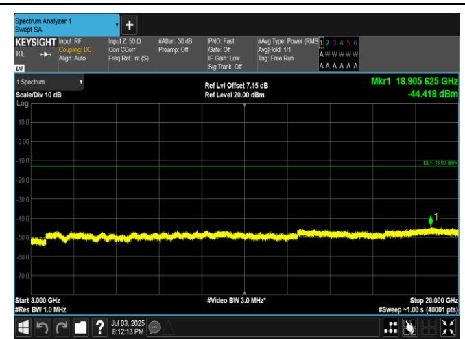
Band4-20MHz-16QAM-20050-1RB#0-3000-20000-PASS
