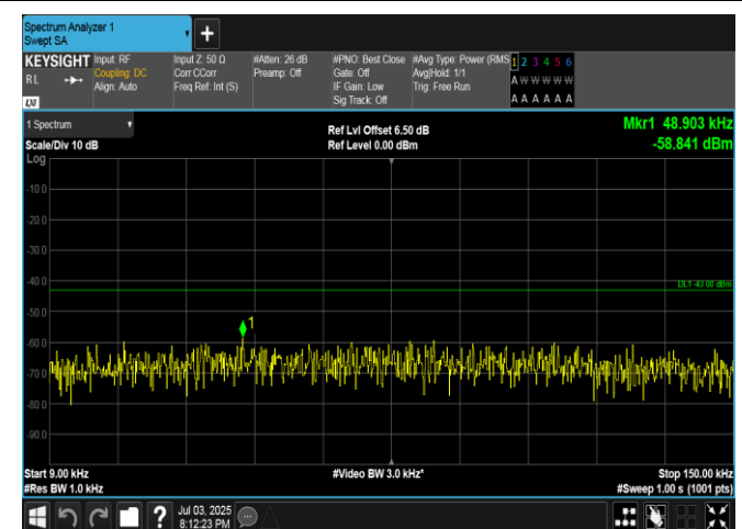
Band4-20MHz-QPSK-20050-1RB#99-0.009~0.15-PASS
