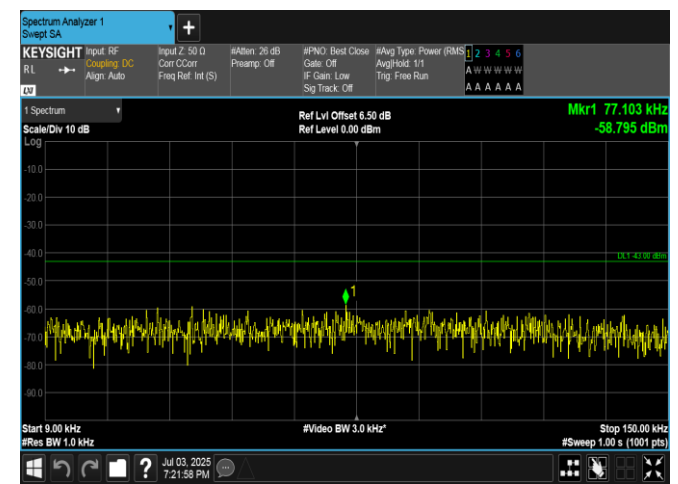
Band4-15MHz-16QAM-20025-1RB#0-0.009~0.15-PASS
