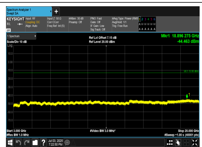
Band4-15MHz-16QAM-20025-1RB#0-3000~20000-PASS
