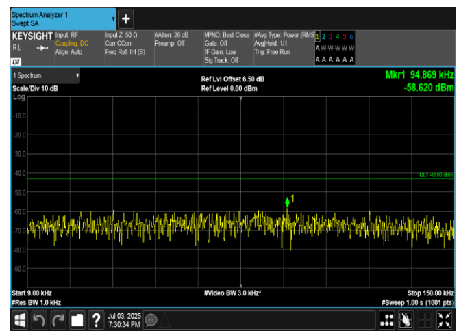
Band4-15MHz-16QAM-20325-1RB#0-0.009~0.15-PASS
