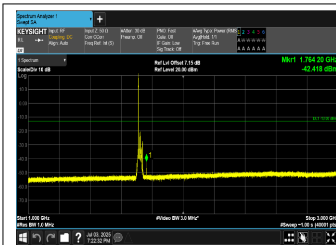
Band4-15MHz-16QAM-20025-1RB#0-1000~3000-PASS
