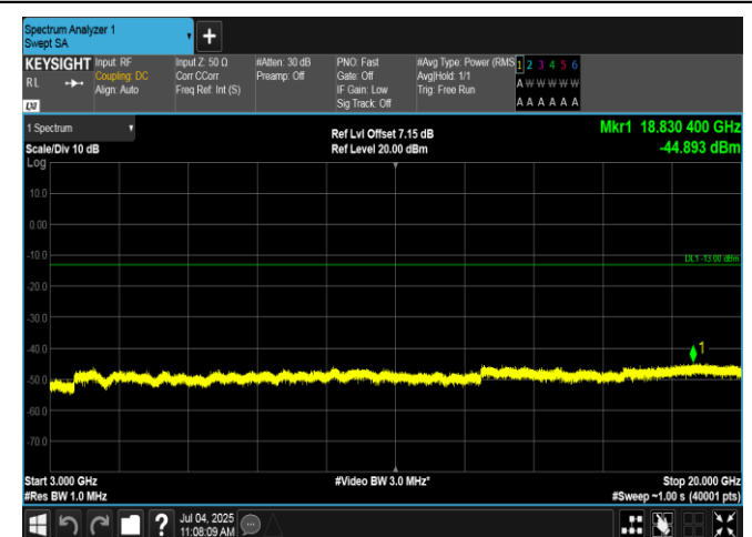
Band4-15MHz-16QAM-2025-75RB#0-3000~20000-PASS
