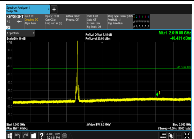
Band4-15MHz-16QAM-20025-1RB#74-1000~3000-PASS
