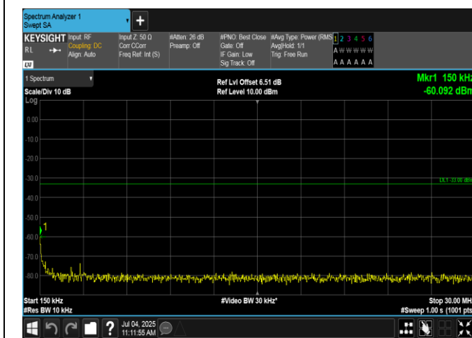
Band4-15MHz-16QAM-20325-75RB#0-0.15~30-PASS
