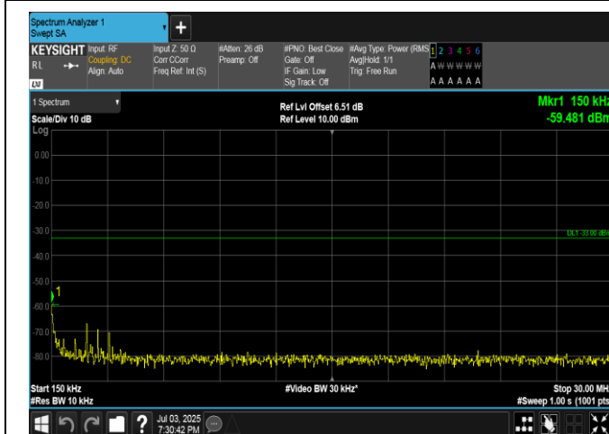
Band4-15MHz-16QAM-20325-1RB#0-0.15~30-PASS
