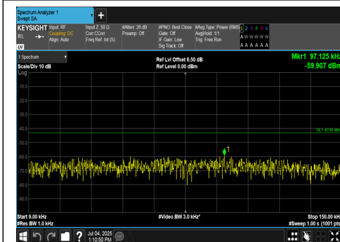
Band4-20MHz-QPSK-20050-100RB#0-0.009~0.15-PASS
