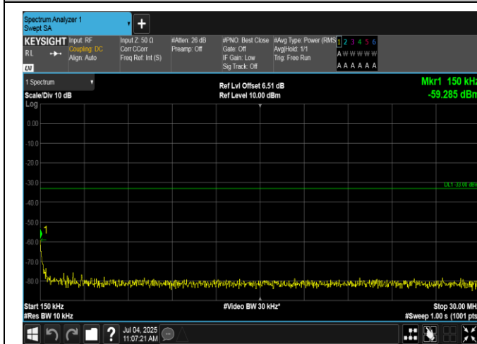
Band4-15MHz-16QAM-2025-75RB#0-0.15~30-PASS
