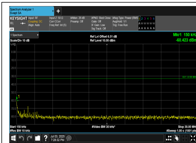
Band4-15MHz-16QAM-20175-1RB#74-0.15~30-PASS
