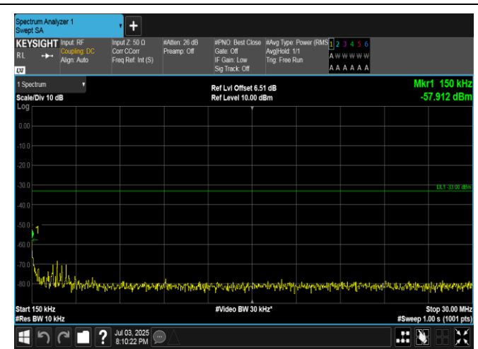
Band4-20MHz-QPSK-20050-1RB#0-0.15~30-PASS
