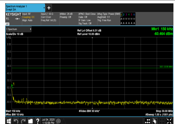
Band4-20MHz-QPSK-20050-100RB#0-0.15~30-PASS
