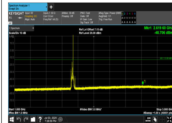
Band4-15MHz-16QAM-20175-1RB#74-1000~3000-PASS
