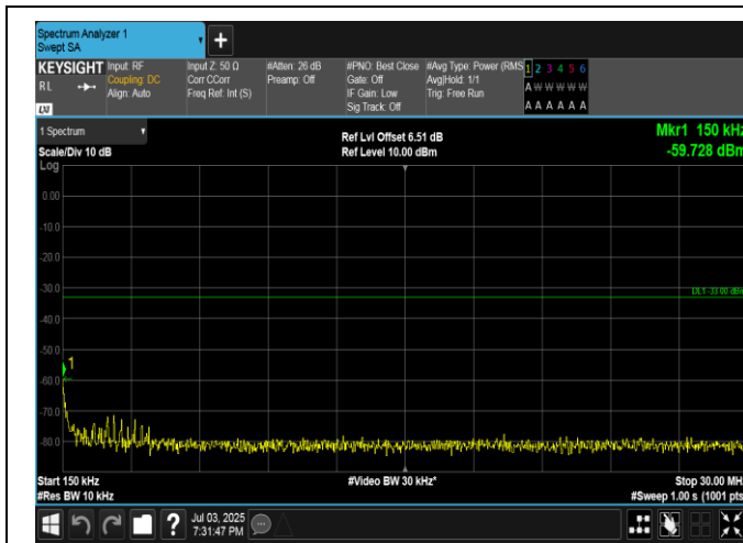
Band4-15MHz-QPSK-20325-1RB#74-0.15~30-PASS
