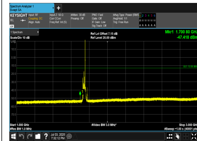
Band4-15MHz-QPSK-20325-1RB#74-1000~3000-PASS
