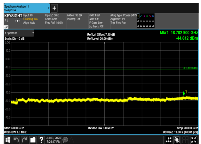
Band4-15MHz-16QAM-20175-1RB#74-3000~20000-PASS
