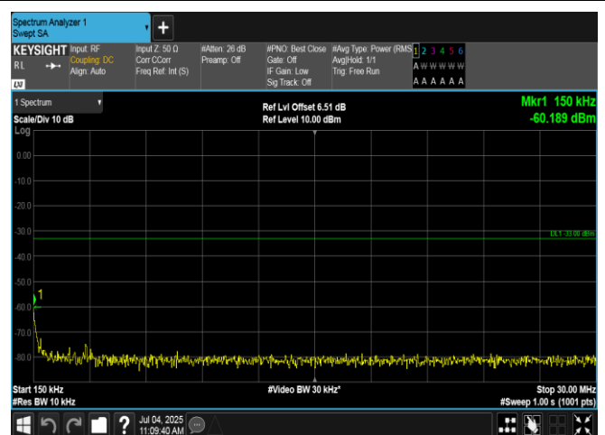
Band4-15MHz-16QAM-20175-75RB#0-0.15~30-PASS
