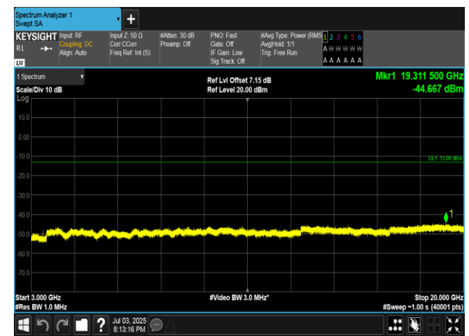
Band4-20MHz-QPSK-20050-1RB#99-3000~20000-PASS
