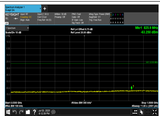
Band4-20MHz-QPSK-20050-1RB#99-30~1000-PASS
