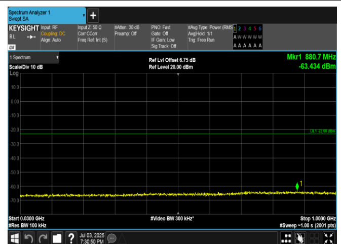
Band4-15MHz-16QAM-20325-1RB#0-30~1000-PASS
