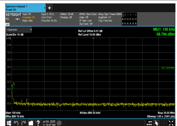
Band4-15MHz-QPSK-20325-75RB#0-0.15~30-PASS
