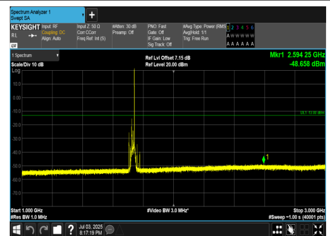
Band4-20MHz-QPSK-20175-1RB#99-1000-3000-PASS
