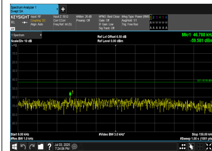
Band4-15MHz-16QAM-20025-1RB#74-0.009~0.15-PASS
