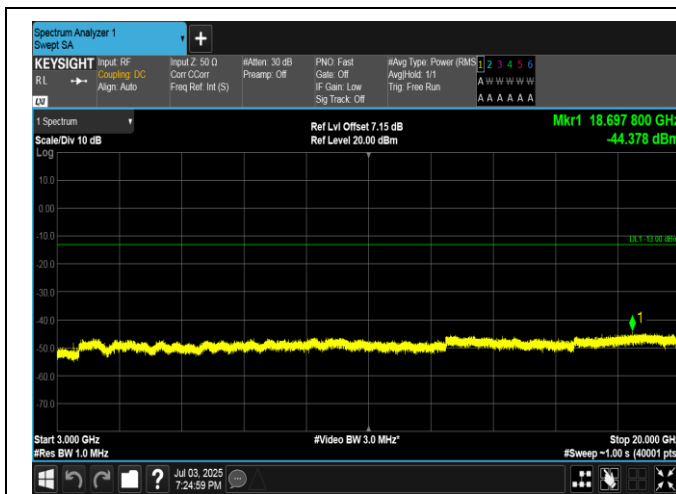
Band4-15MHz-16QAM-2025-1RB#74-3000~20000-PASS
