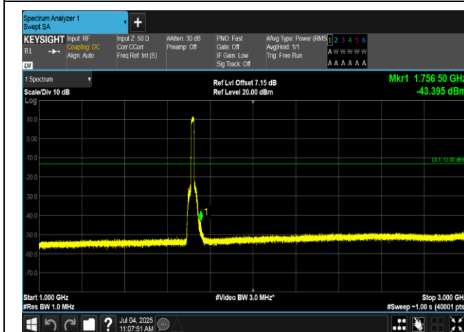
Band4-15MHz-16QAM-2025-75RB#0-1000~3000-PASS
