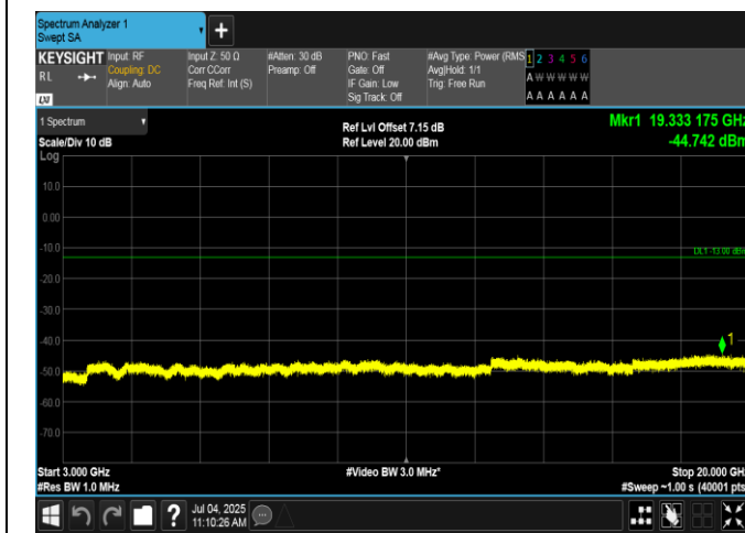
Band4-15MHz-16QAM-20175-75RB#0-3000~20000-PASS
