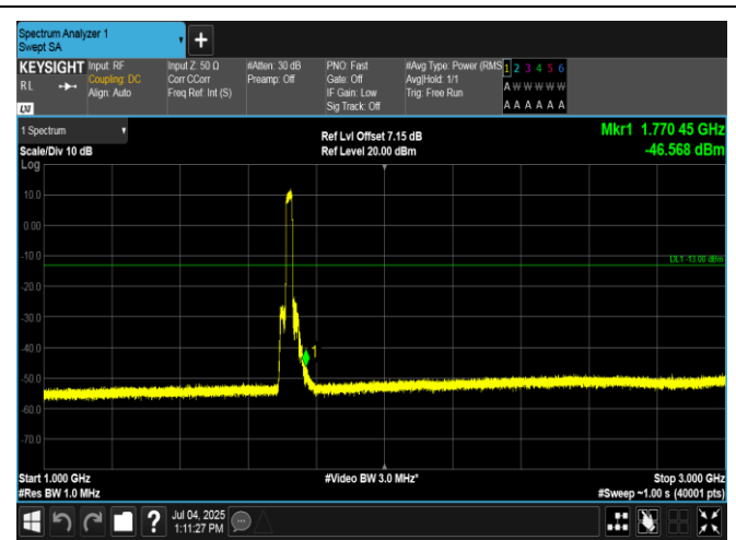
Band4-20MHz-QPSK-20050-100RB#0-1000-3000-PASS
