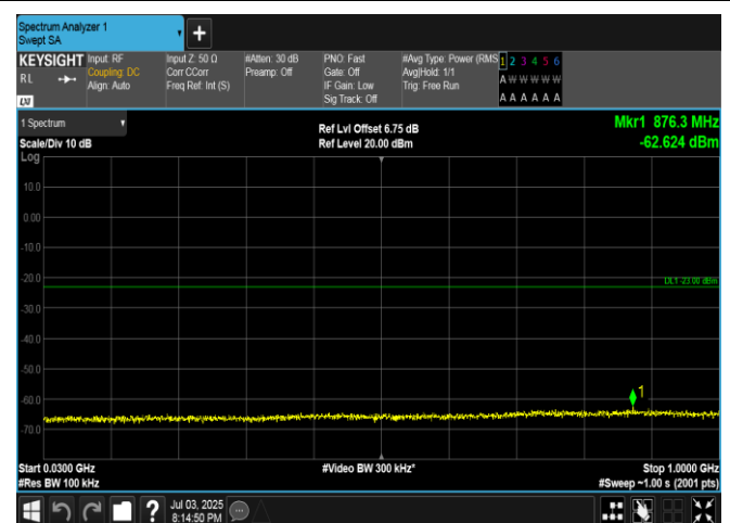
Band4-20MHz-QPSK-20175-1RB#0-30-1000-PASS
