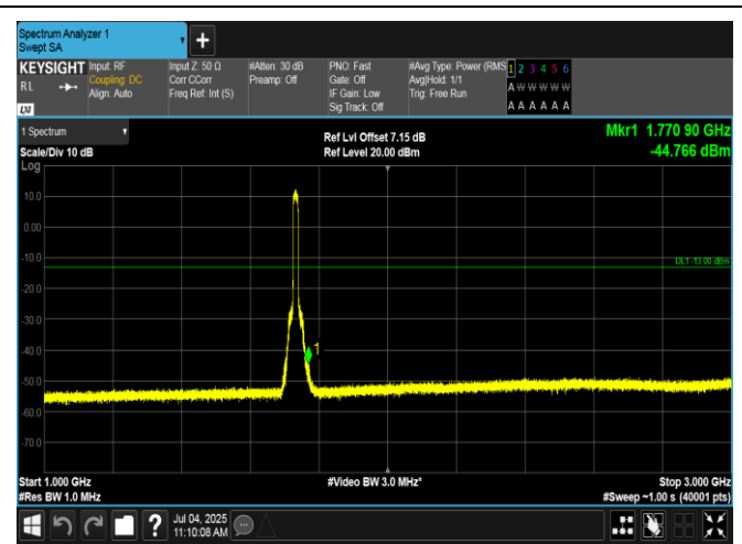
Band4-15MHz-16QAM-20175-75RB#0-1000~3000-PASS
