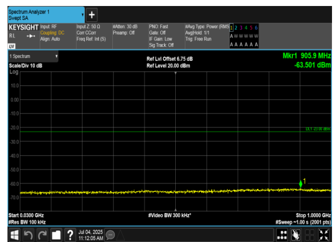
Band4-15MHz-16QAM-20325-75RB#0-30~1000-PASS
