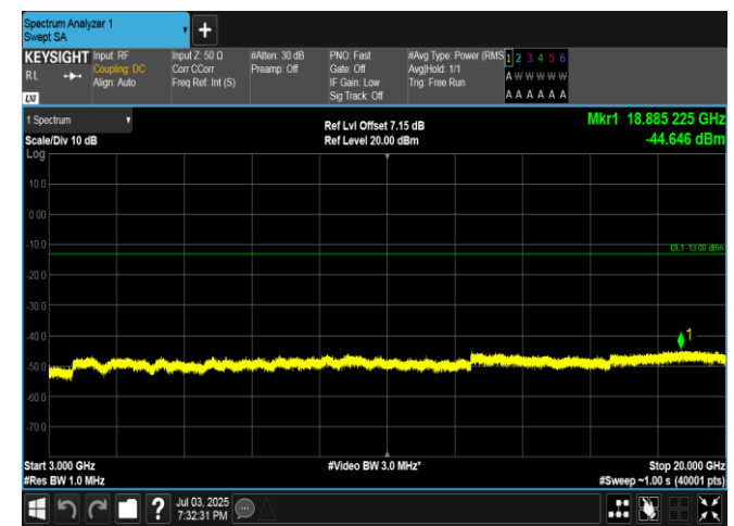
Band4-15MHz-QPSK-20325-1RB#74-3000~20000-PASS
