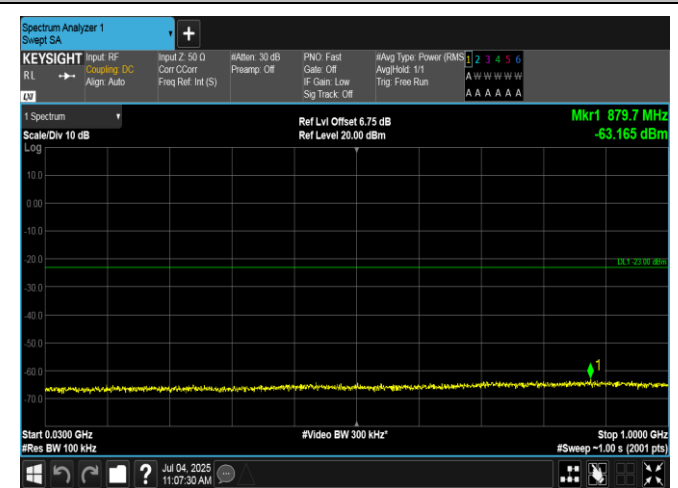
Band4-15MHz-16QAM-2025-75RB#0-30~1000-PASS
