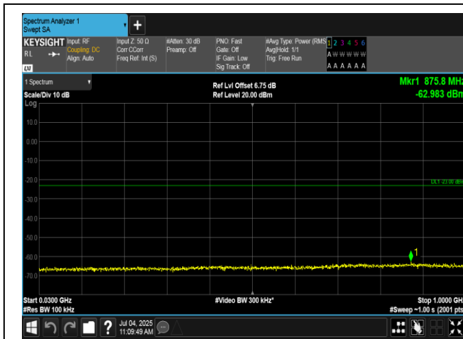
Band4-15MHz-16QAM-20175-75RB#0-30~1000-PASS
