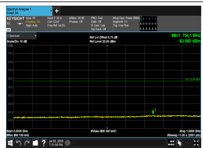
Band4-15MHz-QPSK-20325-1RB#74-30~1000-PASS
