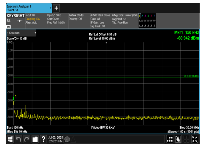
Band4-20MHz-QPSK-20175-1RB#99-0.15-30-PASS
