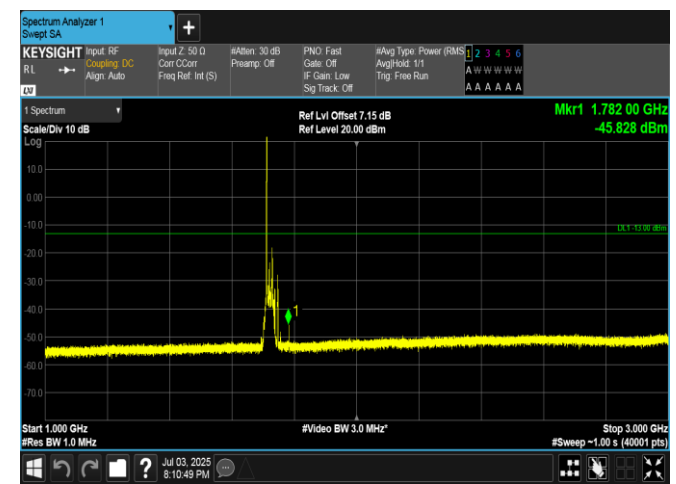
Band4-20MHz-QPSK-20050-1RB#0-1000~3000-PASS
