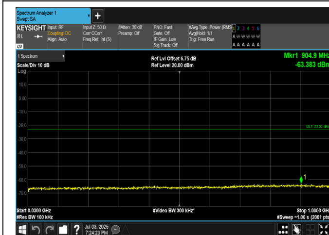
Band4-15MHz-16QAM-20025-1RB#74-30~1000-PASS
