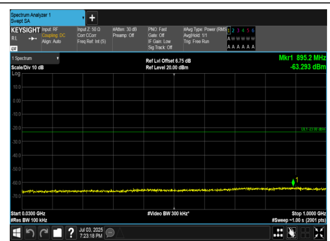
Band4-15MHz-QPSK-20025-1RB#74-30~1000-PASS
