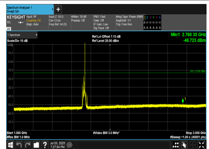
Band4-15MHz-QPSK-20175-1RB#74-1000-3000-PASS
