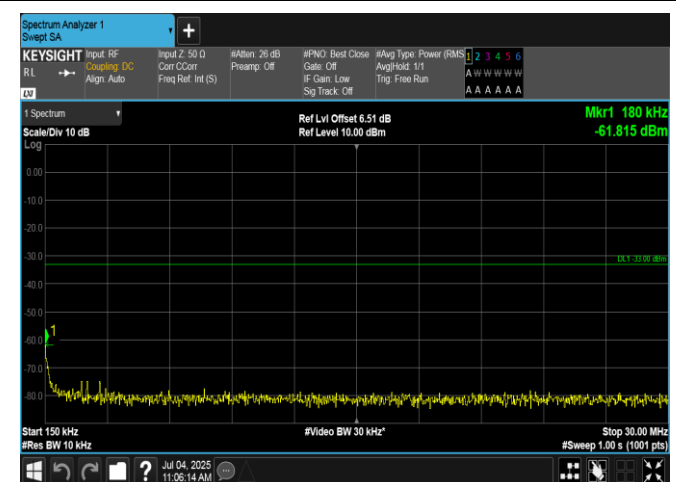
Band4-15MHz-QPSK-20025-75RB#0-0.15~30-PASS
