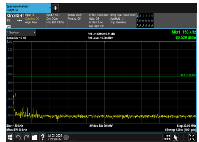
Band4-15MHz-QPSK-20175-1RB#74-0.15-30-PASS
