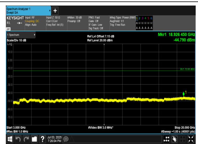
Band4-15MHz-QPSK-20175-1RB#0-3000-20000-PASS
