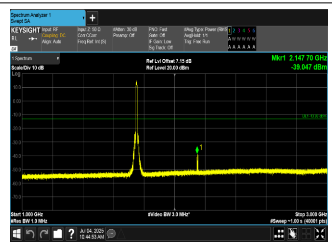
Band4-10MHz-QPSK-20350-50RB#0-1000~3000-PASS
