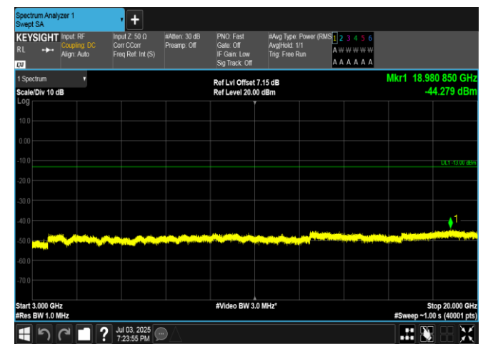
Band4-15MHz-QPSK-20025-1RB#74-3000~20000-PASS
