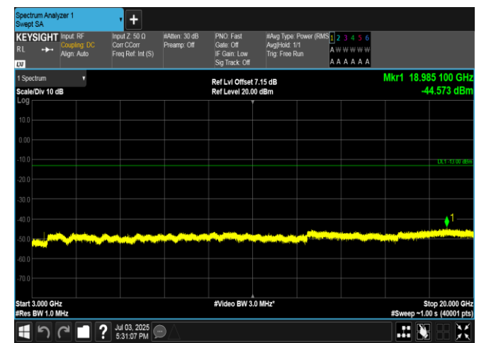
Band4-5MHz-16QAM-20175-1RB#24-3000~20000-PASS
