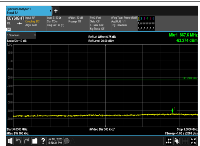
Band4-5MHz-16QAM-20175-1RB#24-30~1000-PASS
