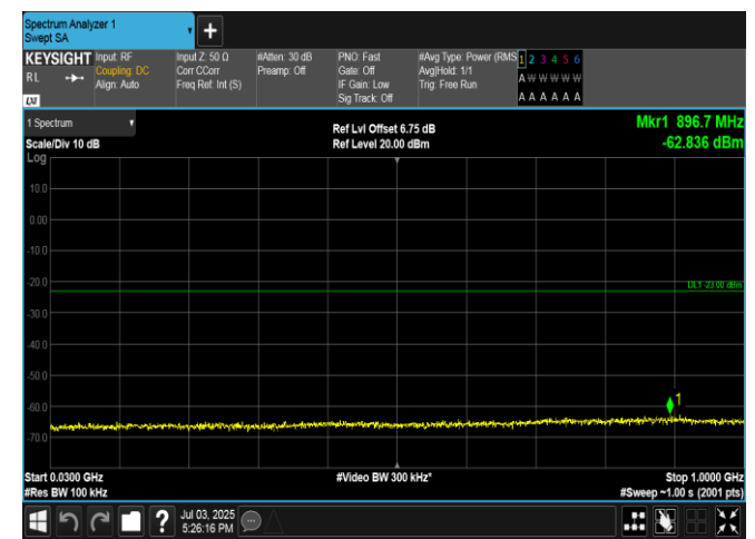
Band4-5MHz-16QAM-19975-25RB#0-30~1000-PASS
