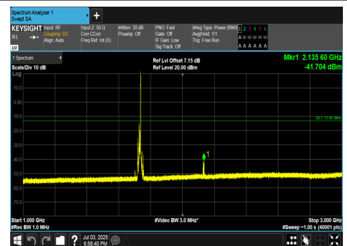
Band4-10MHz-QPSK-20175-1RB#49-1000~3000-PASS
