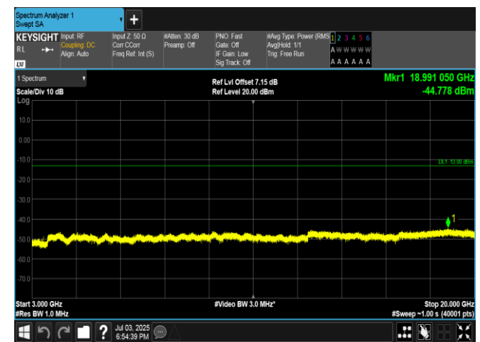
Band4-10MHz-QPSK-20000-1RB#49-3000~20000-PASS
