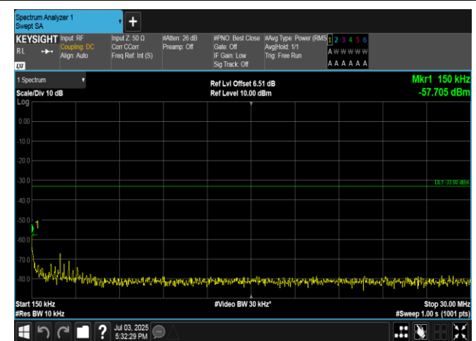
Band4-5MHz-16QAM-20175-25RB#0-0.15~30-PASS
