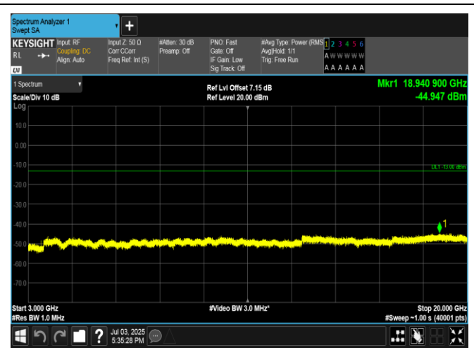
Band4-5MHz-16QAM-20375-1RB#0-3000-20000-PASS
