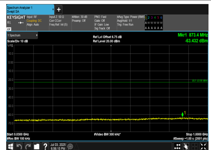
Band4-10MHz-QPSK-20175-1RB#0-30~1000-PASS
