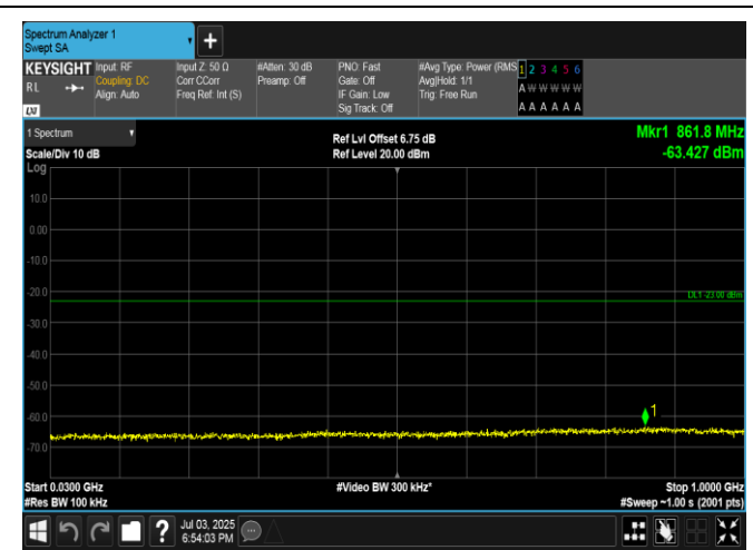
Band4-10MHz-QPSK-20000-1RB#49-30~1000-PASS
