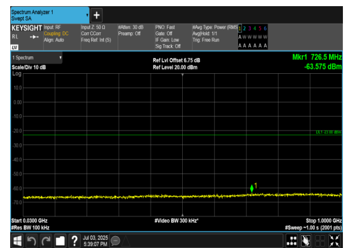
Band4-5MHz-16QAM-20375-25RB#0-30~1000-PASS
