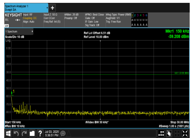
Band4-5MHz-16QAM-20375-1RB#24-0.15-30-PASS
