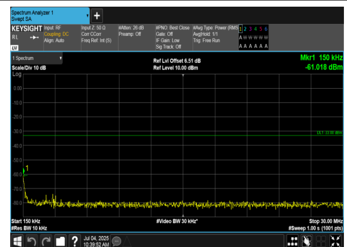
Band4-10MHz-QPSK-20000-50RB#0-0.15~30-PASS
