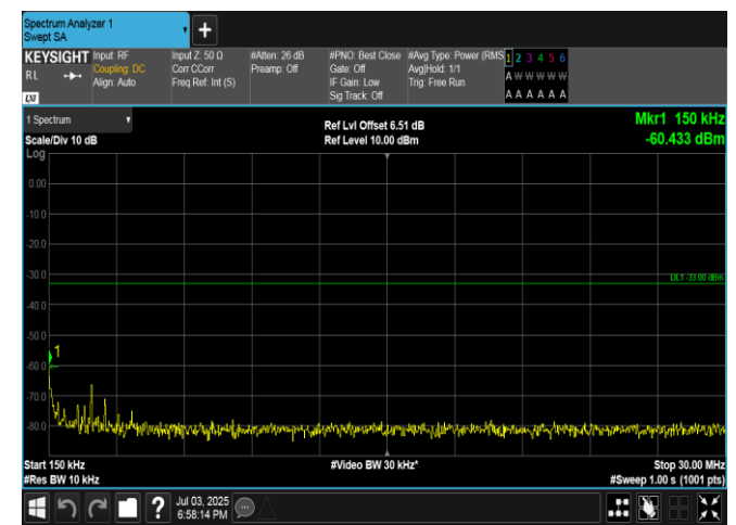
Band4-10MHz-QPSK-20175-1RB#49-0.15~30-PASS
