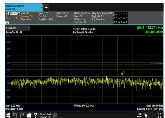
Band4-10MHz-QPSK-20350-1RB#49-0.009~0.15-PASS
