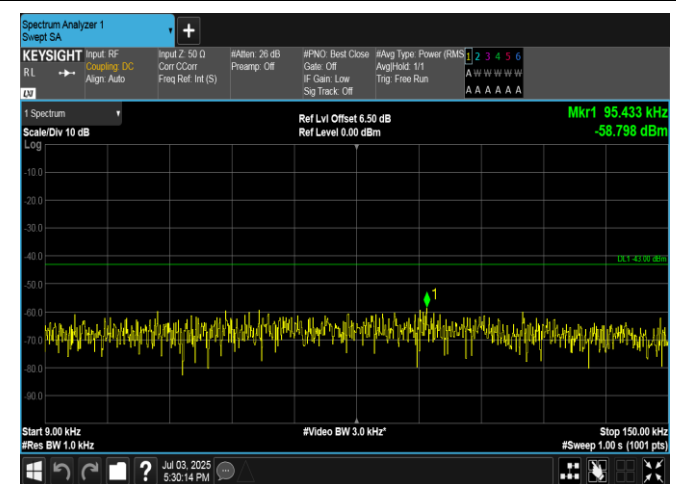
Band4-5MHz-16QAM-20175-1RB#24-0.009~0.15-PASS
