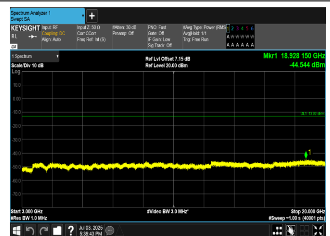
Band4-5MHz-16QAM-20375-25RB#0-3000~20000-PASS
