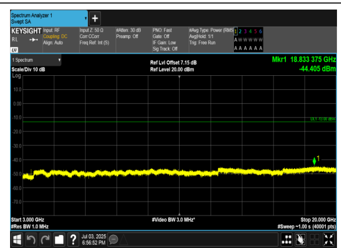
Band4-10MHz-QPSK-20175-1RB#0-3000~20000-PASS
