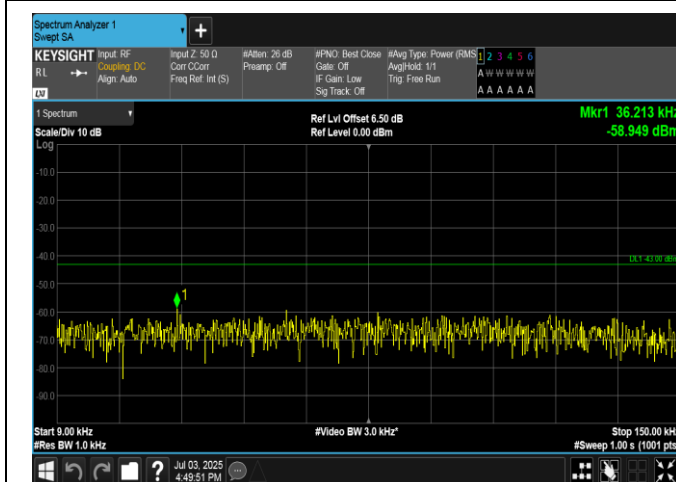
Band4-3MHz-QPSK-20385-15RB#0-0.009~0.15-PASS
