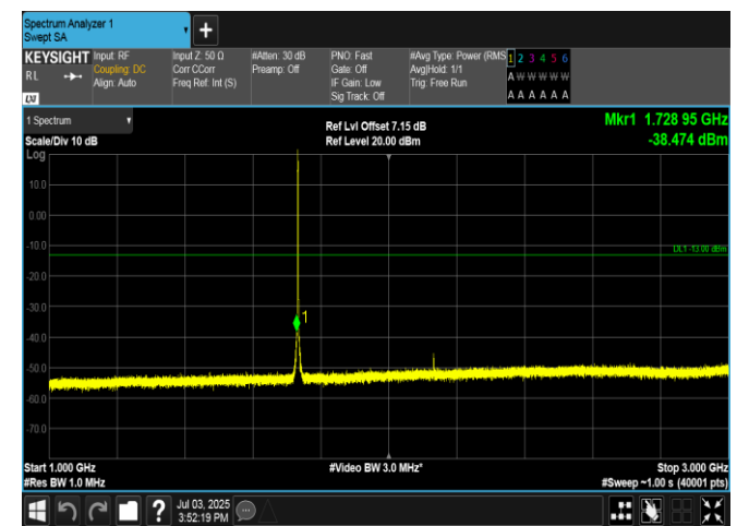
Band4-1.4MHz-16QAM-20175-1RB#0-1000~3000-PASS
