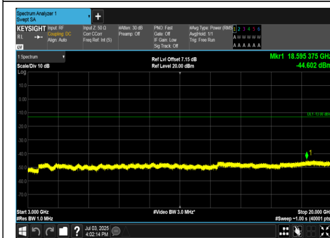
Band4-1.4MHz-QPSK-20393-6RB#0-3000~20000-PASS
