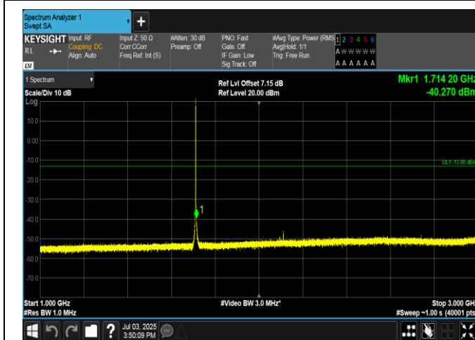
Band4-1.4MHz-16QAM-19957-6RB#0-1000~3000-PASS
