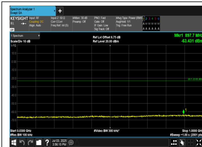
Band4-1.4MHz-16QAM-20175-6RB#0-30~1000-PASS
