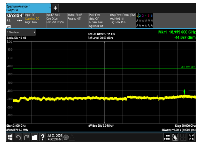
Band4-3MHz-QPSK-19965-1RB#14-3000~20000-PASS
