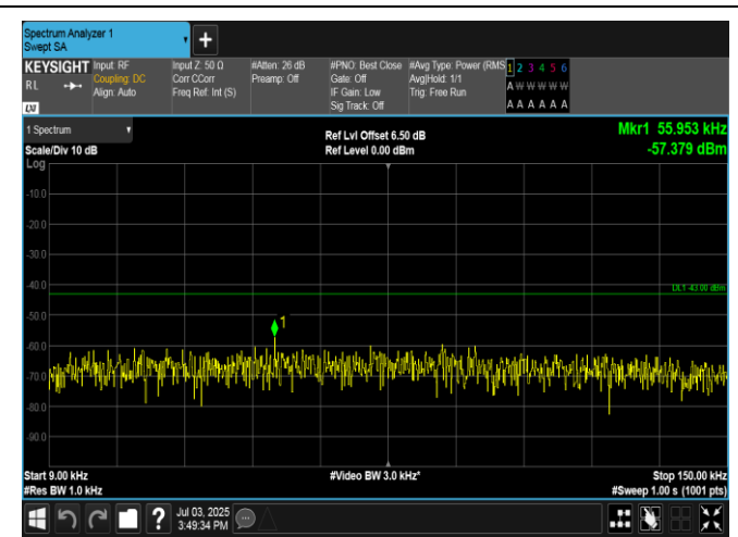
Band4-1.4MHz-16QAM-19957-6RB#0-0.009~0.15-PASS
