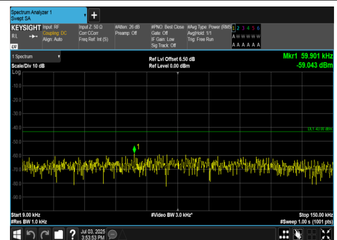
Band4-1.4MHz-16QAM-20175-1RB#5-0.009~0.15-PASS
