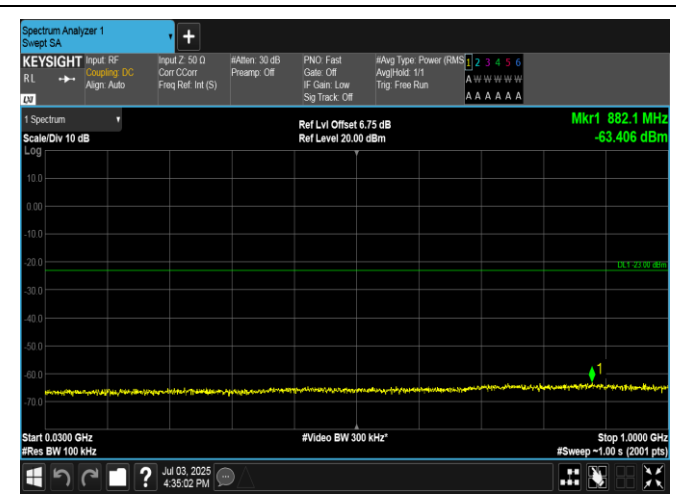
Band4-3MHz-QPSK-19965-1RB#14-30~1000-PASS
