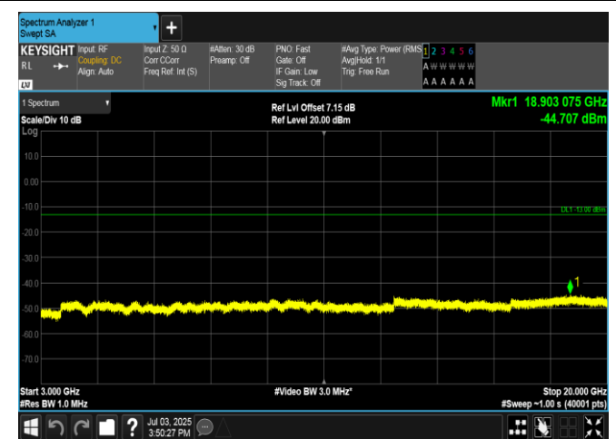
Band4-1.4MHz-16QAM-19957-6RB#0-3000~20000-PASS
