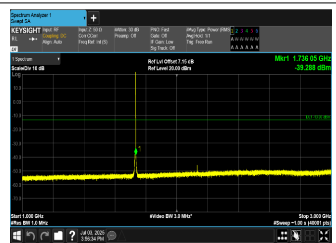
Band4-1.4MHz-16QAM-20175-6RB#0-1000~3000-PASS
