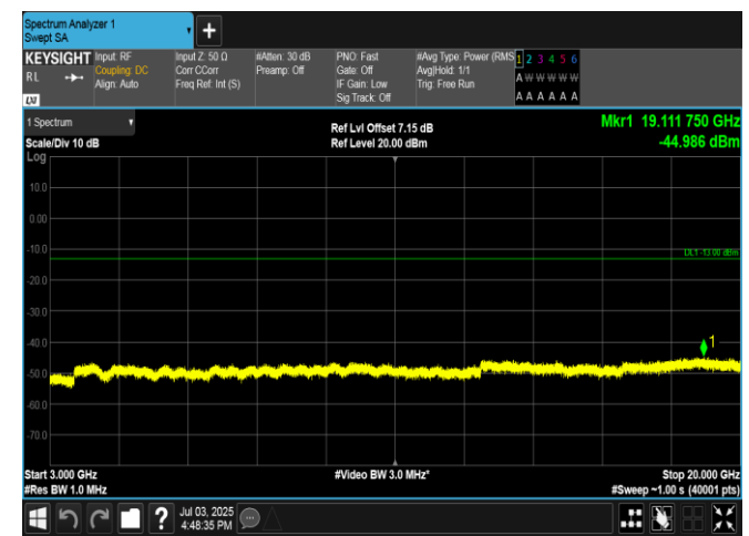
Band4-3MHz-QPSK-20385-1RB#14-3000~20000-PASS
