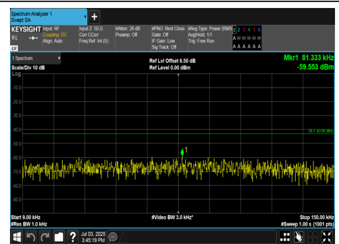
Band4-1.4MHz-16QAM-19957-1RB#0-0.009~0.15-PASS
