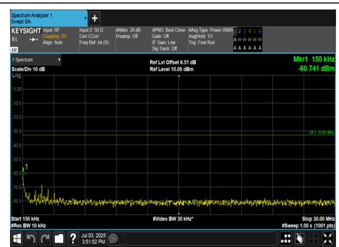
Band4-1.4MHz-16QAM-20175-1RB#0-0.15~30-PASS
