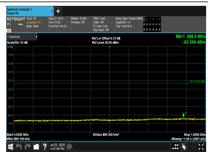
Band4-3MHz-QPSK-20385-1RB#14-30~1000-PASS
