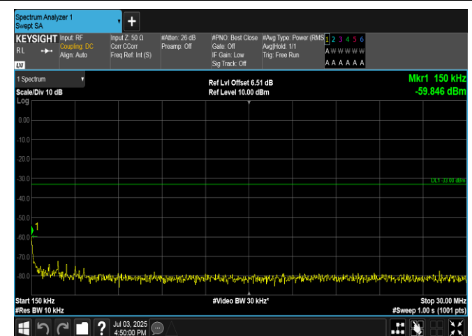
Band4-3MHz-QPSK-20385-15RB#0-0.15~30-PASS
