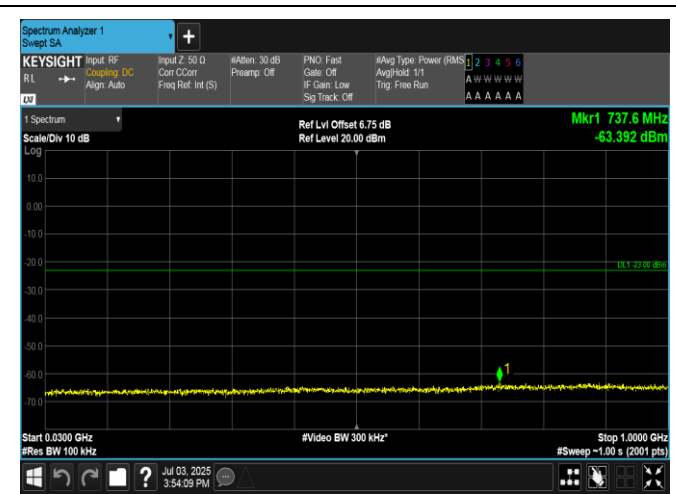
Band4-1.4MHz-16QAM-20175-1RB#5-30-1000-PASS
