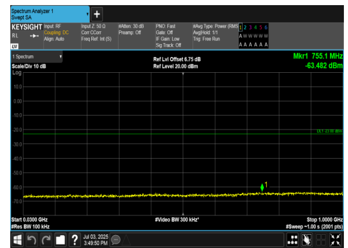
Band4-1.4MHz-16QAM-19957-6RB#0-30~1000-PASS
