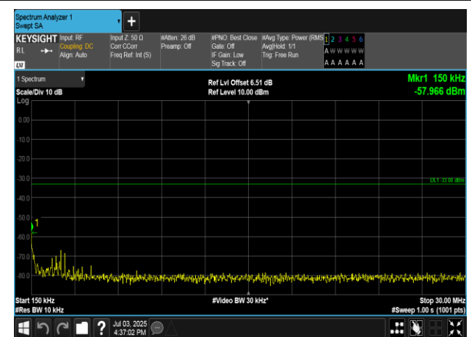
Band4-3MHz-QPSK-19965-15RB#0-0.15~30-PASS
