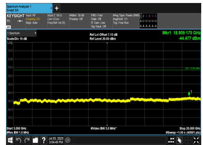
Band4-1.4MHz-16QAM-20175-1RB#5-3000-20000-PASS
