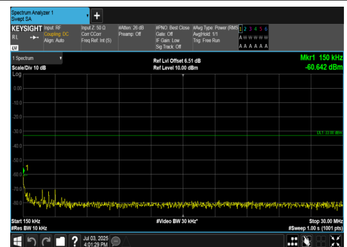
Band4-1.4MHz-QPSK-20393-6RB#0-0.15~30-PASS
