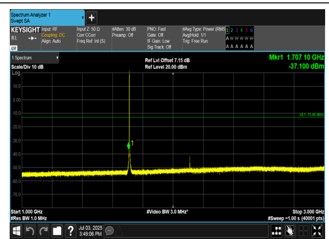
Band4-1.4MHz-QPSK-19957-6RB#0-1000~3000-PASS
