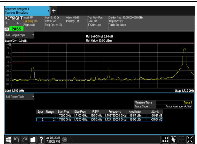
Band4-15MHz-QPSK-20025-1RB#74-PASS
