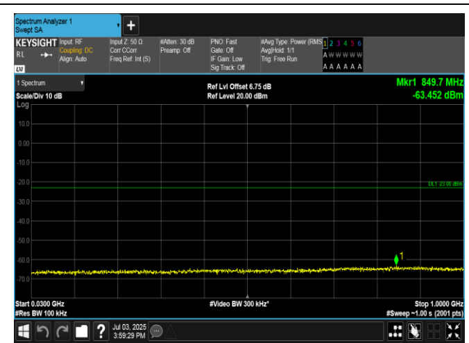
Band4-1.4MHz-QPSK-20393-1RB#5-30~1000-PASS
