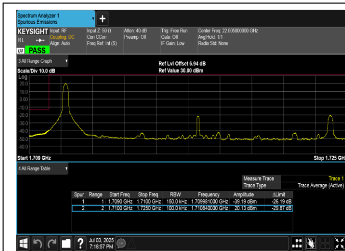
Band4-15MHz-QPSK-20025-1RB#0-PASS
