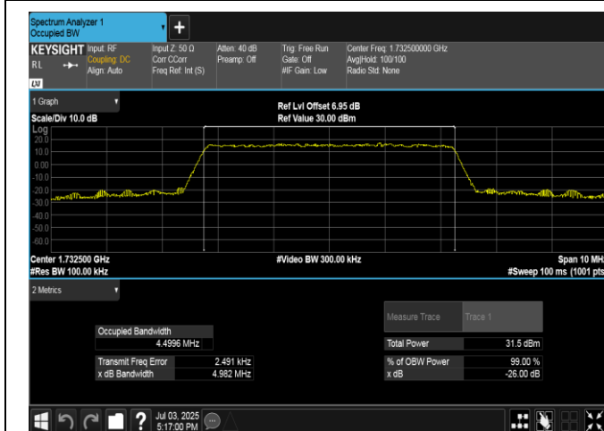
Band4-5MHz-16QAM-20175-25RB#0-PASS
