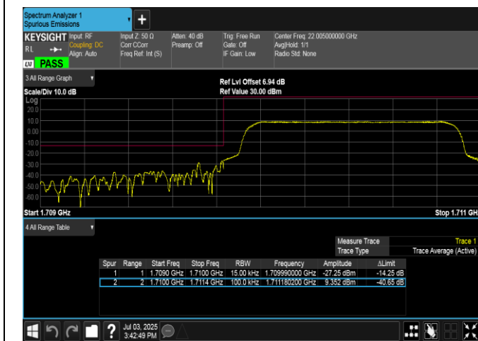
Band4-1.4MHz-16QAM-19957-6RB#0-PASS
