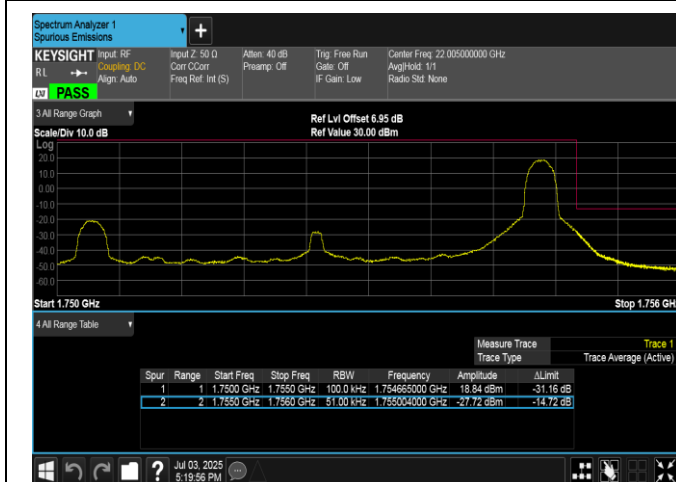
Band4-5MHz-16QAM-20375-1RB#24-PASS
