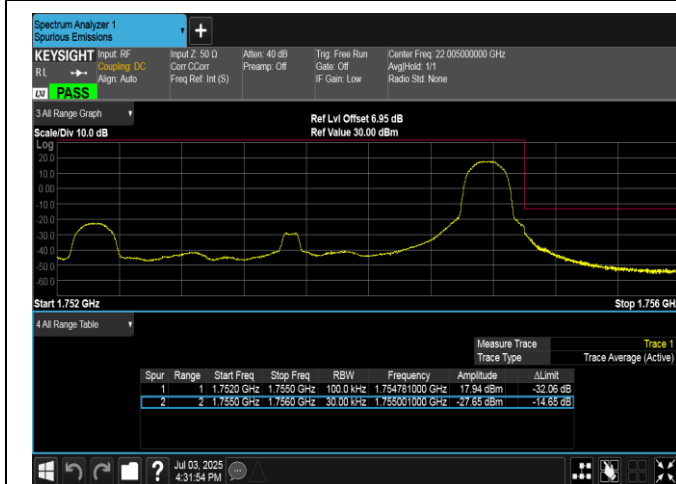
Band4-3MHz-16QAM-20385-1RB#14-PASS
