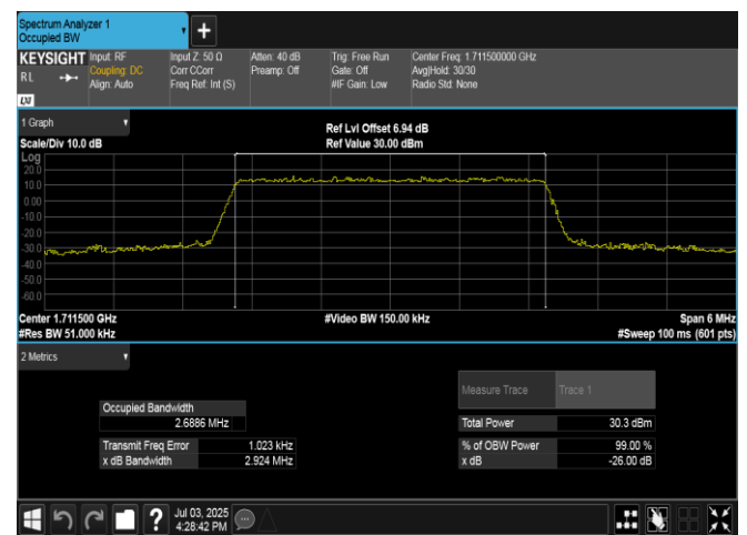
Band4-3MHz-16QAM-19965-15RB#0-PASS
