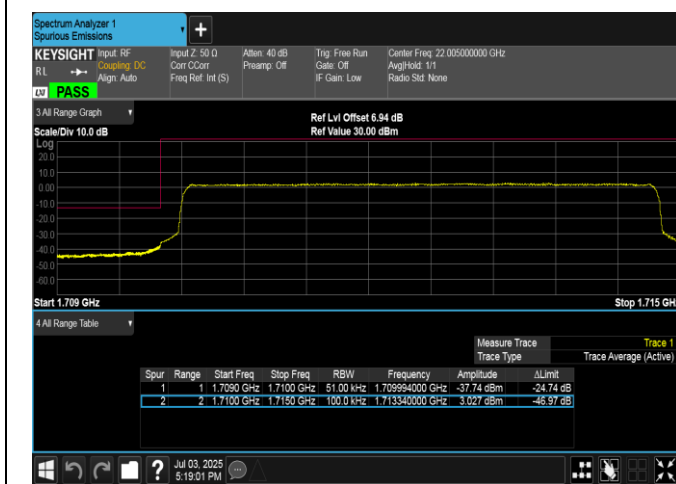
Band4-5MHz-16QAM-19975-25RB#0-PASS
