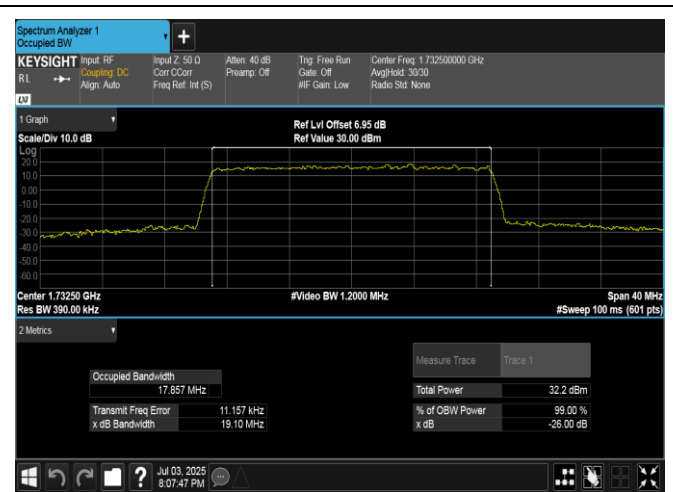
Band4-20MHz-QPSK-20175-100RB#0-PASS
