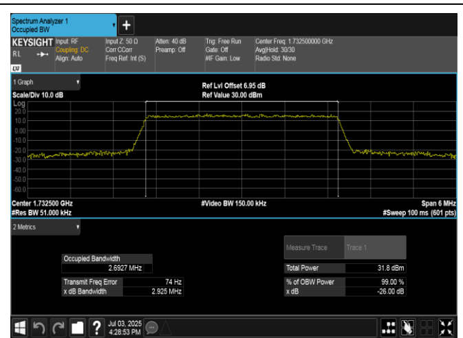
Band4-3MHz-QPSK-20175-15RB#0-PASS
