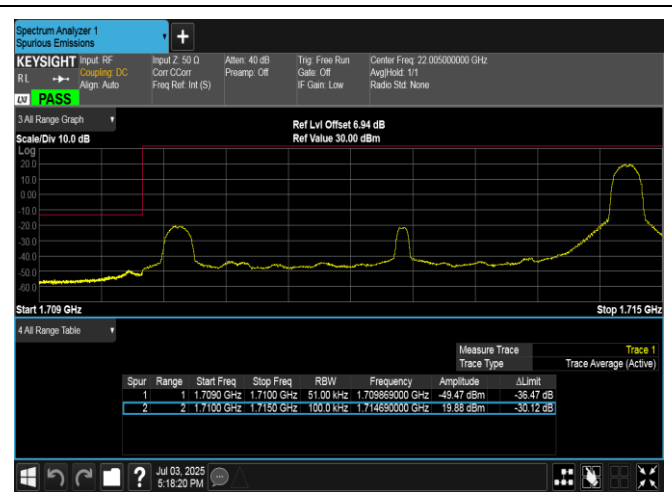
Band4-5MHz-QPSK-19975-1RB#24-PASS
