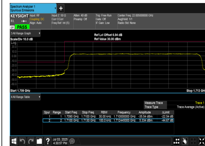
Band4-3MHz-16QAM-19965-15RB#0-PASS
