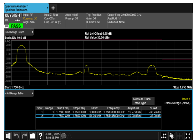
Band4-5MHz-QPSK-20375-1RB#0-PASS
