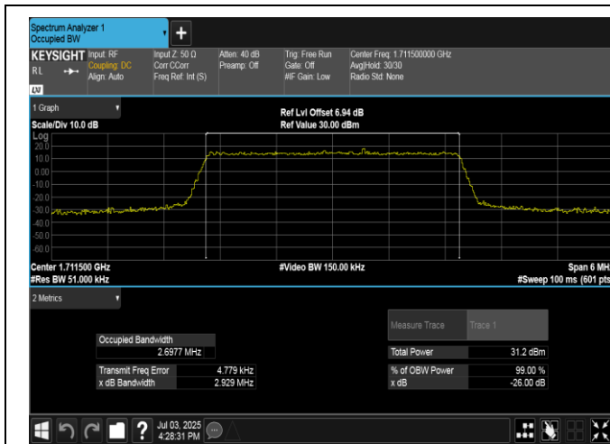
Band4-3MHz-QPSK-19965-15RB#0-PASS
