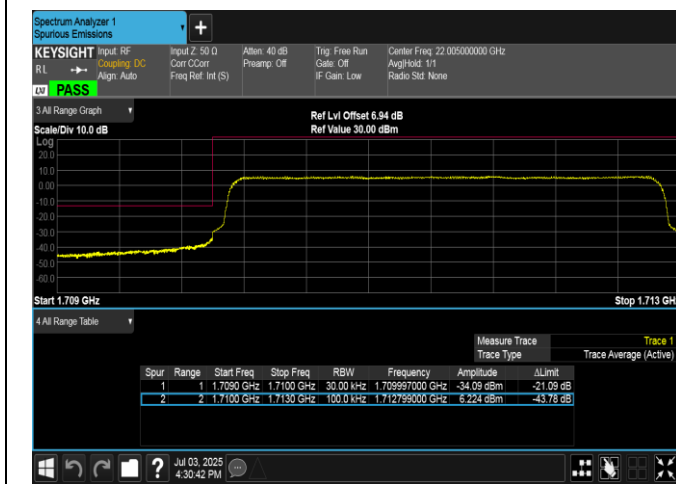
Band4-3MHz-QPSK-19965-15RB#0-PASS
