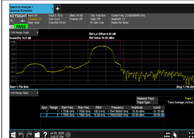
Band4-1.4MHz-16QAM-20393-1RB#5-PASS
