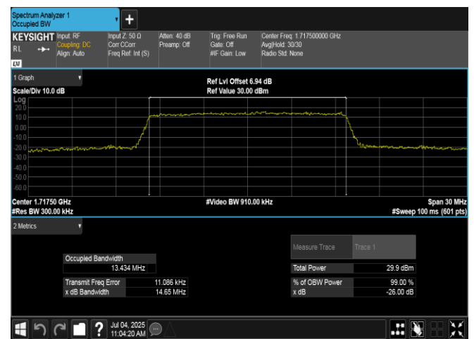
Band4-15MHz-16QAM-2025-75RB#0-PASS
