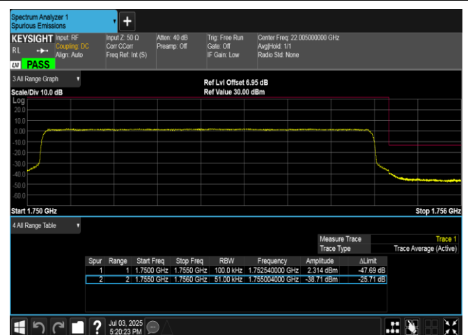
Band4-5MHz-16QAM-20375-25RB#0-PASS
