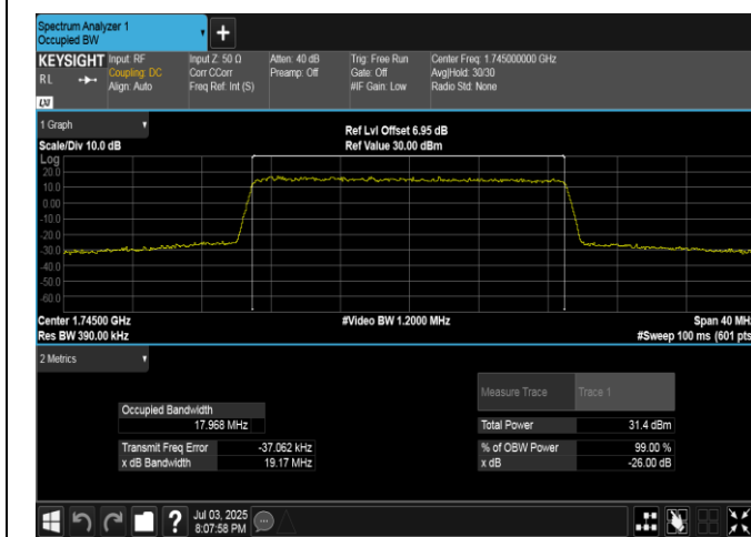
Band4-20MHz-QPSK-20300-100RB#0-PASS
