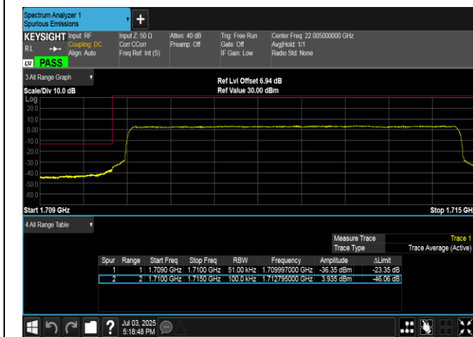
Band4-5MHz-QPSK-19975-25RB#0-PASS
