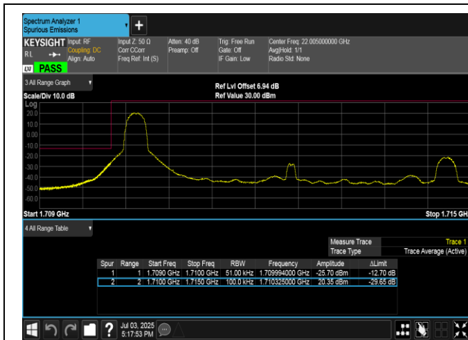
Band4-5MHz-QPSK-19975-1RB#0-PASS
