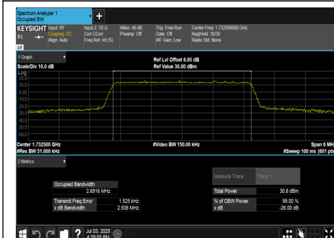
Band4-3MHz-16QAM-20175-15RB#0-PASS
