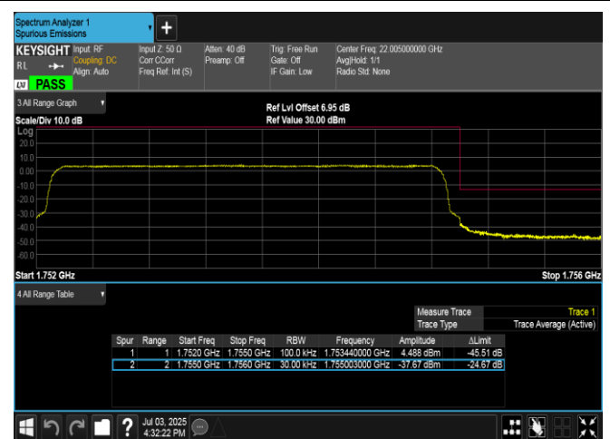
Band4-3MHz-16QAM-20385-15RB#0-PASS
