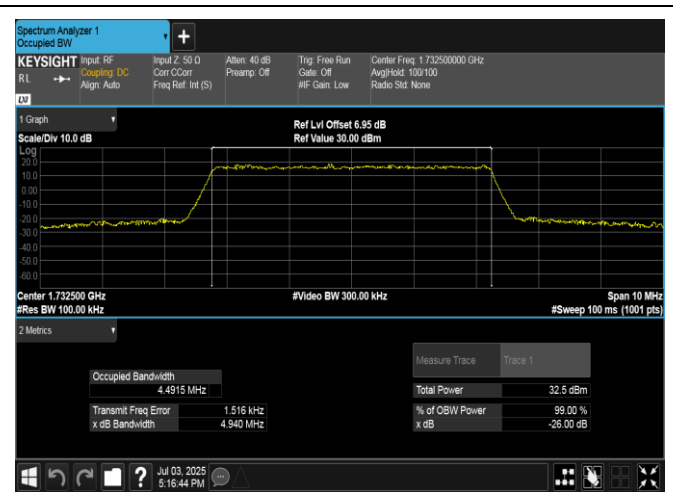
Band4-5MHz-QPSK-20175-25RB#0-PASS
