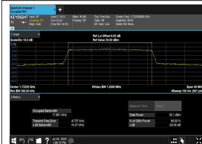
Band4-20MHz-16QAM-20175-100RB#0-PASS
