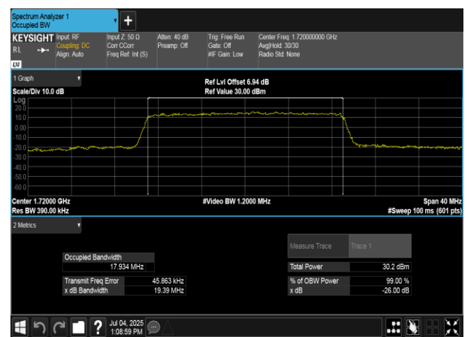
Band4-20MHz-16QAM-20050-100RB#0-PASS
