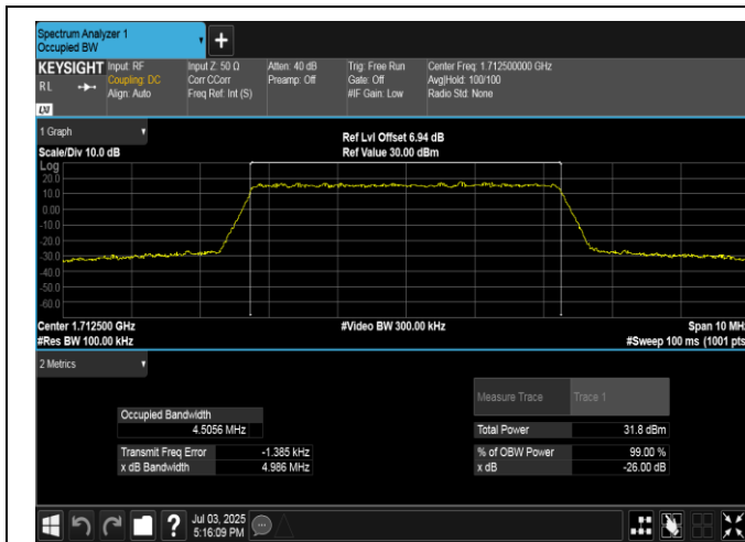
Band4-5MHz-QPSK-19975-25RB#0-PASS
