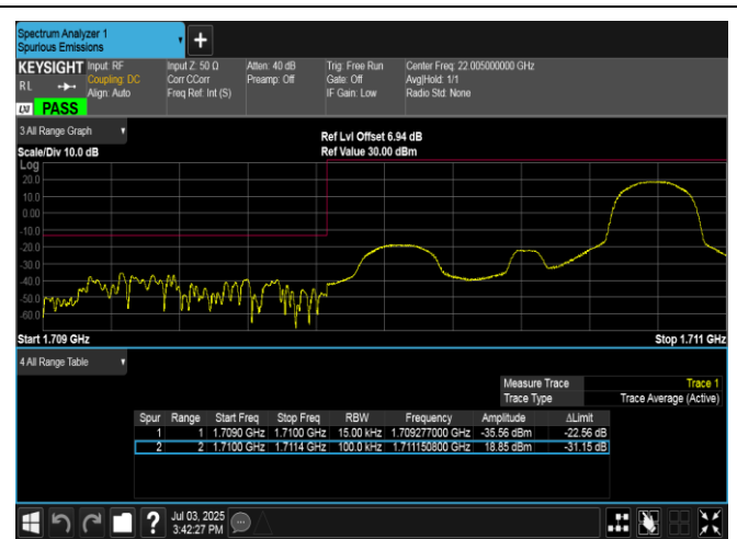
Band4-1.4MHz-16QAM-19957-1RB#5-PASS
