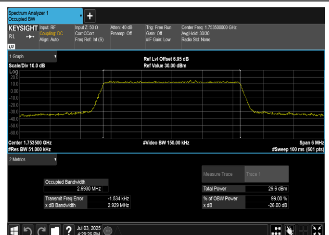
Band4-3MHz-16QAM-20385-15RB#0-PASS
