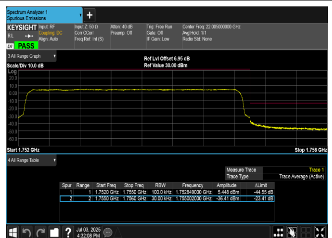
Band4-3MHz-QPSK-20385-15RB#0-PASS
