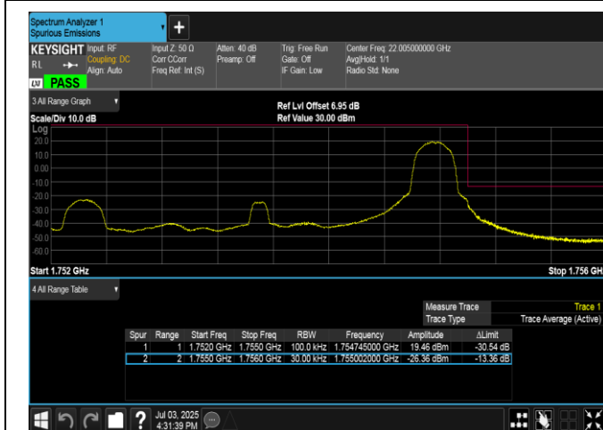
Band4-3MHz-QPSK-20385-1RB#14-PASS
