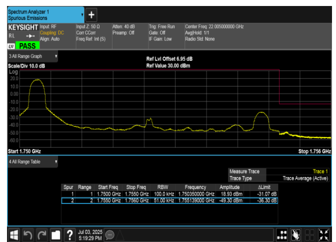
Band4-5MHz-16QAM-20375-1RB#0-PASS
