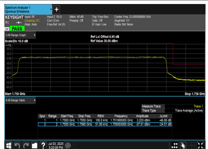
Band4-5MHz-QPSK-20375-25RB#0-PASS
