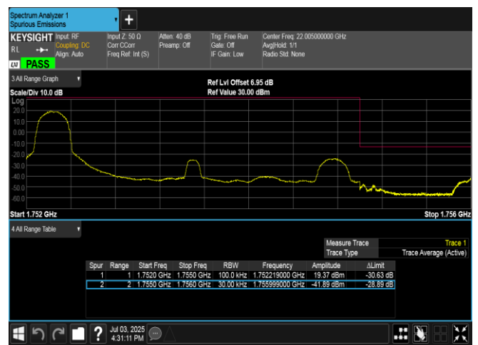
Band4-3MHz-QPSK-20385-1RB#0-PASS
