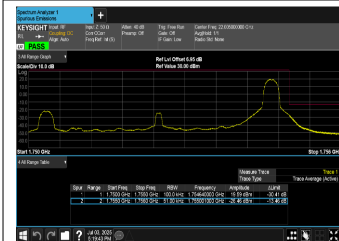
Band4-5MHz-QPSK-20375-1RB#24-PASS
