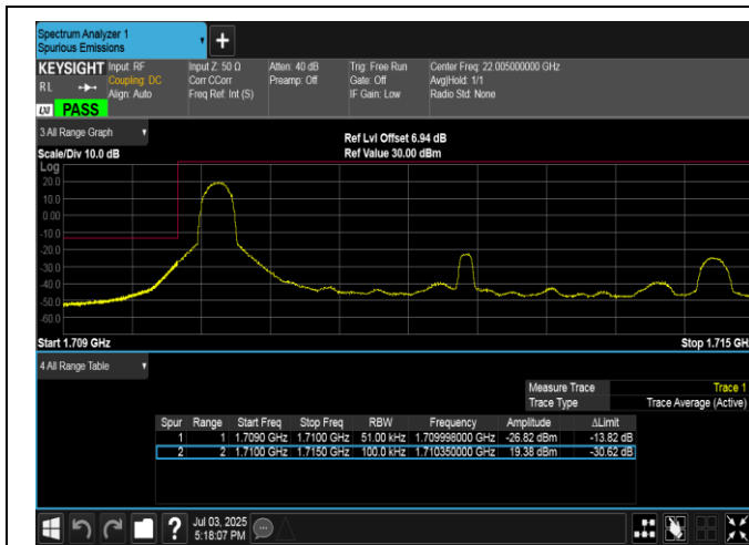
Band4-5MHz-16QAM-19975-1RB#0-PASS
