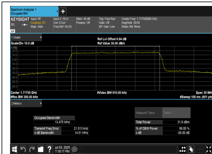
Band4-15MHz-QPSK-2025-75RB#0-PASS
