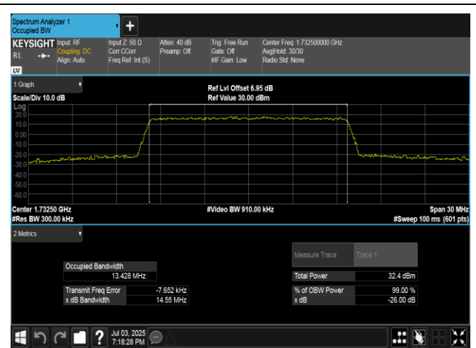
Band4-15MHz-QPSK-20175-75RB#0-PASS
