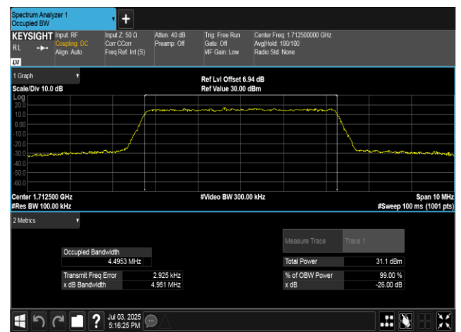
Band4-5MHz-16QAM-19975-25RB#0-PASS
