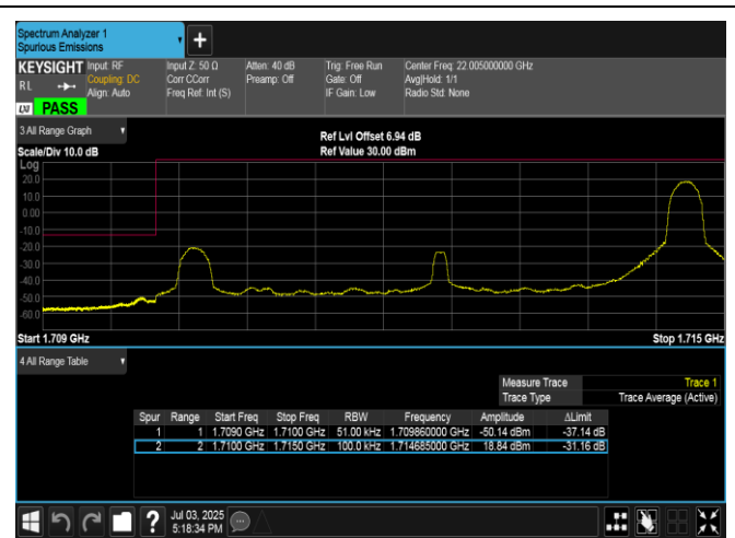
Band4-5MHz-16QAM-19975-1RB#24-PASS
