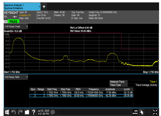
Band4-3MHz-16QAM-20385-1RB#0-PASS
