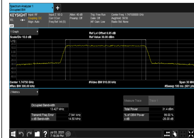
Band4-15MHz-QPSK-20325-75RB#0-PASS
