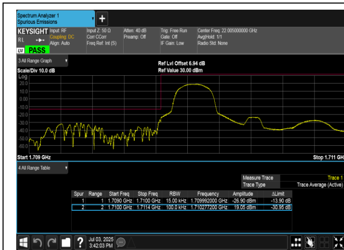
Band4-1.4MHz-16QAM-19957-1RB#0-PASS
