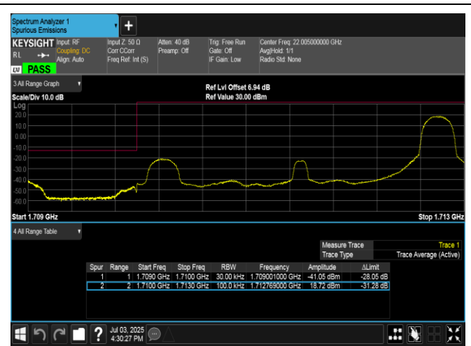
Band4-3MHz-16QAM-19965-1RB#14-PASS
