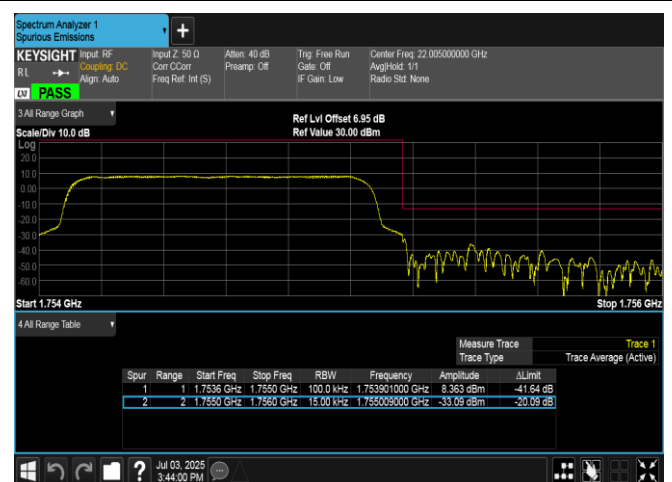
Band4-1.4MHz-16QAM-20393-6RB#0-PASS
