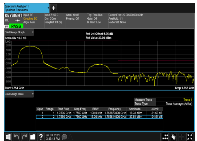
Band4-1.4MHz-16QAM-20393-1RB#0-PASS
