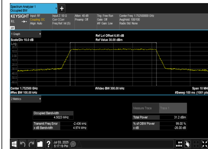
Band4-5MHz-QPSK-20375-25RB#0-PASS
