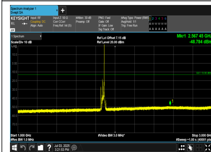
Band2-20MHz-16QAM-18900-1RB#99-1000~3000-PASS
