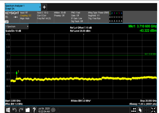
Band2-20MHz-16QAM-18700-100RB#0-3000~20000-PASS
