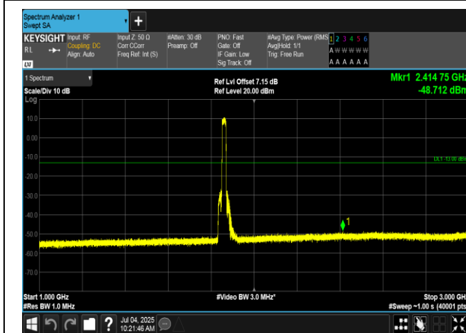
Band2-20MHz-16QAM-18700-100RB#0-1000~3000-PASS
