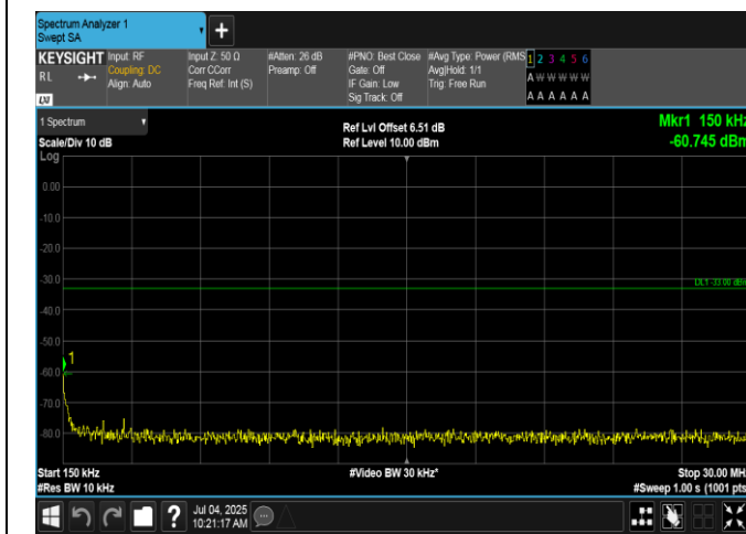
Band2-20MHz-16QAM-18700-100RB#0-0.15~30-PASS
