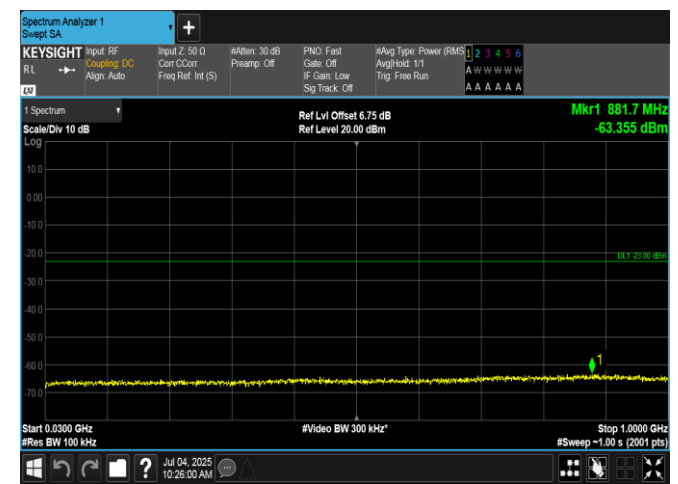
Band2-20MHz-16QAM-19100-100RB#0-30~1000-PASS
