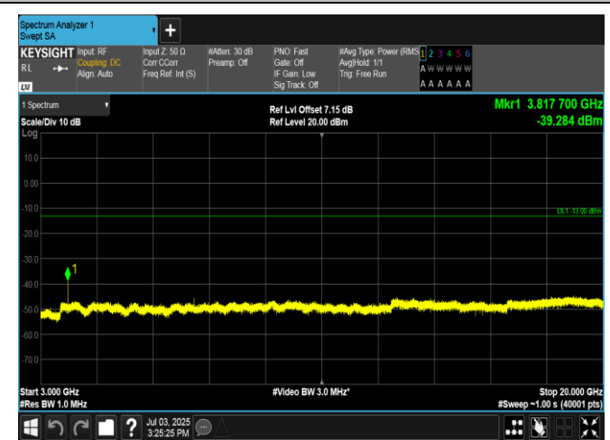
Band2-20MHz-QPSK-19100-1RB#99-3000~20000-PASS
