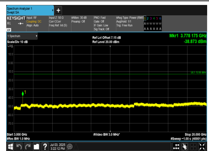
Band2-20MHz-16QAM-18900-1RB#99-3000~20000-PASS
