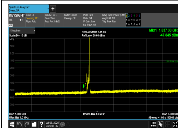
Band2-20MHz-QPSK-19100-1RB#99-1000~3000-PASS
