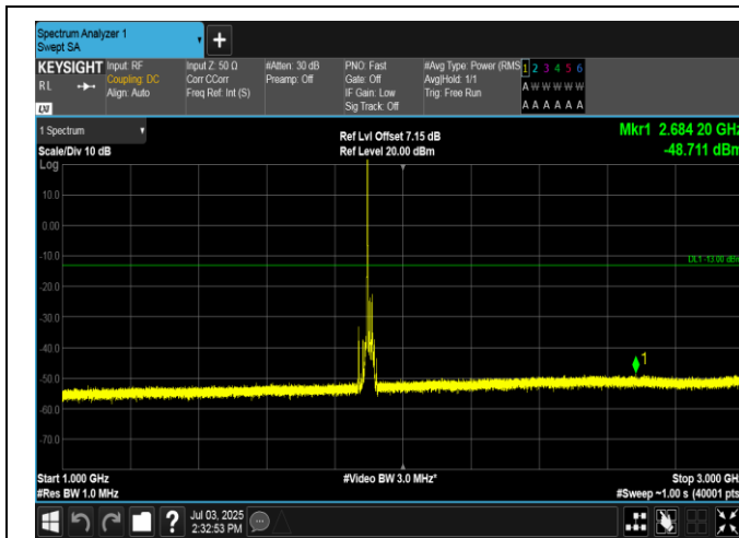
Band2-15MHz-16QAM-19125-1RB#0-1000~3000-PASS
