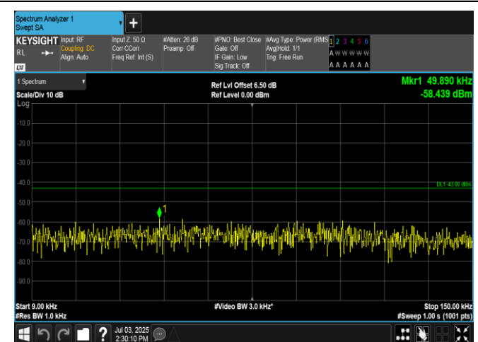
Band2-15MHz-16QAM-18900-1RB#74-0.009~0.15-PASS
