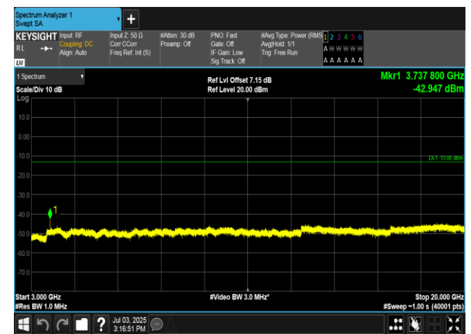
Band2-20MHz-QPSK-18700-1RB#99-3000~20000-PASS
