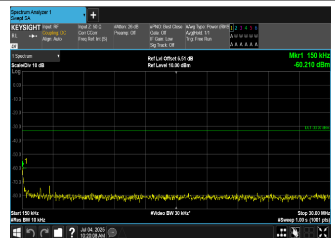
Band2-20MHz-QPSK-18700-100RB#0-0.15~30-PASS
