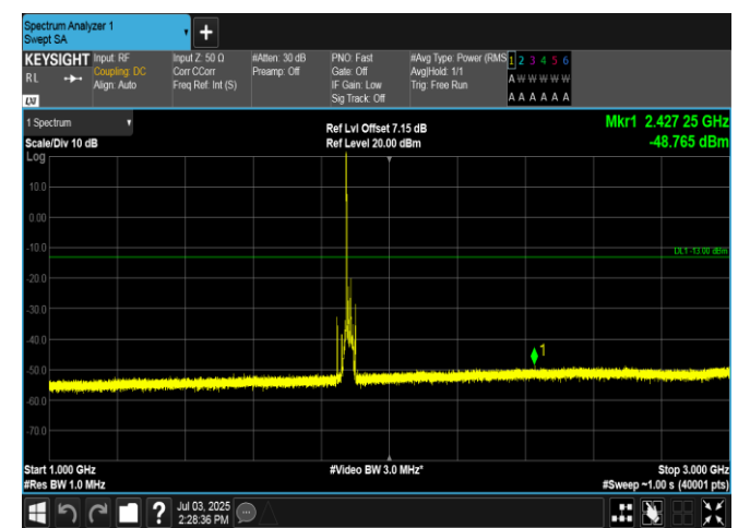
Band2-15MHz-16QAM-18900-1RB#0-1000~3000-PASS
