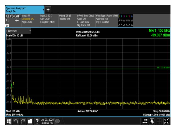
Band2-15MHz-16QAM-18900-1RB#0-0.15~30-PASS
