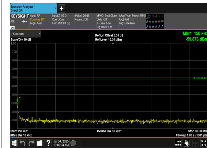
Band2-15MHz-16QAM-19125-75RB#0-0.15~30-PASS
