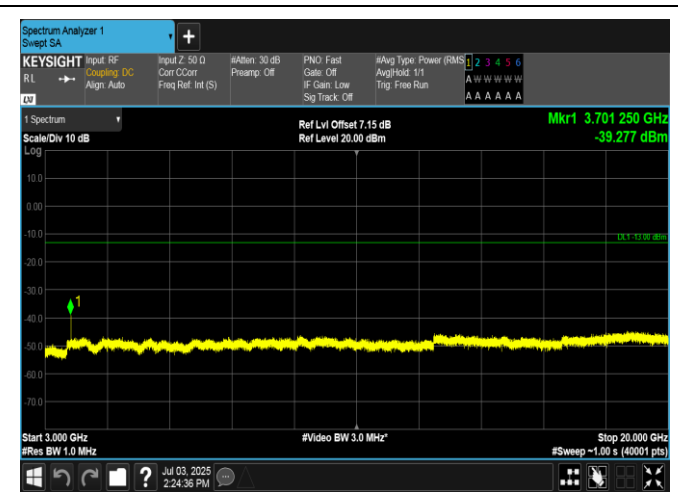
Band2-15MHz-16QAM-18675-1RB#0-3000~20000-PASS
