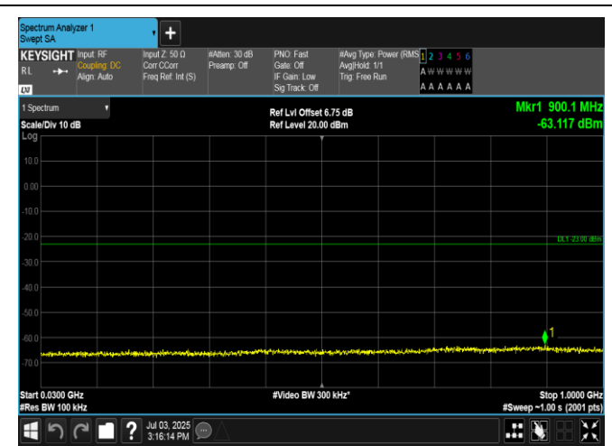
Band2-20MHz-QPSK-18700-1RB#99-30~1000-PASS
