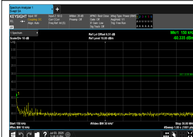
Band2-20MHz-QPSK-18900-1RB#0-0.15~30-PASS
