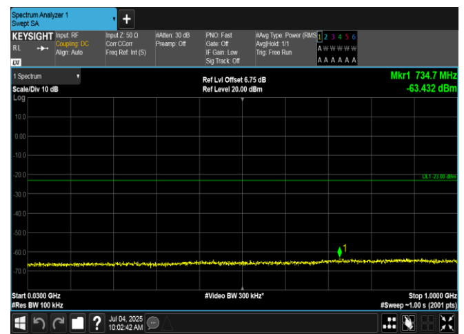
Band2-15MHz-16QAM-19125-75RB#0-30~1000-PASS
