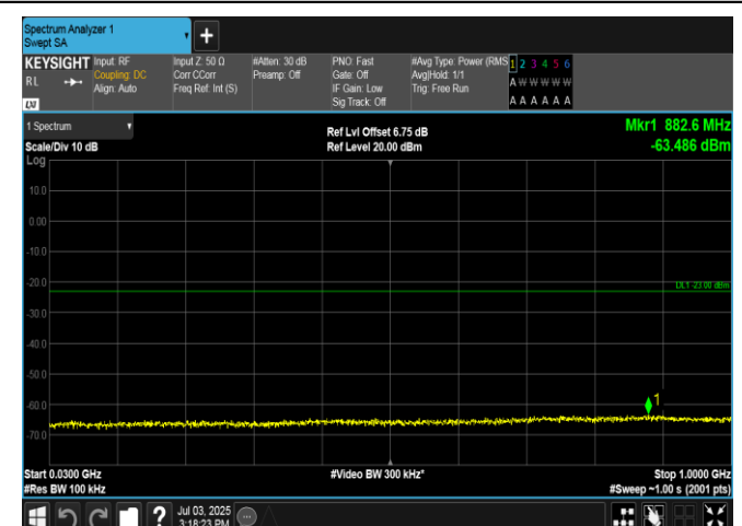
Band2-20MHz-QPSK-18900-1RB#0-30~1000-PASS
