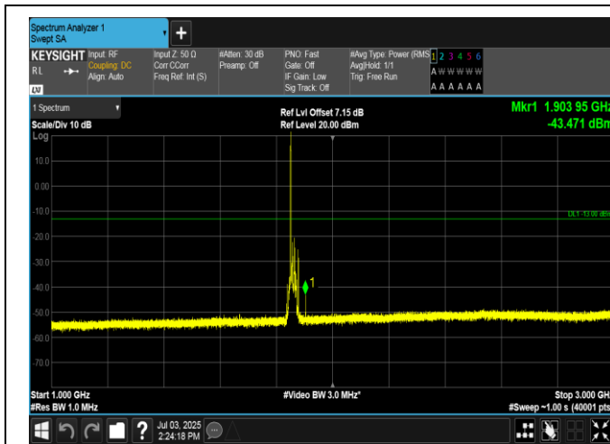
Band2-15MHz-16QAM-18675-1RB#0-1000~3000-PASS
