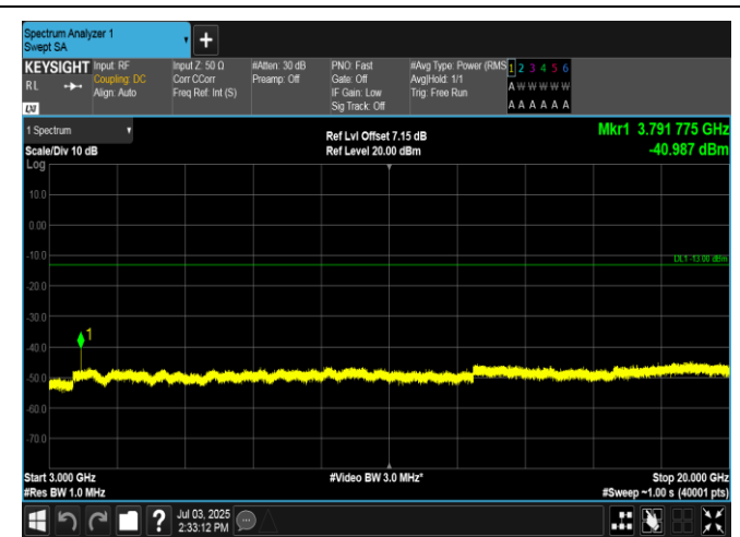
Band2-15MHz-16QAM-19125-1RB#0-3000~20000-PASS
