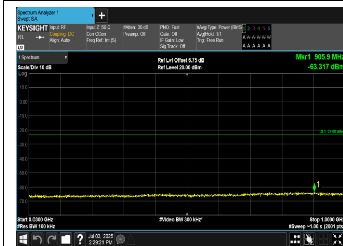
Band2-15MHz-QPSK-18900-1RB#74-30~1000-PASS
