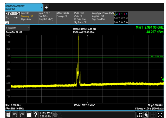
Band2-15MHz-QPSK-18900-1RB#74-1000~3000-PASS
