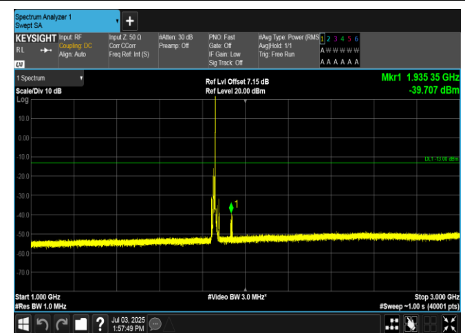
Band2-10MHz-16QAM-18650-1RB#49-1000~3000-PASS
