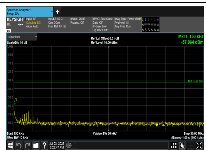
Band2-15MHz-QPSK-18675-1RB#0-0.15~30-PASS
