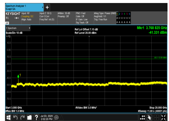
Band2-10MHz-16QAM-18900-1RB#49-3000~20000-PASS
