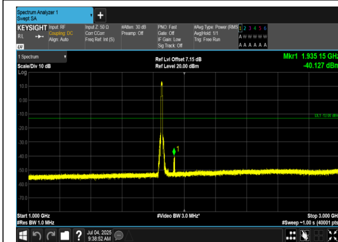
Band2-10MHz-16QAM-18650-50RB#0-1000~3000-PASS
