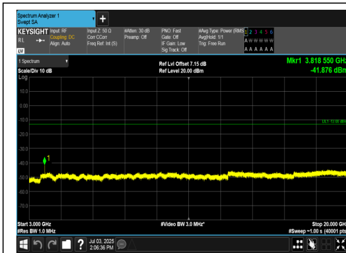
Band2-10MHz-16QAM-19150-1RB#49-3000~20000-PASS
