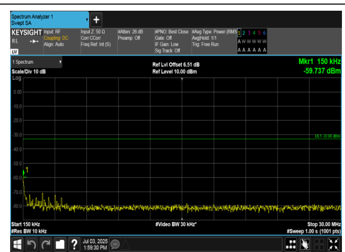
Band2-10MHz-16QAM-18900-1RB#0-0.15~30-PASS
