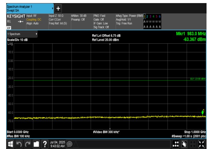
Band2-10MHz-16QAM-19150-50RB#0-30~1000-PASS
