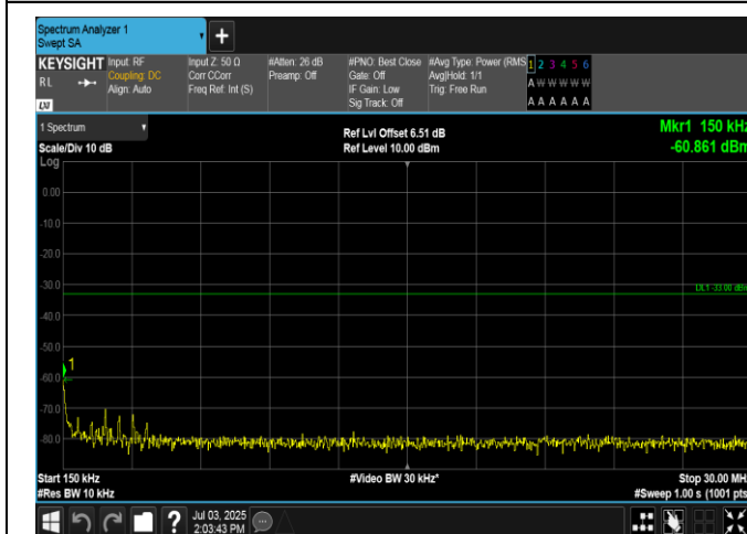
Band2-10MHz-16QAM-19150-1RB#0-0.15~30-PASS
