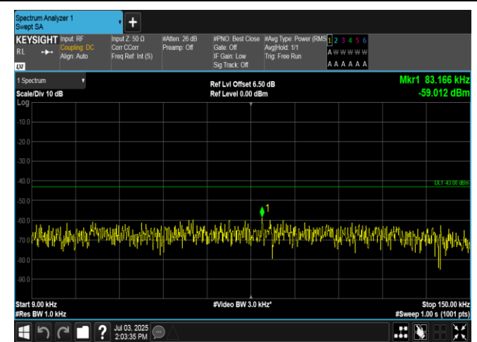
Band2-10MHz-16QAM-19150-1RB#0-0.009~0.15-PASS
