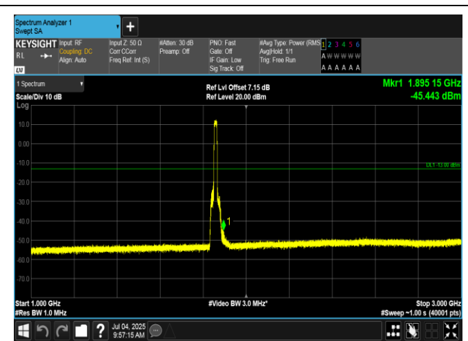
Band2-15MHz-QPSK-18675-75RB#0-1000~3000-PASS
