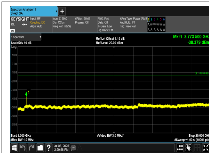
Band2-15MHz-QPSK-18900-1RB#74-3000~20000-PASS
