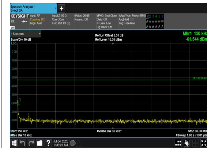
Band2-10MHz-16QAM-18650-50RB#0-0.15~30-PASS
