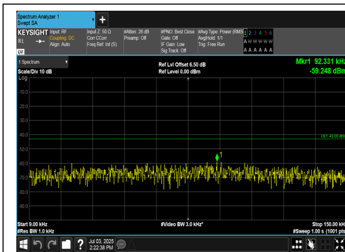
Band2-15MHz-QPSK-18675-1RB#0-0.009~0.15-PASS
