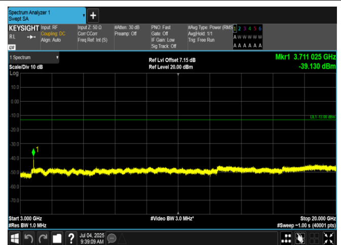
Band2-10MHz-16QAM-18650-50RB#0-3000~20000-PASS
