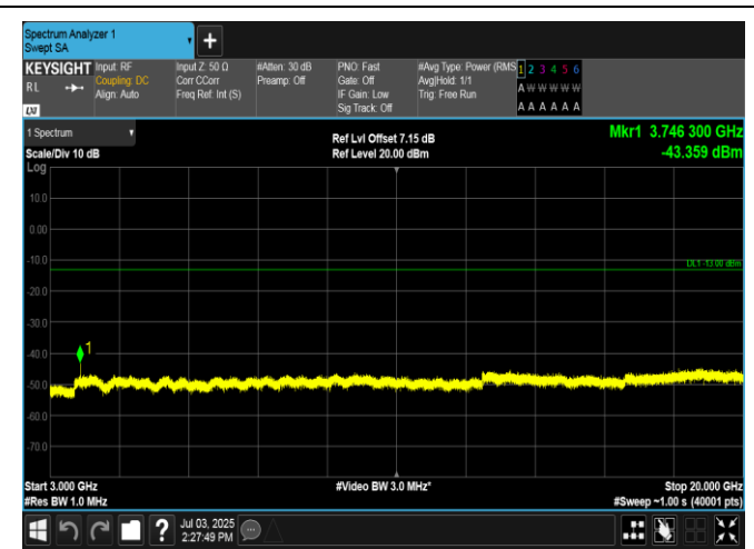
Band2-15MHz-QPSK-18900-1RB#0-3000~20000-PASS
