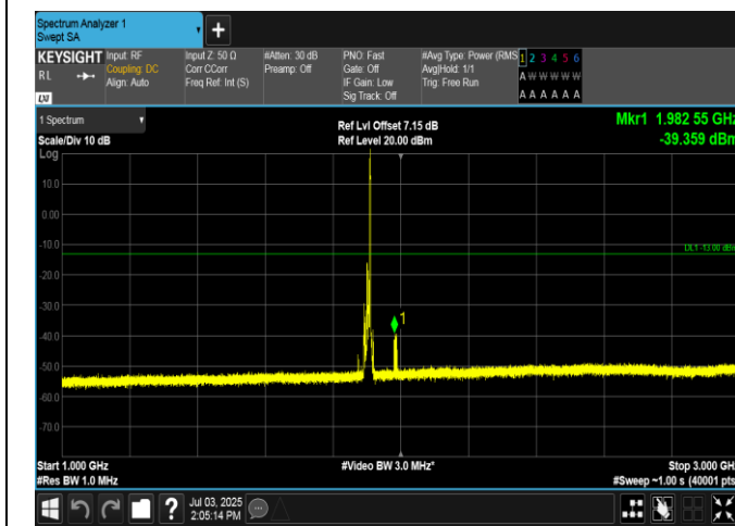
Band2-10MHz-QPSK-19150-1RB#49-1000~3000-PASS
