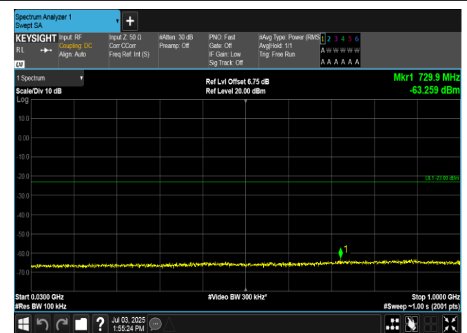
Band2-10MHz-16QAM-18650-1RB#0-30~1000-PASS
