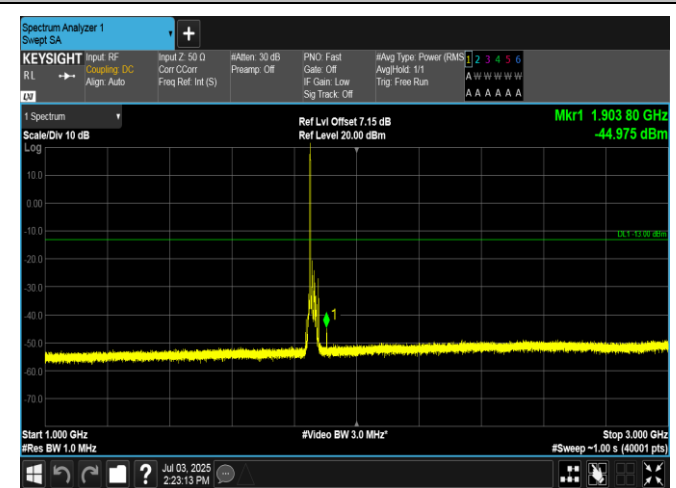
Band2-15MHz-QPSK-18675-1RB#0-1000~3000-PASS
