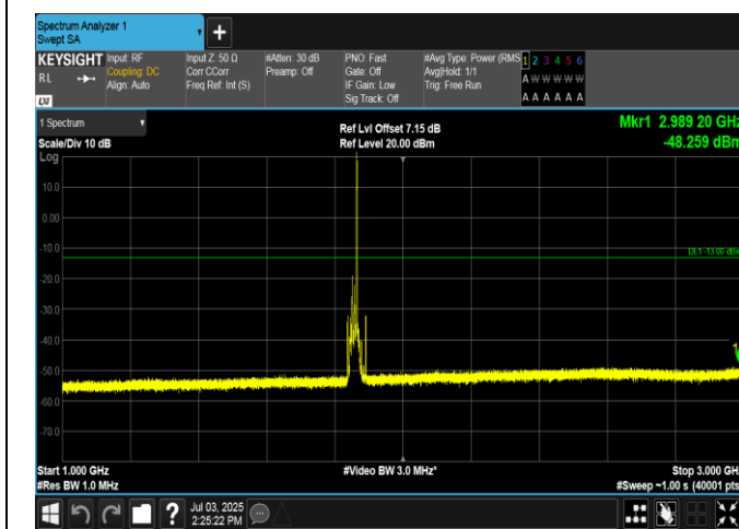
Band2-15MHz-QPSK-18675-1RB#74-1000~3000-PASS
