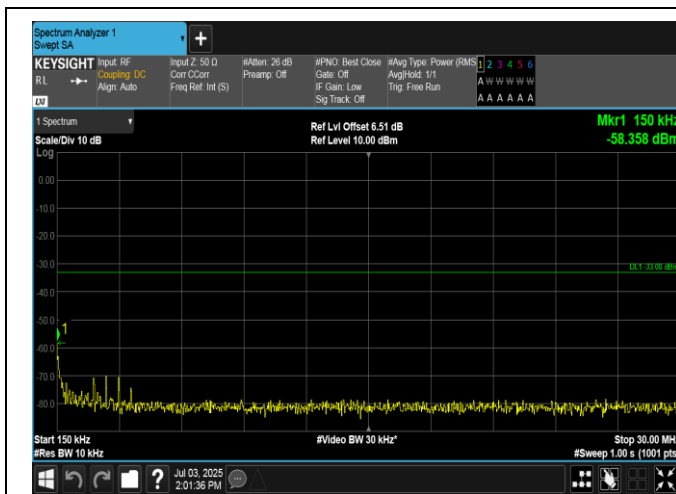
Band2-10MHz-16QAM-18900-1RB#49-0.15~30-PASS
