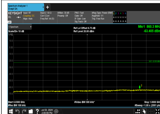
Band2-10MHz-16QAM-19150-1RB#49-30~1000-PASS
