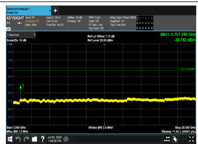
Band2-10MHz-16QAM-18650-1RB#0-3000~20000-PASS
