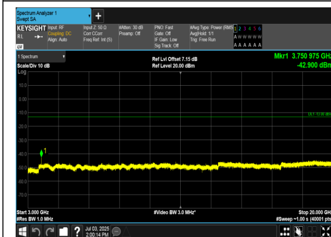
Band2-10MHz-16QAM-18900-1RB#0-3000~20000-PASS
