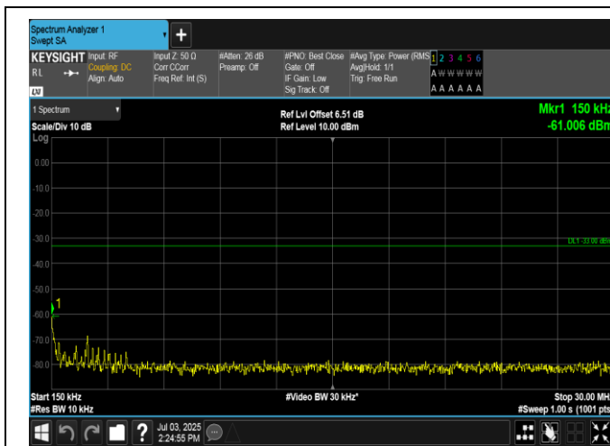
Band2-15MHz-QPSK-18675-1RB#74-0.15~30-PASS
