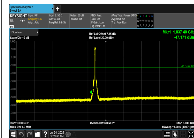
Band2-15MHz-QPSK-18900-75RB#0-1000~3000-PASS
