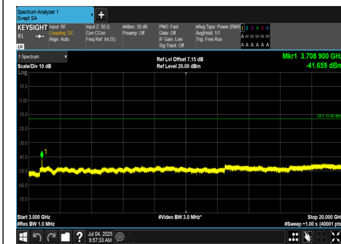
Band2-15MHz-QPSK-18675-75RB#0-3000~20000-PASS
