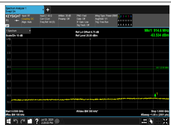
Band2-15MHz-QPSK-18675-1RB#74-30~1000-PASS
