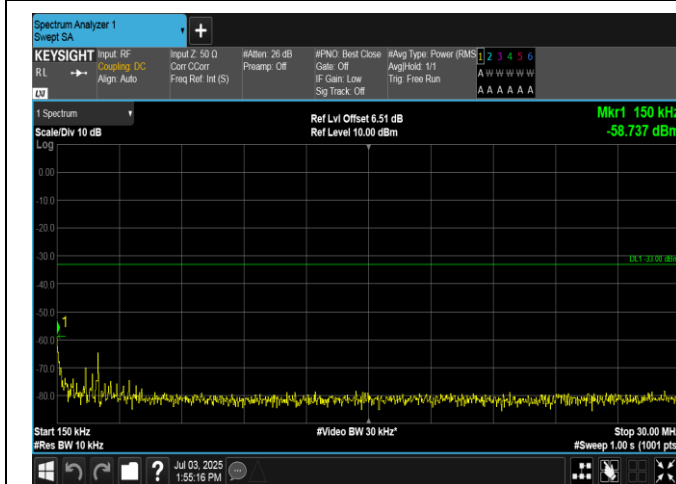
Band2-10MHz-16QAM-18650-1RB#0-0.15~30-PASS
