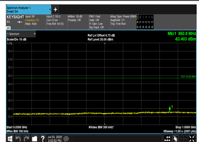
Band2-10MHz-16QAM-19150-1RB#0-30~1000-PASS
