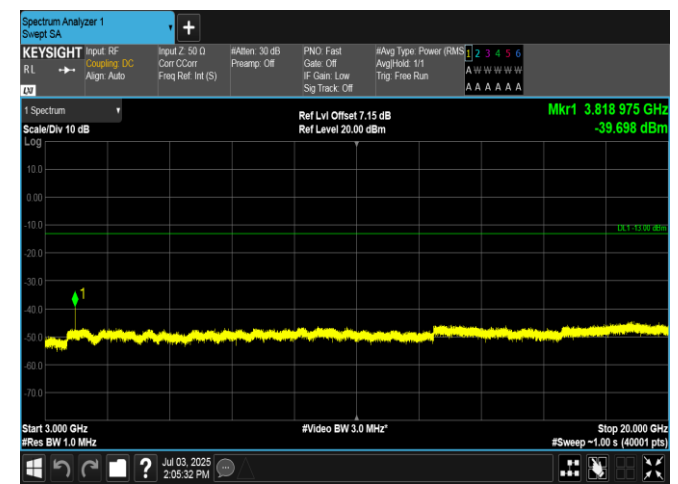
Band2-10MHz-QPSK-19150-1RB#49-3000~20000-PASS
