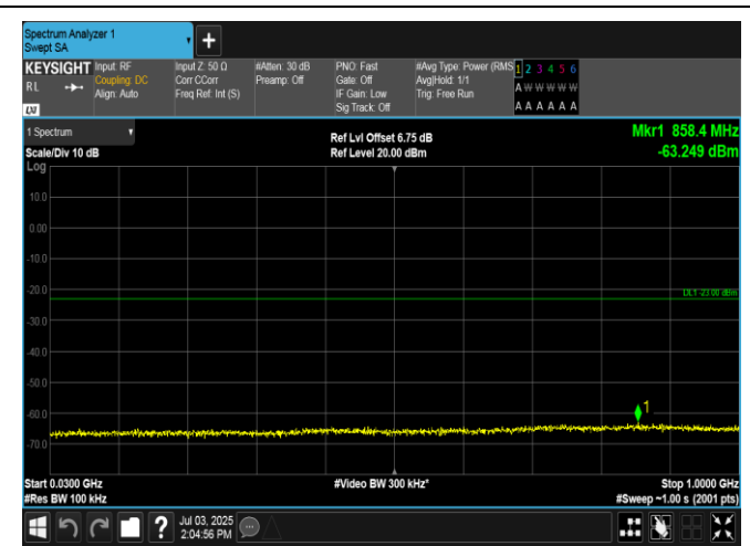
Band2-10MHz-QPSK-19150-1RB#49-30~1000-PASS
