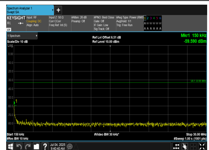
Band2-10MHz-16QAM-18900-50RB#0-0.15~30-PASS
