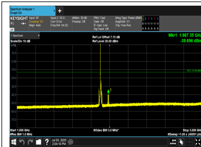
Band2-10MHz-16QAM-19150-1RB#0-1000~3000-PASS
