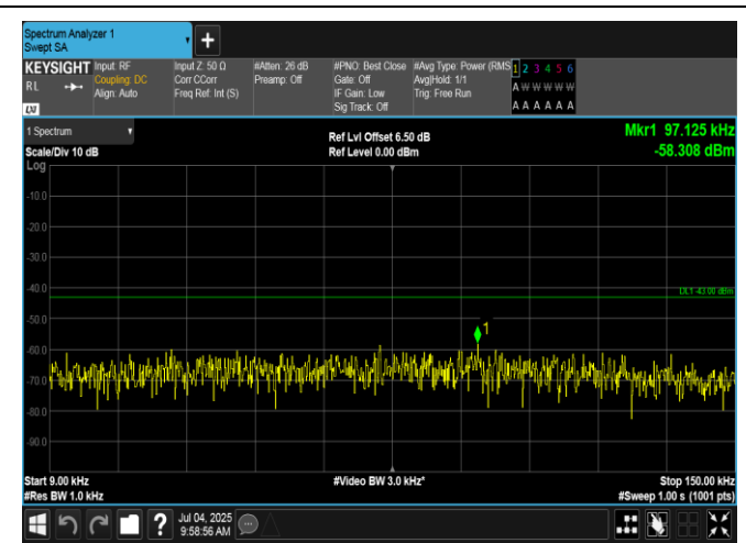
Band2-15MHz-QPSK-18900-75RB#0-0.009~0.15-PASS
