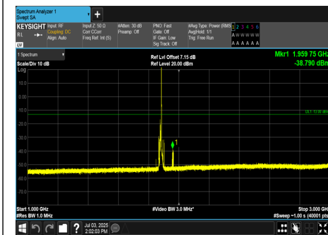
Band2-10MHz-16QAM-18900-1RB#49-1000~3000-PASS
