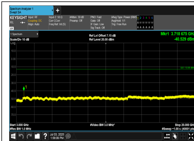
Band2-10MHz-16QAM-18650-1RB#49-3000~20000-PASS
