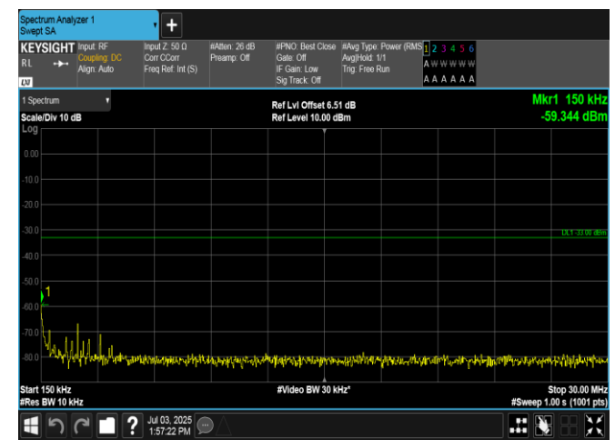
Band2-10MHz-16QAM-18650-1RB#49-0.15~30-PASS
