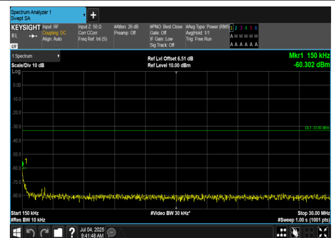
Band2-10MHz-QPSK-19150-50RB#0-0.15~30-PASS
