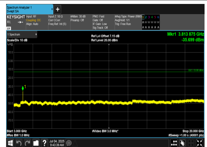
Band2-10MHz-16QAM-19150-50RB#0-3000~20000-PASS
