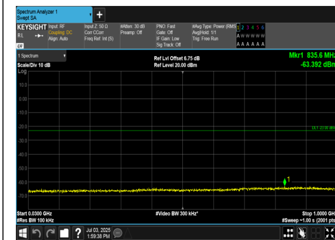
Band2-10MHz-16QAM-18900-1RB#0-30~1000-PASS
