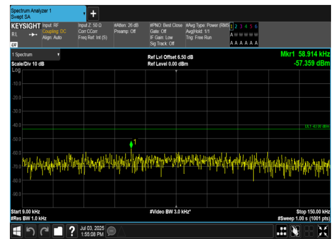
Band2-10MHz-16QAM-18650-1RB#0-0.009~0.15-PASS
