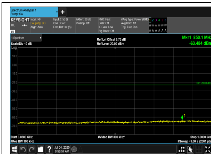
Band2-15MHz-QPSK-18675-75RB#0-30~1000-PASS
