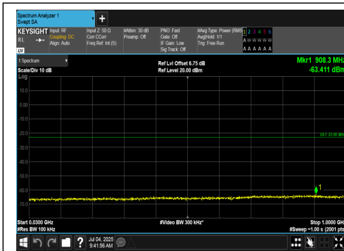
Band2-10MHz-QPSK-19150-50RB#0-30~1000-PASS
