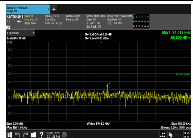
Band2-10MHz-16QAM-18900-1RB#49-0.009~0.15-PASS
