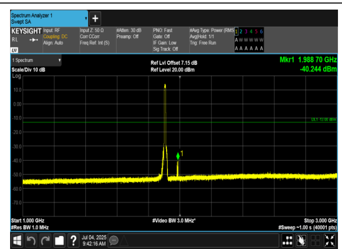
Band2-10MHz-QPSK-19150-50RB#0-1000~3000-PASS
