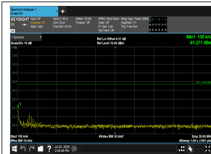
Band2-10MHz-QPSK-19150-1RB#49-0.15~30-PASS
