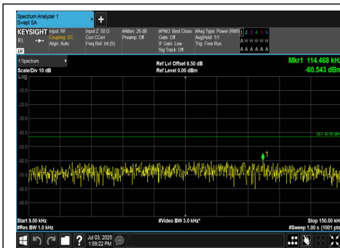
Band2-10MHz-16QAM-18900-1RB#0-0.009~0.15-PASS
