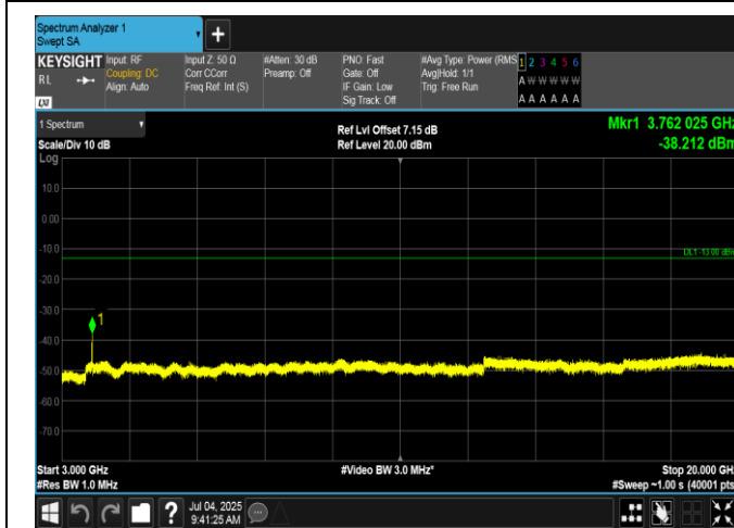
Band2-10MHz-16QAM-18900-50RB#0-3000~20000-PASS
