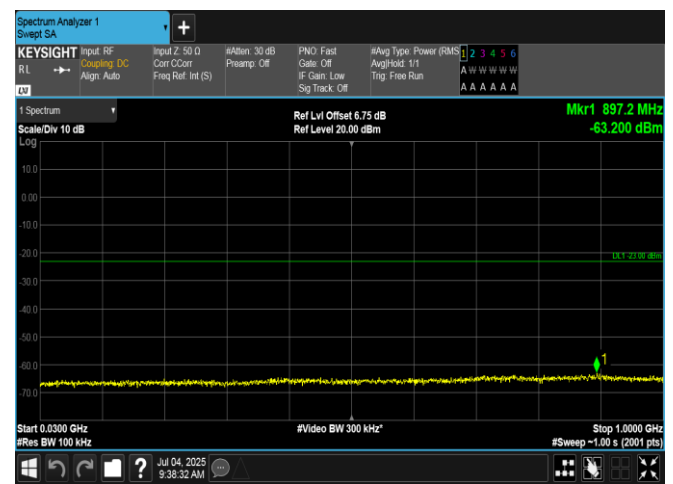
Band2-10MHz-16QAM-18650-50RB#0-30~1000-PASS
