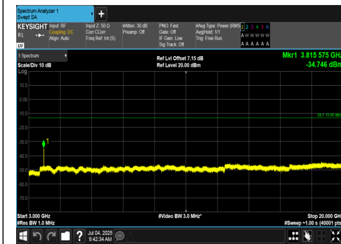
Band2-10MHz-QPSK-19150-50RB#0-3000~20000-PASS
