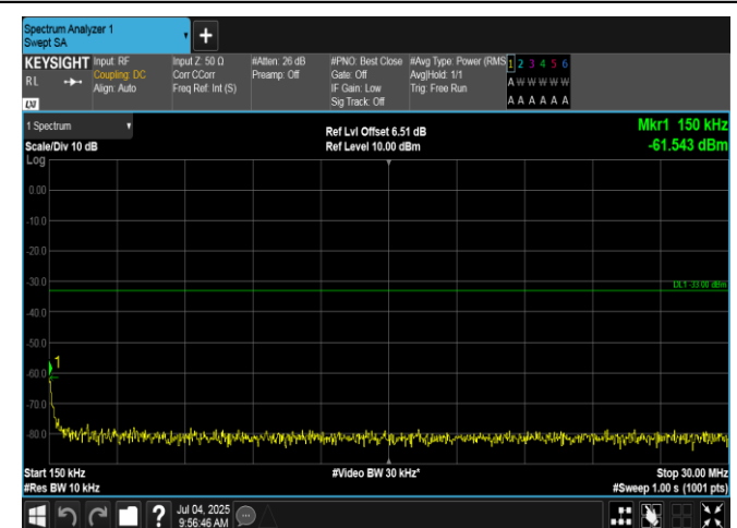
Band2-15MHz-QPSK-18675-75RB#0-0.15~30-PASS
