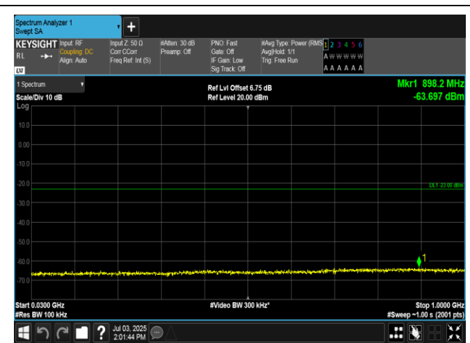
Band2-10MHz-16QAM-18900-1RB#49-30~1000-PASS
