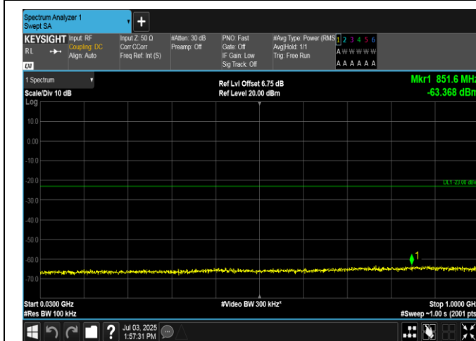
Band2-10MHz-16QAM-18650-1RB#49-30~1000-PASS
