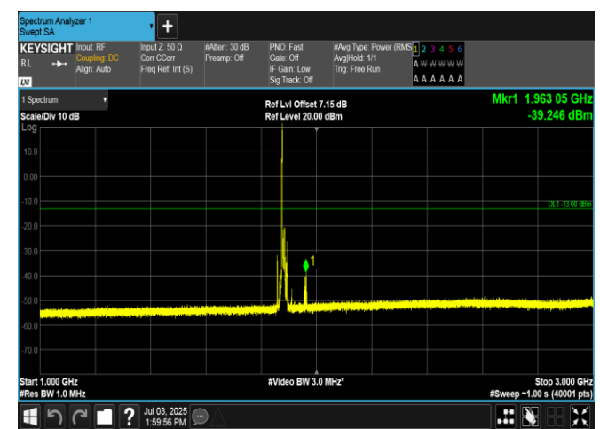
Band2-10MHz-16QAM-18900-1RB#0-1000~3000-PASS
