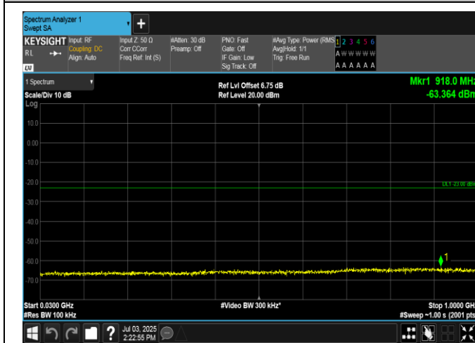
Band2-15MHz-QPSK-18675-1RB#0-30~1000-PASS
