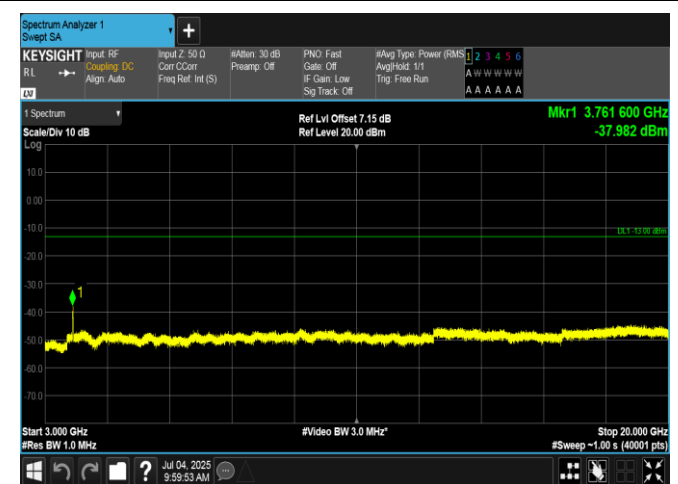
Band2-15MHz-QPSK-18900-75RB#0-3000~20000-PASS
