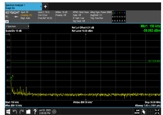
Band2-10MHz-16QAM-19150-1RB#49-0.15~30-PASS
