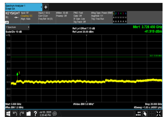
Band2-15MHz-QPSK-18675-1RB#74-3000~20000-PASS
