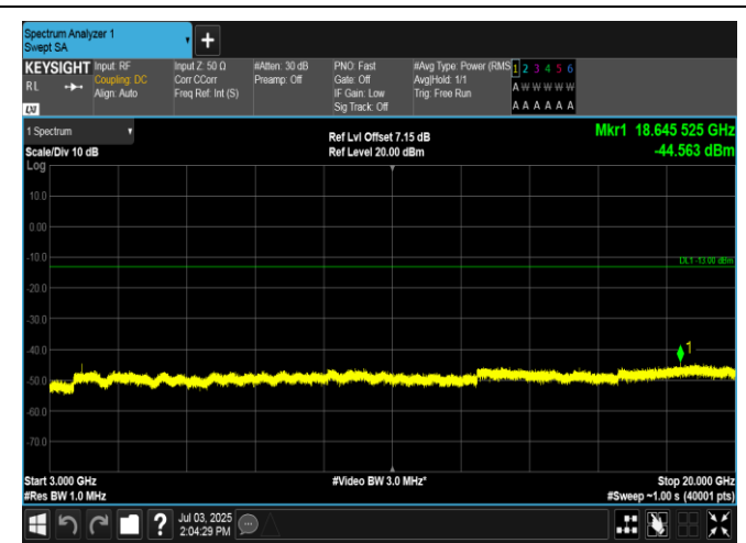
Band2-10MHz-16QAM-19150-1RB#0-3000~20000-PASS
