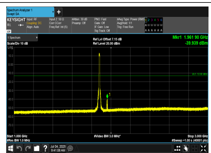
Band2-10MHz-16QAM-18900-50RB#0-1000~3000-PASS
