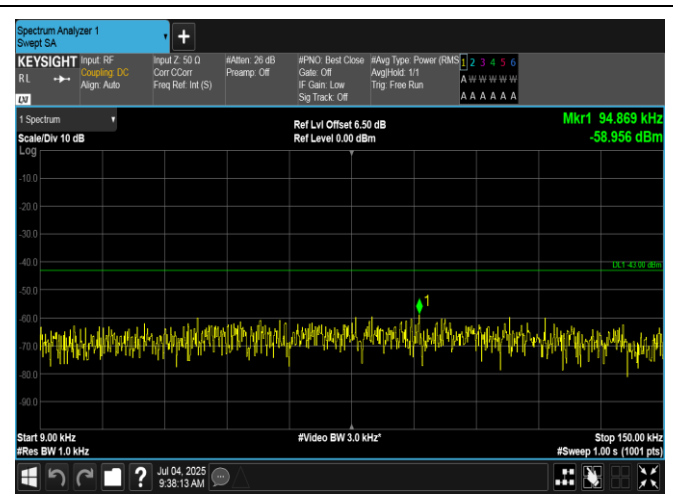
Band2-10MHz-16QAM-18650-50RB#0-0.009~0.15-PASS
