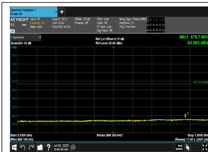
Band2-10MHz-16QAM-18900-50RB#0-30~1000-PASS
