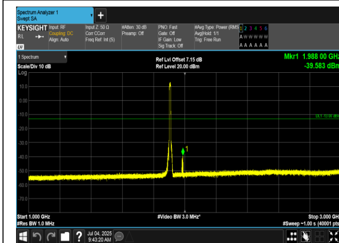
Band2-10MHz-16QAM-19150-50RB#0-1000~3000-PASS
