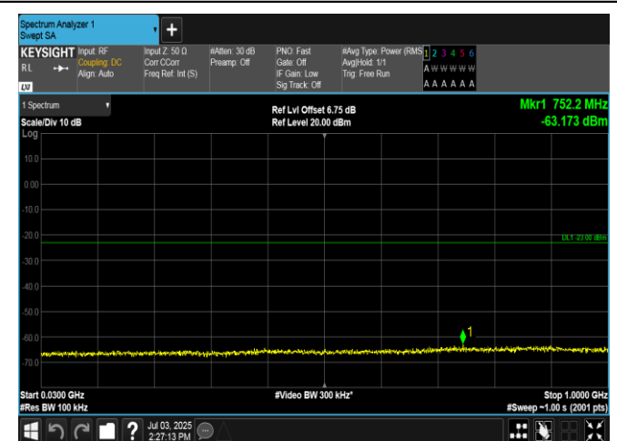
Band2-15MHz-QPSK-18900-1RB#0-30~1000-PASS
