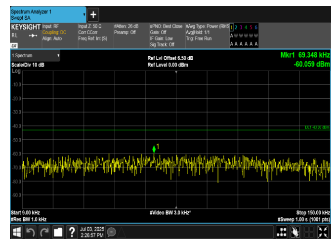
Band2-15MHz-QPSK-18900-1RB#0-0.009~0.15-PASS
