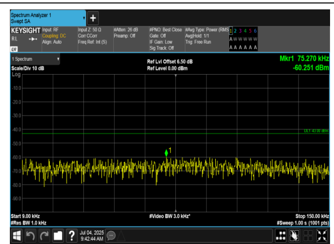
Band2-10MHz-16QAM-19150-50RB#0-0.009~0.15-PASS
