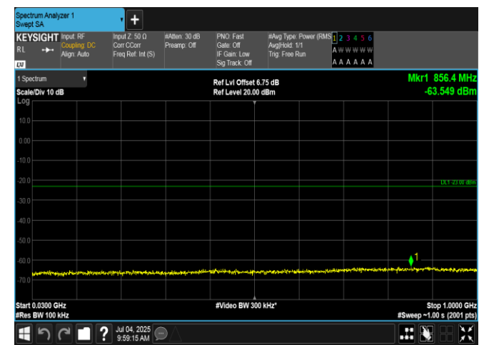
Band2-15MHz-QPSK-18900-75RB#0-30~1000-PASS
