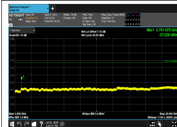
Band2-15MHz-QPSK-18675-1RB#0-3000~20000-PASS
