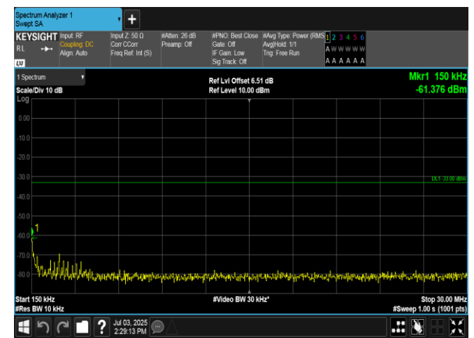
Band2-15MHz-QPSK-18900-1RB#74-0.15~30-PASS
