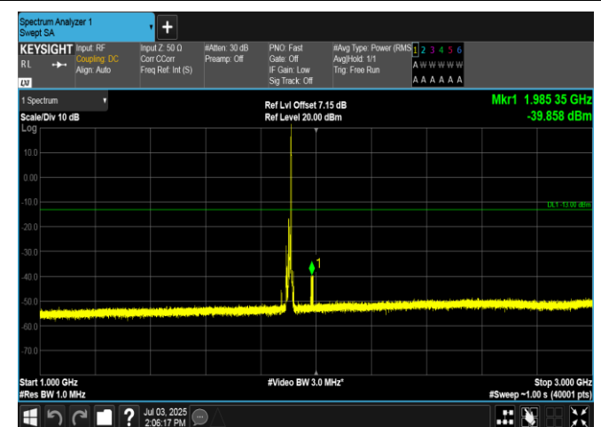
Band2-10MHz-16QAM-19150-1RB#49-1000~3000-PASS
