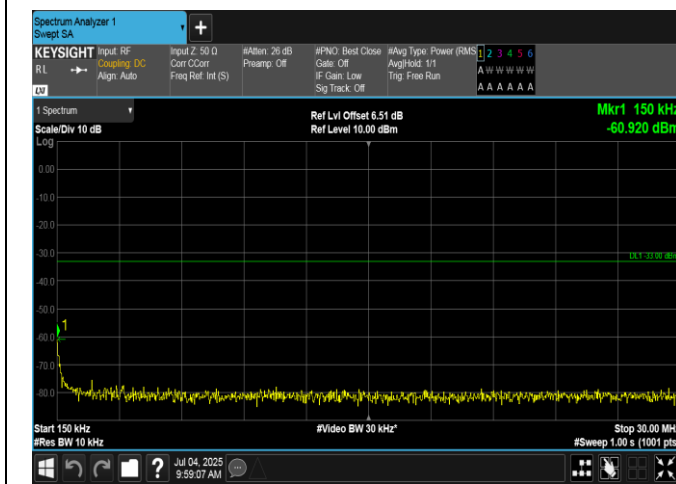
Band2-15MHz-QPSK-18900-75RB#0-0.15~30-PASS
