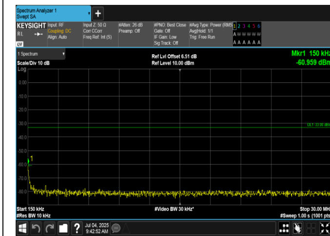
Band2-10MHz-16QAM-19150-50RB#0-0.15~30-PASS
