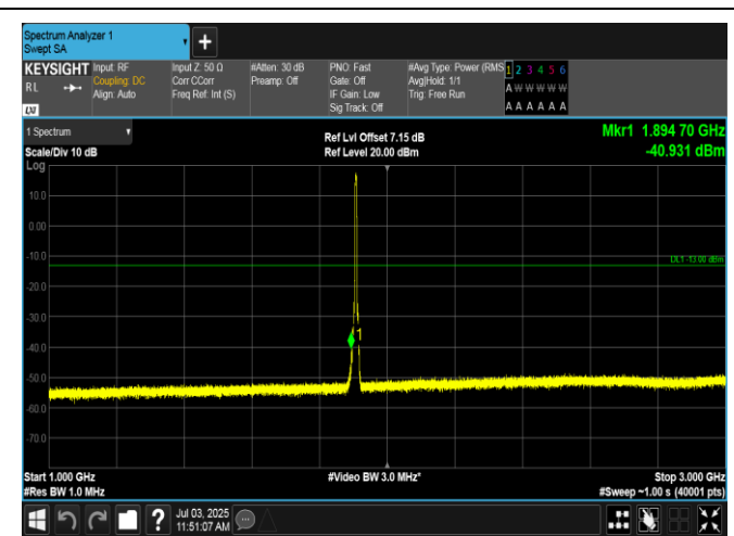
Band2-5MHz-QPSK-19175-25RB#0-1000~3000-PASS
