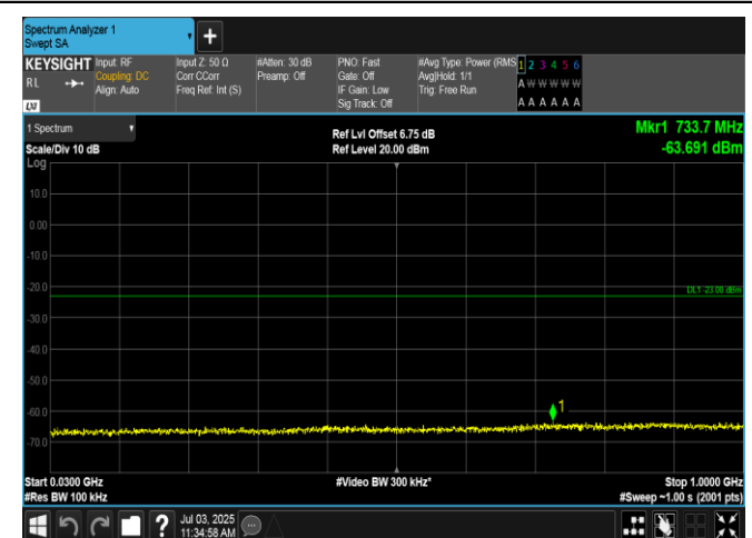
Band2-5MHz-16QAM-18625-1RB#0-30~1000-PASS
