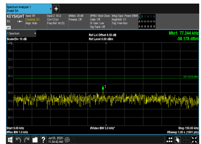
Band2-5MHz-16QAM-18625-1RB#0-0.009~0.15-PASS
