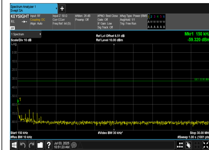
Band2-3MHz-16QAM-18615-15RB#0-0.15~30-PASS
