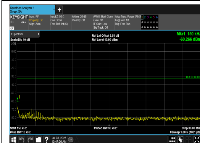
Band2-3MHz-16QAM-18615-1RB#0-0.15~30-PASS
