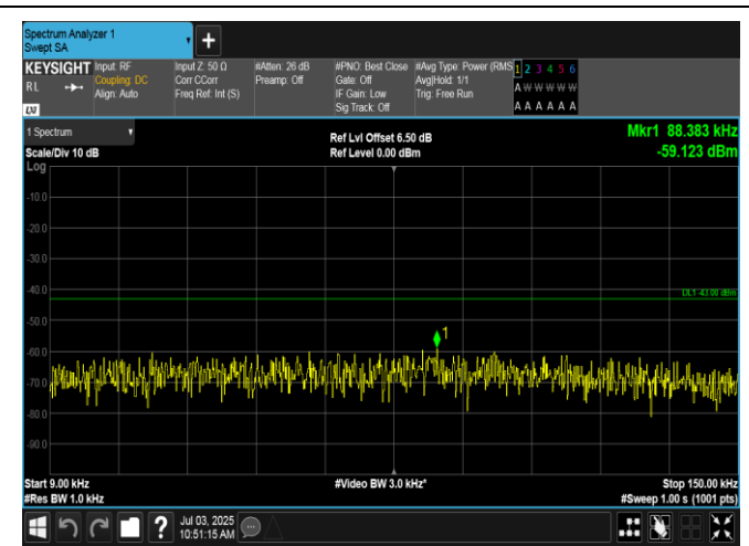
Band2-3MHz-16QAM-18615-15RB#0-0.009~0.15-PASS
