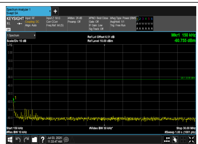
Band2-5MHz-QPSK-18625-1RB#0-0.15~30-PASS
