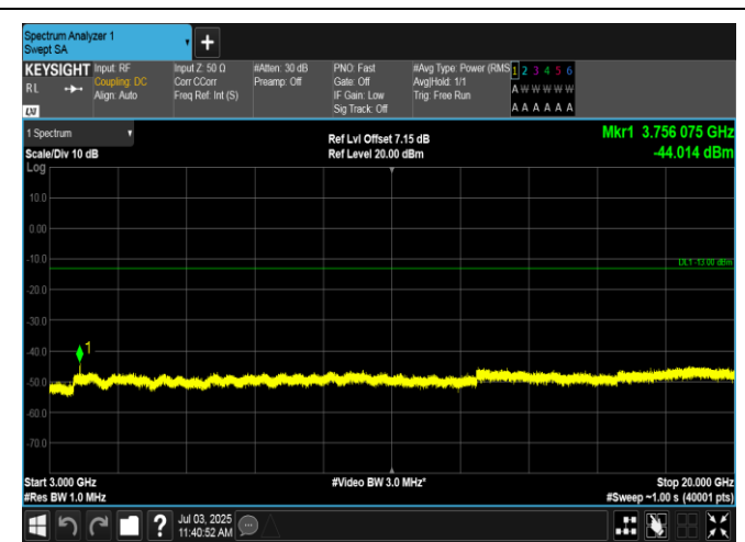
Band2-5MHz-QPSK-18900-1RB#0-3000~20000-PASS
