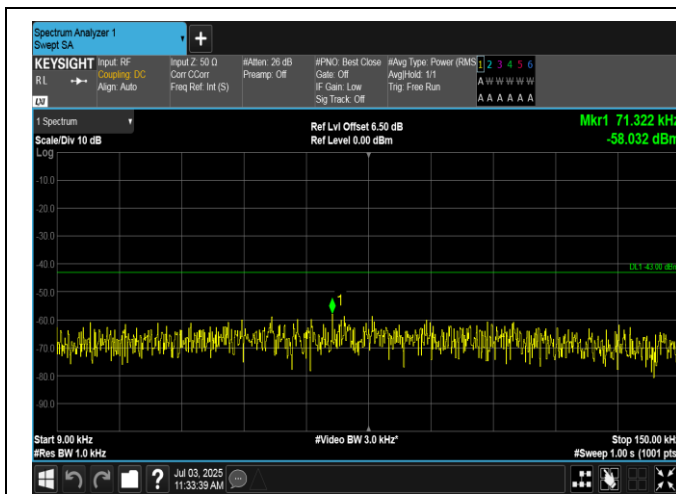
Band2-5MHz-QPSK-18625-1RB#0-0.009~0.15-PASS
