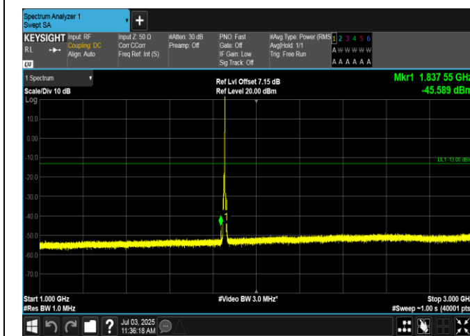
Band2-5MHz-QPSK-18625-1RB#24-1000~3000-PASS
