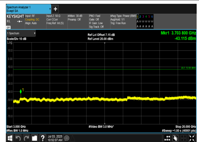
Band2-3MHz-16QAM-18615-15RB#0-3000~20000-PASS
