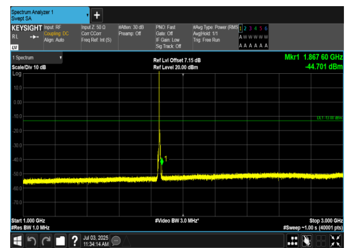
Band2-5MHz-QPSK-18625-1RB#0-1000~3000-PASS
