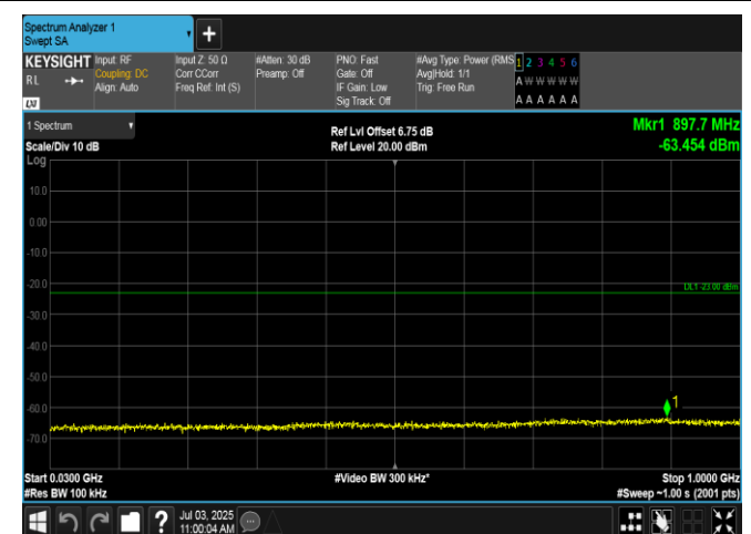
Band2-3MHz-16QAM-19185-1RB#0-30~1000-PASS
