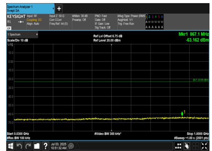
Band2-3MHz-16QAM-18615-15RB#0-30~1000-PASS
