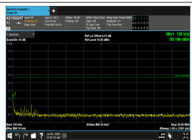
Band2-3MHz-16QAM-18900-1RB#0-0.15~30-PASS
