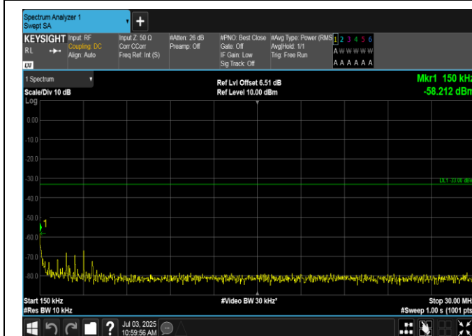
Band2-3MHz-16QAM-19185-1RB#0-0.15~30-PASS
