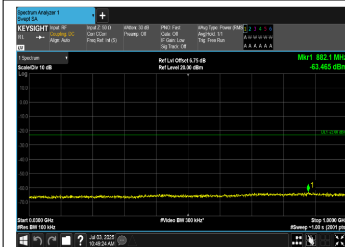
Band2-3MHz-16QAM-18615-1RB#14-30-1000-PASS
