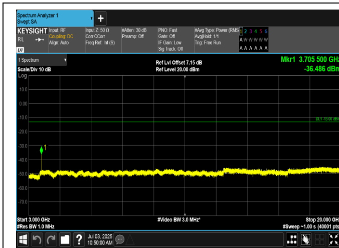
Band2-3MHz-16QAM-18615-1RB#14-3000~20000-PASS
