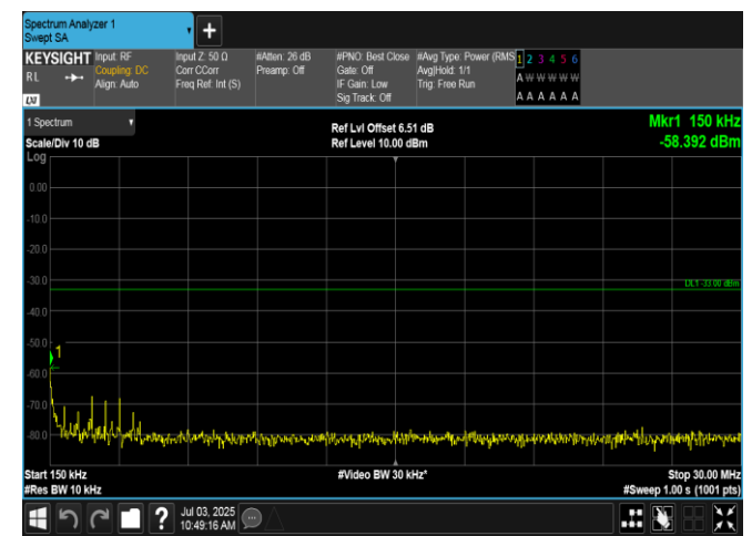
Band2-3MHz-16QAM-18615-1RB#14-0.15-30-PASS
