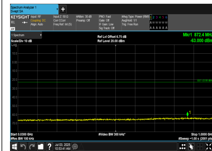
Band2-3MHz-16QAM-18900-1RB#0-30~1000-PASS
