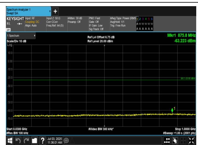
Band2-5MHz-QPSK-18625-1RB#24-30~1000-PASS
