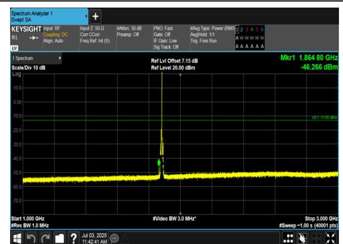
Band2-5MHz-QPSK-18900-1RB#24-1000~3000-PASS
