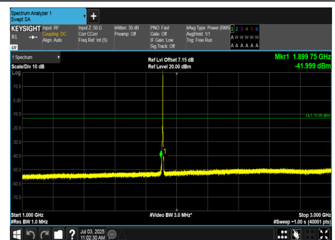
Band2-3MHz-16QAM-19185-1RB#14-1000-3000-PASS
