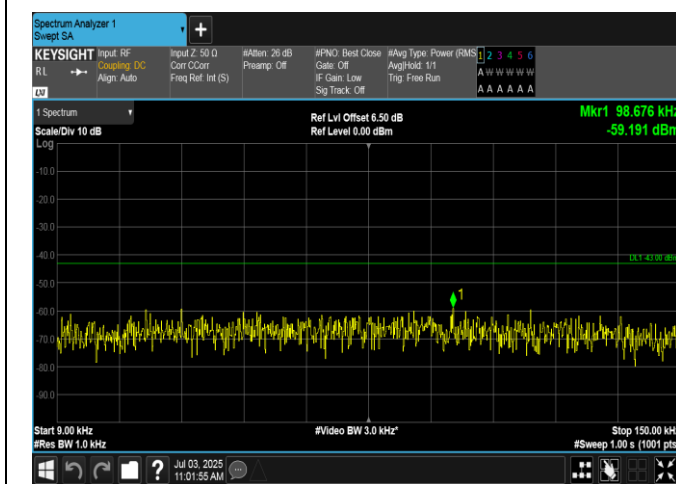
Band2-3MHz-16QAM-19185-1RB#14-0.009-0.15-PASS
