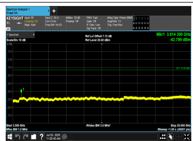
Band2-3MHz-16QAM-19185-1RB#0-3000-20000-PASS
