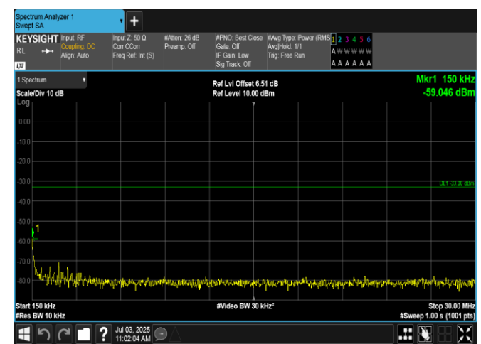
Band2-3MHz-16QAM-19185-1RB#14-0.15-30-PASS
