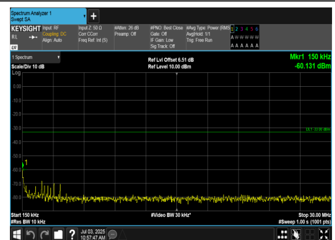
Band2-3MHz-16QAM-18900-15RB#0-0.15~30-PASS
