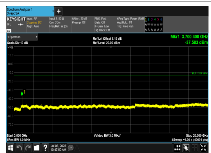
Band2-3MHz-16QAM-18615-1RB#0-3000-20000-PASS
