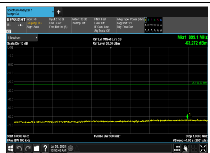
Band2-3MHz-16QAM-18900-1RB#14-30~1000-PASS
