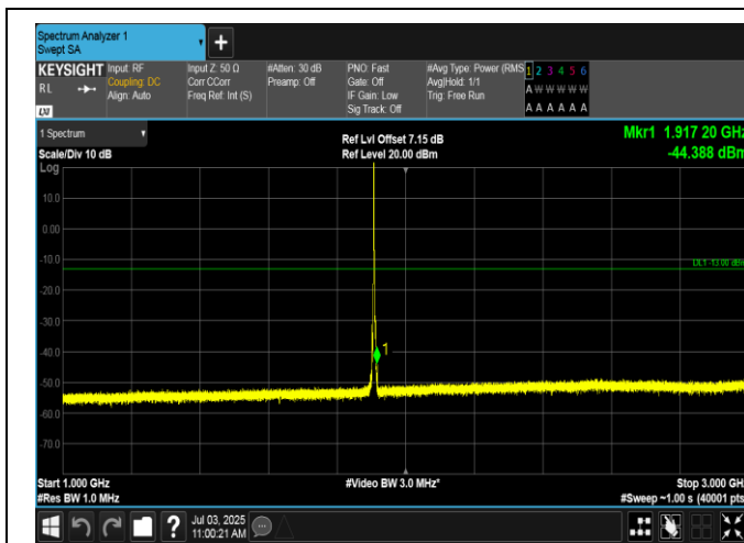
Band2-3MHz-16QAM-19185-1RB#0-1000-3000-PASS
