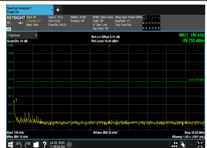
Band2-5MHz-QPSK-18625-25RB#0-0.15~30-PASS
