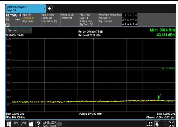
Band2-3MHz-16QAM-18615-1RB#0-30~1000-PASS
