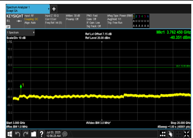
Band2-3MHz-16QAM-18900-1RB#14-3000~20000-PASS
