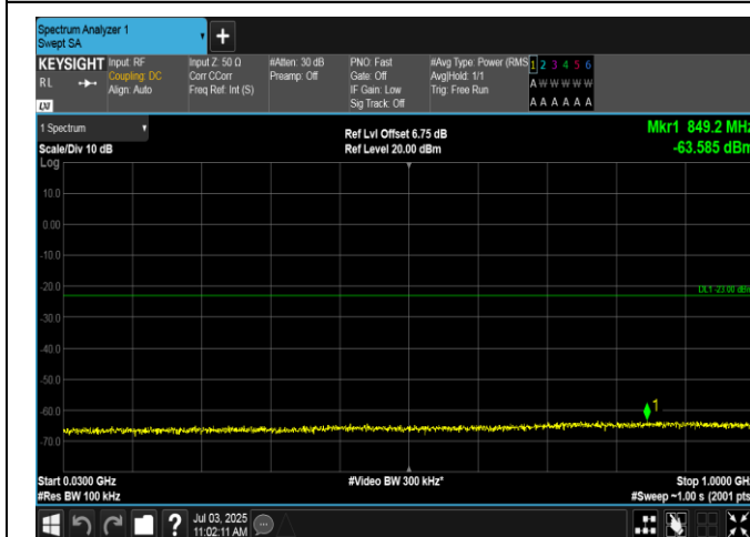
Band2-3MHz-16QAM-19185-1RB#14-30-1000-PASS
