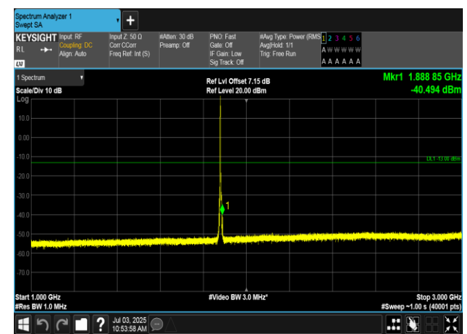
Band2-3MHz-16QAM-18900-1RB#0-1000~3000-PASS
