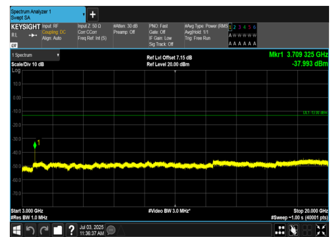
Band2-5MHz-QPSK-18625-1RB#24-3000~20000-PASS
