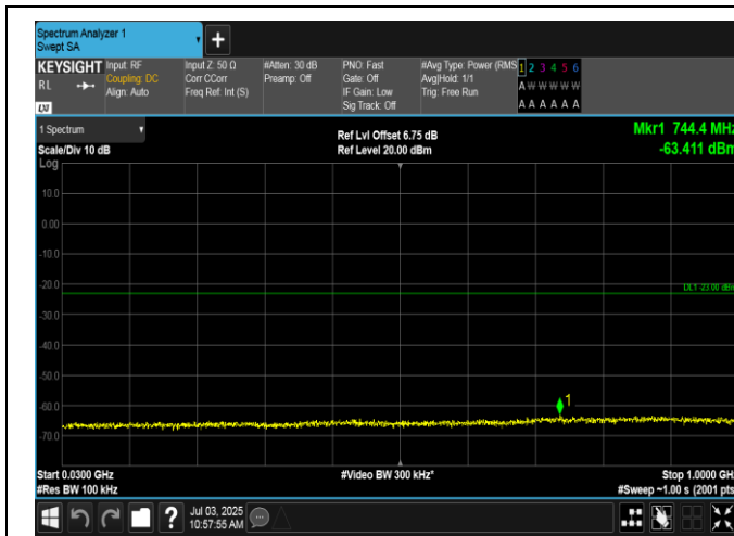
Band2-3MHz-16QAM-18900-15RB#0-30~1000-PASS
