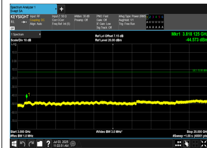
Band2-3MHz-QPSK-19185-15RB#0-3000~20000-PASS
