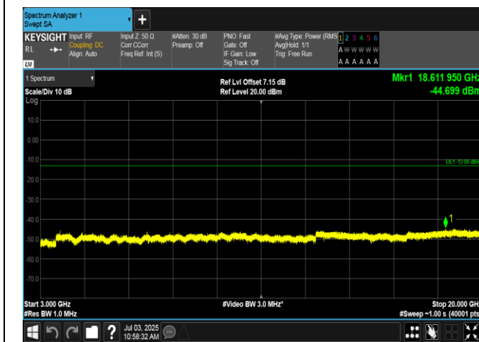
Band2-3MHz-16QAM-18900-15RB#0-3000~20000-PASS
