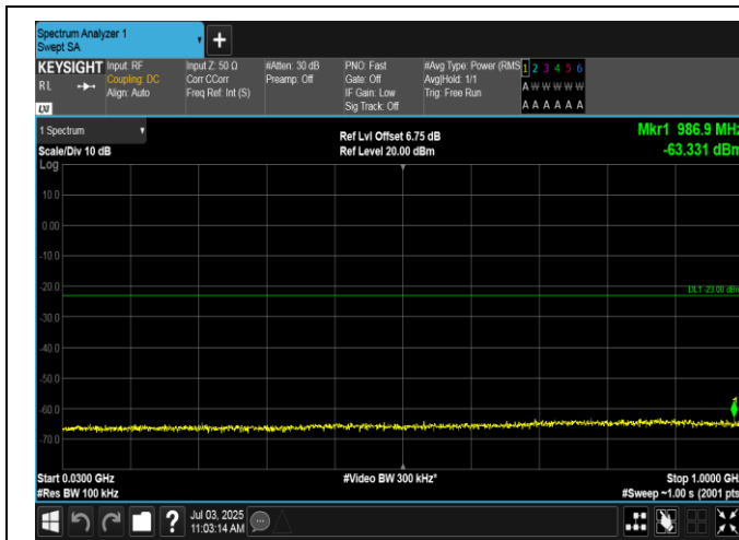
Band2-3MHz-QPSK-19185-15RB#0-30~1000-PASS
