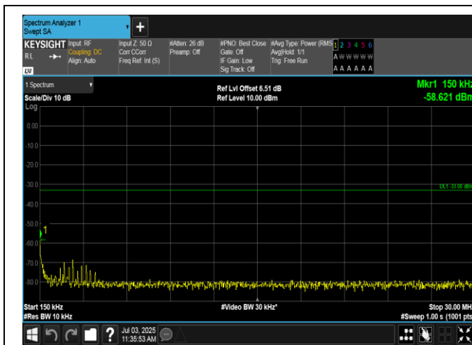
Band2-5MHz-QPSK-18625-1RB#24-0.15~30-PASS
