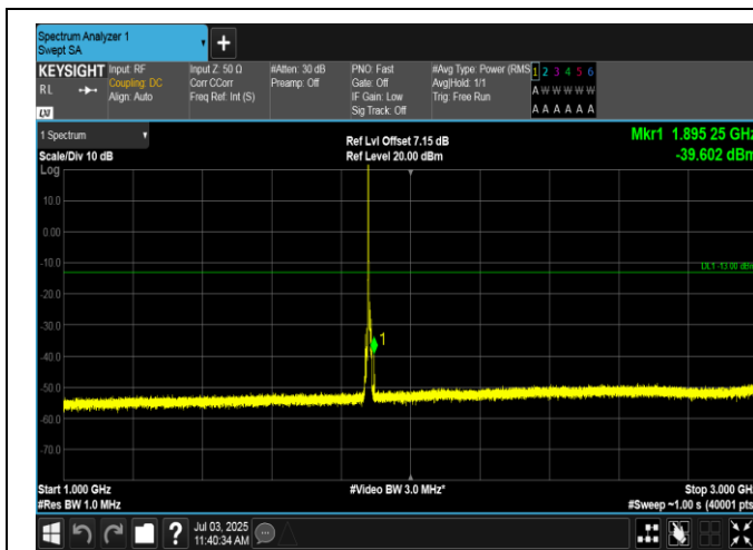
Band2-5MHz-QPSK-18900-1RB#0-1000~3000-PASS
