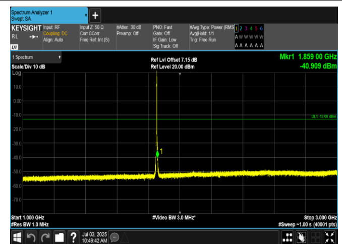
Band2-3MHz-16QAM-18615-1RB#14-1000-3000-PASS
