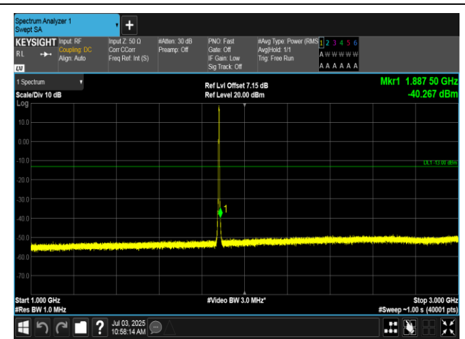
Band2-3MHz-16QAM-18900-15RB#0-1000~3000-PASS
