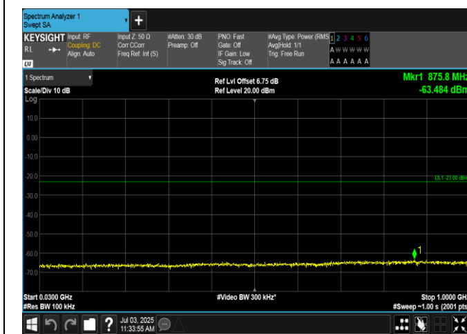
Band2-5MHz-QPSK-18625-1RB#0-30~1000-PASS
