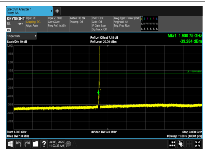
Band2-3MHz-QPSK-19185-15RB#0-1000~3000-PASS
