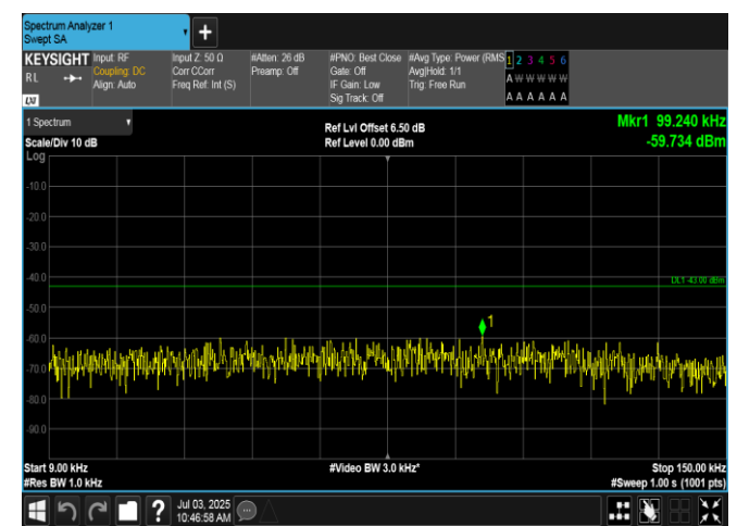
Band2-3MHz-16QAM-18615-1RB#0-0.009~0.15-PASS
