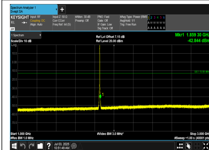
Band2-3MHz-16QAM-18615-15RB#0-1000~3000-PASS
