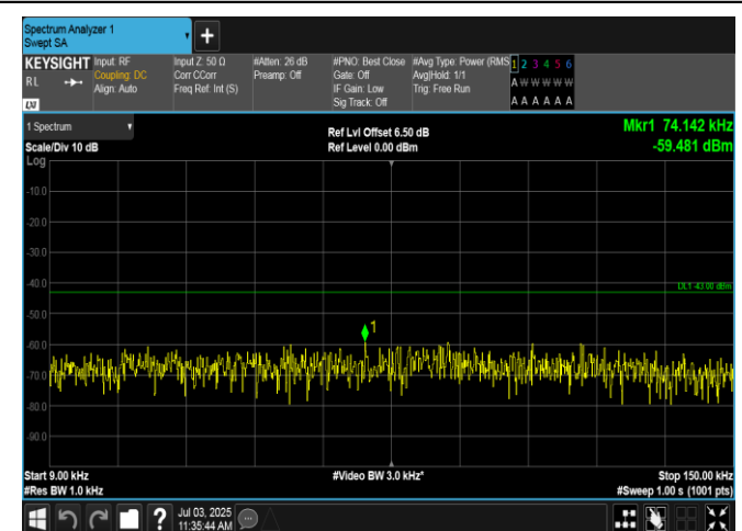
Band2-5MHz-QPSK-18625-1RB#24-0.009~0.15-PASS
