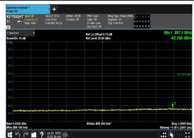
Band2-3MHz-QPSK-18900-1RB#0-30~1000-PASS
