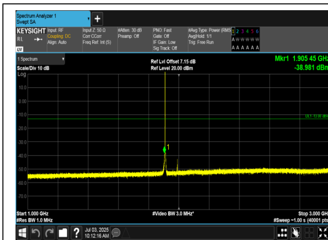
Band2-1.4MHz-16QAM-19193-1RB#0-1000-3000-PASS
