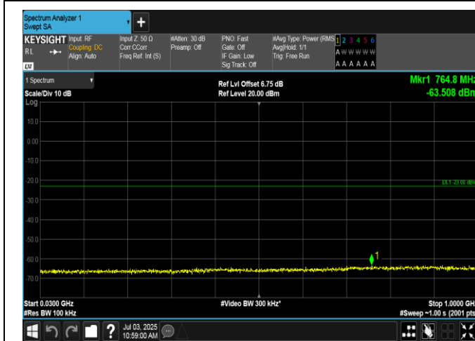
Band2-3MHz-QPSK-19185-1RB#0-30~1000-PASS
