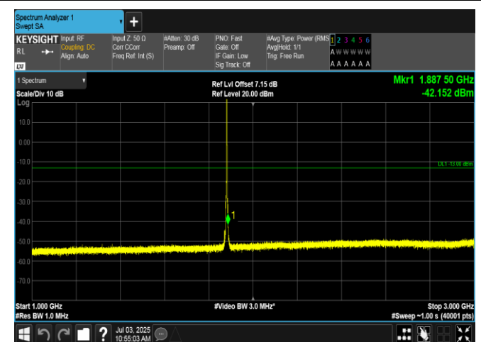
Band2-3MHz-QPSK-18900-1RB#14-1000~3000-PASS
