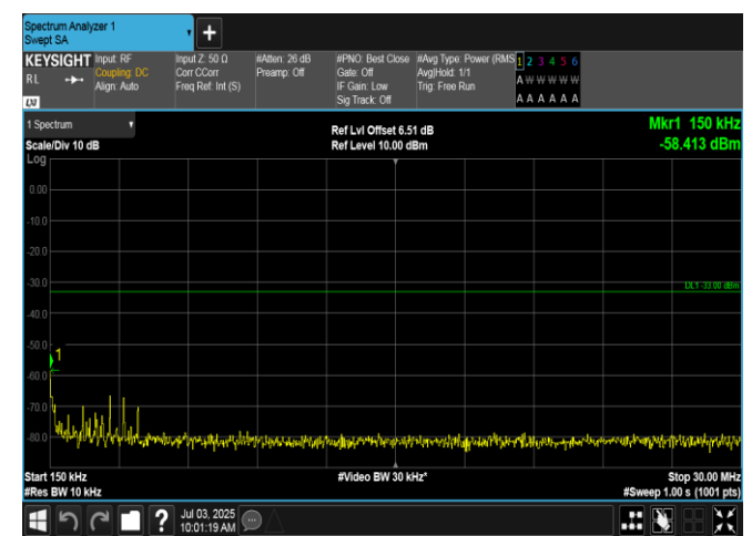
Band2-1.4MHz-16QAM-18607-1RB#5-0.15-30-PASS
