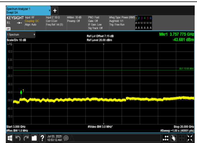
Band2-3MHz-QPSK-18900-1RB#0-3000~20000-PASS
