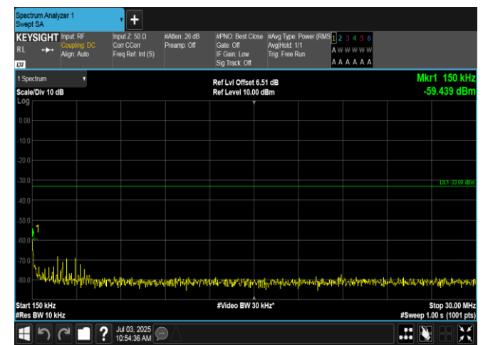
Band2-3MHz-QPSK-18900-1RB#14-0.15~30-PASS
