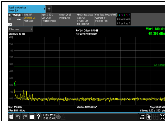
Band2-3MHz-QPSK-18615-1RB#14-0.15~30-PASS
