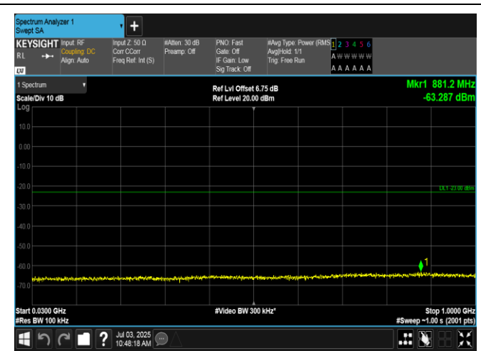
Band2-3MHz-QPSK-18615-1RB#14-30~1000-PASS
