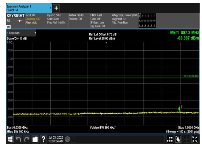
Band2-1.4MHz-16QAM-18607-6RB#0-30~1000-PASS
