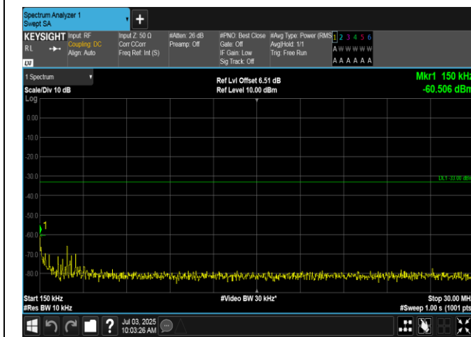
Band2-1.4MHz-16QAM-18607-6RB#0-0.15~30-PASS
