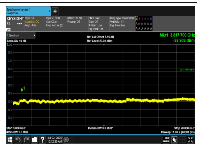
Band2-1.4MHz-16QAM-19193-1RB#0-3000-20000-PASS
