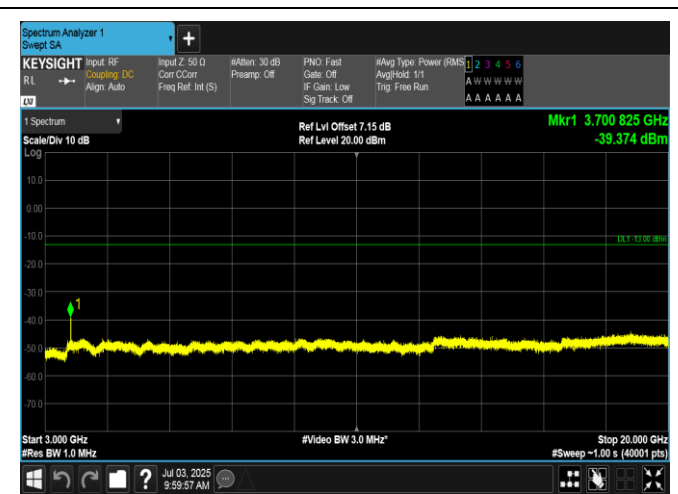
Band2-1.4MHz-16QAM-18607-1RB#0-3000-20000-PASS
