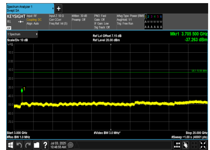
Band2-3MHz-QPSK-18615-1RB#14-3000~20000-PASS
