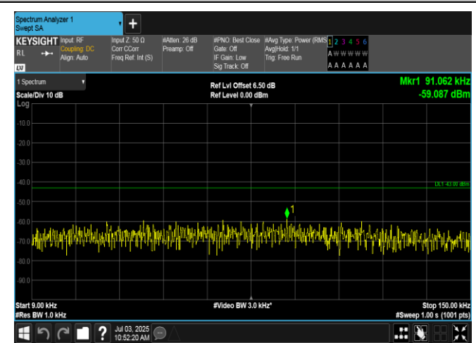
Band2-3MHz-QPSK-18900-1RB#0-0.009~0.15-PASS
