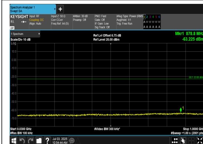
Band2-3MHz-QPSK-18900-1RB#14-30~1000-PASS
