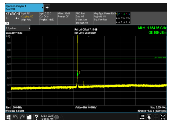
Band2-1.4MHz-16QAM-18607-1RB#5-1000-3000-PASS
