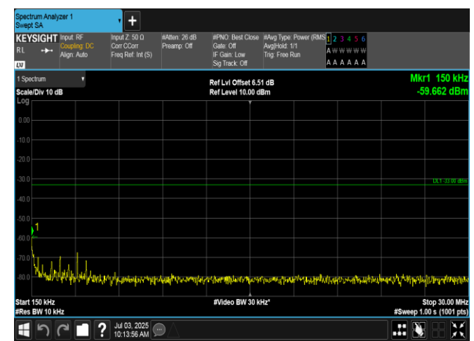
Band2-1.4MHz-16QAM-19193-1RB#5-0.15-30-PASS
