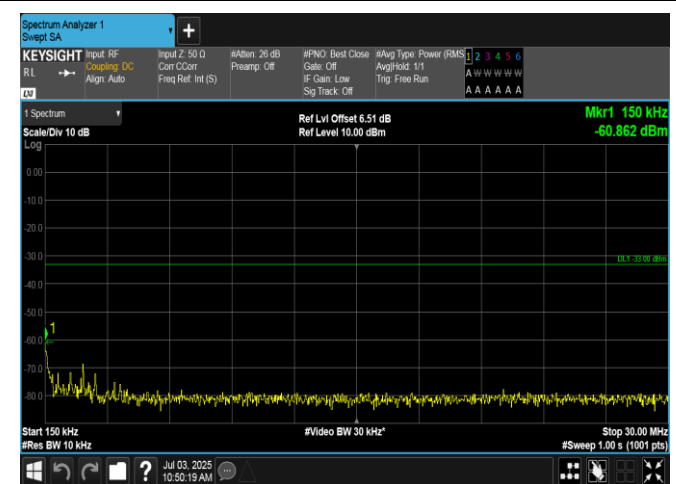
Band2-3MHz-QPSK-18615-15RB#0-0.15~30-PASS
