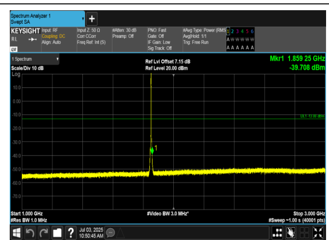
Band2-3MHz-QPSK-18615-15RB#0-1000~3000-PASS
