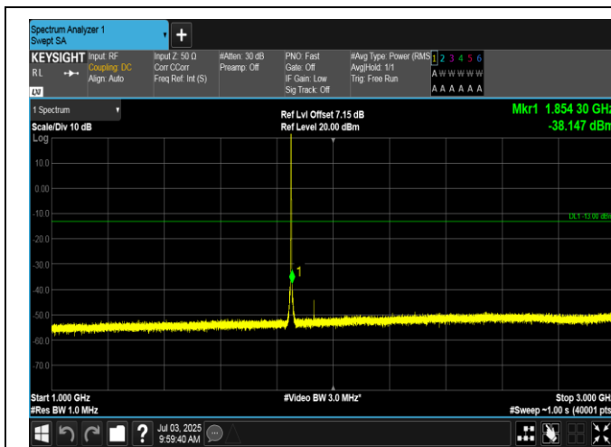
Band2-1.4MHz-16QAM-18607-1RB#0-1000-3000-PASS
