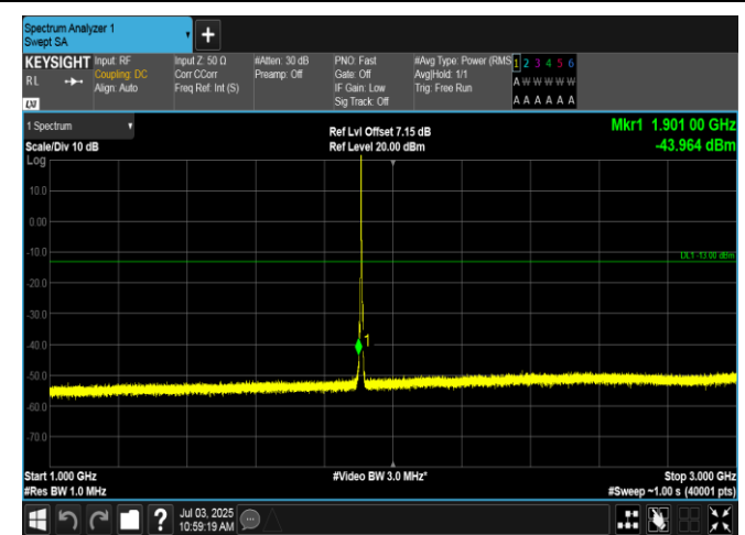
Band2-3MHz-QPSK-19185-1RB#0-1000~3000-PASS
