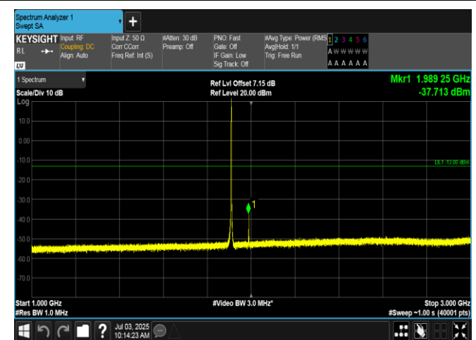
Band2-1.4MHz-16QAM-19193-1RB#5-1000-3000-PASS
