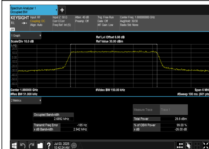
Band2-3MHz-16QAM-18900-15RB#0-PASS
