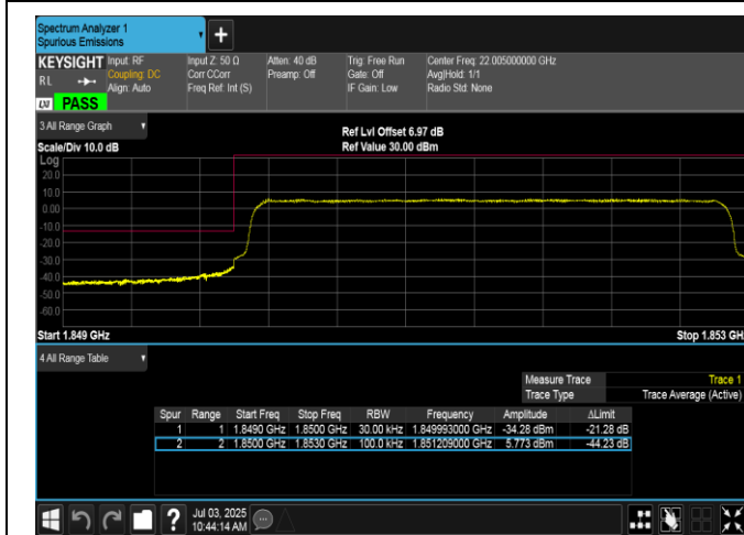
Band2-3MHz-16QAM-18615-15RB#0-PASS
