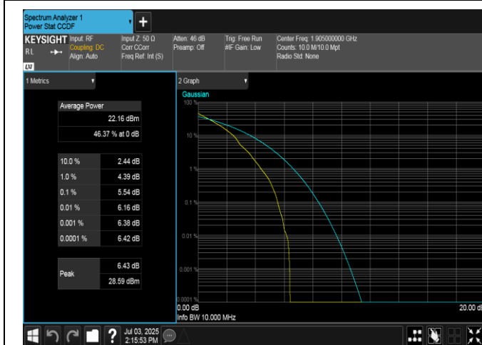
Band2-10MHz-QPSK-19150-1RB#0-PASS
