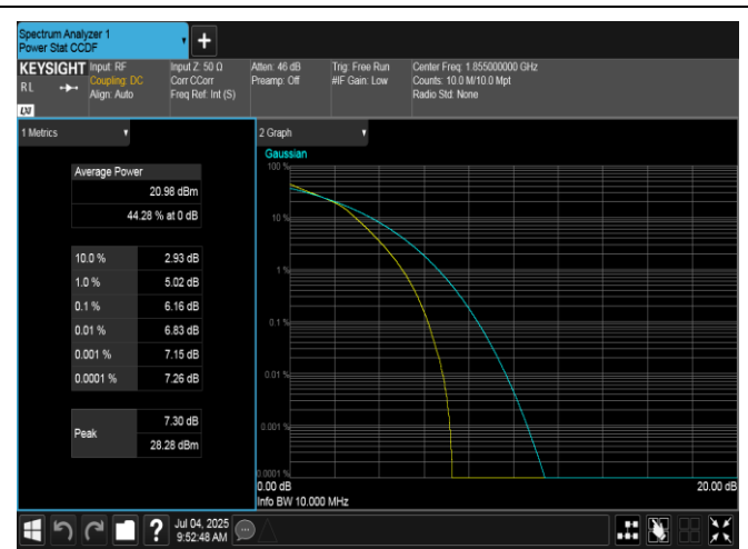
Band2-10MHz-16QAM-18650-50RB#0-PASS
