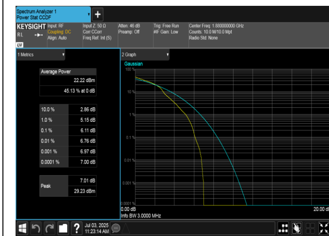
Band2-3MHz-16QAM-18900-1RB#0-PASS
