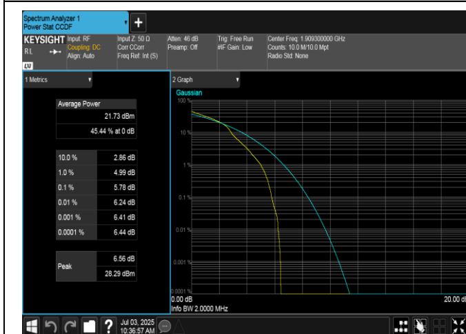
Band2-1.4MHz-16QAM-19193-1RB#0-PASS
