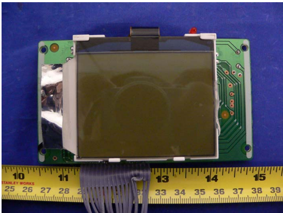
EUT –Display View
