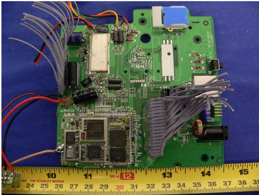
EUT –Main Board Without Shielding View
