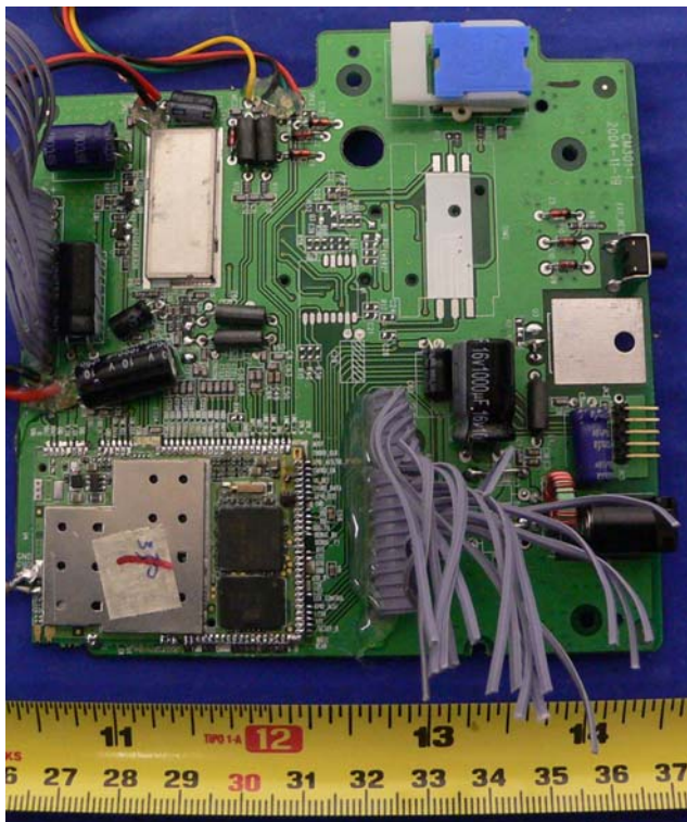
EUT –Main Board View
