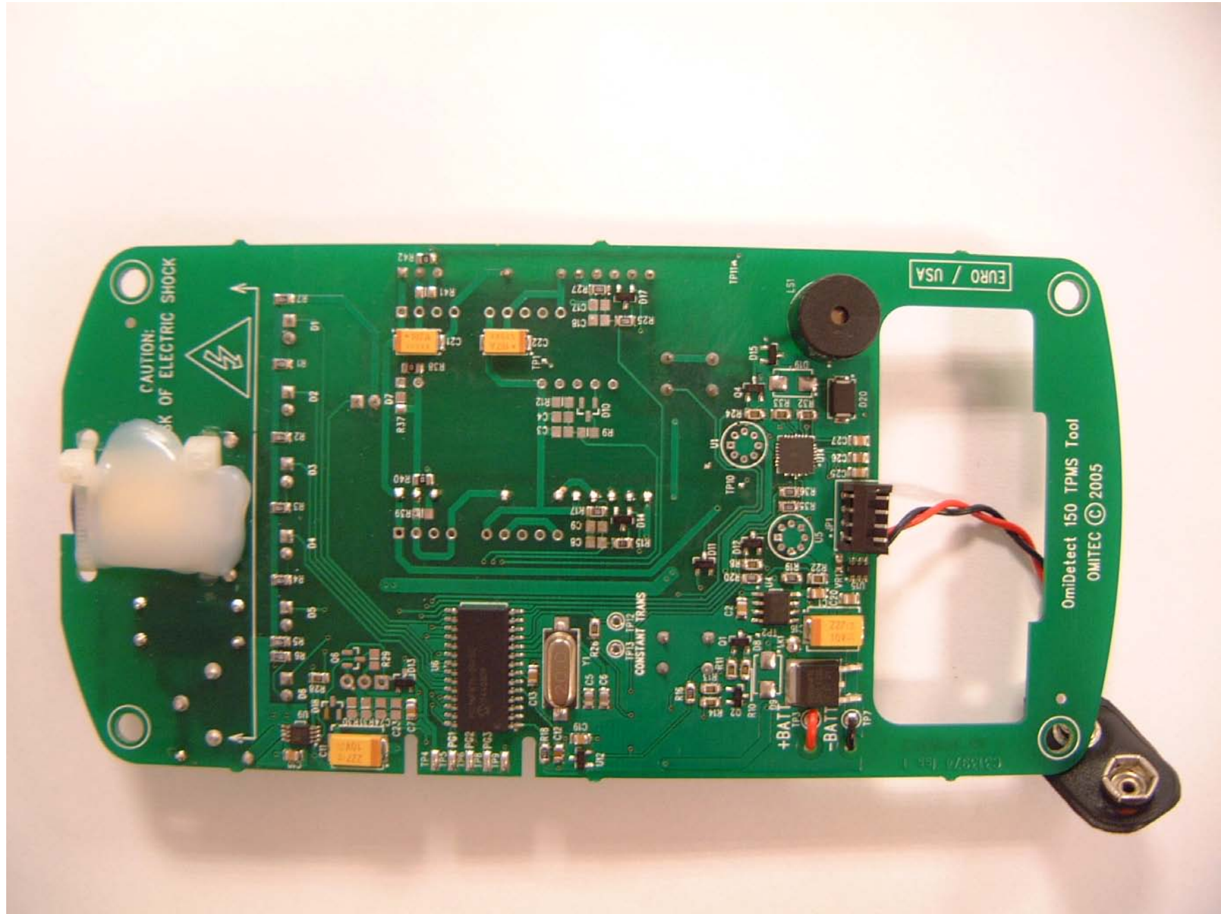
OmiDetect 50 Internal Photograph – PCB Rear
