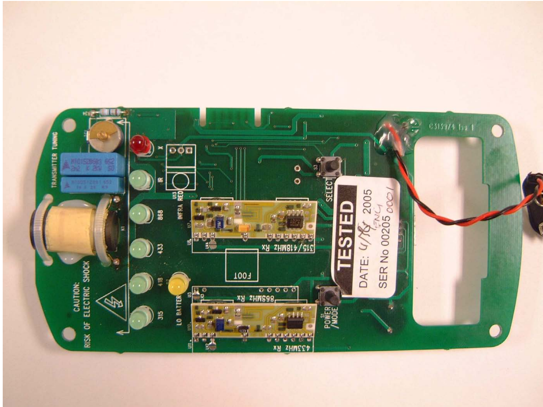
OmiDetect 50 Internal Photograph – PCB Front
