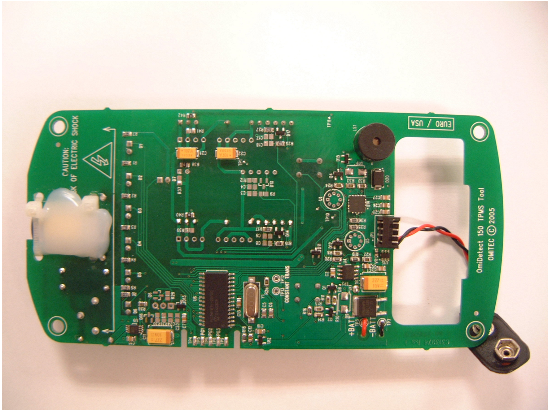
OmiDetect 100 Internal Photograph – PCB Rear
